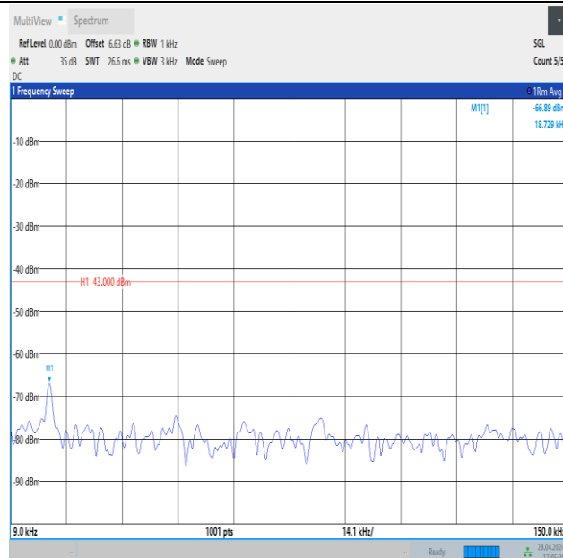
Band4_5MHz_16QAM_20175_25RB#0_0.009~0.15_0.009~0.15
