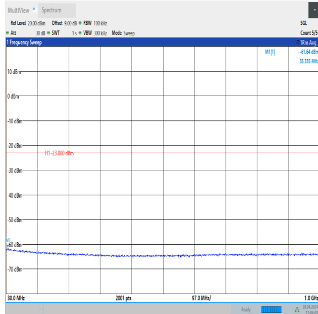
Band4_5MHz_16QAM_20175_1RB#24_30~1000_30~1000
