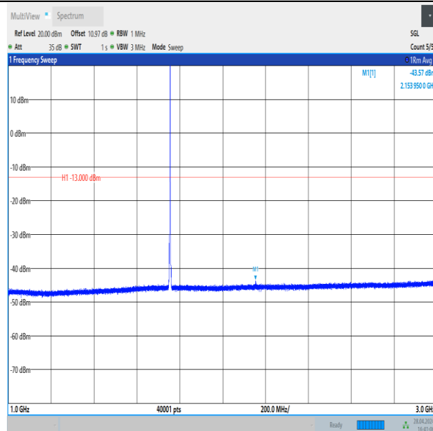
Band4_3MHz_QPSK_20385_1RB#14_1000~3000_1000~3000
