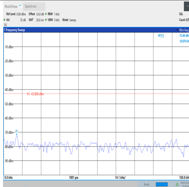
Band4_3MHz_16QAM_20385_15RB#0_0.009~0.15_0.009~0.15
