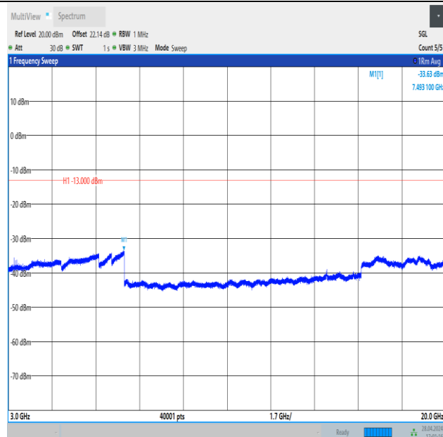
Band4_5MHz_16QAM_19975_25RB#0_3000~20000_3000~20000
