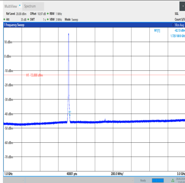
Band4_5MHz_16QAM_19975_25RB#0_1000~3000_1000~3000
