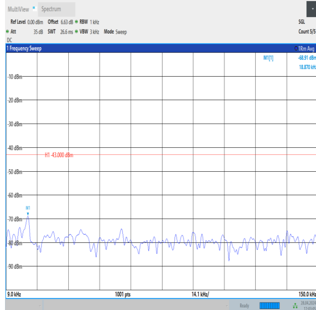
Band4_5MHz_QPSK_20175_1RB#24_0.009~0.15_0.009~0.15
