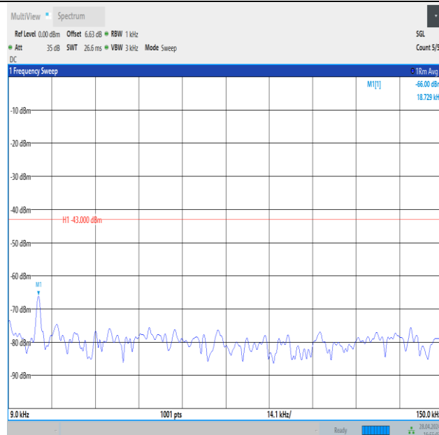
Band4_20MHz_QPSK_20300_100RB#0_0.009~0.15_0.009~0.15
