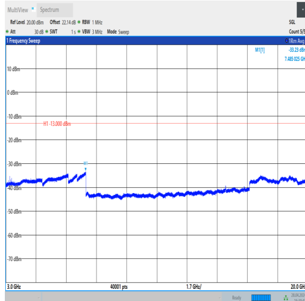
Band4_3MHz_QPSK_20385_1RB#0_3000~20000_3000~20000
