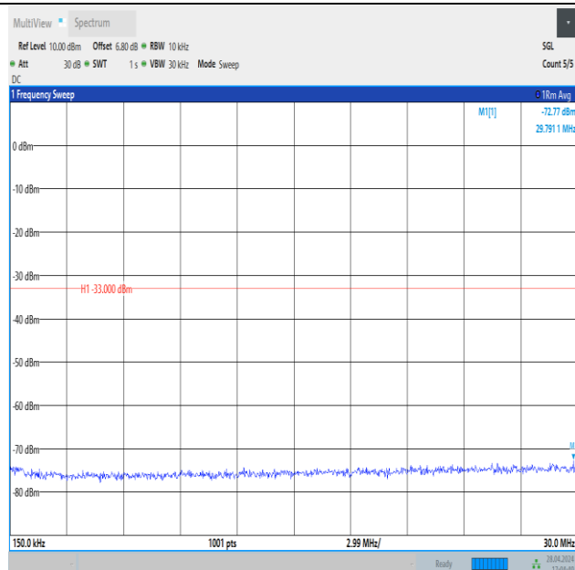
Band4_5MHz_QPSK_20175_25RB#0_0.15~30_0.15~30
