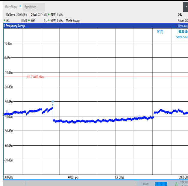
Band4_20MHz_QPSK_20300_100RB#0_3000~20000_3000~20000
