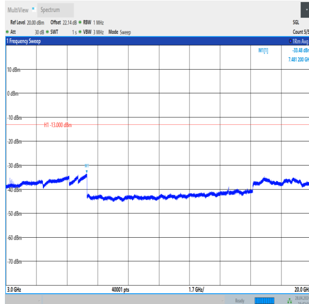
Band4_3MHz_QPSK_20385_15RB#0_3000~20000_3000~20000
