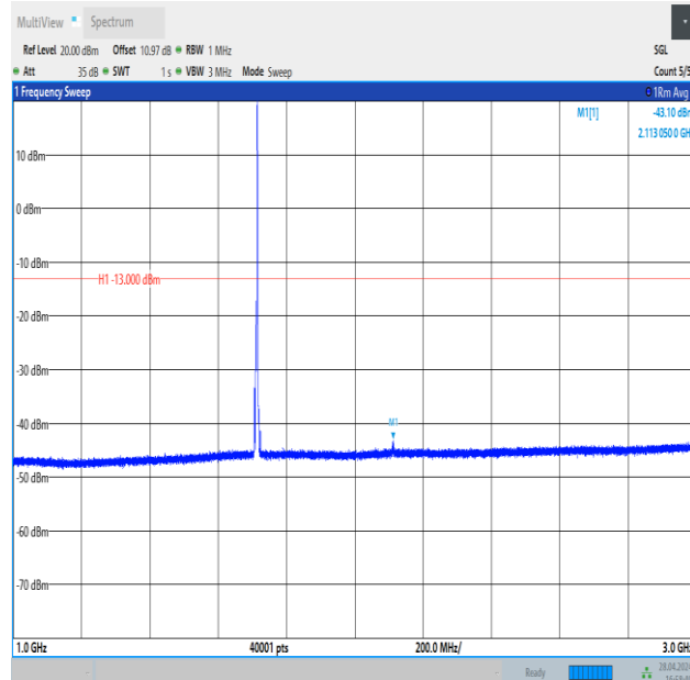
Band4_5MHz_QPSK_19975_1RB#24_1000~3000_1000~3000
