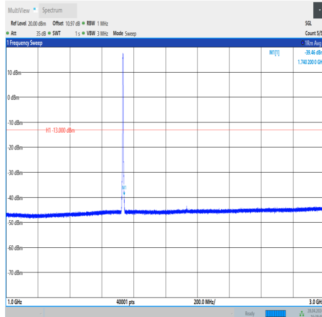
Band4_3MHz_16QAM_20175_15RB#0_1000~3000_1000~3000
