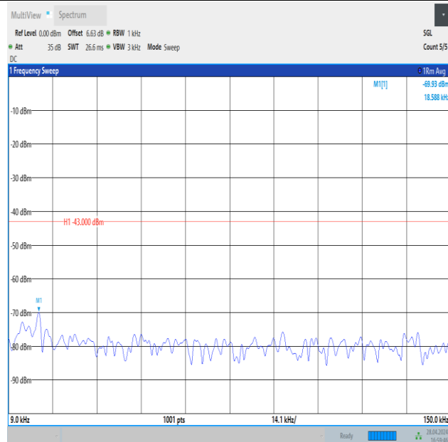
Band4_5MHz_QPSK_19975_25RB#0_0.009~0.15_0.009~0.15
