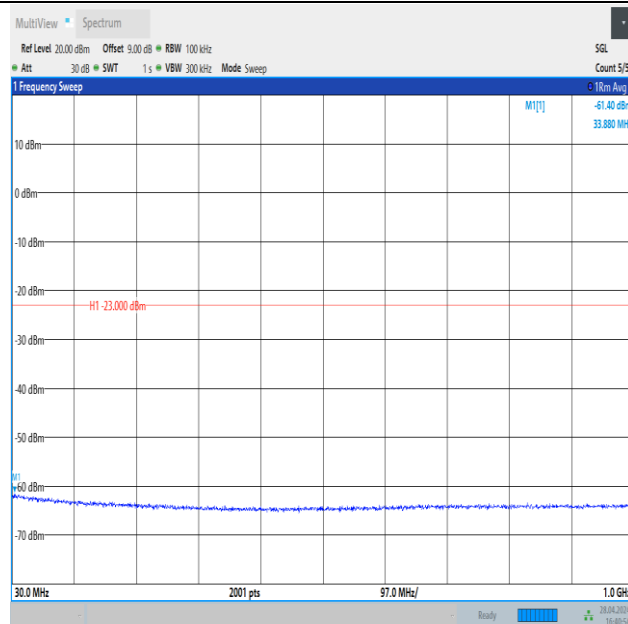
Band4_3MHz_QPSK_20385_1RB#14_30~1000_30~1000
