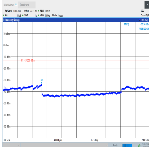
Band4_5MHz_16QAM_20175_1RB#0_3000~20000_3000~20000
