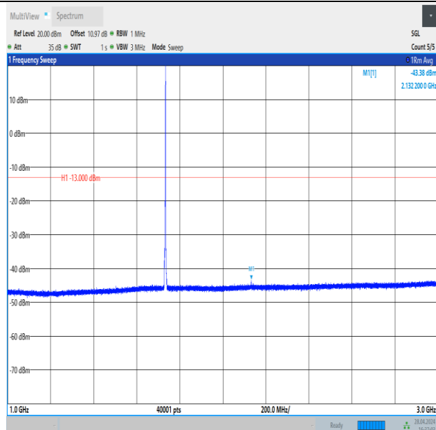
Band4_3MHz_16QAM_20175_1RB#14_1000~3000_1000~3000
