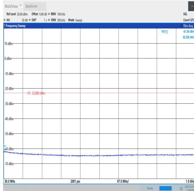
Band4_5MHz_16QAM_19975_25RB#0_30~1000_30~1000
