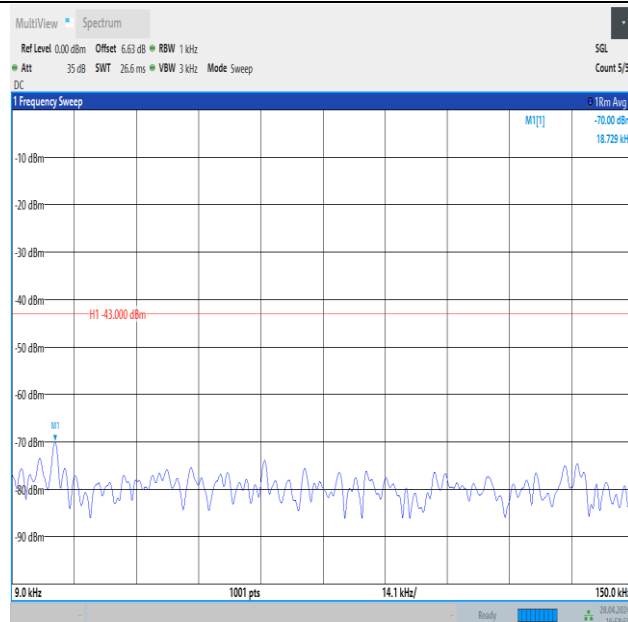
Band4_5MHz_16QAM_19975_1RB#24_0.009~0.15_0.009~0.15
