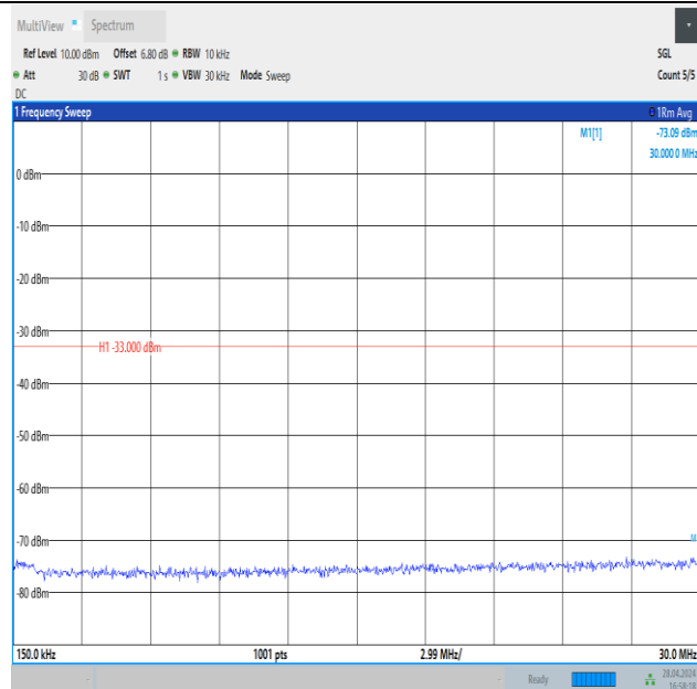
Band4_5MHz_QPSK_19975_1RB#24_0.15~30_0.15~30
