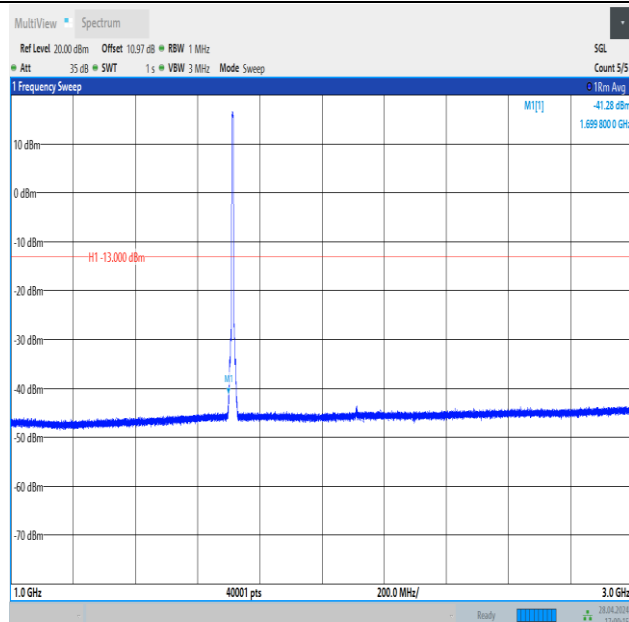
Band4_5MHz_QPSK_19975_25RB#0_1000~3000_1000~3000
