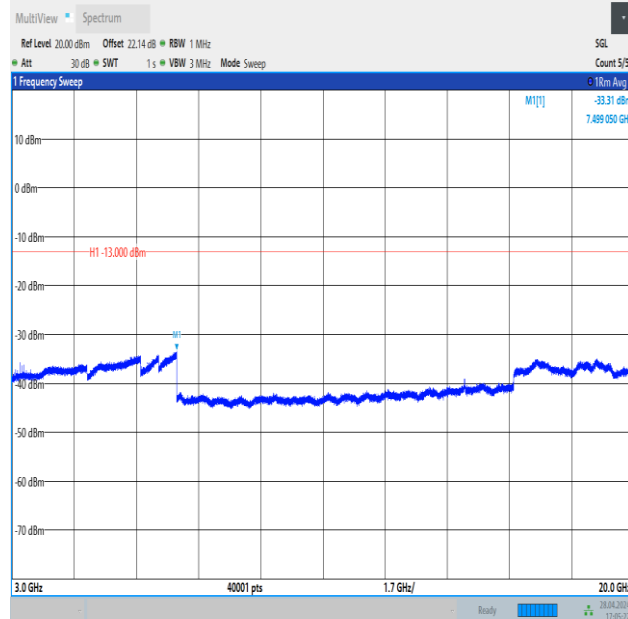
Band4_5MHz_QPSK_20175_25RB#0_3000~20000_3000~20000
