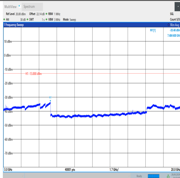
Band4_5MHz_16QAM_19975_1RB#24_3000~20000_3000~20000
