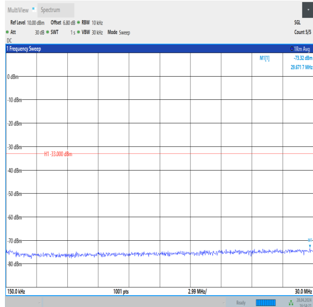
Band4_20MHz_QPSK_20175_100RB#0_0.15~30_0.15~30
