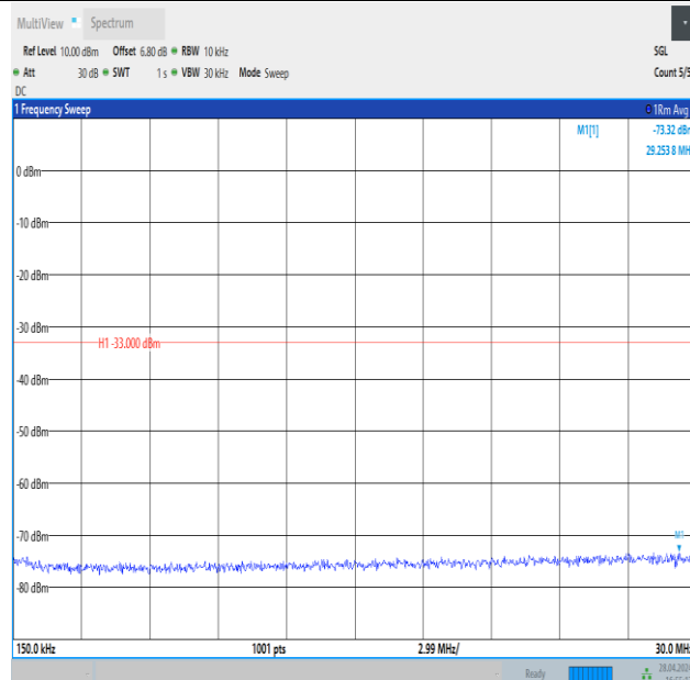
Band4_20MHz_QPSK_20300_100RB#0_0.15~30_0.15~30
