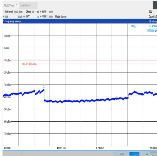
Band4_3MHz_16QAM_20385_15RB#0_3000~20000_3000~20000
