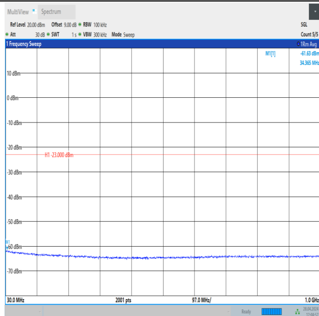
Band4_5MHz_QPSK_20175_25RB#0_30~1000_30~1000
