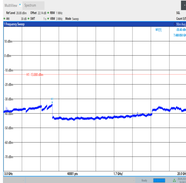
Band4_5MHz_QPSK_19975_1RB#24_3000~20000_3000~20000
