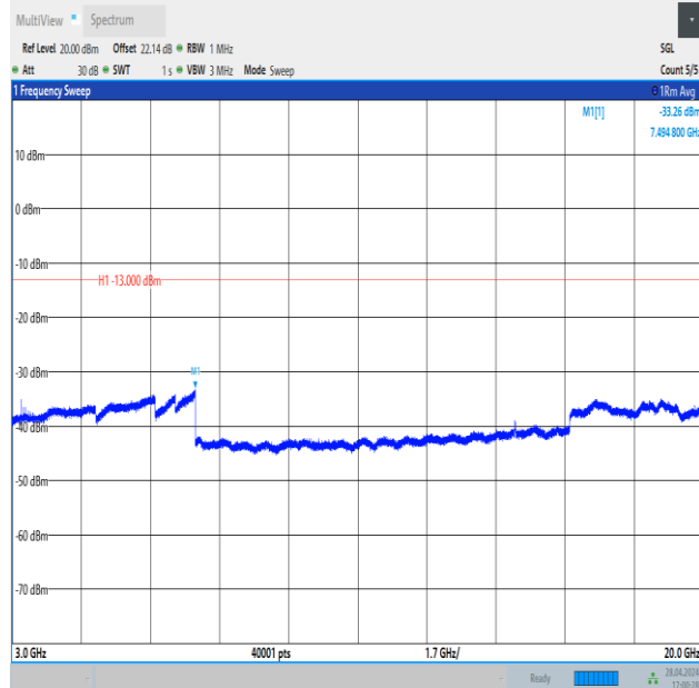
Band4_5MHz_QPSK_19975_25RB#0_3000~20000_3000~20000
