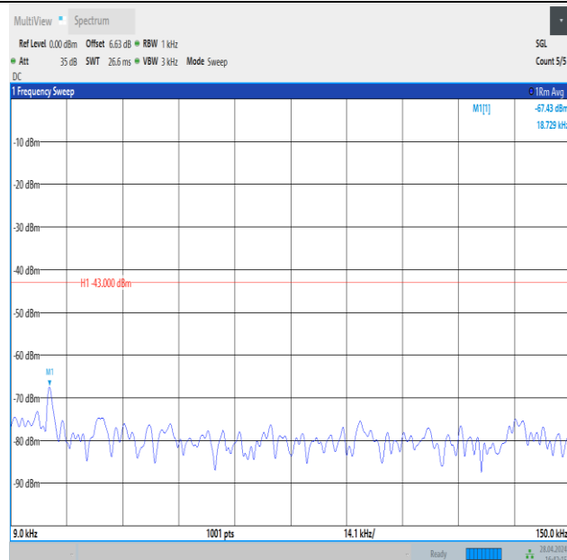
Band4_3MHz_QPSK_20385_15RB#0_0.009~0.15_0.009~0.15
