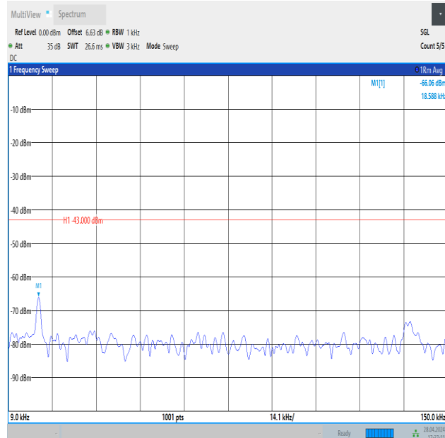
Band4_10MHz_16QAM_20175_1RB#0_0.009~0.15_0.009~0.15
