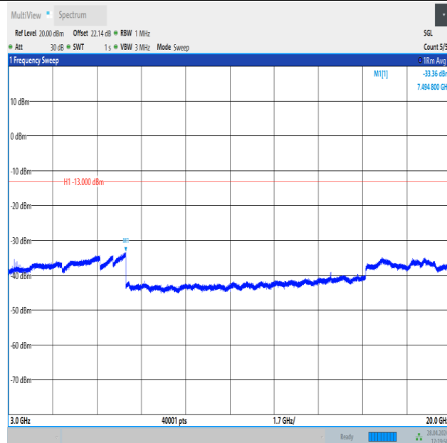
Band4_20MHz_QPSK_20175_1RB#99_3000~20000_3000~20000
