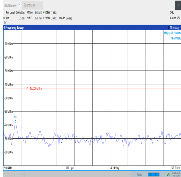
Band4_20MHz_QPSK_20050_1RB#0_0.009~0.15_0.009~0.15
