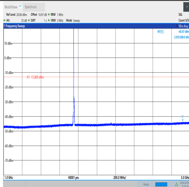
Band4_5MHz_16QAM_20375_1RB#0_1000~3000_1000~3000
