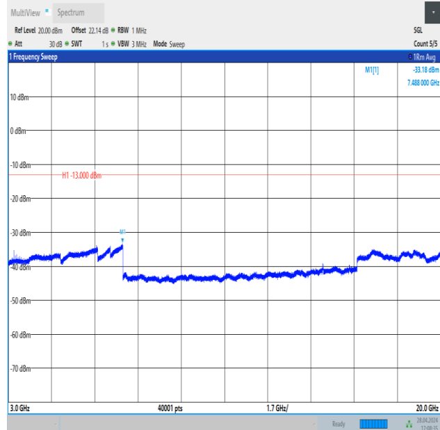
Band4_5MHz_QPSK_20375_1RB#24_3000~20000_3000~20000
