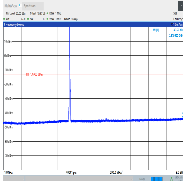
Band4_10MHz_QPSK_20175_1RB#0_1000~3000_1000~3000
