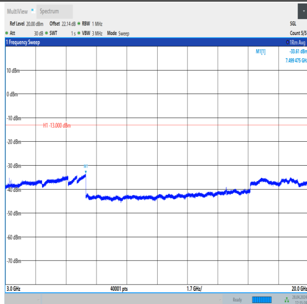
Band4_10MHz_QPSK_20000_1RB#49_3000~20000_3000~20000
