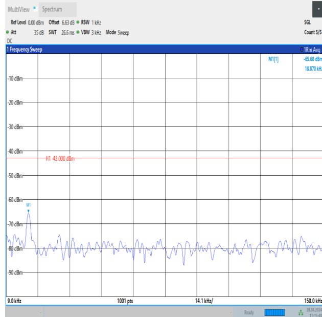
Band4_20MHz_QPSK_20050_1RB#99_0.009~0.15_0.009~0.15
