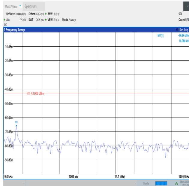
Band4_20MHz_QPSK_20300_1RB#99_0.009~0.15_0.009~0.15
