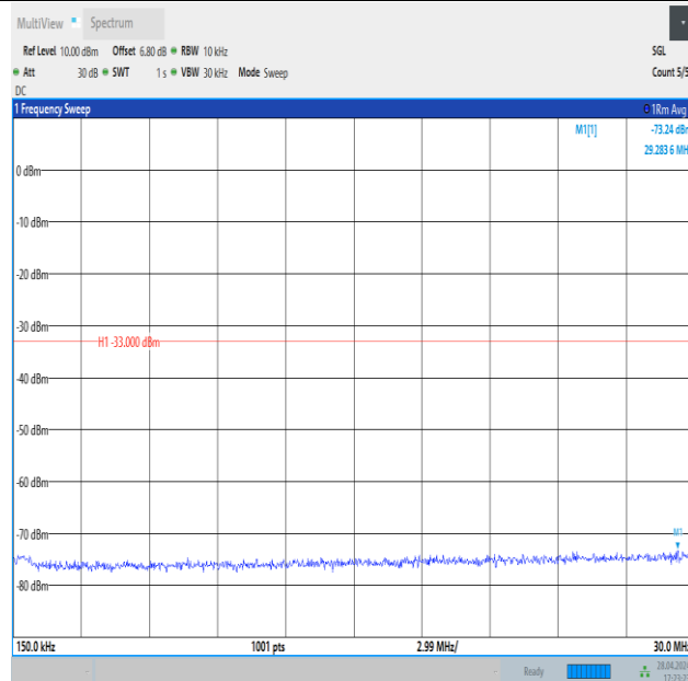
Band4_20MHz_16QAM_20300_1RB#99_0.15~30_0.15~30
