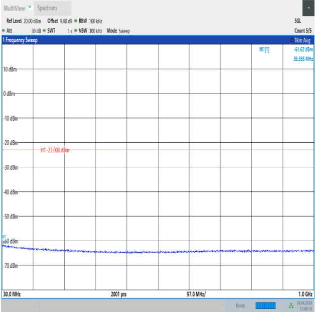
Band4_5MHz_QPSK_20375_1RB#24_30~1000_30~1000
