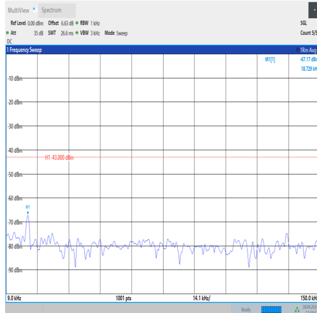
Band4_20MHz_16QAM_20175_1RB#99_0.009~0.15_0.009~0.15
