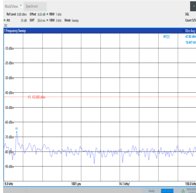
Band4_5MHz_16QAM_20375_25RB#0_0.009~0.15_0.009~0.15
