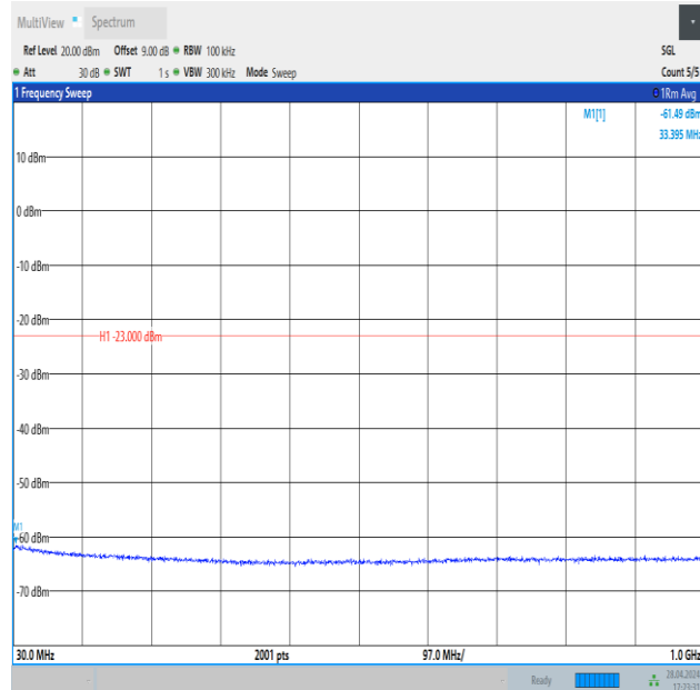
Band4_20MHz_16QAM_20300_1RB#99_30~1000_30~1000
