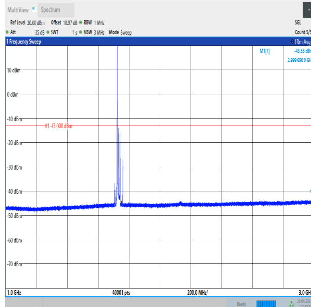
Band4_20MHz_QPSK_20175_1RB#0_1000~3000_1000~3000
