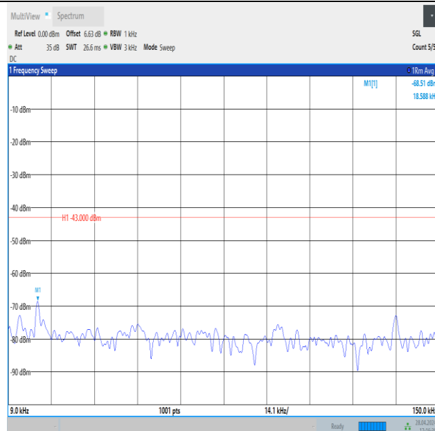
Band4_20MHz_16QAM_20050_1RB#99_0.009~0.15_0.009~0.15
