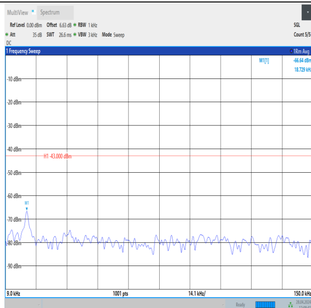
Band4_5MHz_16QAM_20375_1RB#24_0.009~0.15_0.009~0.15
