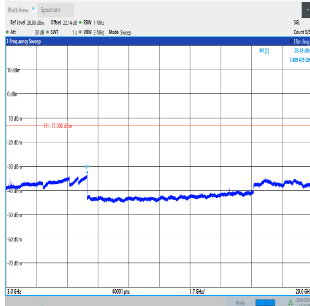
Band4_5MHz_16QAM_20375_25RB#0_3000~20000_3000~20000
