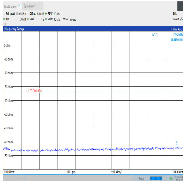
Band4_5MHz_16QAM_20375_1RB#24_0.15~30_0.15~30
