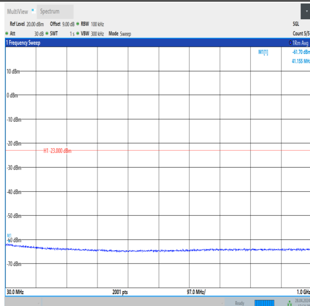
Band4_15MHz_QPSK_20175_75RB#0_30~1000_30~1000
