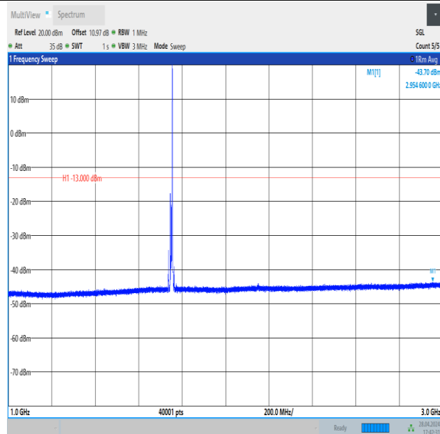
Band4_10MHz_16QAM_20350_1RB#49_1000~3000_1000~3000
