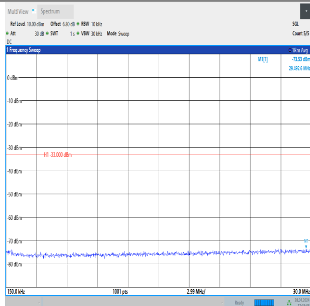
Band4_10MHz_QPSK_20175_1RB#49_0.15~30_0.15~30
