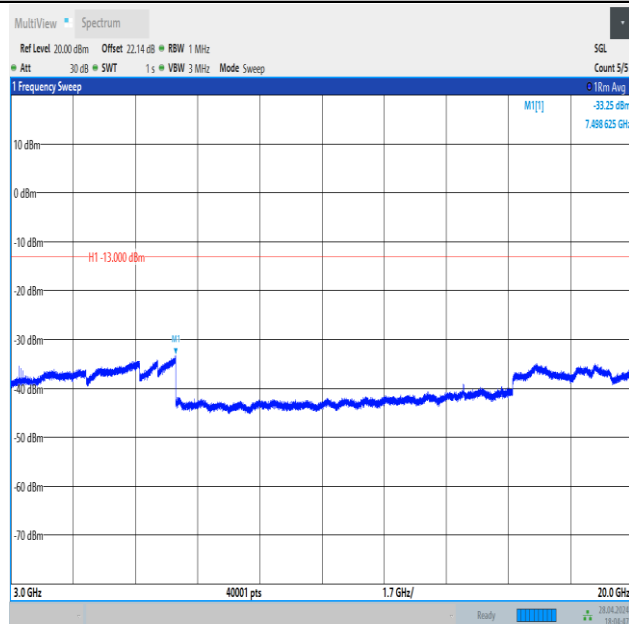
Band4_15MHz_QPSK_20325_1RB#74_3000~20000_3000~20000
