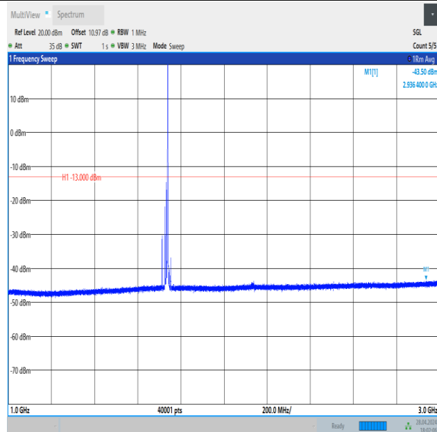
Band4_15MHz_16QAM_20175_1RB#74_1000~3000_1000~3000
