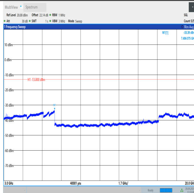
Band4_10MHz_QPSK_20350_50RB#0_3000~20000_3000~20000
