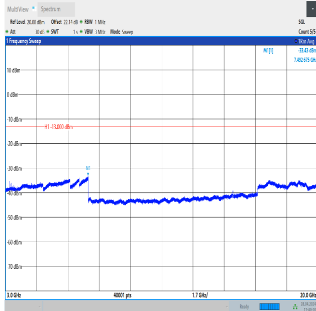
Band4_10MHz_QPSK_20350_1RB#0_3000~20000_3000~20000
