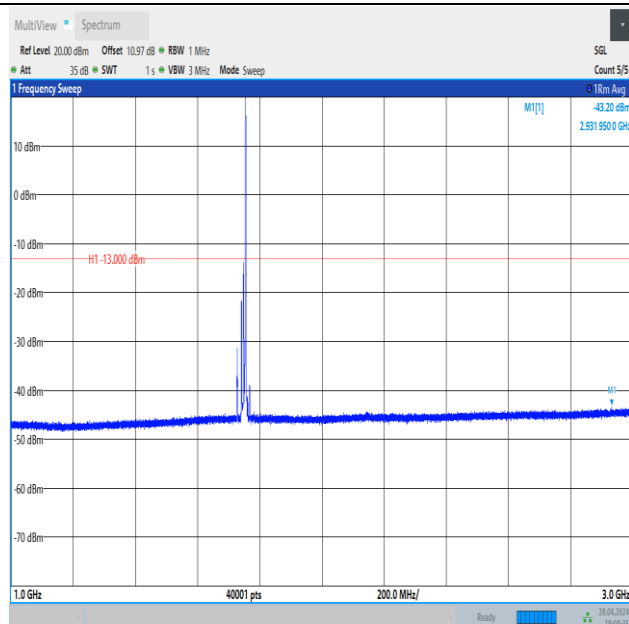
Band4_15MHz_QPSK_20325_1RB#74_1000~3000_1000~3000
