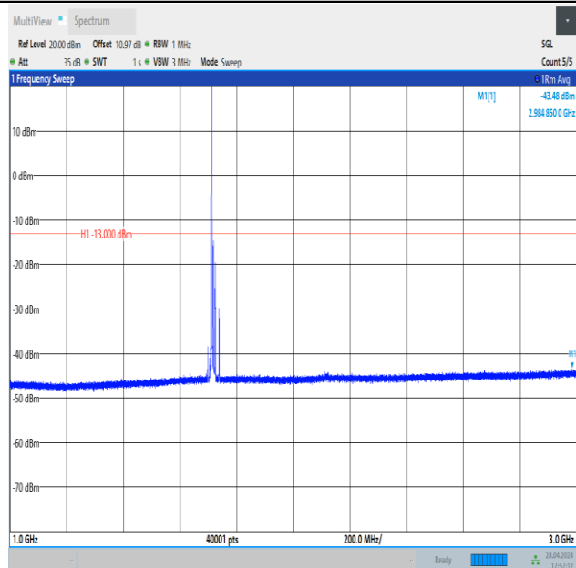
Band4_15MHz_16QAM_20025_1RB#0_1000~3000_1000~3000
