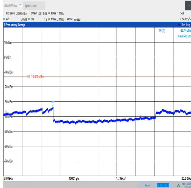
Band4_15MHz_QPSK_20025_1RB#0_3000~20000_3000~20000
