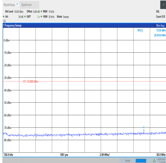
Band4_15MHz_QPSK_20325_75RB#0_0.15~30_0.15~30
