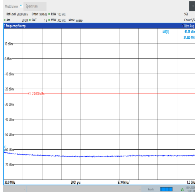
Band4_15MHz_16QAM_20325_1RB#0_30~1000_30~1000
