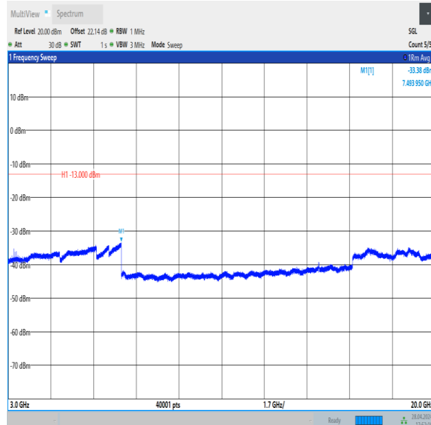
Band4_10MHz_QPSK_20175_50RB#0_3000~20000_3000~20000
