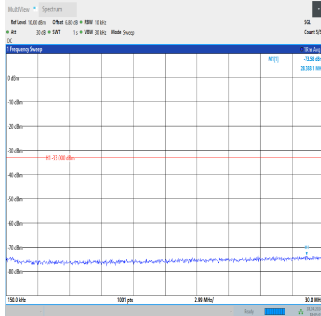
Band4_15MHz_16QAM_20325_1RB#74_0.15~30_0.15~30
