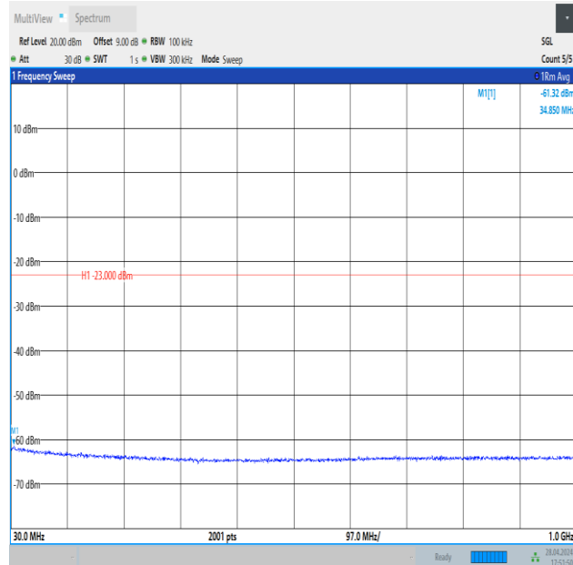
Band4_10MHz_QPSK_20175_50RB#0_30~1000_30~1000
