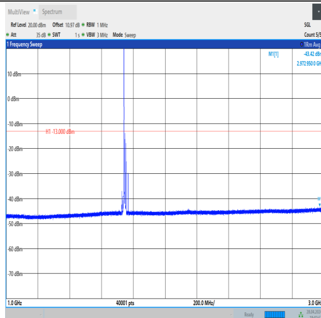
Band4_15MHz_QPSK_20325_1RB#0_1000~3000_1000~3000
