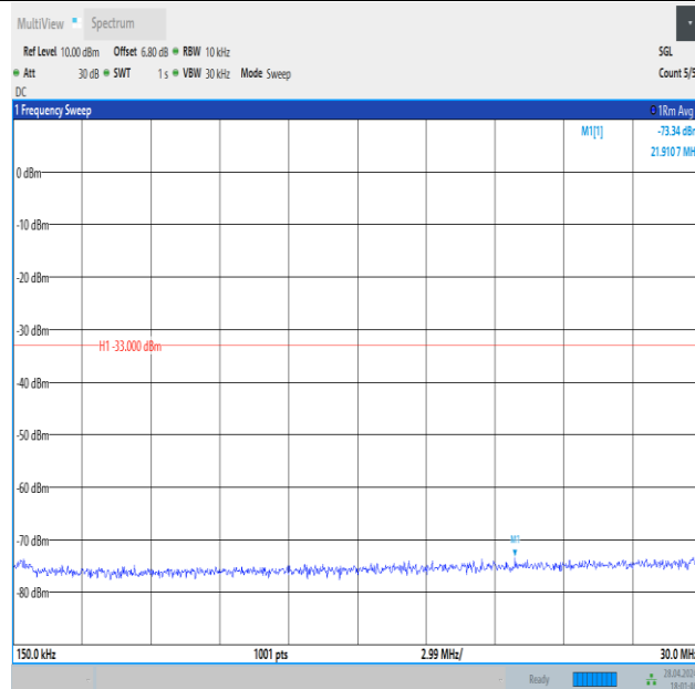
Band4_15MHz_16QAM_20175_1RB#74_0.15~30_0.15~30
