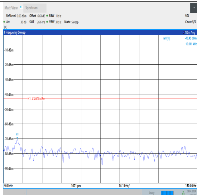
Band4_15MHz_QPSK_20325_75RB#0_0.009~0.15_0.009~0.15
