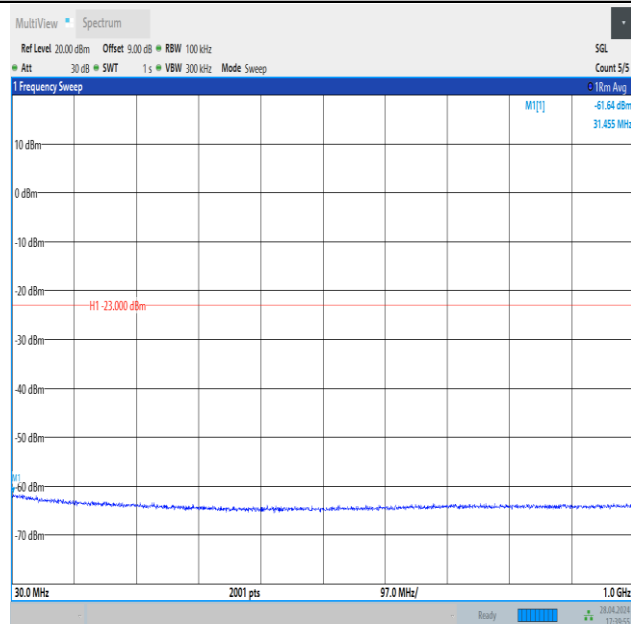
Band4_10MHz_QPSK_20350_1RB#0_30~1000_30~1000
