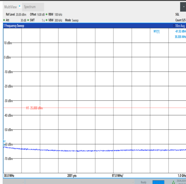
Band41_20MHz_QPSK_39750_1RB#99_30~1000_30~1000
