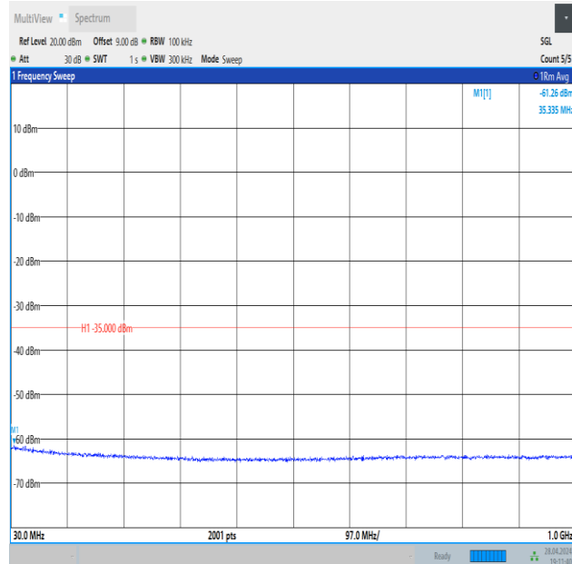
Band41_15MHz_QPSK_40620_1RB#0_30~1000_30~1000
