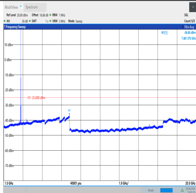
Band41_20MHz_16QAM_41490_1RB#0_1000~20000_1000~20000
