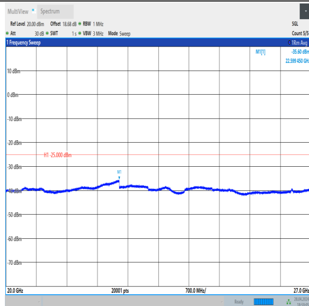
Band41_20MHz_16QAM_40620_1RB#0_20000~27000_20000~27000
