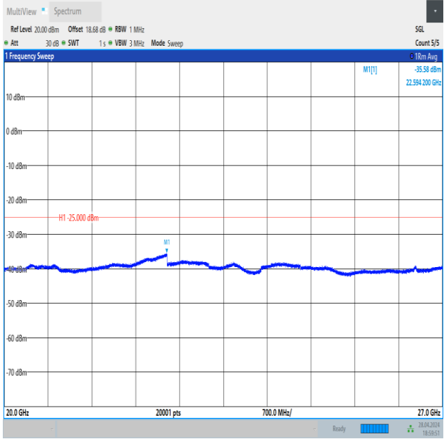
Band41_20MHz_QPSK_40620_1RB#99_20000~27000_20000~27000
