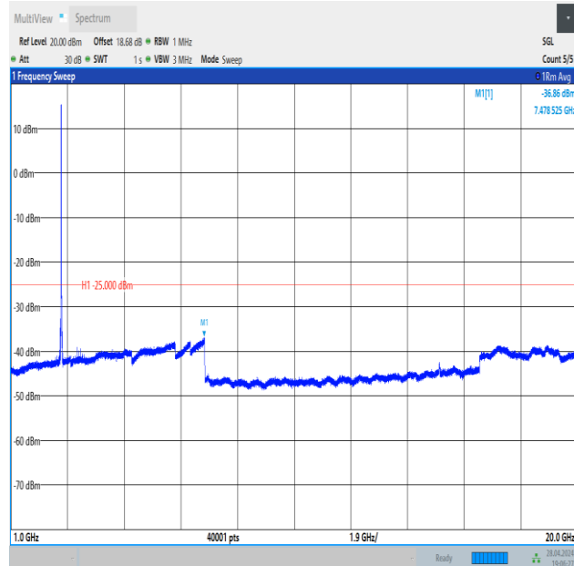
Band41_15MHz_QPSK_41515_75RB#0_1000~20000_1000~20000
