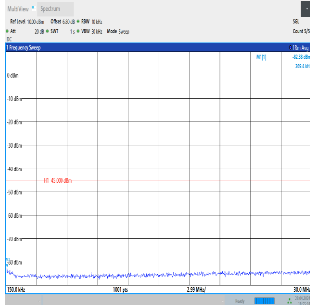
Band41_20MHz_16QAM_39750_1RB#0_0.15~30_0.15~30
