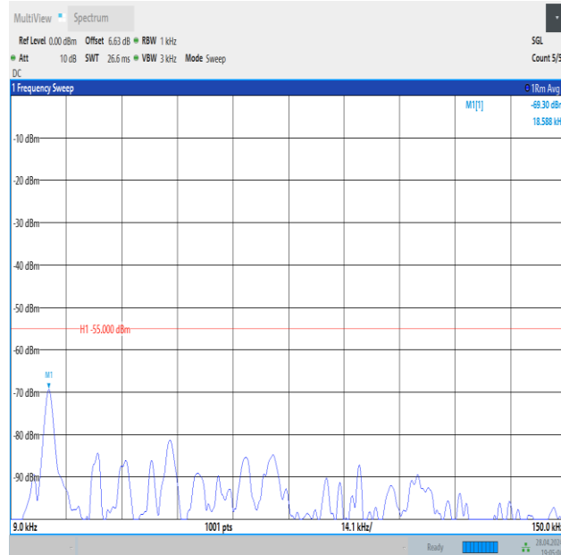
Band41_15MHz_QPSK_40620_75RB#0_0.009~0.15_0.009~0.15
