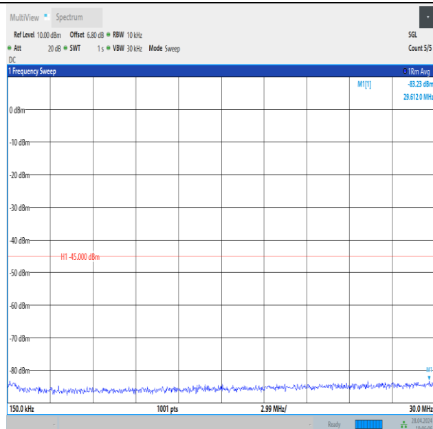
Band41_15MHz_QPSK_41515_75RB#0_0.15~30_0.15~30
