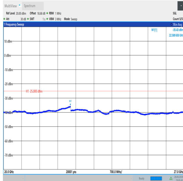
Band41_15MHz_QPSK_40620_75RB#0_20000~27000_20000~27000
