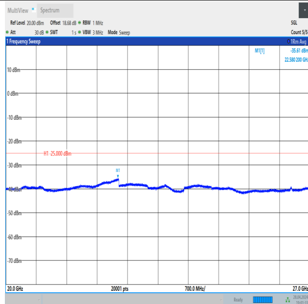
Band41_20MHz_QPSK_41490_1RB#0_20000~27000_20000~27000
