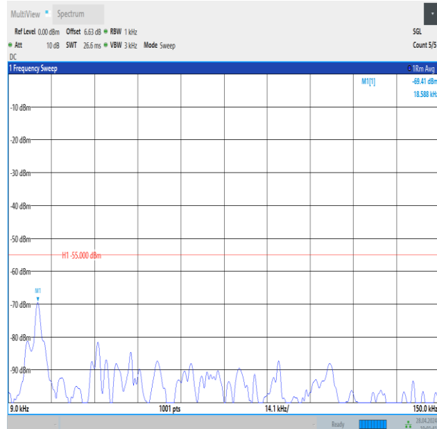
Band41_20MHz_16QAM_41490_1RB#0_0.009~0.15_0.009~0.15
