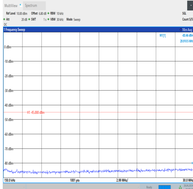
Band41_15MHz_QPSK_39725_1RB#74_0.15~30_0.15~30
