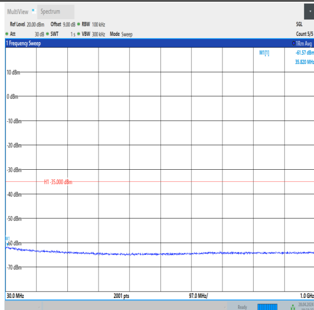
Band41_20MHz_QPSK_40620_1RB#99_30~1000_30~1000
