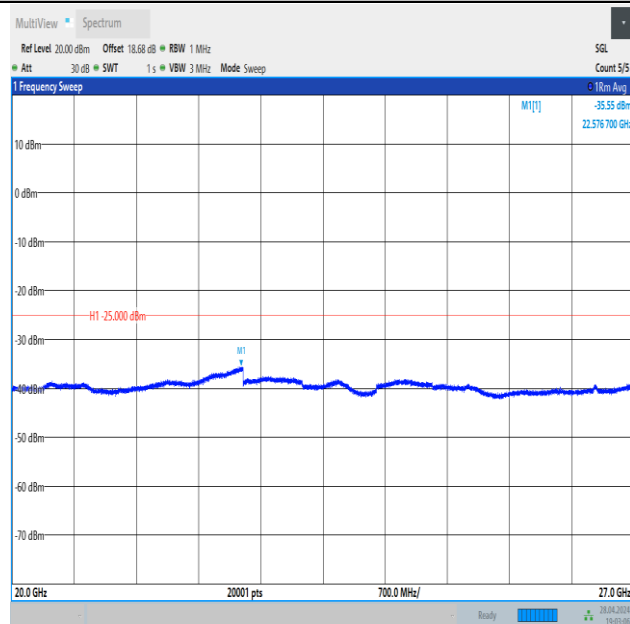
Band41_20MHz_QPSK_41490_1RB#99_20000~27000_20000~27000
