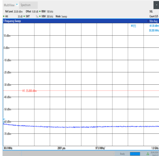
Band41_20MHz_16QAM_41490_1RB#0_30~1000_30~1000
