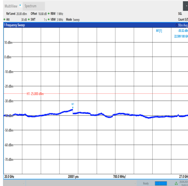
Band41_20MHz_16QAM_41490_1RB#99_20000~27000_20000~27000
