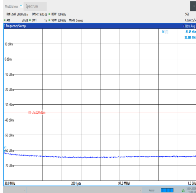
Band41_15MHz_QPSK_39725_1RB#74_30~1000_30~1000
