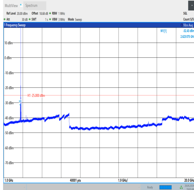
Band41_20MHz_16QAM_41490_1RB#99_1000~20000_1000~20000
