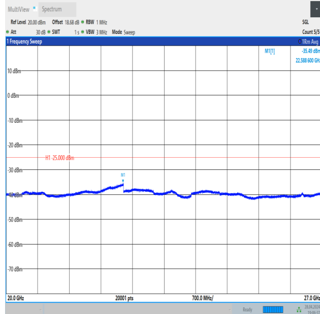
Band41_15MHz_QPSK_41515_75RB#0_20000~27000_20000~27000
