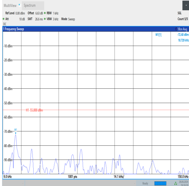
Band41_15MHz_16QAM_39725_1RB#74_0.009~0.15_0.009~0.15
