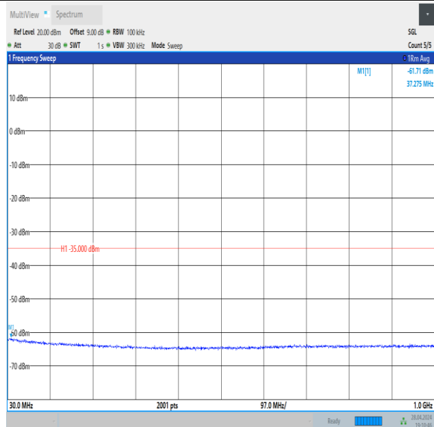
Band41_15MHz_16QAM_39725_1RB#74_30~1000_30~1000
