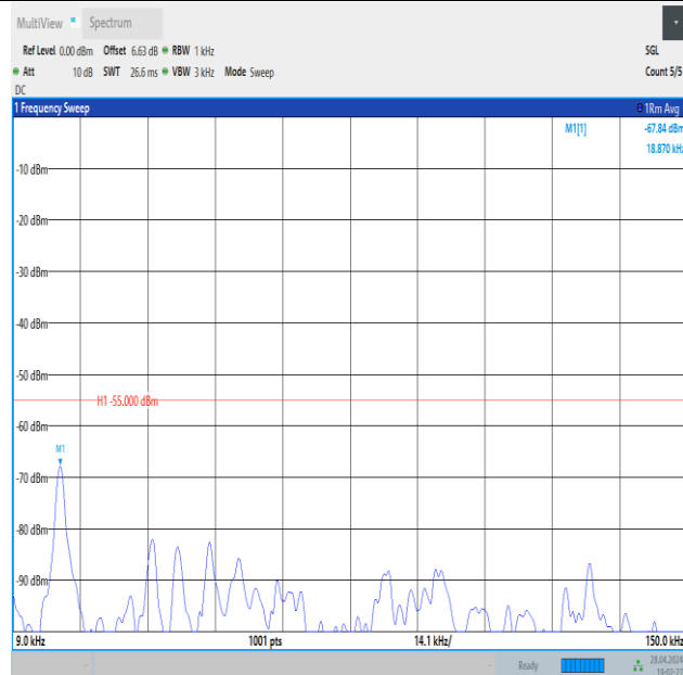
Band41_20MHz_QPSK_41490_1RB#99_0.009~0.15_0.009~0.15
