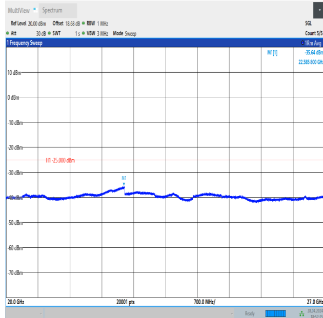
Band41_20MHz_16QAM_39750_1RB#99_20000~27000_20000~27000
