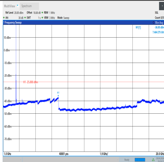
Band41_15MHz_QPSK_39725_1RB#74_1000~20000_1000~20000
