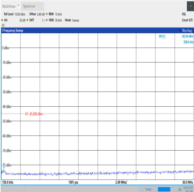
Band41_20MHz_QPSK_40620_1RB#0_0.15~30_0.15~30
