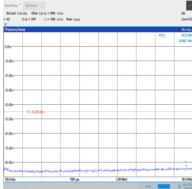
Band41_20MHz_16QAM_41490_1RB#0_0.15~30_0.15~30
