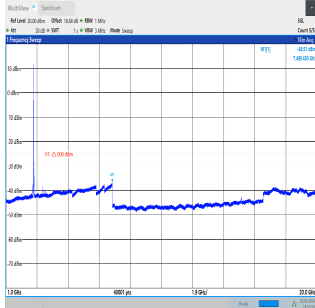
Band41_20MHz_QPSK_41490_100RB#0_1000~20000_1000~20000
