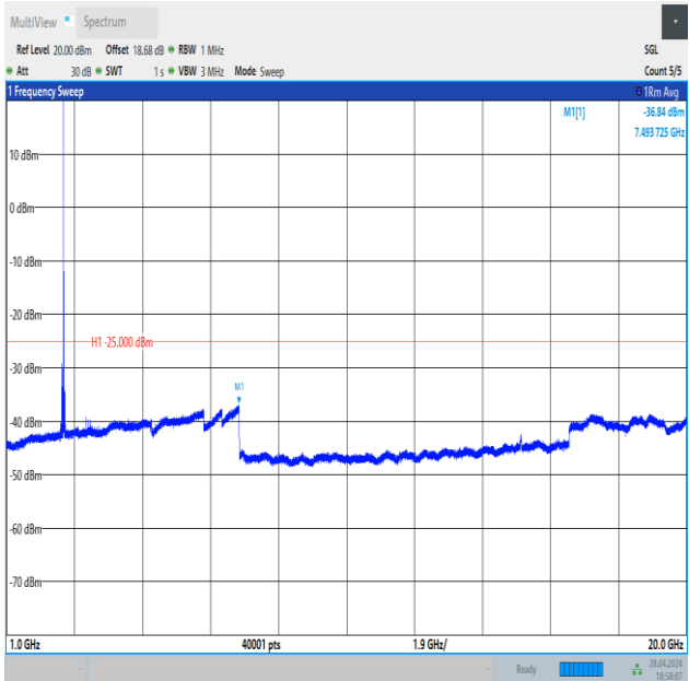
Band41_20MHz_QPSK_40620_1RB#0_1000~20000_1000~20000
