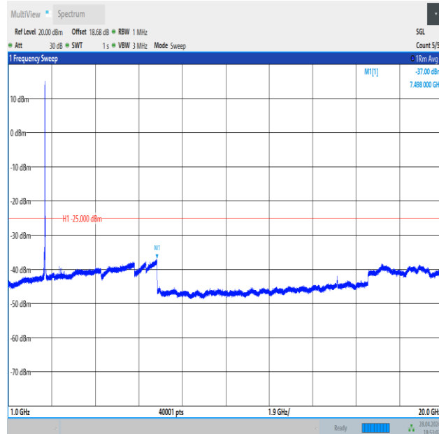
Band41_20MHz_QPSK_40620_100RB#0_1000~20000_1000~20000
