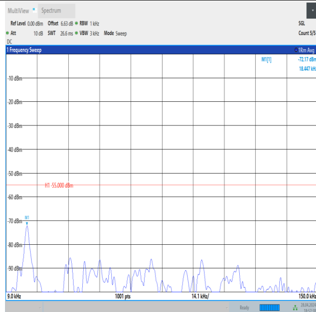
Band41_20MHz_QPSK_40620_1RB#0_0.009~0.15_0.009~0.15
