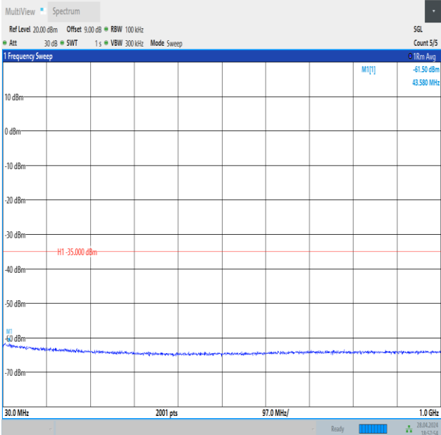
Band41_20MHz_QPSK_40620_1RB#0_30~1000_30~1000
