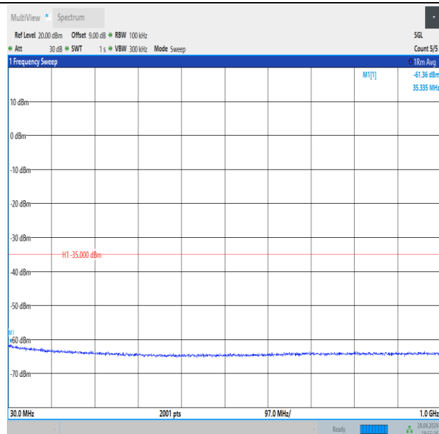
Band41_20MHz_16QAM_39750_1RB#0_30~1000_30~1000
