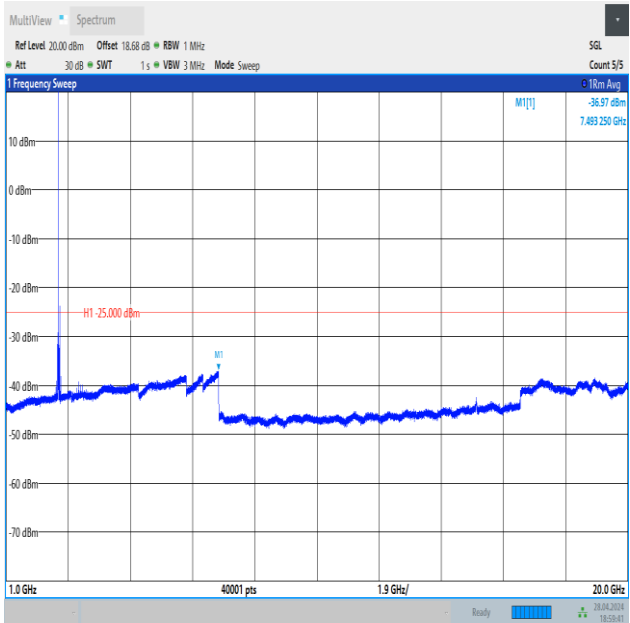
Band41_20MHz_QPSK_40620_1RB#99_1000~20000_1000~20000
