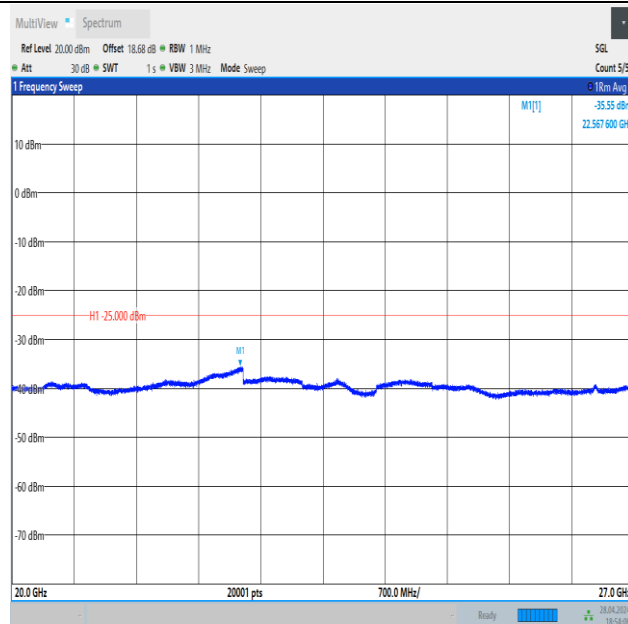
Band41_20MHz_QPSK_41490_100RB#0_20000~27000_20000~27000
