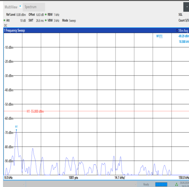
Band41_20MHz_16QAM_39750_1RB#0_0.009~0.15_0.009~0.15
