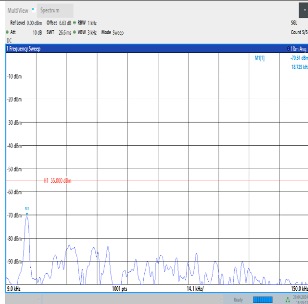
Band41_20MHz_QPSK_40620_1RB#99_0.009~0.15_0.009~0.15
