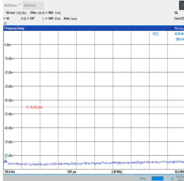
Band41_15MHz_QPSK_40620_75RB#0_0.15~30_0.15~30
