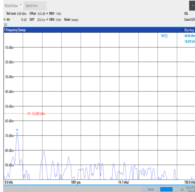
Band41_15MHz_QPSK_41515_75RB#0_0.009~0.15_0.009~0.15
