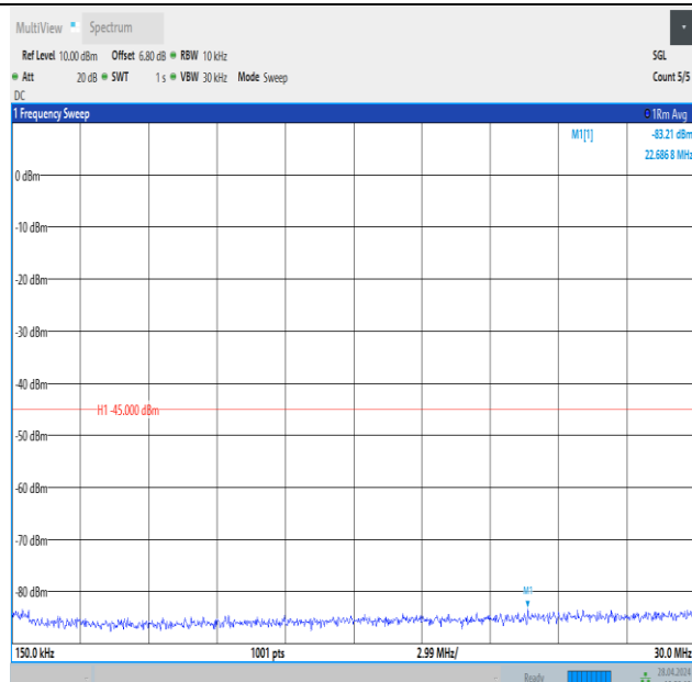
Band41_20MHz_QPSK_40620_1RB#99_0.15~30_0.15~30
