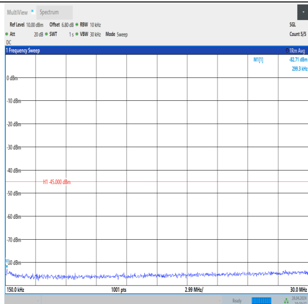
Band41_15MHz_16QAM_39725_1RB#74_0.15~30_0.15~30
