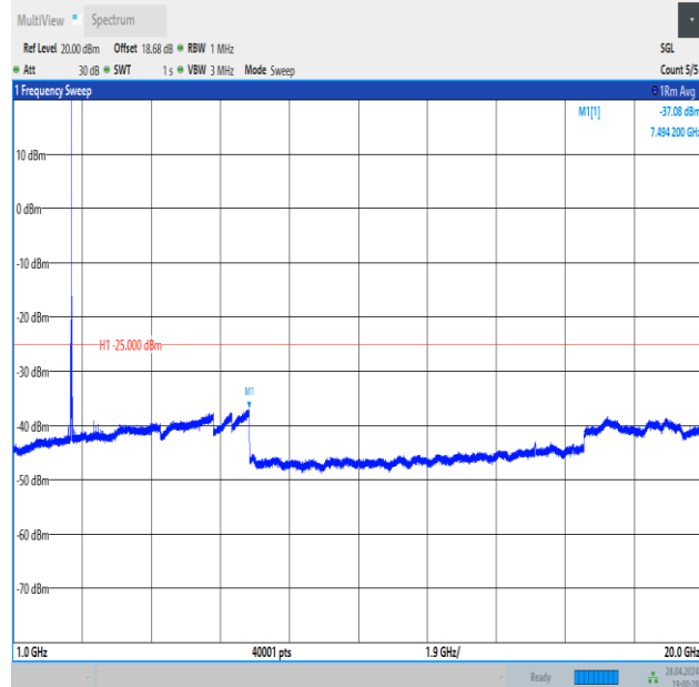
Band41_20MHz_16QAM_40620_1RB#99_1000~20000_1000~20000
