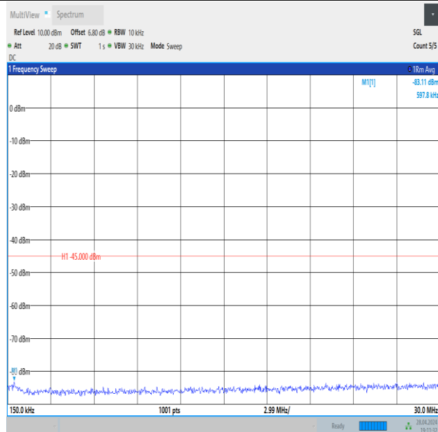
Band41_15MHz_QPSK_40620_1RB#0_0.15~30_0.15~30
