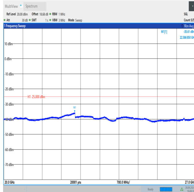
Band41_20MHz_16QAM_40620_1RB#99_20000~27000_20000~27000
