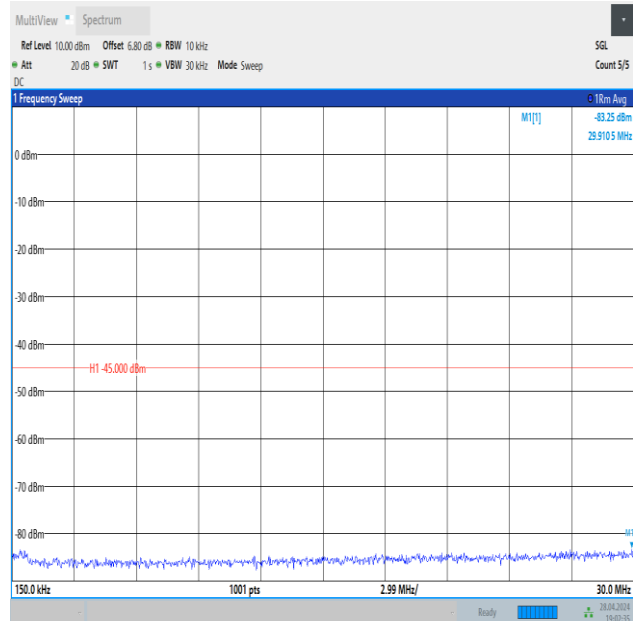
Band41_20MHz_QPSK_41490_1RB#99_0.15~30_0.15~30
