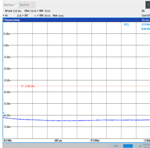
Band41_20MHz_QPSK_41490_100RB#0_30~1000_30~1000
