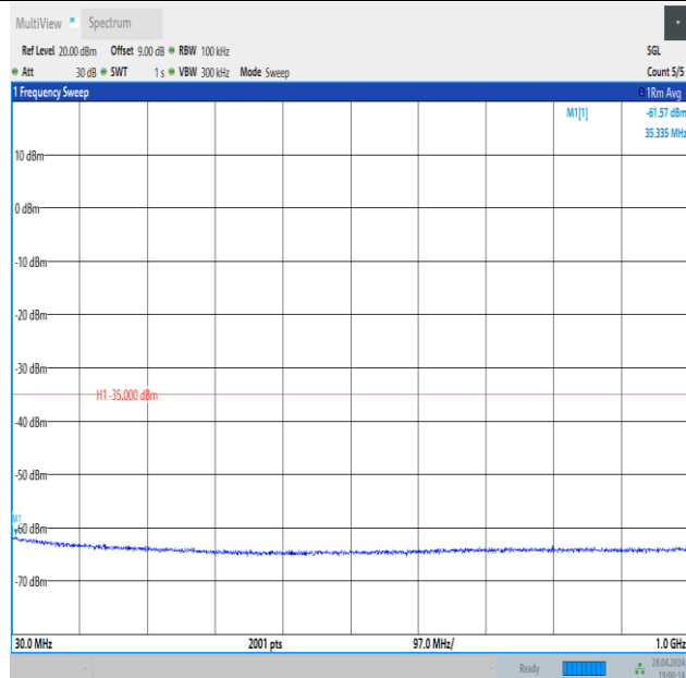
Band41_15MHz_QPSK_41515_75RB#0_30~1000_30~1000
