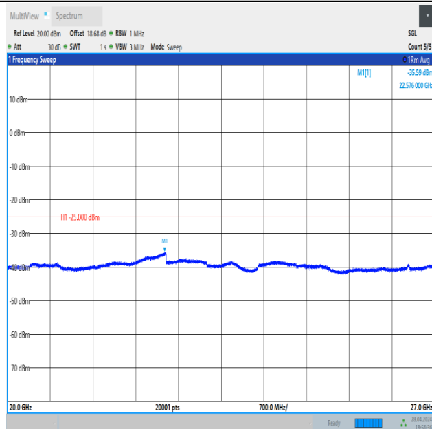
Band41_20MHz_QPSK_39750_1RB#99_20000~27000_20000~27000
