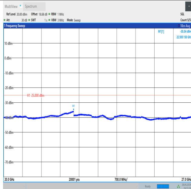
Band41_15MHz_16QAM_39725_1RB#74_20000~27000_20000~27000
