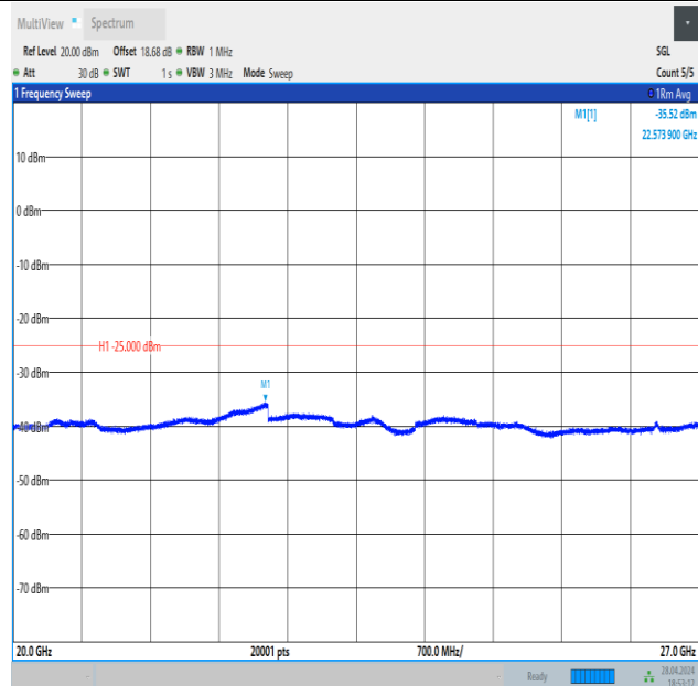
Band41_20MHz_QPSK_40620_100RB#0_20000~27000_20000~27000
