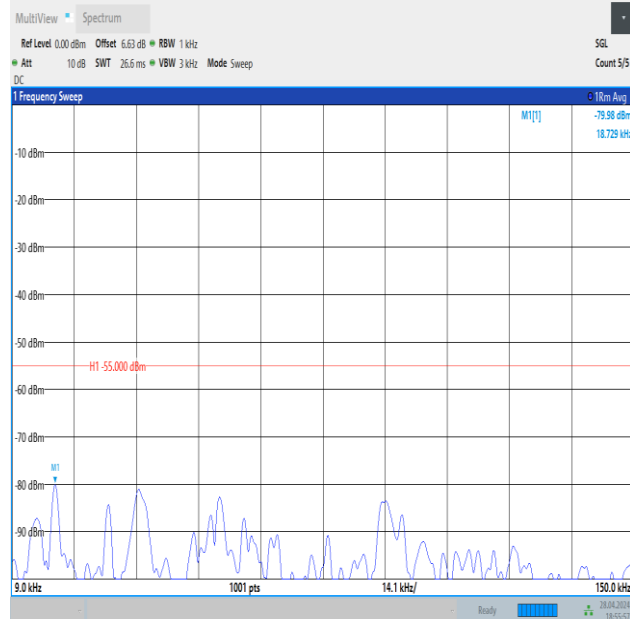
Band41_20MHz_QPSK_39750_1RB#99_0.009~0.15_0.009~0.15
