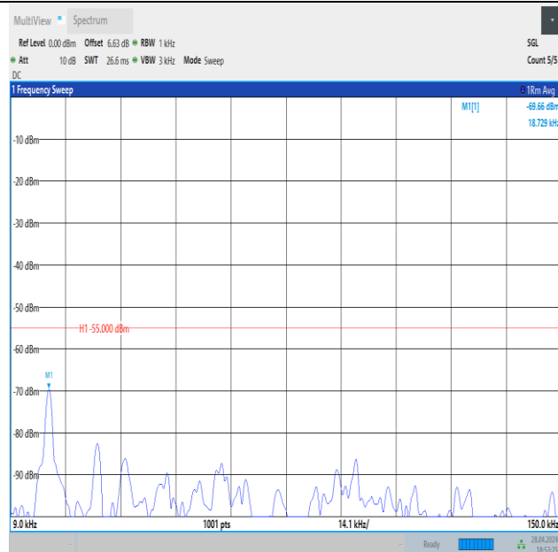
Band41_20MHz_QPSK_41490_100RB#0_0.009~0.15_0.009~0.15
