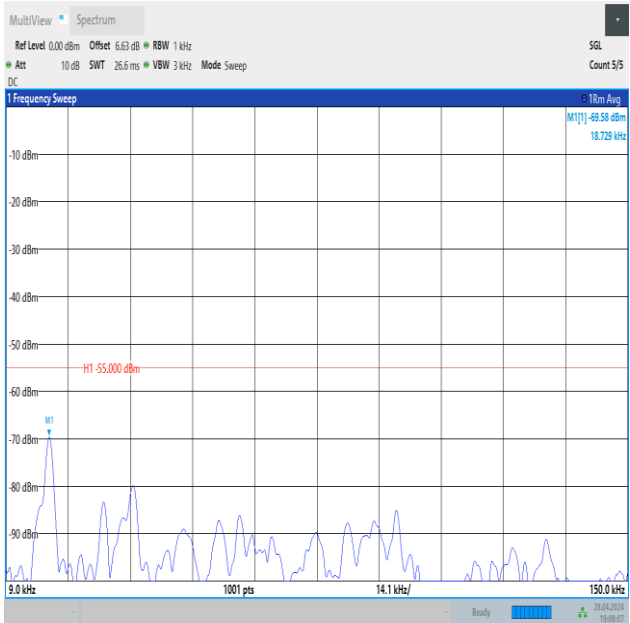
Band41_15MHz_QPSK_39725_1RB#0_0.009~0.15_0.009~0.15
