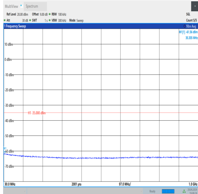
Band41_15MHz_QPSK_39725_1RB#0_30~1000_30~1000
