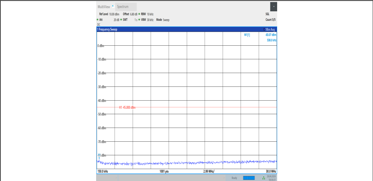
Band41_20MHz_QPSK_39750_1RB#0_0.15~30_0.15~30
