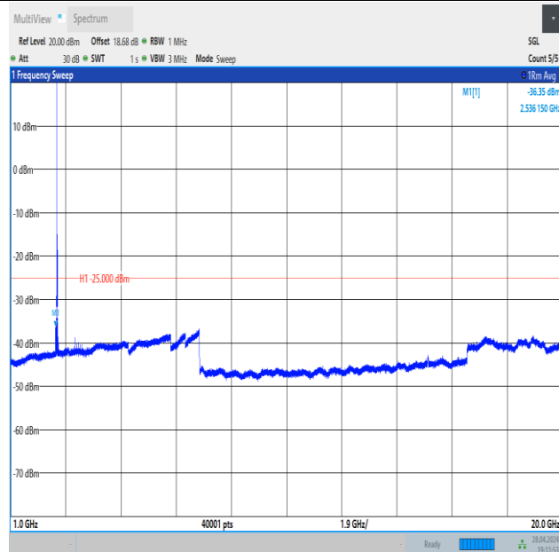
Band41_15MHz_QPSK_40620_1RB#0_1000~20000_1000~20000
