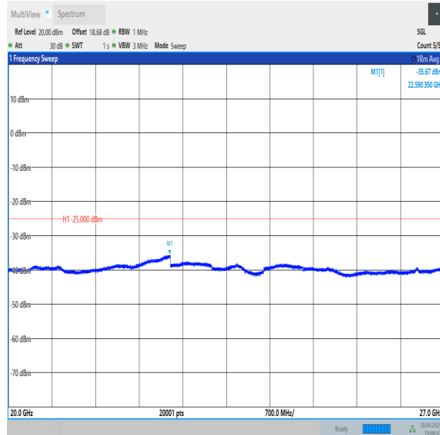
Band41_15MHz_QPSK_39725_1RB#0_20000~27000_20000~27000
