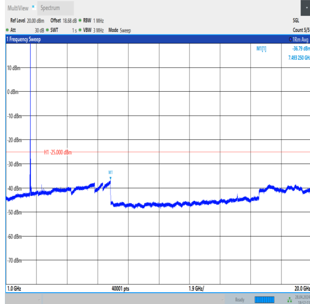
Band41_20MHz_16QAM_39750_1RB#99_1000~20000_1000~20000
