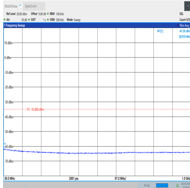
Band41_20MHz_16QAM_40620_1RB#0_30~1000_30~1000
