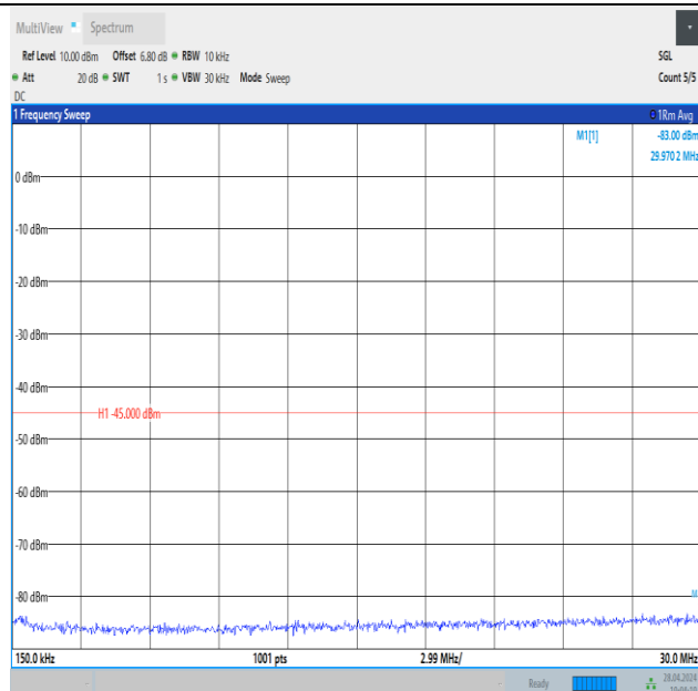
Band41_15MHz_QPSK_39725_75RB#0_0.15~30_0.15~30
