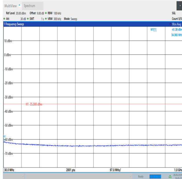
Band41_15MHz_QPSK_40620_75RB#0_30~1000_30~1000
