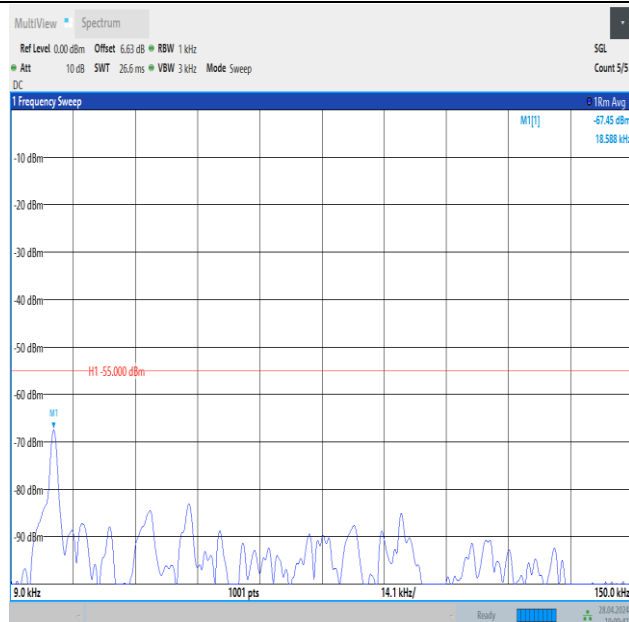
Band41_15MHz_QPSK_39725_1RB#74_0.009~0.15_0.009~0.15
