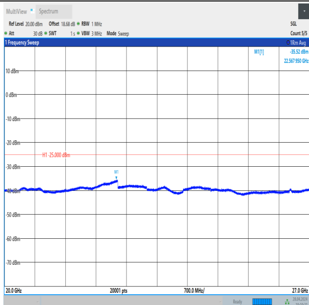
Band41_15MHz_QPSK_39725_1RB#74_20000~27000_20000~27000
