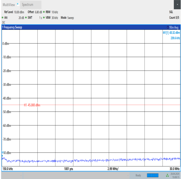
Band41_15MHz_QPSK_39725_1RB#0_0.15~30_0.15~30
