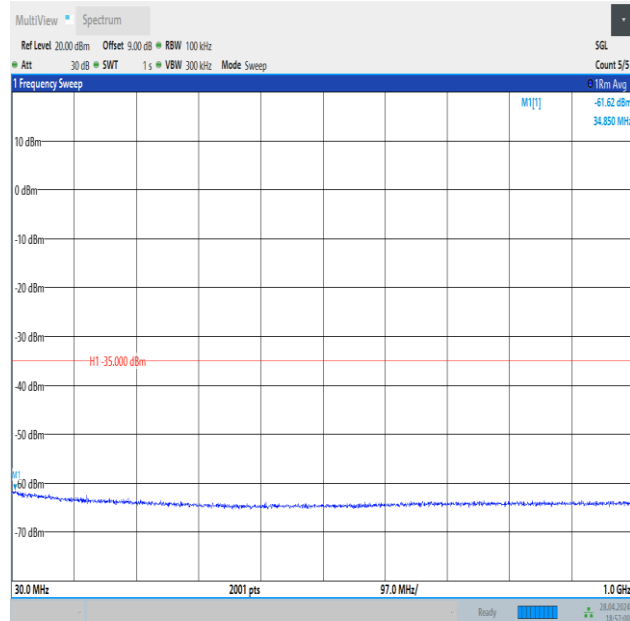
Band41_20MHz_16QAM_39750_1RB#99_30~1000_30~1000
