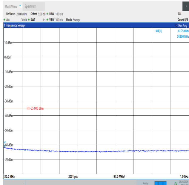
Band41_20MHz_QPSK_41490_1RB#99_30~1000_30~1000
