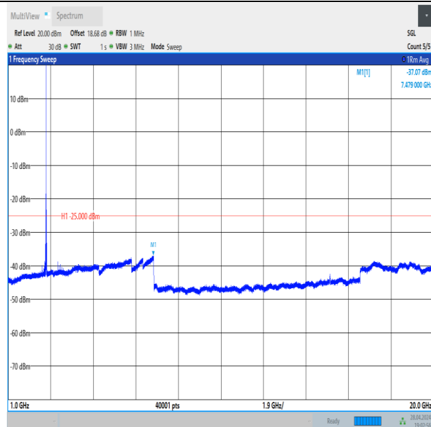
Band41_20MHz_QPSK_41490_1RB#99_1000~20000_1000~20000
