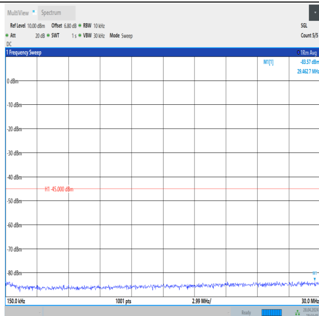
Band41_20MHz_QPSK_39750_1RB#99_0.15~30_0.15~30
