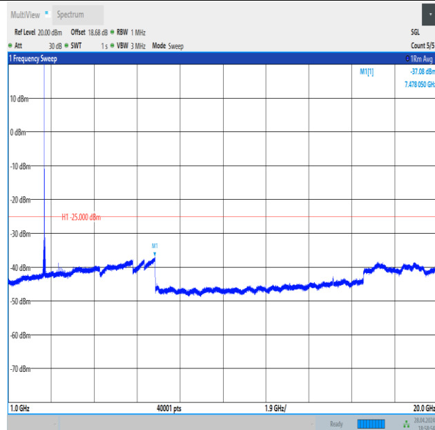
Band41_20MHz_16QAM_40620_1RB#0_1000~20000_1000~20000
