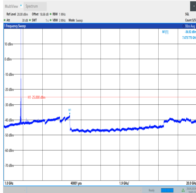
Band41_20MHz_QPSK_41490_1RB#0_1000~20000_1000~20000
