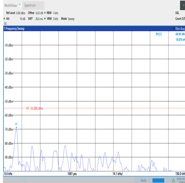
Band41_15MHz_16QAM_39725_1RB#0_0.009~0.15_0.009~0.15
