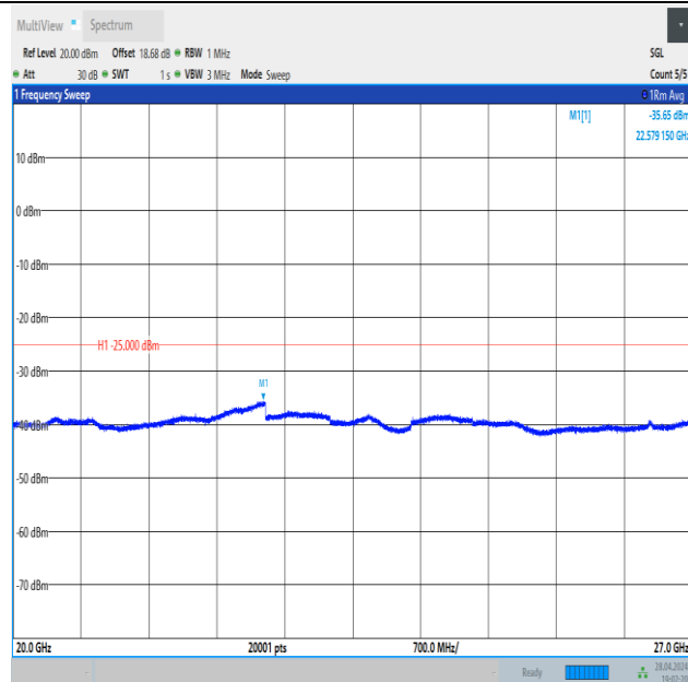
Band41_20MHz_16QAM_41490_1RB#0_20000~27000_20000~27000
