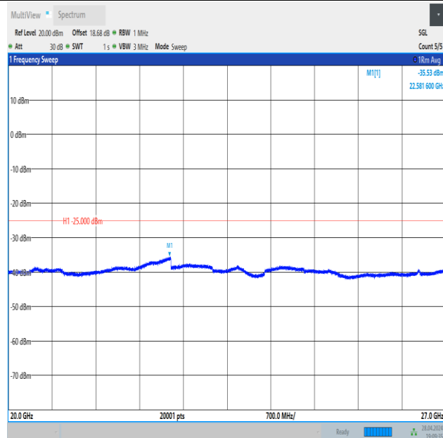
Band41_15MHz_16QAM_39725_1RB#0_20000~27000_20000~27000
