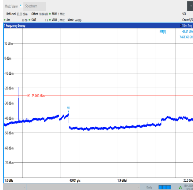
Band41_15MHz_16QAM_39725_1RB#74_1000~20000_1000~20000
