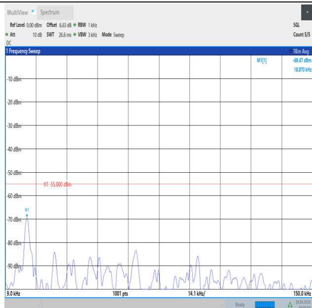
Band41_20MHz_16QAM_40620_1RB#99_0.009~0.15_0.009~0.15
