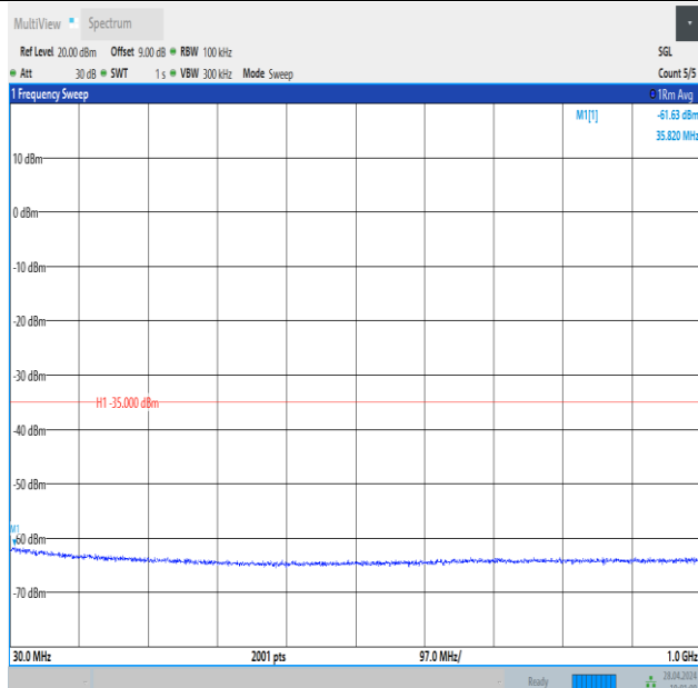
Band41_20MHz_QPSK_41490_1RB#0_30~1000_30~1000
