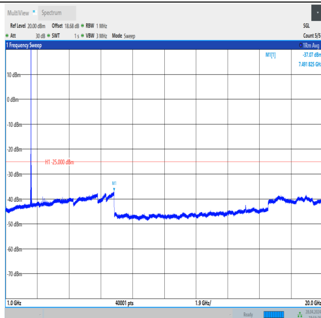
Band41_20MHz_QPSK_39750_1RB#99_1000~20000_1000~20000
