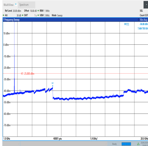
Band41_15MHz_16QAM_39725_1RB#0_1000~20000_1000~20000
