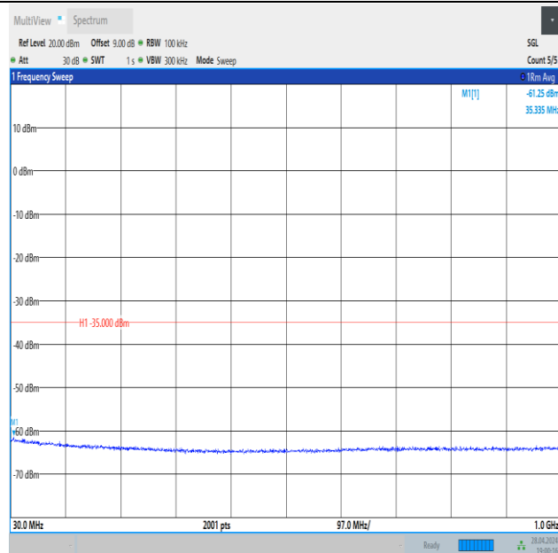
Band41_20MHz_16QAM_40620_1RB#99_30~1000_30~1000
