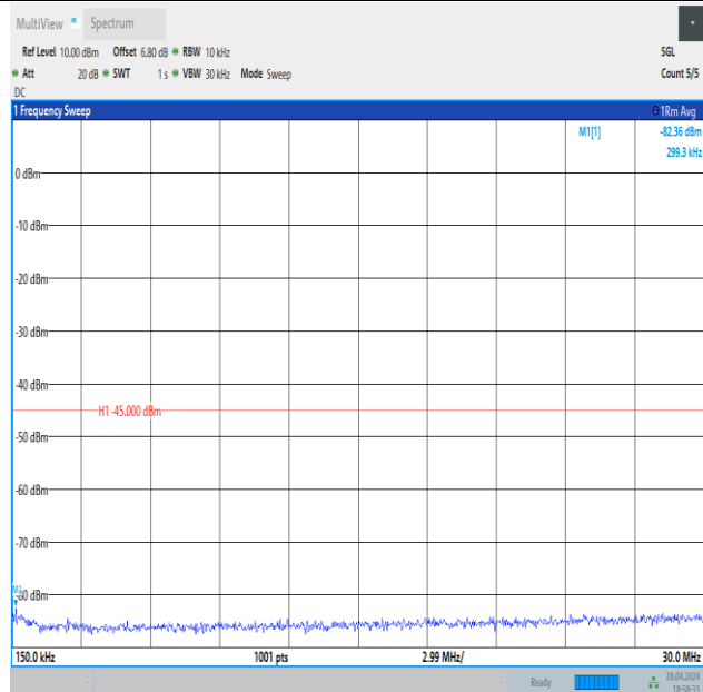
Band41_20MHz_16QAM_40620_1RB#0_0.15~30_0.15~30
