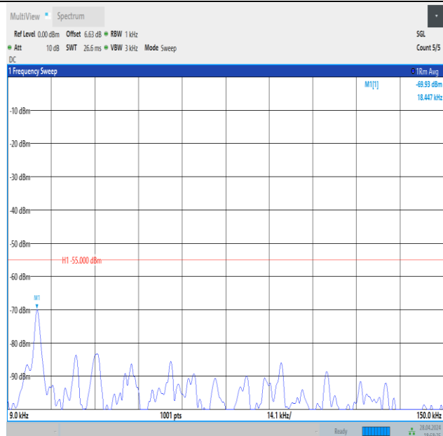
Band41_20MHz_16QAM_40620_1RB#0_0.009~0.15_0.009~0.15
