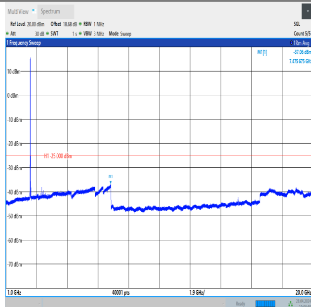
Band41_15MHz_QPSK_39725_75RB#0_1000~20000_1000~20000
