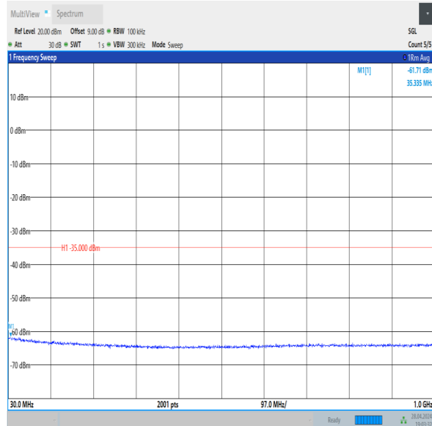
Band41_20MHz_16QAM_41490_1RB#99_30~1000_30~1000
