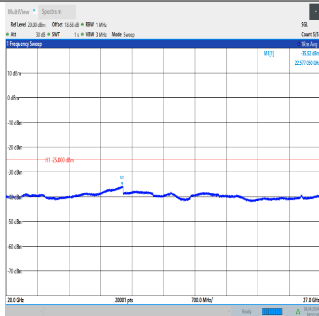
Band41_20MHz_16QAM_39750_1RB#0_20000~27000_20000~27000
