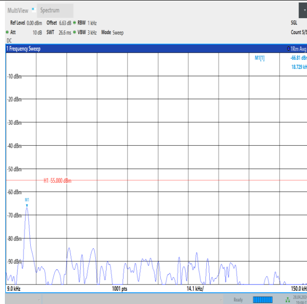
Band41_15MHz_QPSK_39725_75RB#0_0.009~0.15_0.009~0.15
