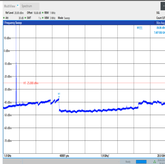
Band41_20MHz_QPSK_39750_1RB#0_1000~20000_1000~20000
