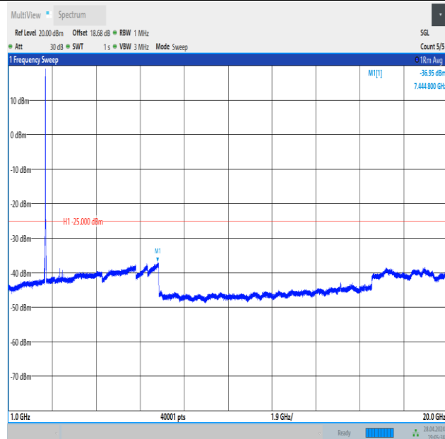
Band41_15MHz_QPSK_40620_75RB#0_1000~20000_1000~20000
