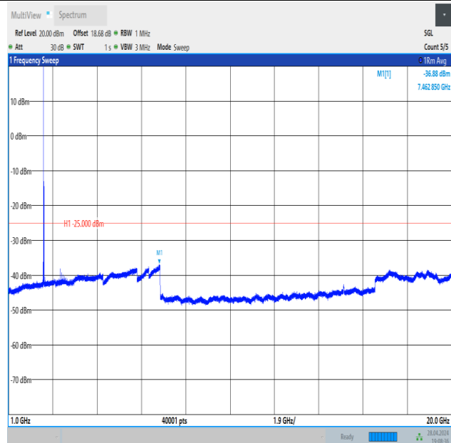
Band41_15MHz_QPSK_39725_1RB#0_1000~20000_1000~20000
