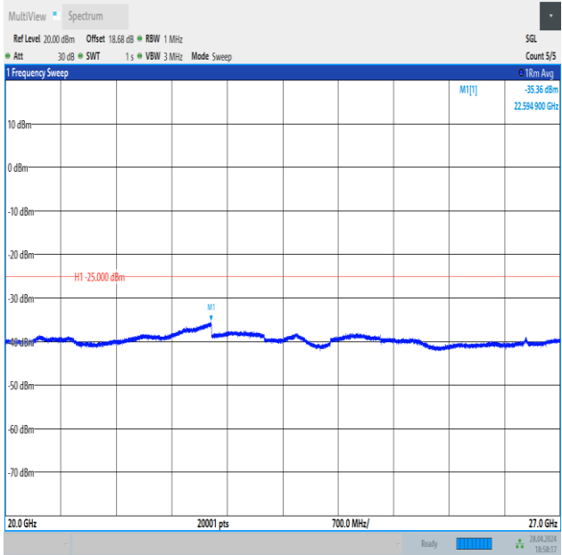
Band41_20MHz_QPSK_40620_1RB#0_20000~27000_20000~27000
