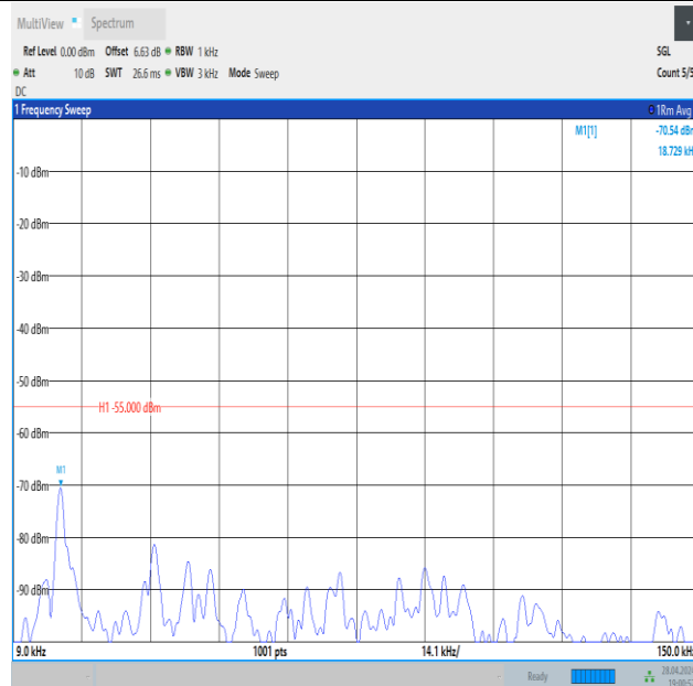
Band41_20MHz_QPSK_41490_1RB#0_0.009~0.15_0.009~0.15
