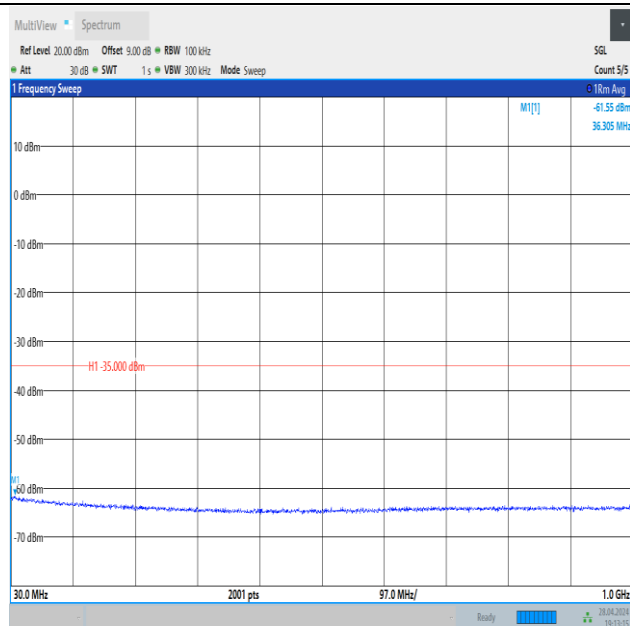
Band41_15MHz_QPSK_40620_1RB#74_30~1000_30~1000
