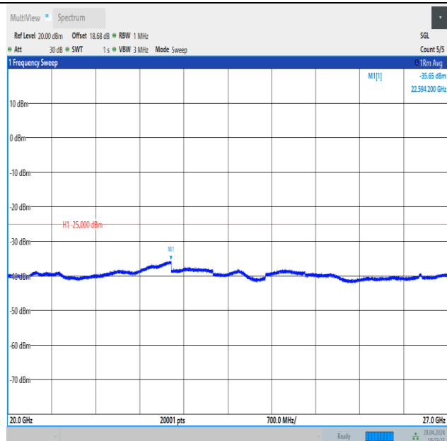
Band41_10MHz_QPSK_41540_50RB#0_20000~27000_20000~27000
