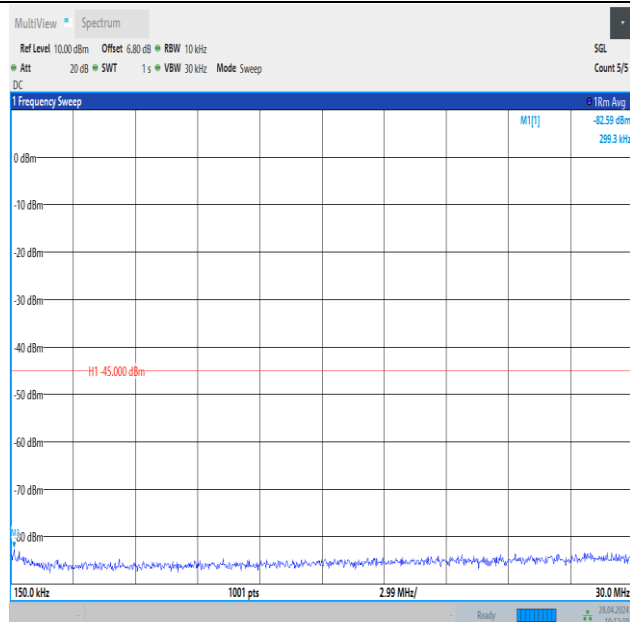
Band41_15MHz_16QAM_40620_1RB#0_0.15~30_0.15~30
