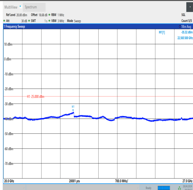
Band41_10MHz_16QAM_40620_1RB#0_20000~27000_20000~27000
