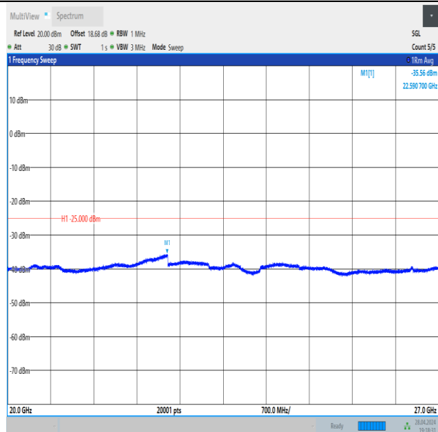
Band41_15MHz_16QAM_41515_1RB#0_20000~27000_20000~27000
