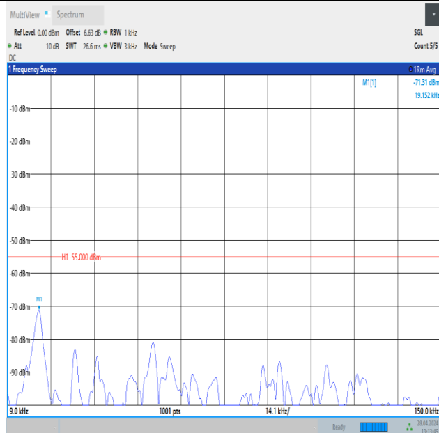
Band41_15MHz_16QAM_40620_1RB#74_0.009~0.15_0.009~0.15
