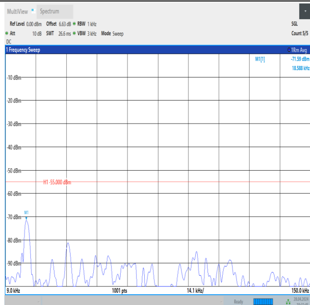
Band41_10MHz_16QAM_40620_1RB#49_0.009~0.15_0.009~0.15
