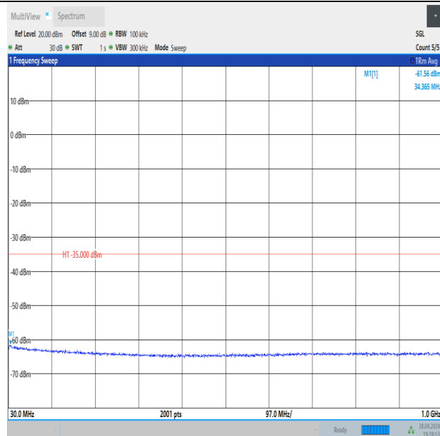
Band41_15MHz_QPSK_41515_1RB#74_30~1000_30~1000
