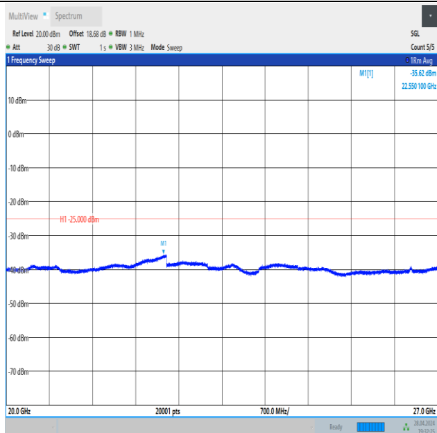
Band41_10MHz_16QAM_40620_1RB#49_20000~27000_20000~27000
