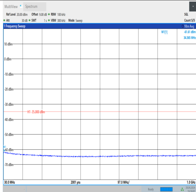
Band41_15MHz_16QAM_40620_1RB#74_30~1000_30~1000
