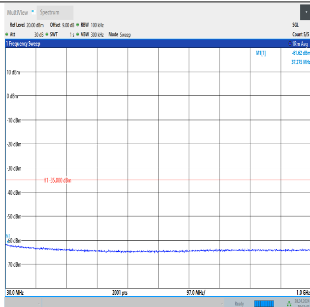
Band41_10MHz_16QAM_41540_1RB#0_30~1000_30~1000
