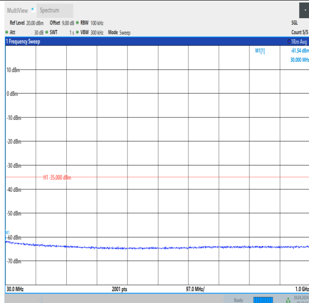
Band41_10MHz_QPSK_41540_1RB#0_30~1000_30~1000
