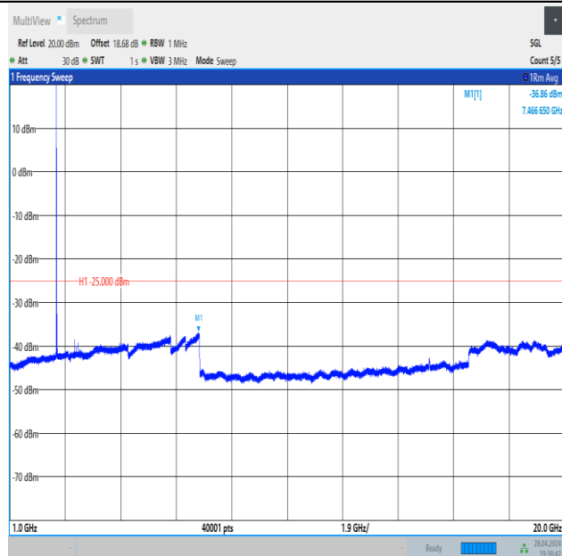
Band41_10MHz_16QAM_40620_1RB#0_1000~20000_1000~20000
