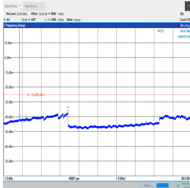
Band41_10MHz_QPSK_40620_50RB#0_1000~20000_1000~20000
