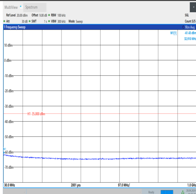
Band41_10MHz_QPSK_39700_1RB#0_30~1000_30~1000
