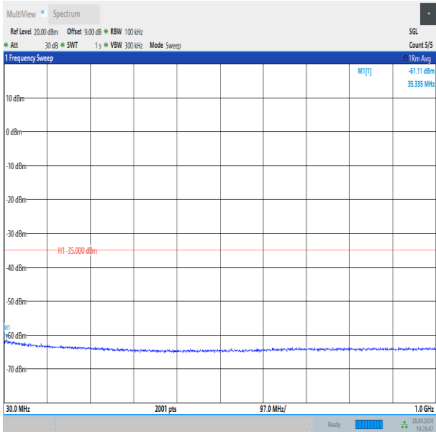
Band41_10MHz_16QAM_39700_1RB#49_30~1000_30~1000
