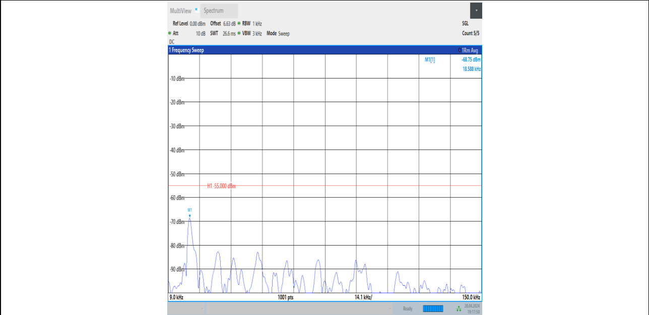
Band41_15MHz_16QAM_41515_1RB#0_0.009~0.15_0.009~0.15
