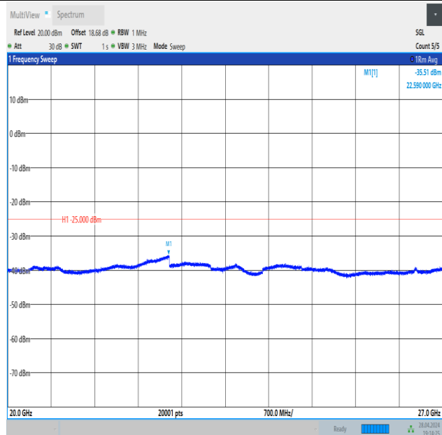
Band41_15MHz_16QAM_40620_1RB#74_20000~27000_20000~27000
