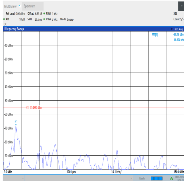
Band41_10MHz_QPSK_41540_1RB#49_0.009~0.15_0.009~0.15
