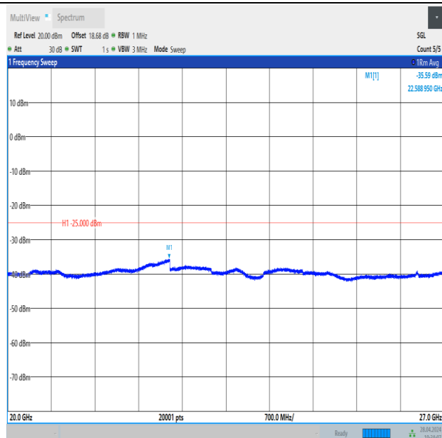
Band41_10MHz_16QAM_41540_1RB#0_20000~27000_20000~27000
