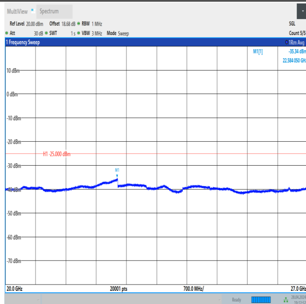
Band41_15MHz_16QAM_40620_1RB#0_20000~27000_20000~27000
