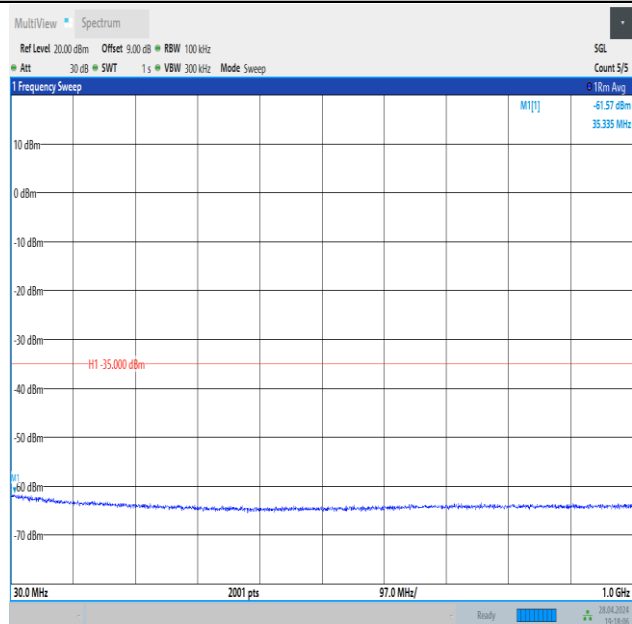
Band41_15MHz_16QAM_41515_1RB#0_30~1000_30~1000
