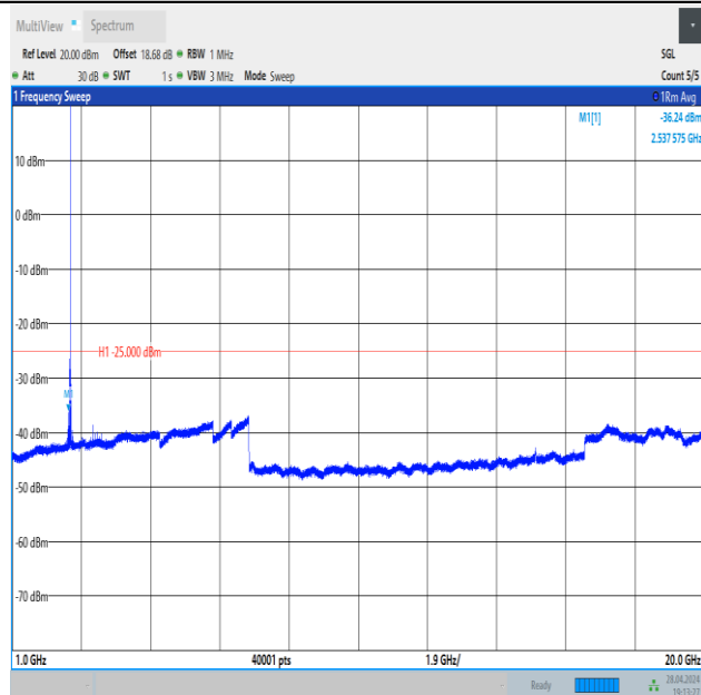
Band41_15MHz_QPSK_40620_1RB#74_1000~20000_1000~20000
