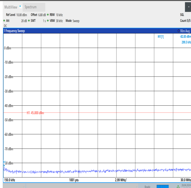
Band41_10MHz_QPSK_41540_1RB#0_0.15~30_0.15~30
