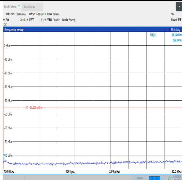
Band41_10MHz_QPSK_41540_1RB#49_0.15~30_0.15~30
