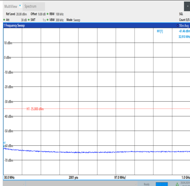
Band41_15MHz_16QAM_40620_1RB#0_30~1000_30~1000
