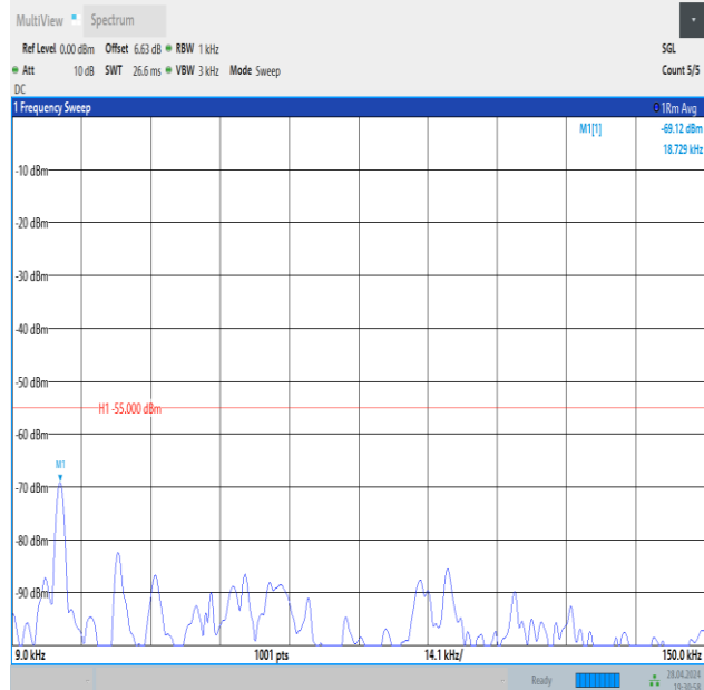
Band41_10MHz_QPSK_40620_1RB#49_0.009~0.15_0.009~0.15
