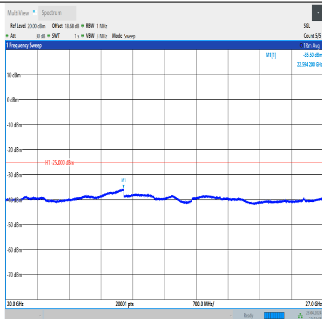
Band41_15MHz_QPSK_40620_1RB#74_20000~27000_20000~27000
