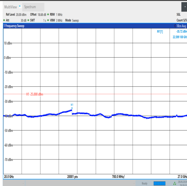
Band41_10MHz_QPSK_39700_1RB#0_20000~27000_20000~27000
