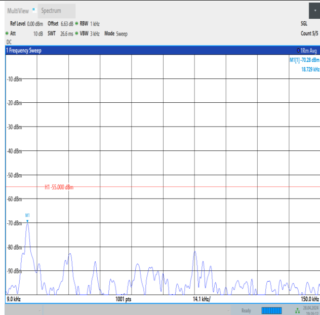
Band41_10MHz_QPSK_39700_1RB#0_0.009~0.15_0.009~0.15
