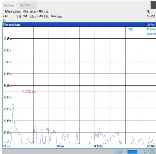
Band41_10MHz_QPSK_40620_50RB#0_0.009~0.15_0.009~0.15
