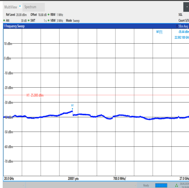
Band41_10MHz_QPSK_40620_1RB#0_20000~27000_20000~27000
