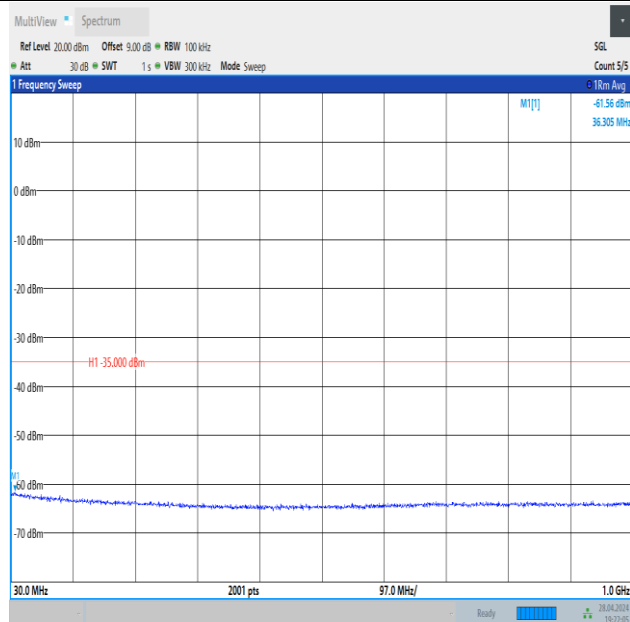
Band41_10MHz_QPSK_40620_50RB#0_30~1000_30~1000
