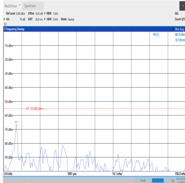
Band41_10MHz_16QAM_39700_1RB#49_0.009~0.15_0.009~0.15
