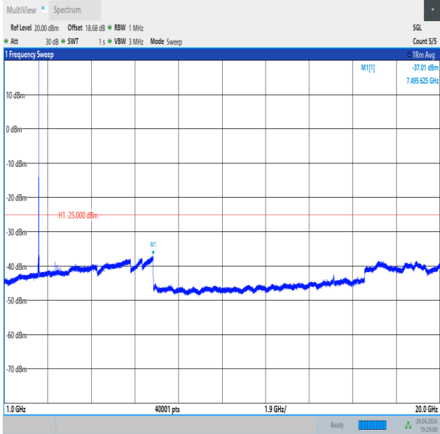
Band41_10MHz_16QAM_39700_1RB#49_1000~20000_1000~20000
