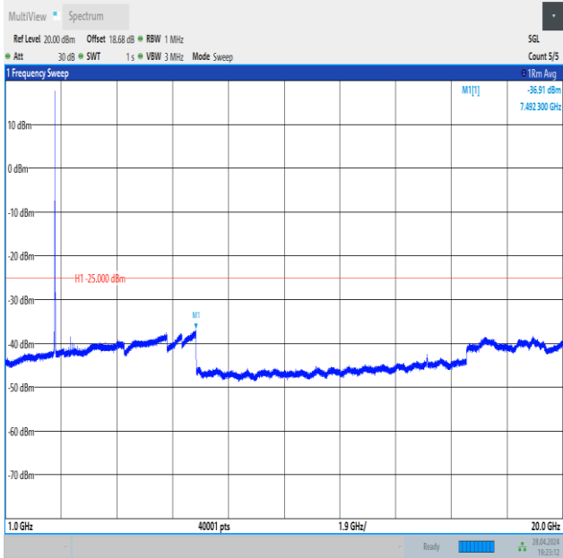
Band41_10MHz_QPSK_41540_50RB#0_1000~20000_1000~20000
