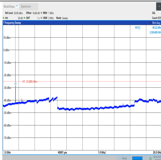
Band41_10MHz_QPSK_39700_1RB#0_1000~20000_1000~20000
