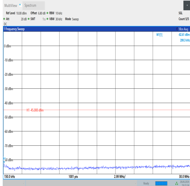
Band41_10MHz_16QAM_40620_1RB#49_0.15~30_0.15~30
