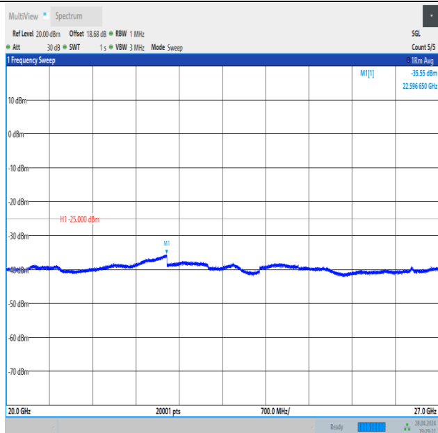
Band41_10MHz_16QAM_39700_1RB#49_20000~27000_20000~27000
