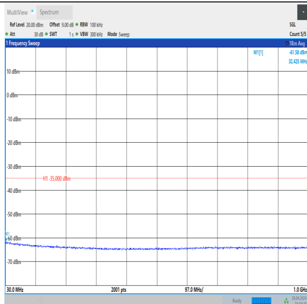
Band41_10MHz_16QAM_40620_1RB#0_30~1000_30~1000
