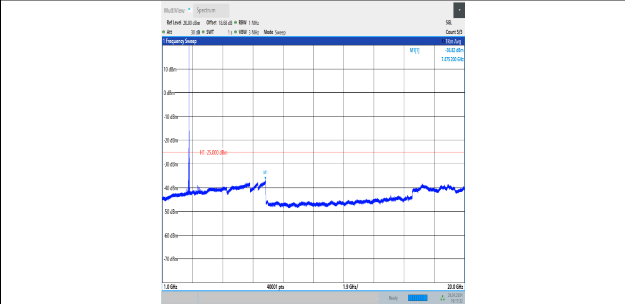
Band41_15MHz_QPSK_41515_1RB#0_1000~20000_1000~20000
