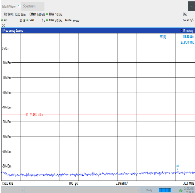
Band41_10MHz_QPSK_40620_1RB#0_0.15~30_0.15~30
