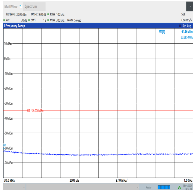
Band41_10MHz_QPSK_41540_1RB#49_30~1000_30~1000
