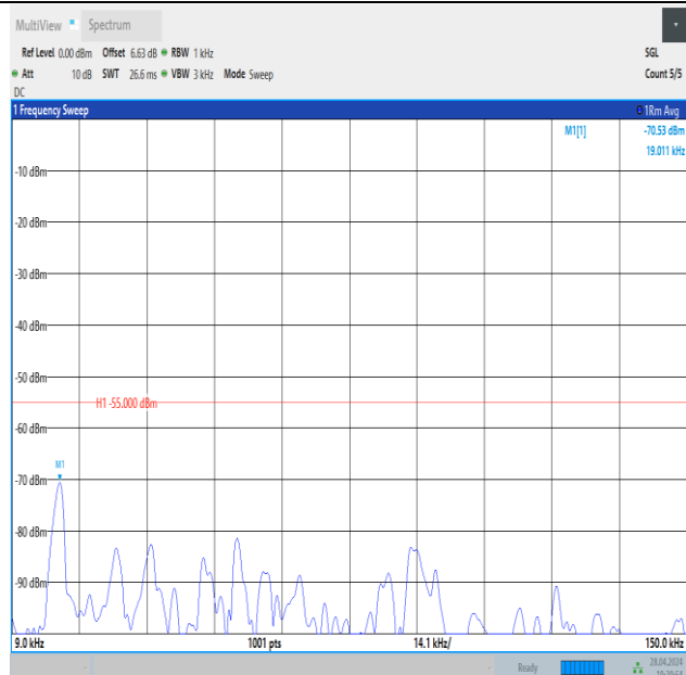
Band41_10MHz_QPSK_39700_50RB#0_0.009~0.15_0.009~0.15
