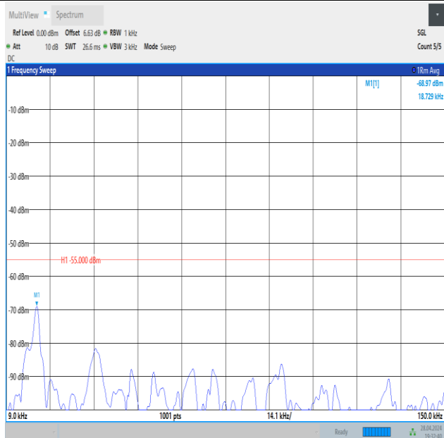
Band41_10MHz_QPSK_41540_1RB#0_0.009~0.15_0.009~0.15
