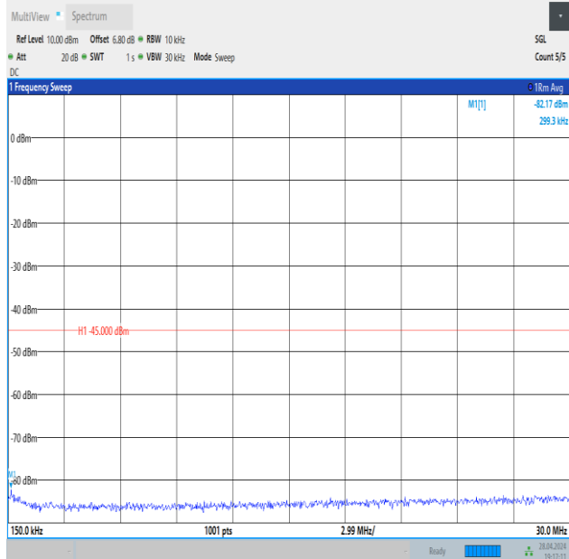
Band41_15MHz_QPSK_41515_1RB#0_0.15~30_0.15~30
