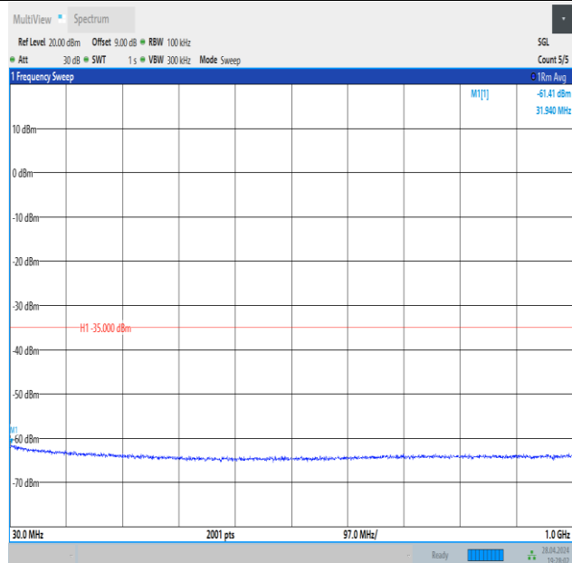
Band41_10MHz_QPSK_39700_1RB#49_30~1000_30~1000
