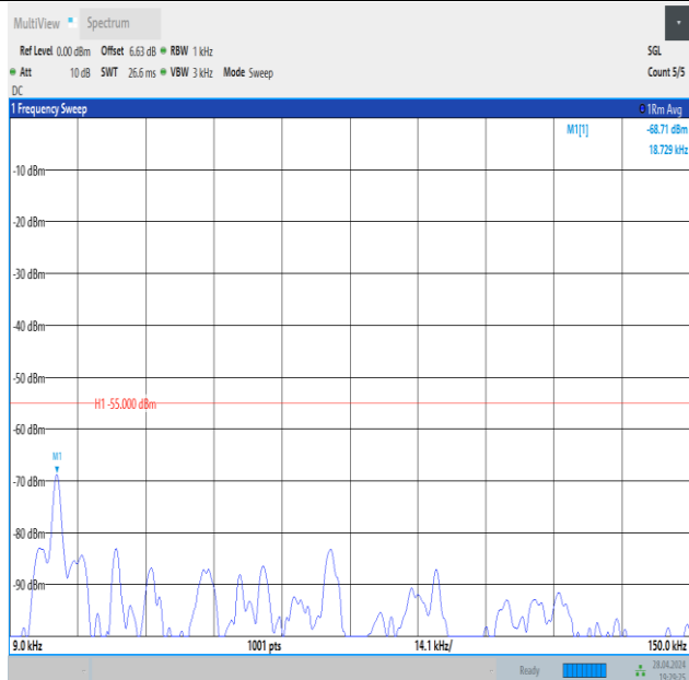
Band41_10MHz_QPSK_40620_1RB#0_0.009~0.15_0.009~0.15
