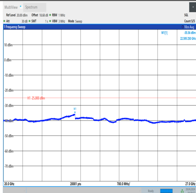
Band41_15MHz_QPSK_41515_1RB#74_20000~27000_20000~27000
