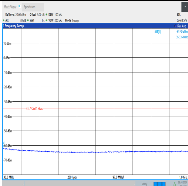
Band41_10MHz_16QAM_40620_1RB#49_30~1000_30~1000
