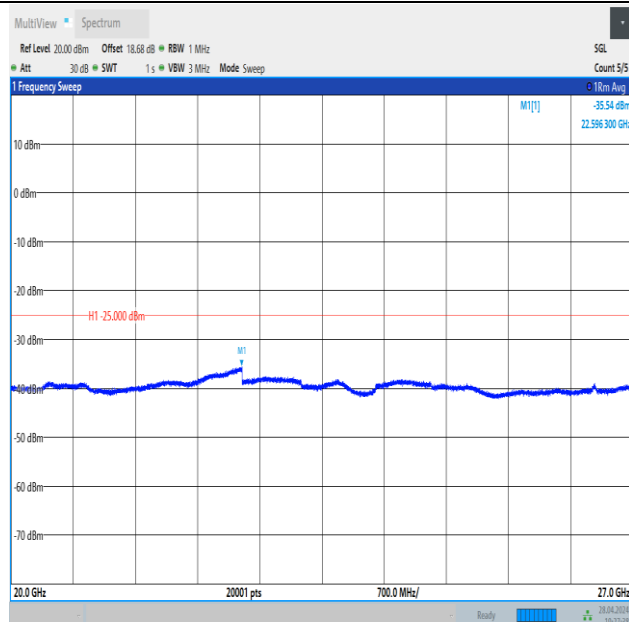
Band41_10MHz_16QAM_39700_1RB#0_20000~27000_20000~27000
