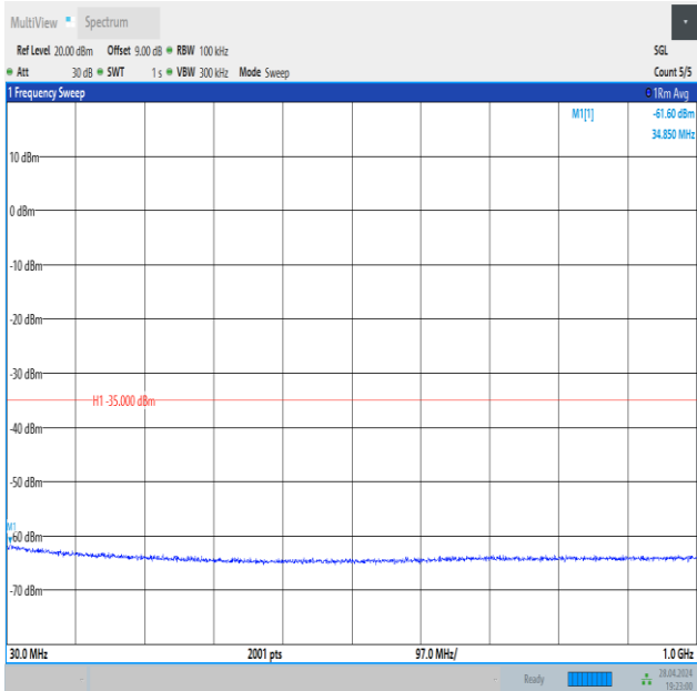
Band41_10MHz_QPSK_41540_50RB#0_30~1000_30~1000
