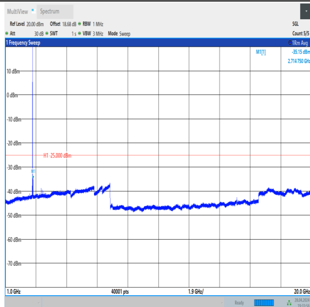
Band41_10MHz_16QAM_41540_1RB#0_1000~20000_1000~20000
