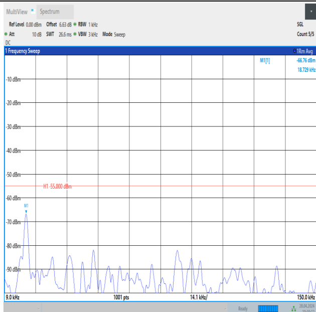
Band41_10MHz_16QAM_40620_1RB#0_0.009~0.15_0.009~0.15
