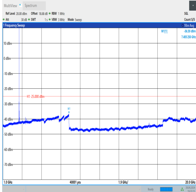
Band41_10MHz_16QAM_40620_1RB#49_1000~20000_1000~20000
