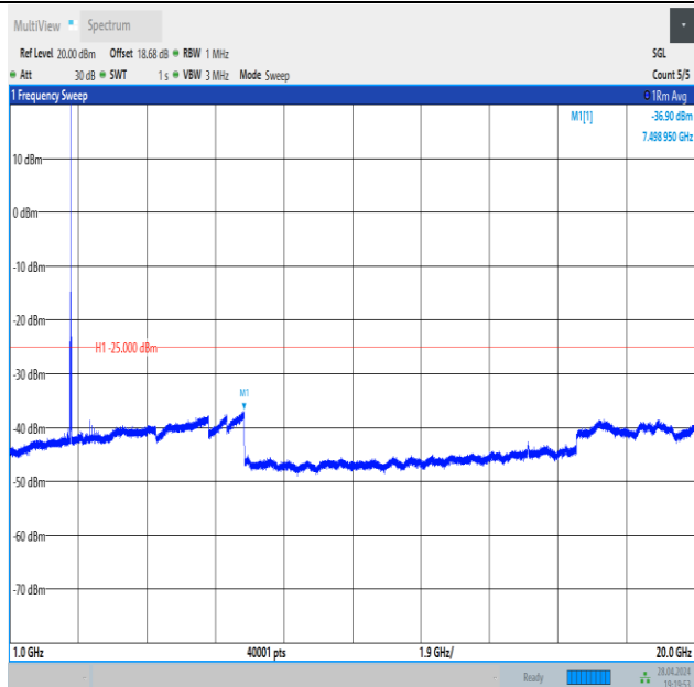
Band41_15MHz_16QAM_41515_1RB#74_1000~20000_1000~20000
