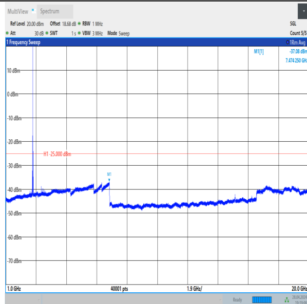
Band41_15MHz_QPSK_41515_1RB#74_1000~20000_1000~20000
