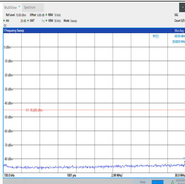
Band41_10MHz_QPSK_40620_50RB#0_0.15~30_0.15~30
