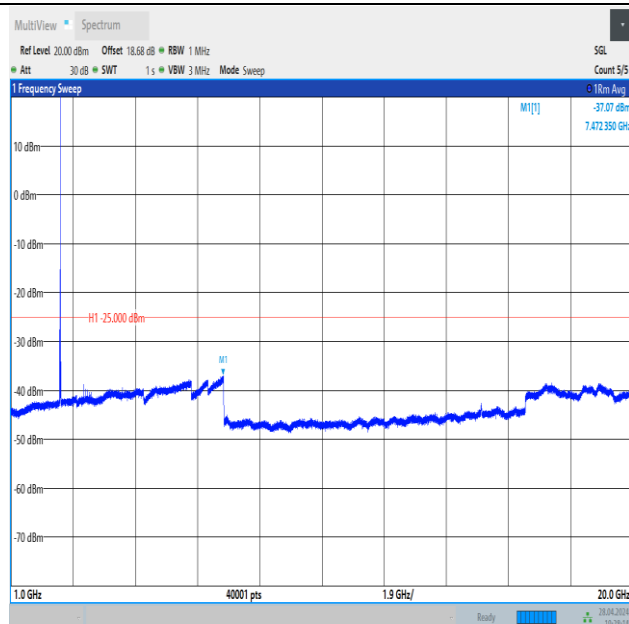
Band41_10MHz_QPSK_39700_1RB#49_1000~20000_1000~20000
