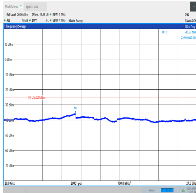
Band41_10MHz_QPSK_40620_1RB#49_20000~27000_20000~27000
