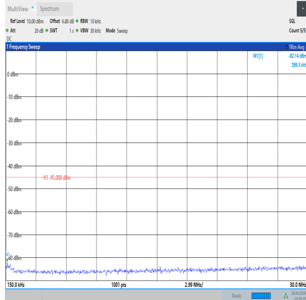
Band41_10MHz_16QAM_39700_1RB#49_0.15~30_0.15~30
