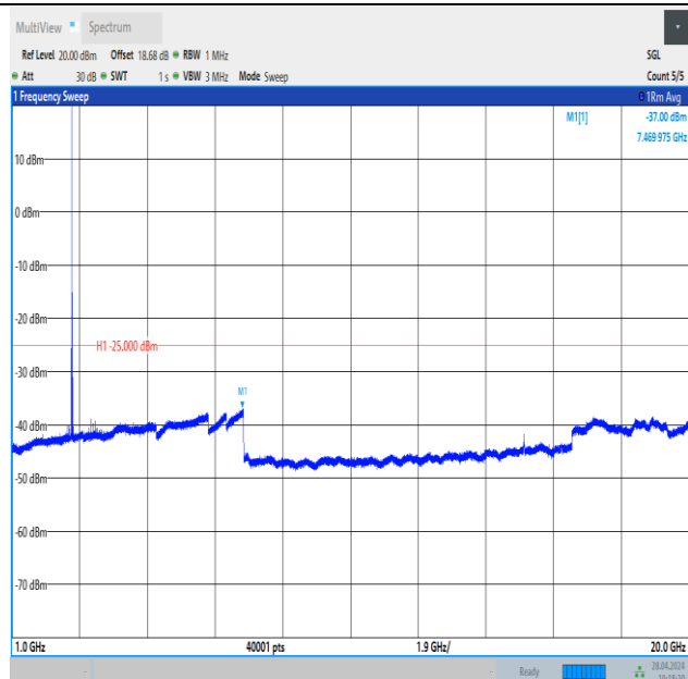
Band41_15MHz_16QAM_41515_1RB#0_1000~20000_1000~20000
