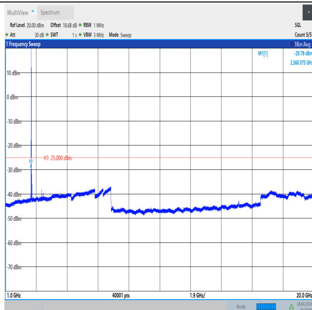
Band41_10MHz_QPSK_40620_1RB#0_1000~20000_1000~20000
