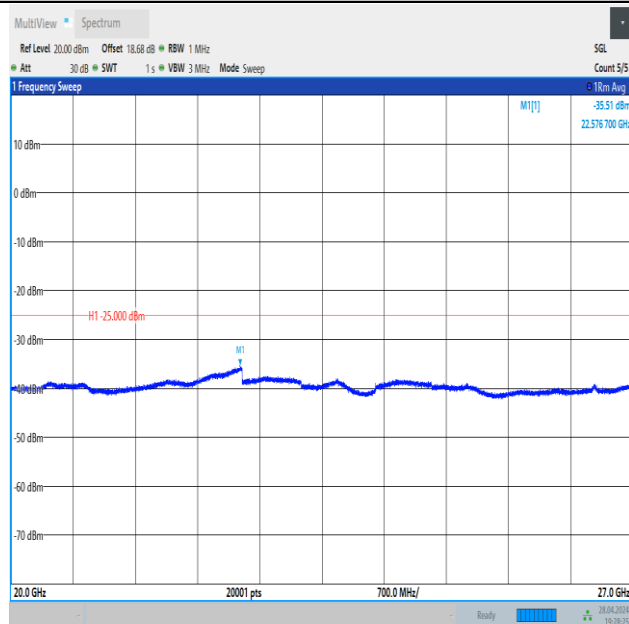
Band41_10MHz_QPSK_39700_1RB#49_20000~27000_20000~27000
