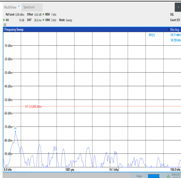
Band41_10MHz_16QAM_41540_1RB#0_0.009~0.15_0.009~0.15
