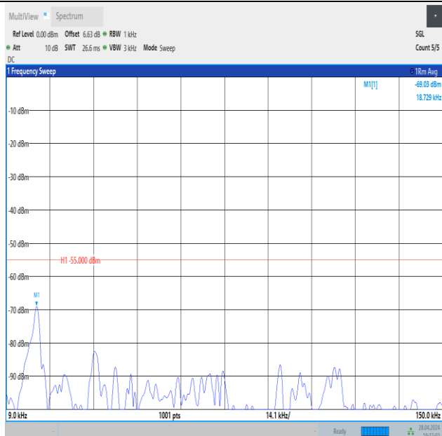
Band41_15MHz_QPSK_41515_1RB#0_0.009~0.15_0.009~0.15
