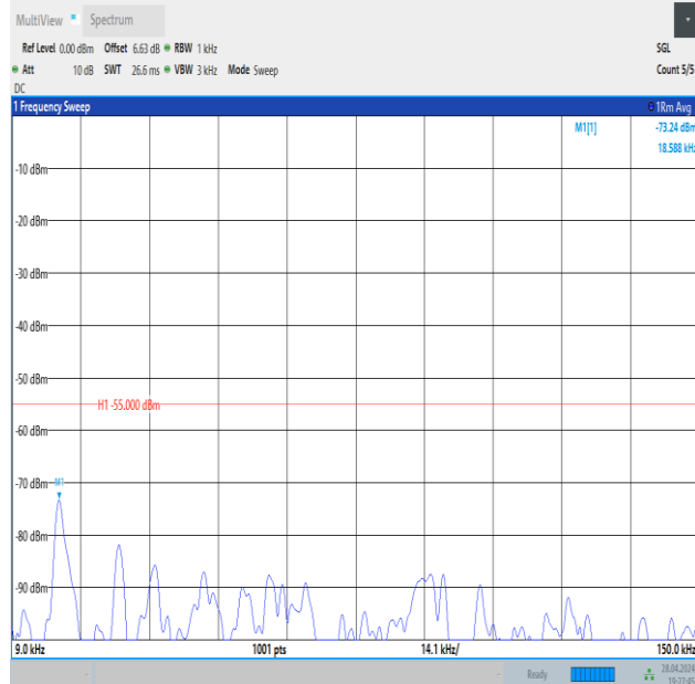
Band41_10MHz_QPSK_39700_1RB#49_0.009~0.15_0.009~0.15
