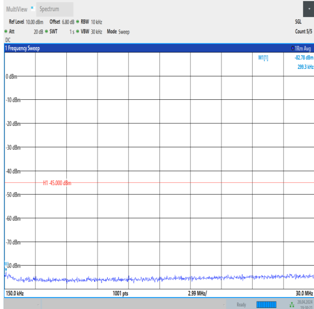
Band41_10MHz_16QAM_40620_1RB#0_0.15~30_0.15~30
