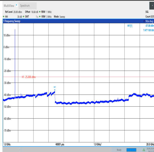
Band41_10MHz_QPSK_39700_50RB#0_1000~20000_1000~20000
