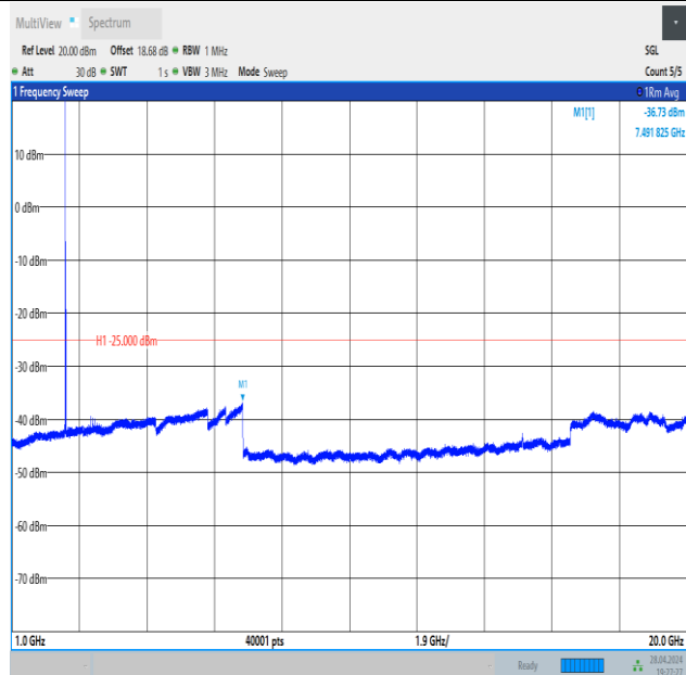
Band41_10MHz_16QAM_39700_1RB#0_1000~20000_1000~20000
