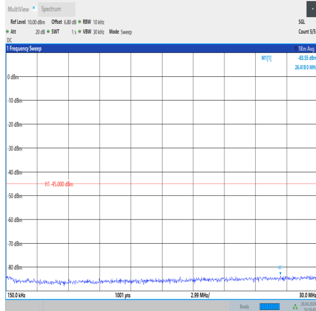
Band41_15MHz_QPSK_41515_1RB#74_0.15~30_0.15~30
