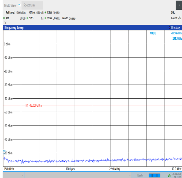
Band41_10MHz_QPSK_39700_50RB#0_0.15~30_0.15~30
