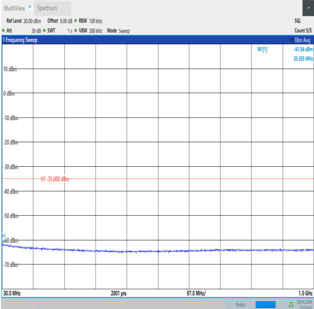
Band41_10MHz_QPSK_40620_1RB#0_30~1000_30~1000
