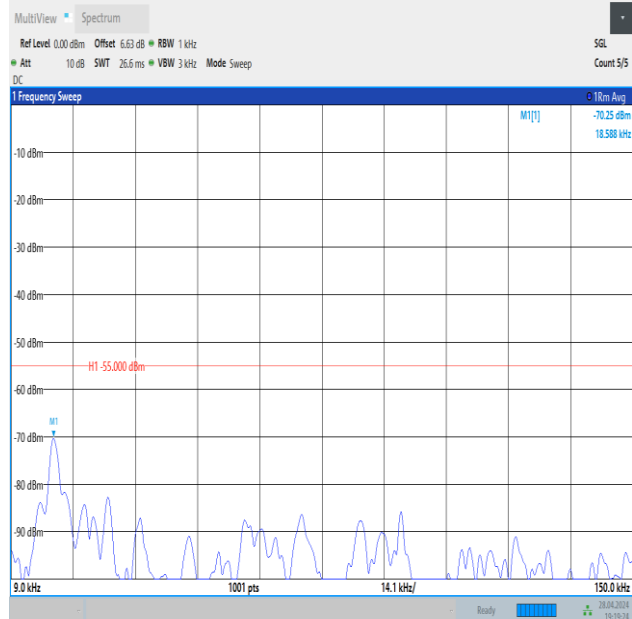
Band41_15MHz_16QAM_41515_1RB#74_0.009~0.15_0.009~0.15
