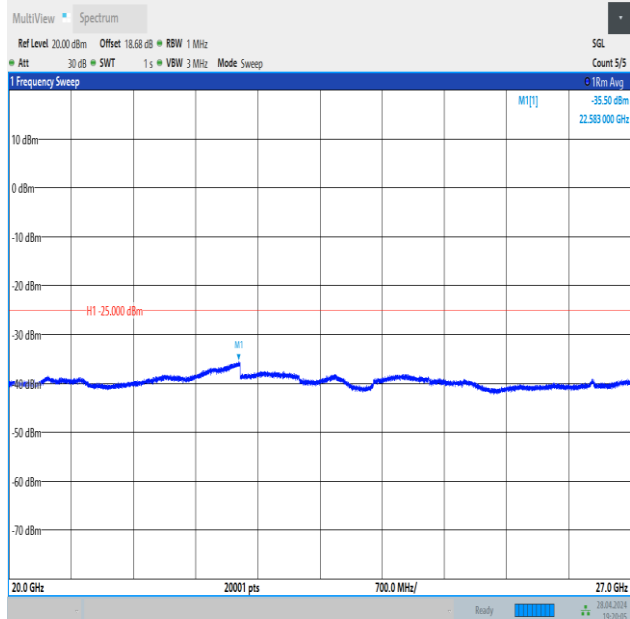
Band41_15MHz_16QAM_41515_1RB#74_20000~27000_20000~27000
