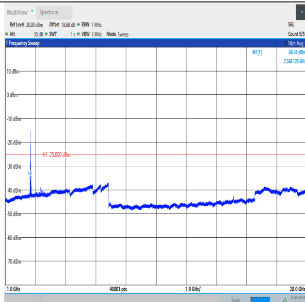
Band41_15MHz_16QAM_40620_1RB#0_1000~20000_1000~20000
