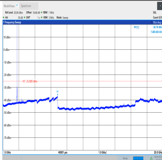
Band41_10MHz_QPSK_41540_1RB#49_1000~20000_1000~20000
