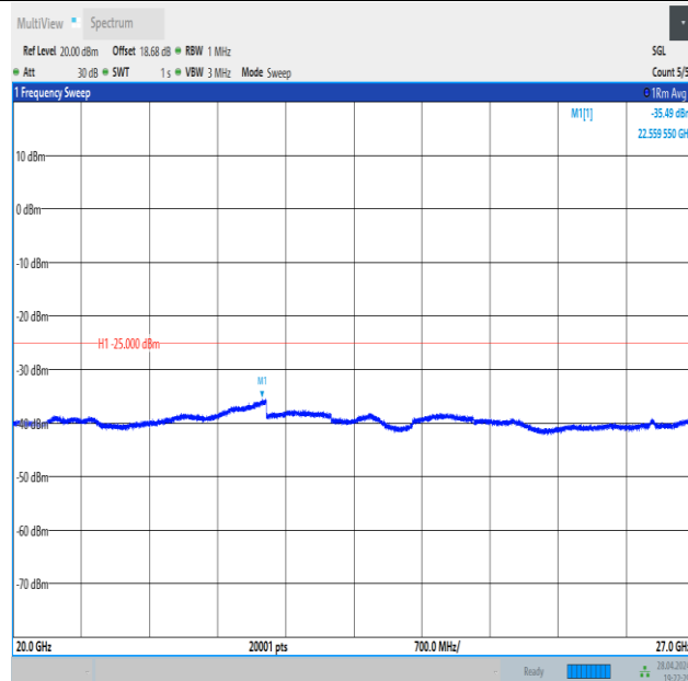
Band41_10MHz_QPSK_40620_50RB#0_20000~27000_20000~27000
