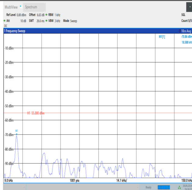
Band41_15MHz_QPSK_41515_1RB#74_0.009~0.15_0.009~0.15
