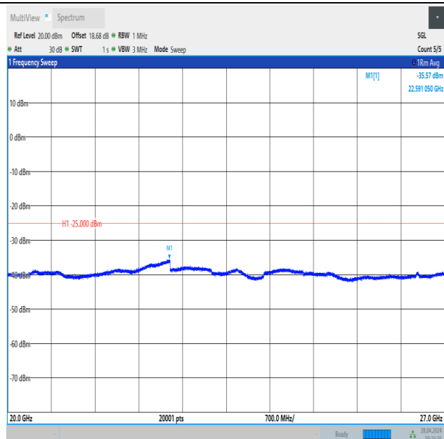
Band41_10MHz_QPSK_39700_50RB#0_20000~27000_20000~27000
