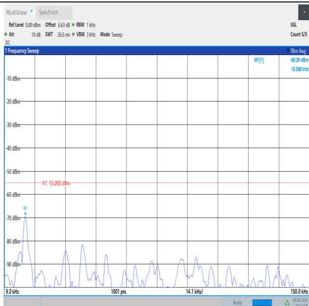
Band41_15MHz_QPSK_40620_1RB#74_0.009~0.15_0.009~0.15
