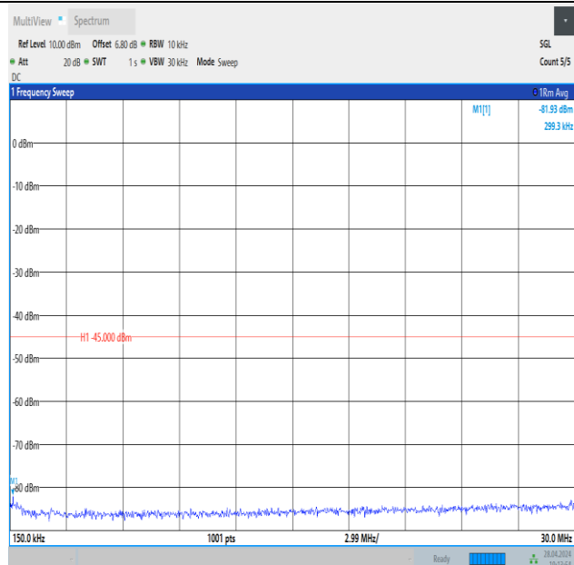
Band41_15MHz_16QAM_40620_1RB#74_0.15~30_0.15~30
