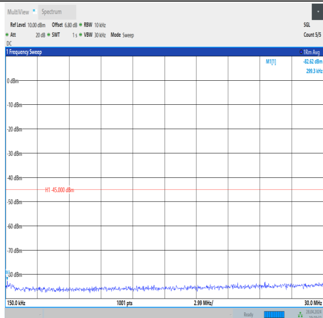
Band41_15MHz_16QAM_41515_1RB#74_0.15~30_0.15~30
