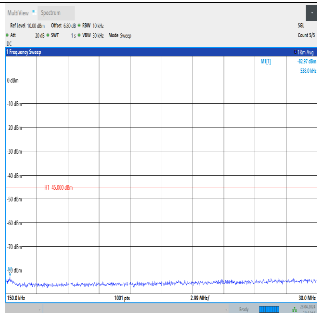
Band41_10MHz_QPSK_39700_1RB#49_0.15~30_0.15~30
