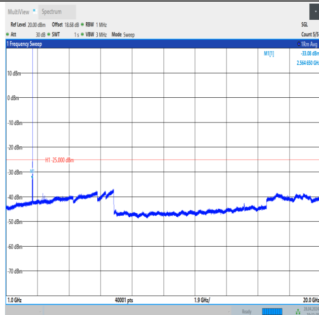
Band41_10MHz_QPSK_40620_1RB#49_1000~20000_1000~20000
