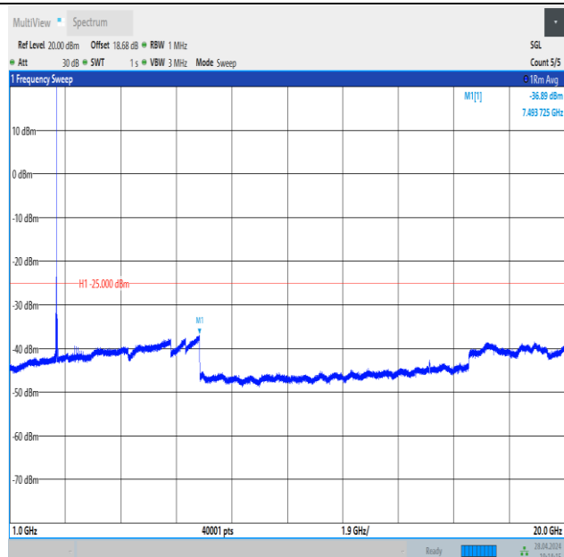
Band41_15MHz_16QAM_40620_1RB#74_1000~20000_1000~20000
