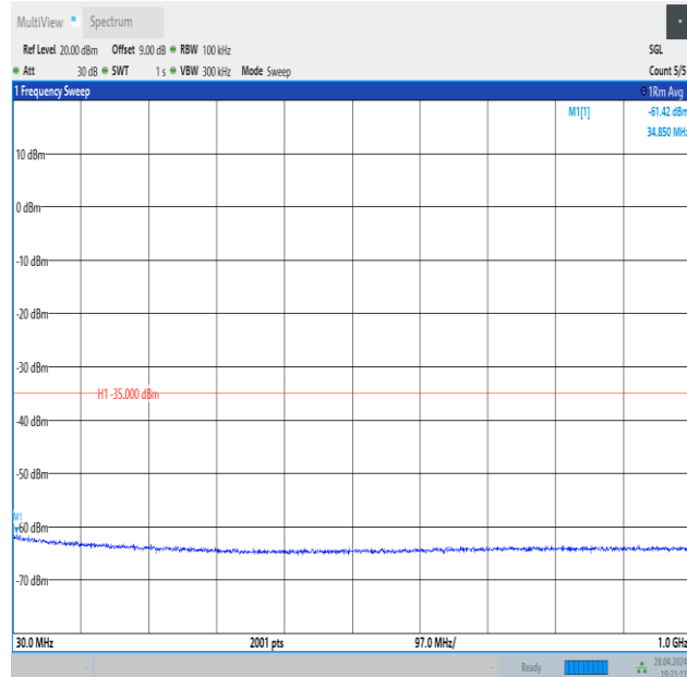
Band41_10MHz_QPSK_39700_50RB#0_30~1000_30~1000
