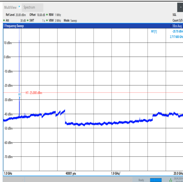
Band41_10MHz_QPSK_41540_1RB#0_1000~20000_1000~20000
