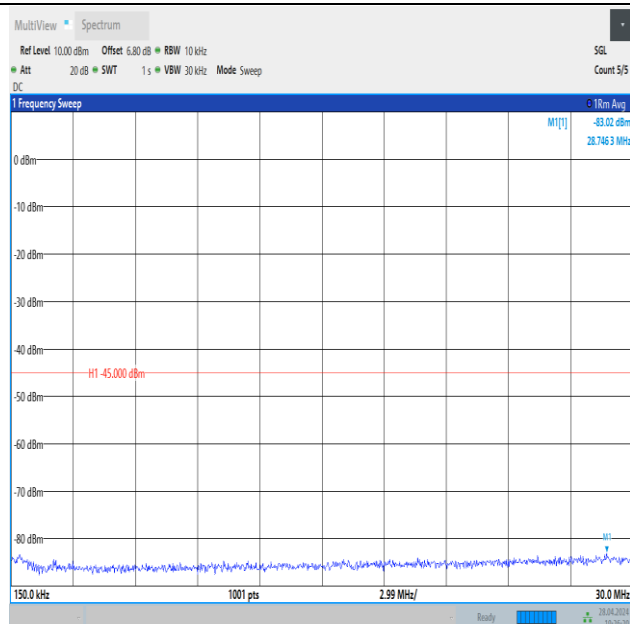
Band41_10MHz_QPSK_39700_1RB#0_0.15~30_0.15~30
