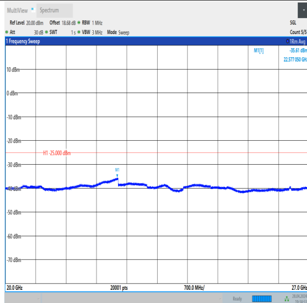
Band41_10MHz_QPSK_41540_1RB#49_20000~27000_20000~27000
