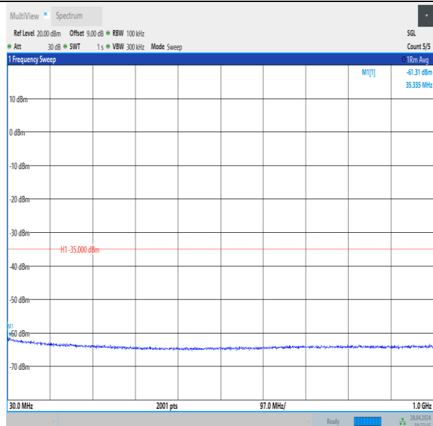
Band41_10MHz_16QAM_39700_1RB#0_30~1000_30~1000
