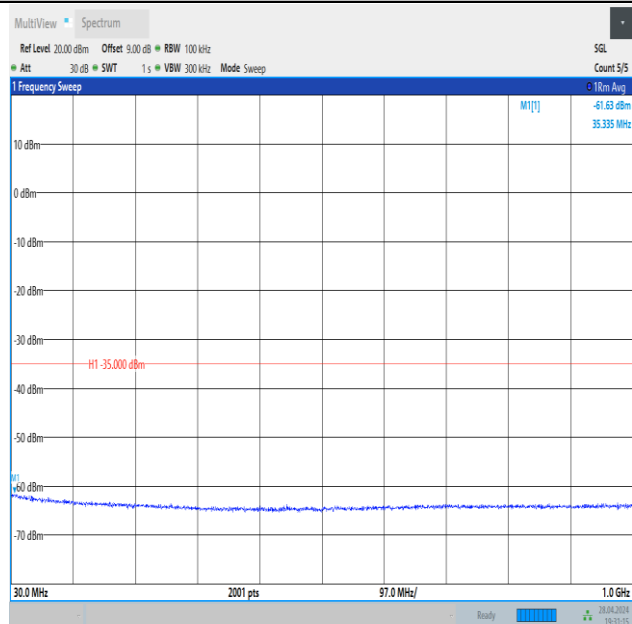
Band41_10MHz_QPSK_40620_1RB#49_30~1000_30~1000
