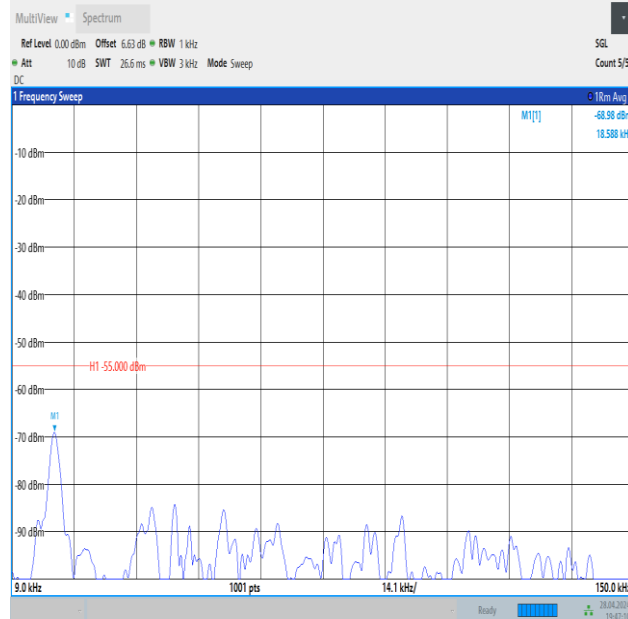
Band41_5MHz_QPSK_40620_1RB#24_0.009~0.15_0.009~0.15
