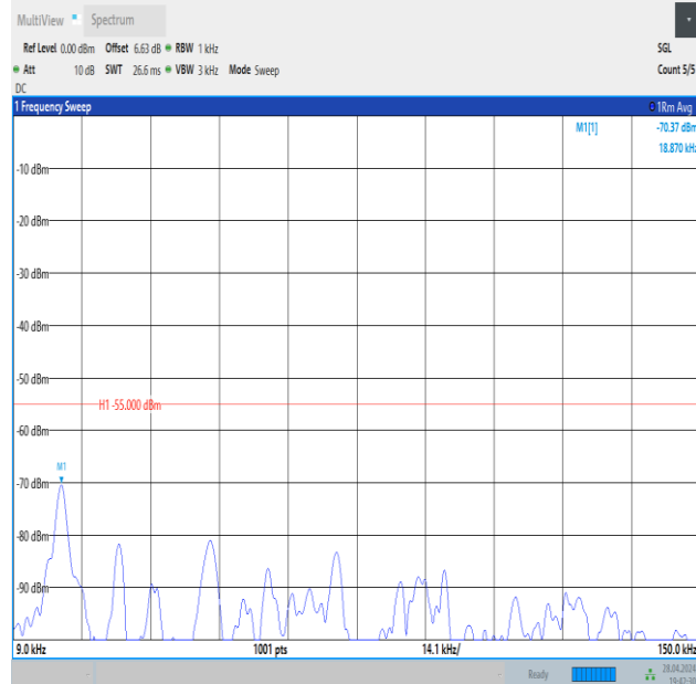
Band41_5MHz_QPSK_39675_1RB#24_0.009~0.15_0.009~0.15
