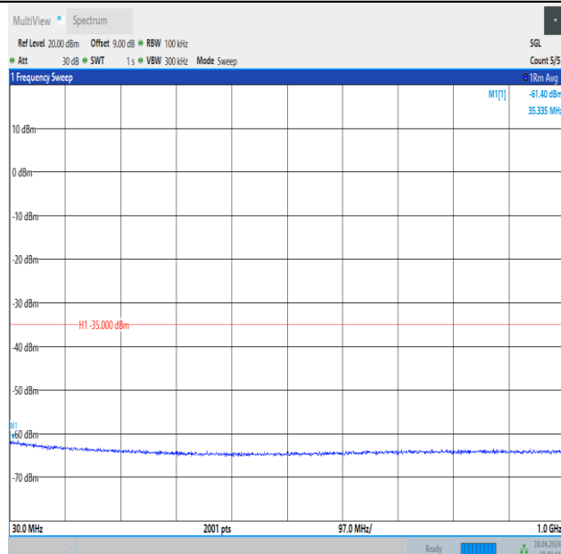
Band41_5MHz_QPSK_39675_1RB#0_30~1000_30~1000
