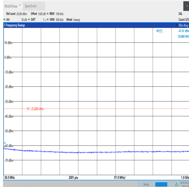
Band41_5MHz_16QAM_41565_1RB#0_30~1000_30~1000
