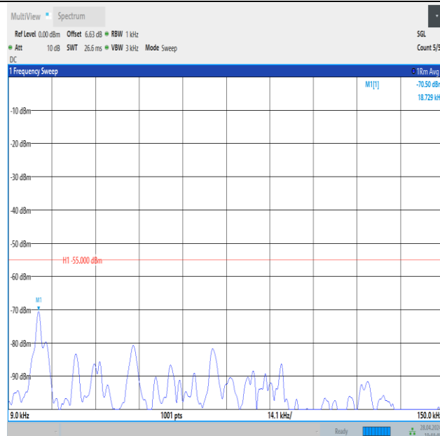
Band41_5MHz_16QAM_39675_25RB#0_0.009~0.15_0.009~0.15
