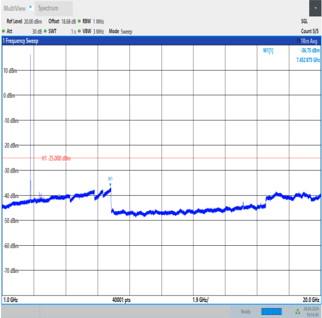
Band41_5MHz_16QAM_41565_25RB#0_1000~20000_1000~20000
