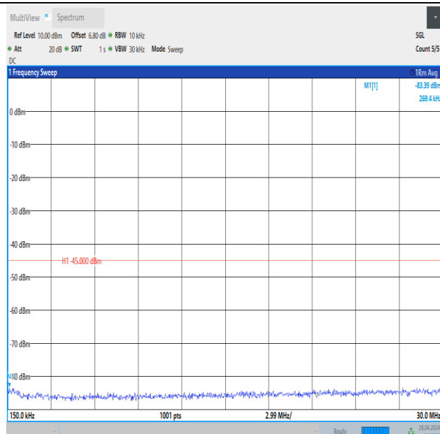
Band41_5MHz_QPSK_39675_1RB#24_0.15~30_0.15~30
