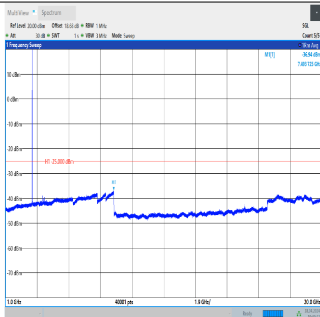
Band41_5MHz_QPSK_40620_25RB#0_1000~20000_1000~20000
