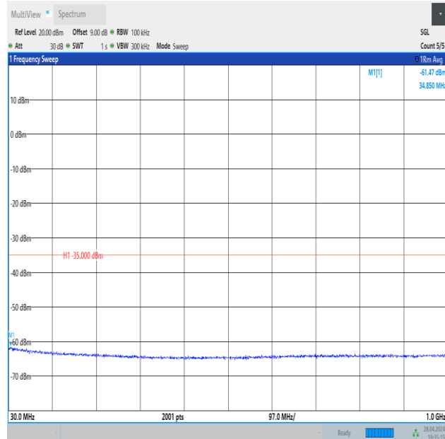
Band41_10MHz_16QAM_41540_1RB#49_30~1000_30~1000
