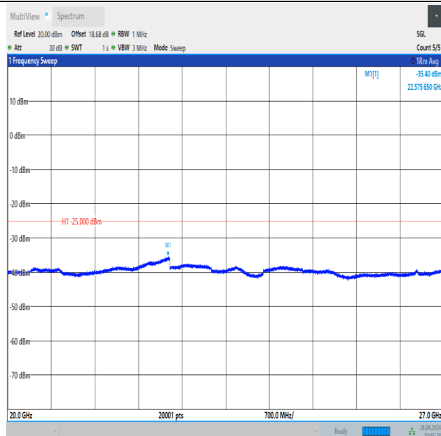
Band41_5MHz_16QAM_39675_25RB#0_20000~27000_20000~27000
