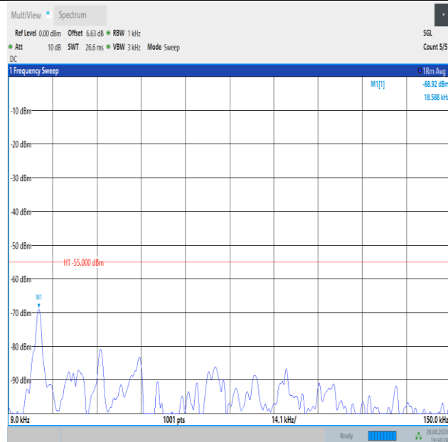
Band41_5MHz_QPSK_41565_1RB#0_0.009~0.15_0.009~0.15
