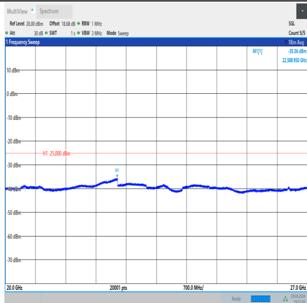
Band41_5MHz_QPSK_41565_1RB#0_20000~27000_20000~27000
