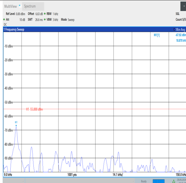
Band41_5MHz_QPSK_40620_1RB#0_0.009~0.15_0.009~0.15
