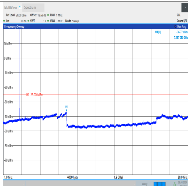
Band41_5MHz_QPSK_41565_1RB#0_1000~20000_1000~20000
