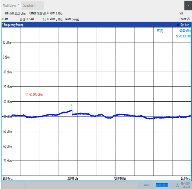
Band41_5MHz_QPSK_41565_25RB#0_20000~27000_20000~27000
