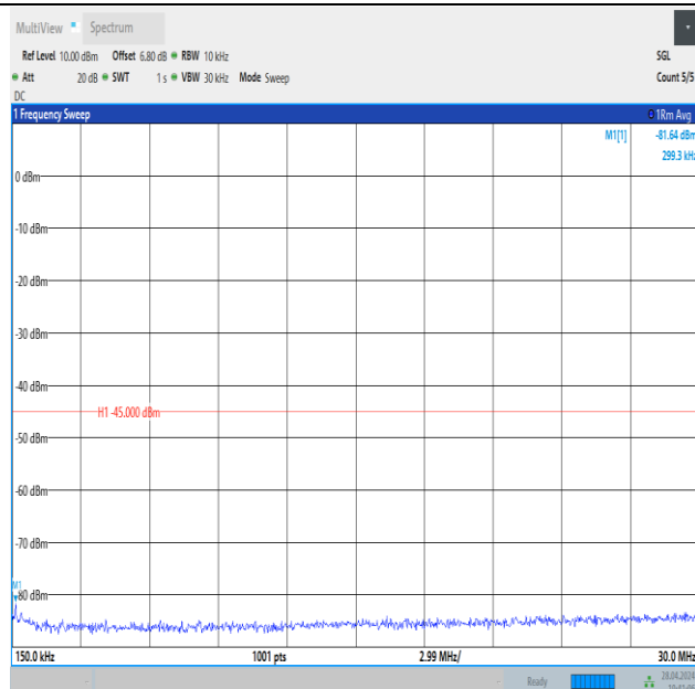
Band41_5MHz_QPSK_39675_1RB#0_0.15~30_0.15~30
