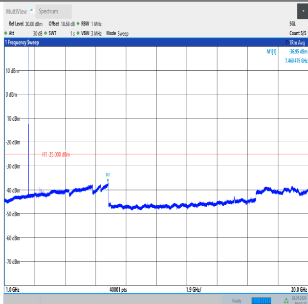
Band41_5MHz_QPSK_39675_1RB#0_1000~20000_1000~20000
