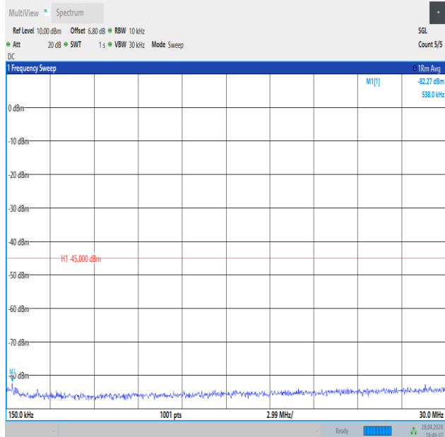
Band41_5MHz_16QAM_40620_1RB#0_0.15~30_0.15~30
