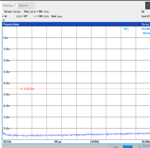
Band41_5MHz_QPSK_41565_25RB#0_0.15~30_0.15~30
