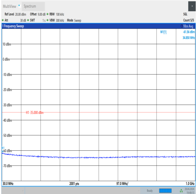
Band41_5MHz_16QAM_40620_1RB#24_30~1000_30~1000
