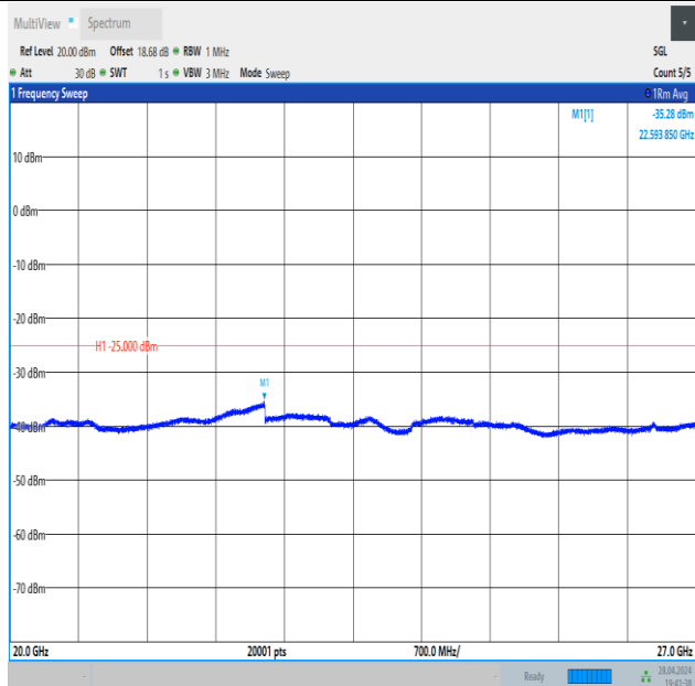
Band41_5MHz_QPSK_39675_1RB#0_20000~27000_20000~27000
