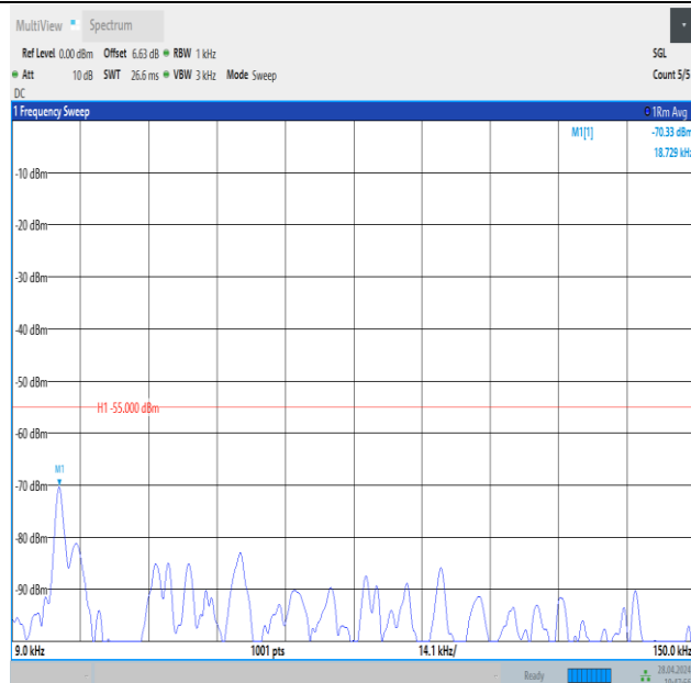
Band41_5MHz_16QAM_40620_1RB#24_0.009~0.15_0.009~0.15
