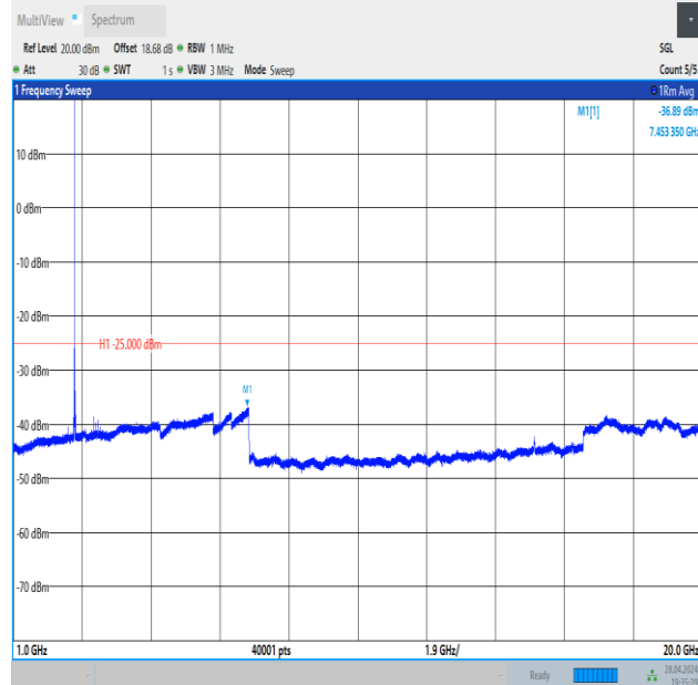
Band41_10MHz_16QAM_41540_1RB#49_1000~20000_1000~20000
