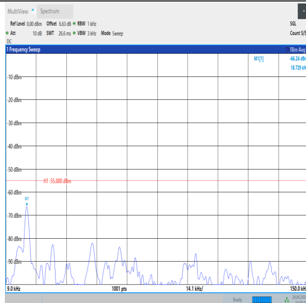
Band41_5MHz_16QAM_40620_25RB#0_0.009~0.15_0.009~0.15
