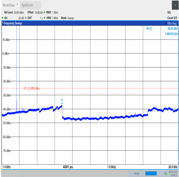
Band41_5MHz_16QAM_40620_1RB#24_1000~20000_1000~20000
