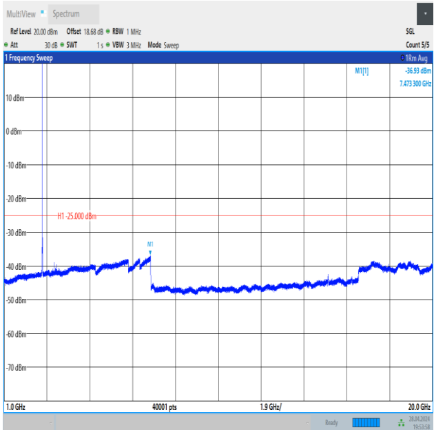
Band41_5MHz_QPSK_41565_25RB#0_1000~20000_1000~20000
