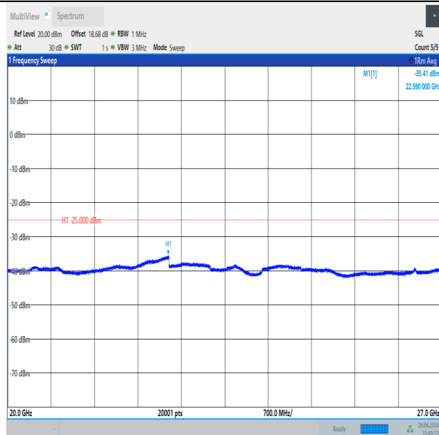
Band41_5MHz_QPSK_40620_25RB#0_20000~27000_20000~27000
