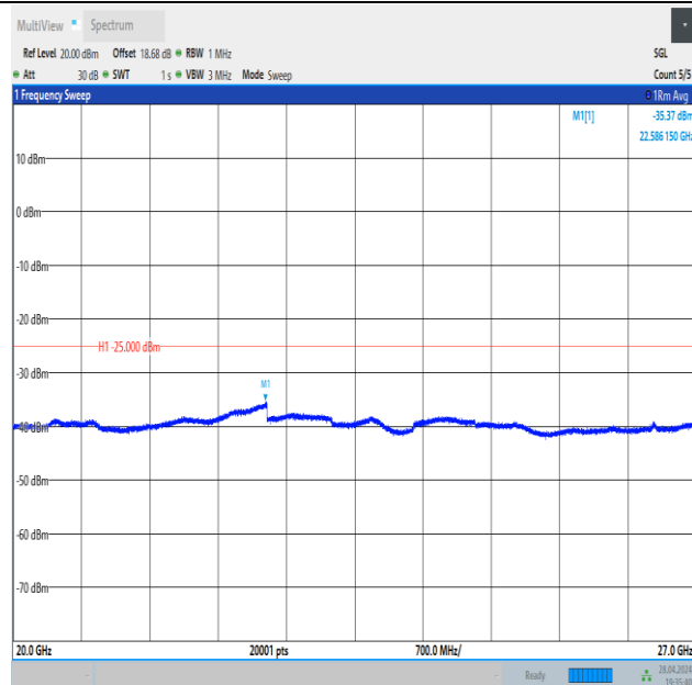
Band41_10MHz_16QAM_41540_1RB#49_20000~27000_20000~27000
