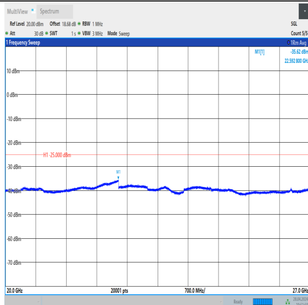
Band41_5MHz_16QAM_41565_1RB#0_20000~27000_20000~27000
