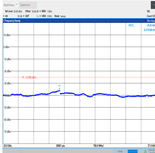
Band41_5MHz_16QAM_40620_1RB#0_20000~27000_20000~27000
