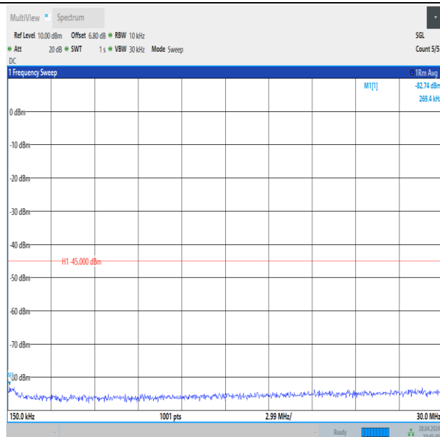
Band41_5MHz_QPSK_40620_1RB#0_0.15~30_0.15~30
