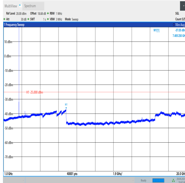
Band41_5MHz_QPSK_40620_1RB#24_1000~20000_1000~20000
