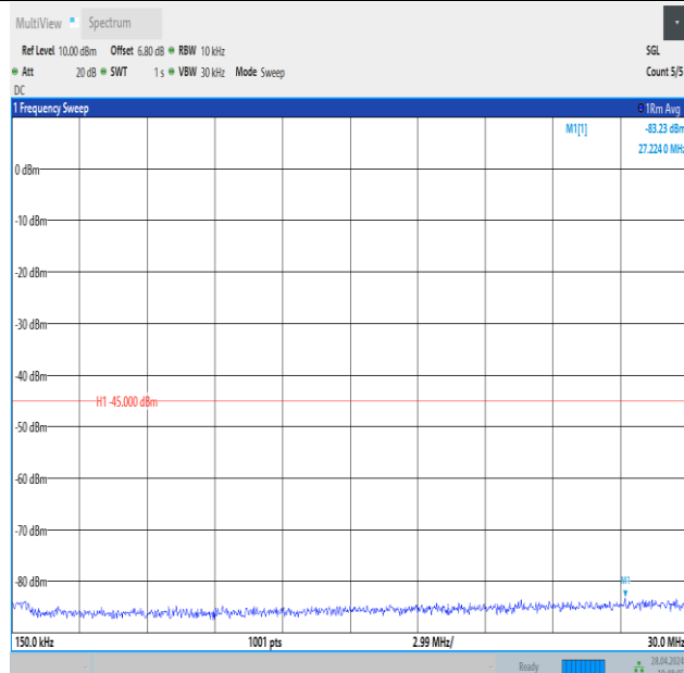
Band41_5MHz_16QAM_40620_1RB#24_0.15~30_0.15~30
