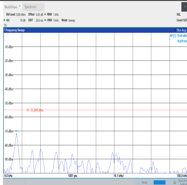
Band41_5MHz_QPSK_39675_1RB#0_0.009~0.15_0.009~0.15
