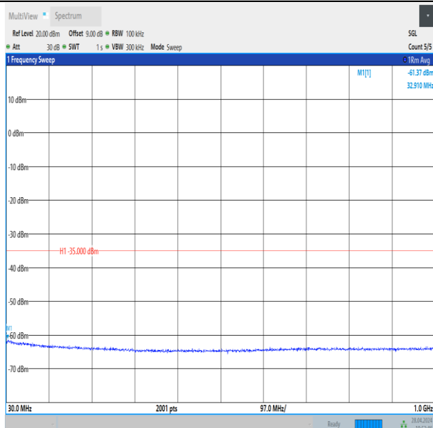
Band41_5MHz_QPSK_41565_25RB#0_30~1000_30~1000
