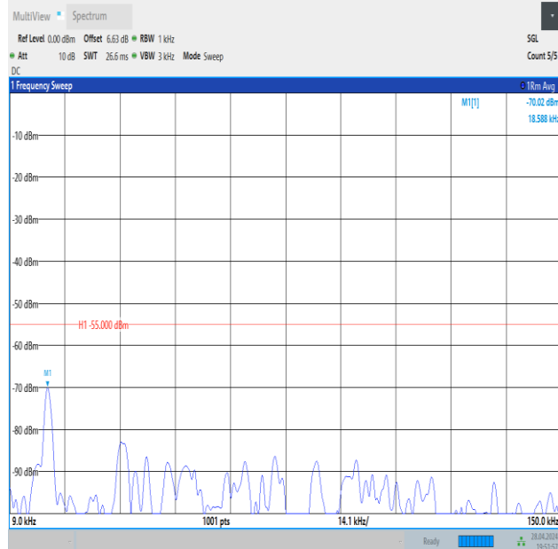
Band41_5MHz_QPSK_41565_1RB#24_0.009~0.15_0.009~0.15
