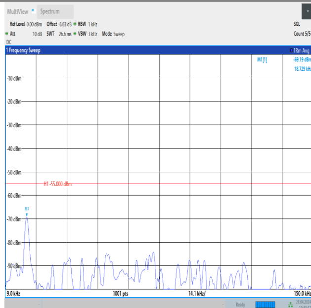
Band41_5MHz_16QAM_39675_1RB#24_0.009~0.15_0.009~0.15
