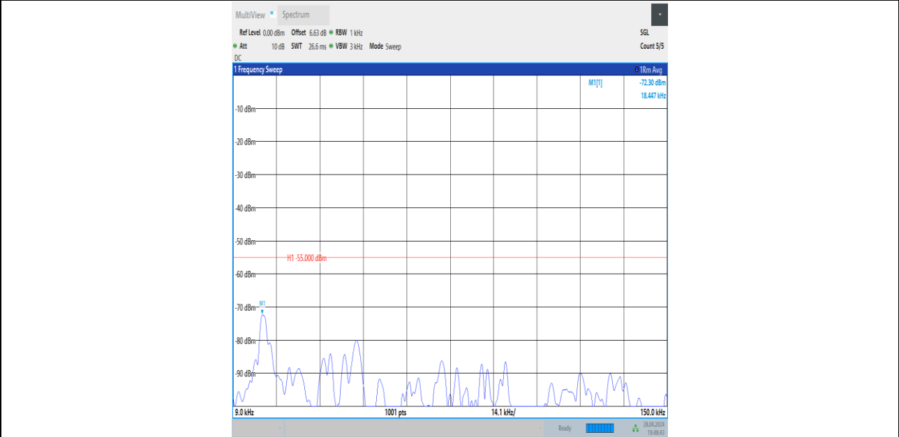
Band41_5MHz_QPSK_40620_25RB#0_0.009~0.15_0.009~0.15
