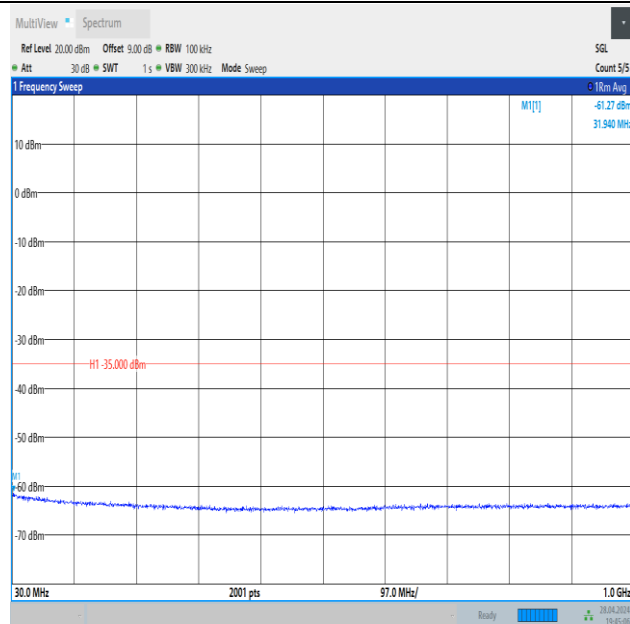
Band41_5MHz_16QAM_39675_25RB#0_30~1000_30~1000
