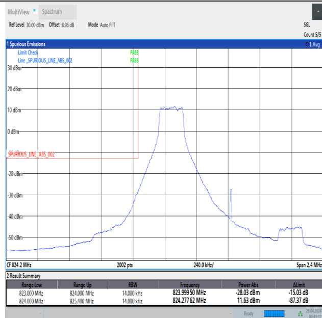
Band5_1.4MHz_QPSK_20407_1RB#0
