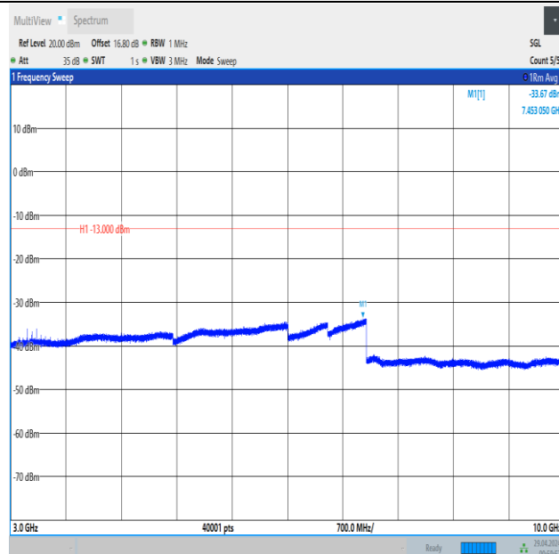
Band5_1.4MHz_QPSK_20407_1RB#5_3000~10000_3000~10000
