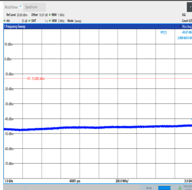
Band5_1.4MHz_16QAM_20525_6RB#0_1000~3000_1000~3000
