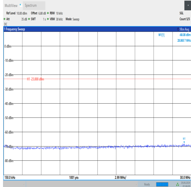
Band5_1.4MHz_QPSK_20525_1RB#5_0.15~30_0.15~30
