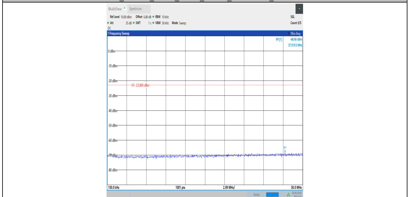
Band5_1.4MHz_QPSK_20407_1RB#0_0.15~30_0.15~30
