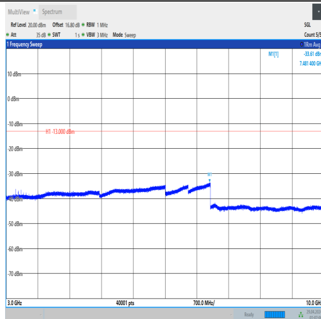
Band5_1.4MHz_16QAM_20525_6RB#0_3000~10000_3000~10000
