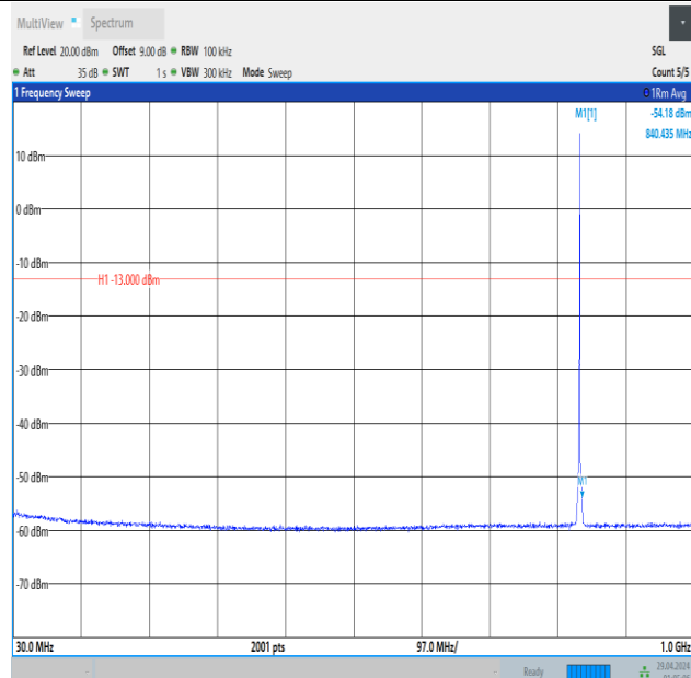
Band5_1.4MHz_16QAM_20525_1RB#5_30~1000_30~1000
