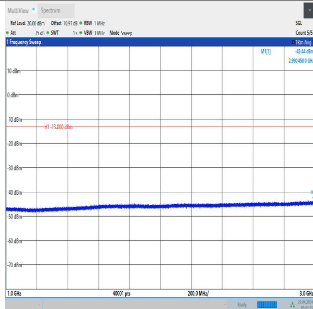
Band5_1.4MHz_QPSK_20407_6RB#0_1000~3000_1000~3000
