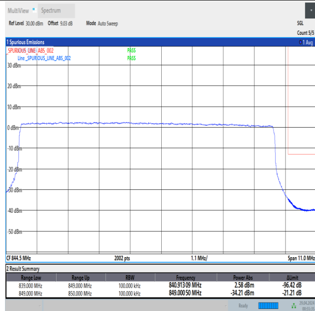
Band5_10MHz_QPSK_20600_50RB#0
