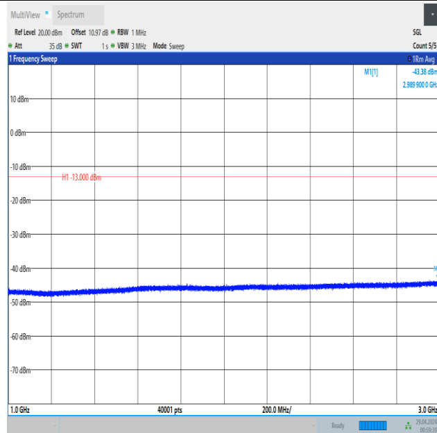
Band5_1.4MHz_QPSK_20407_1RB#5_1000~3000_1000~3000
