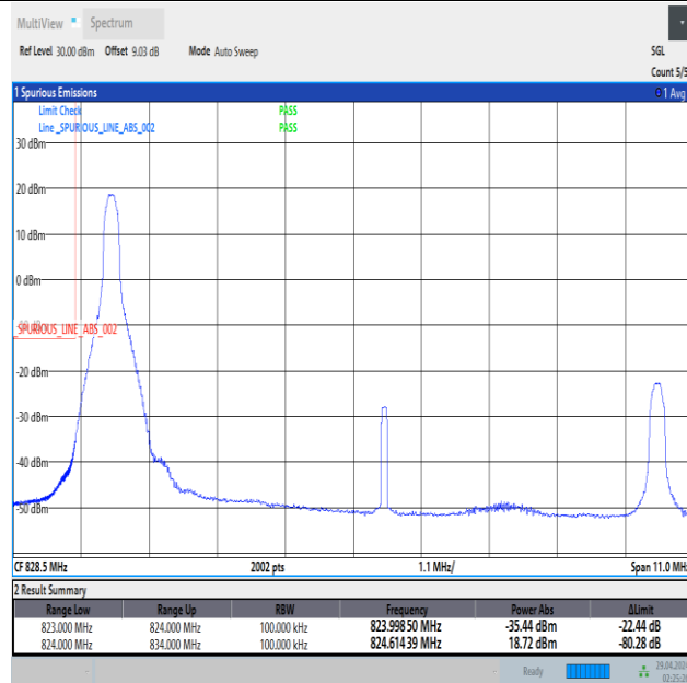
Band5_10MHz_16QAM_20450_1RB#0
