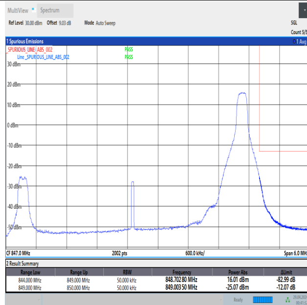
Band5_5MHz_16QAM_20625_1RB#24
