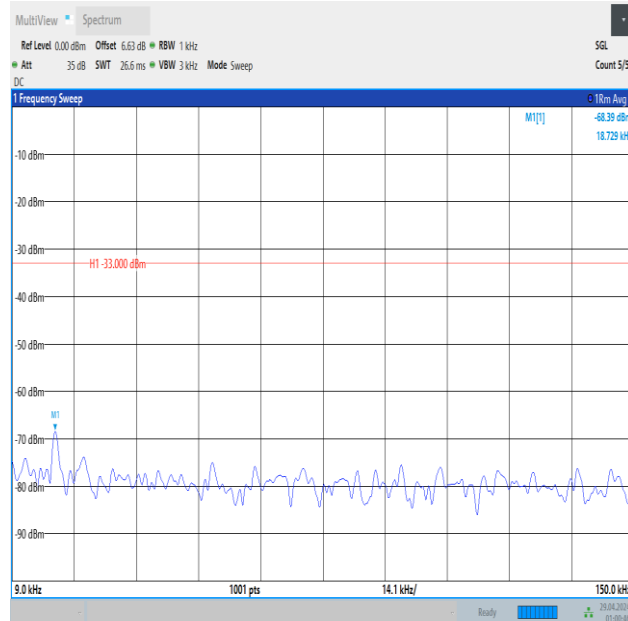
Band5_1.4MHz_QPSK_20407_6RB#0_0.009~0.15_0.009~0.15
