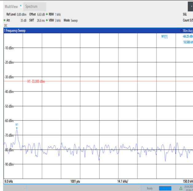
Band5_1.4MHz_16QAM_20525_6RB#0_0.009~0.15_0.009~0.15
