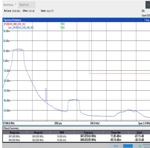
Band5_1.4MHz_QPSK_20643_1RB#0
