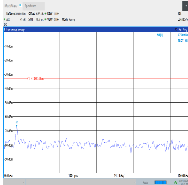
Band5_1.4MHz_QPSK_20525_1RB#0_0.009~0.15_0.009~0.15
