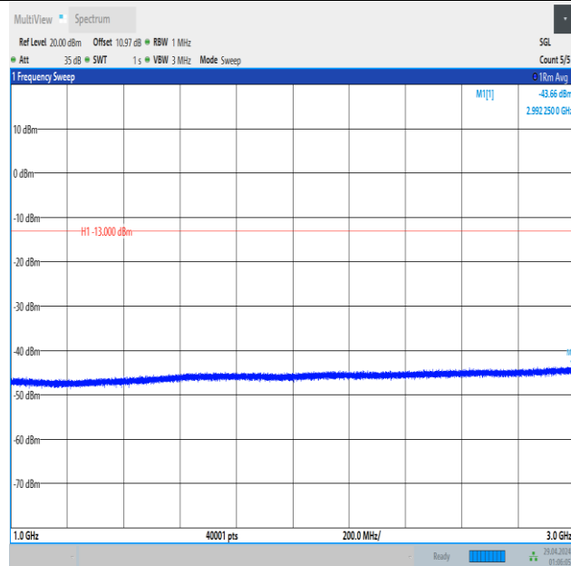
Band5_1.4MHz_QPSK_20525_6RB#0_1000~3000_1000~3000
