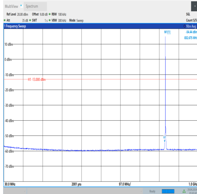
Band5_1.4MHz_QPSK_20525_1RB#0_30~1000_30~1000
