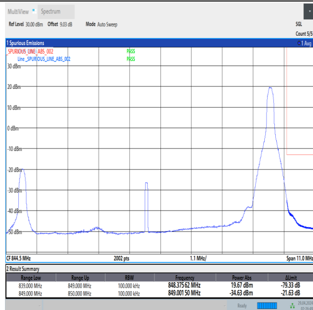
Band5_10MHz_QPSK_20600_1RB#49
