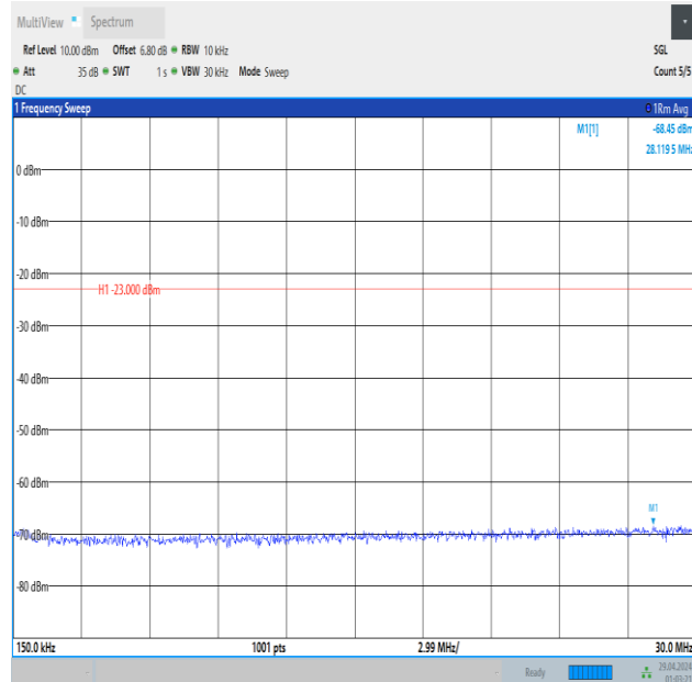
Band5_1.4MHz_16QAM_20525_1RB#0_0.15~30_0.15~30
