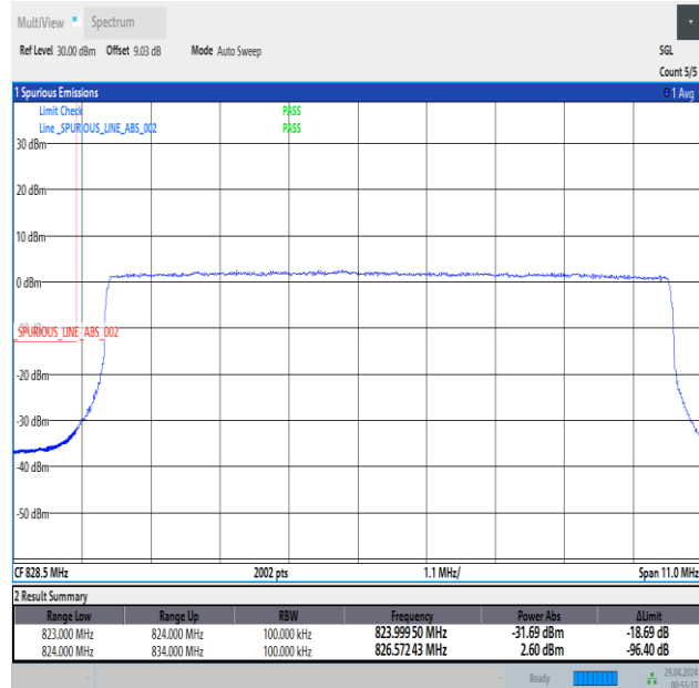
Band5_10MHz_QPSK_20450_50RB#0
