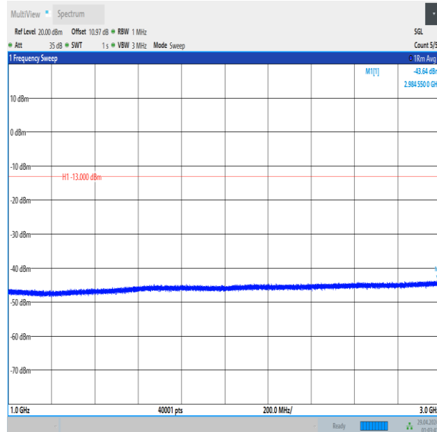
Band5_1.4MHz_16QAM_20525_1RB#0_1000~3000_1000~3000
