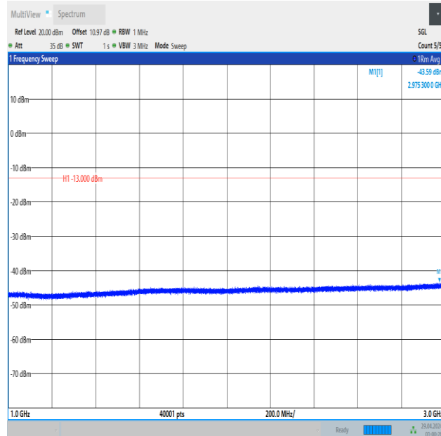
Band5_1.4MHz_16QAM_20407_1RB#5_1000~3000_1000~3000
