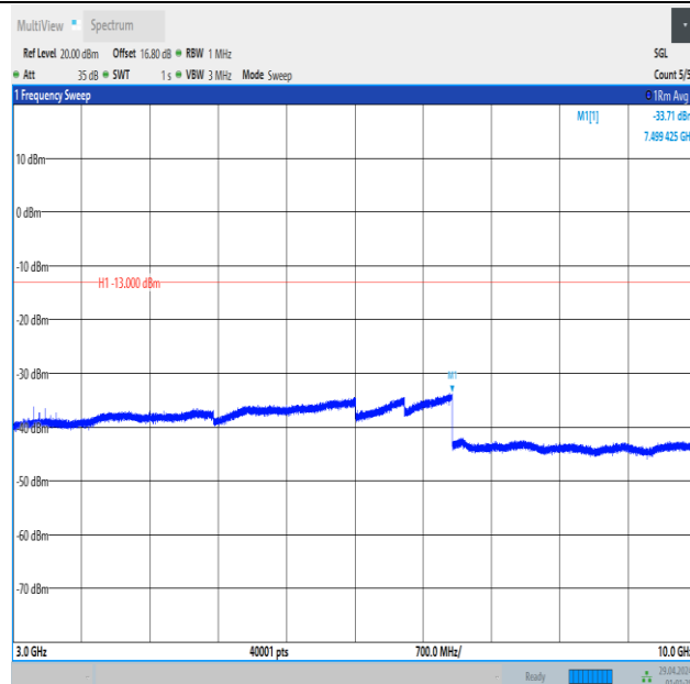
Band5_1.4MHz_QPSK_20407_6RB#0_3000~10000_3000~10000
