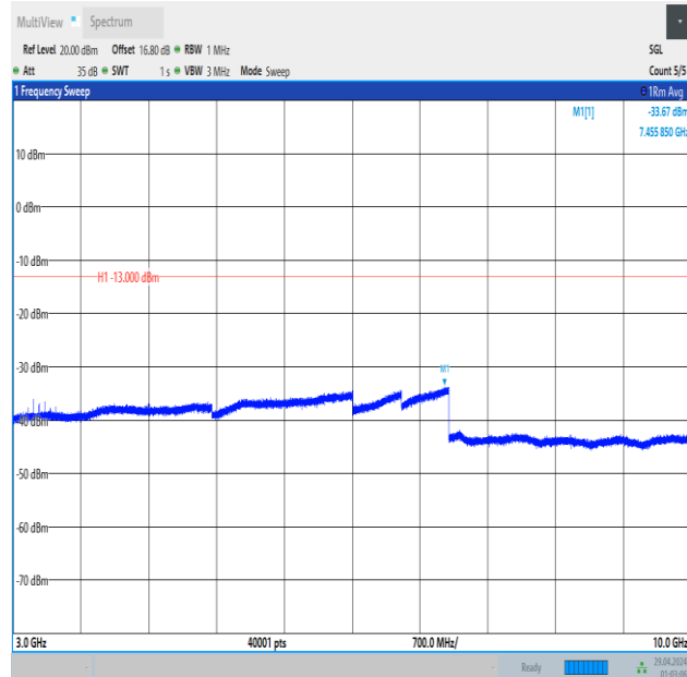
Band5_1.4MHz_QPSK_20525_1RB#0_3000~10000_3000~10000
