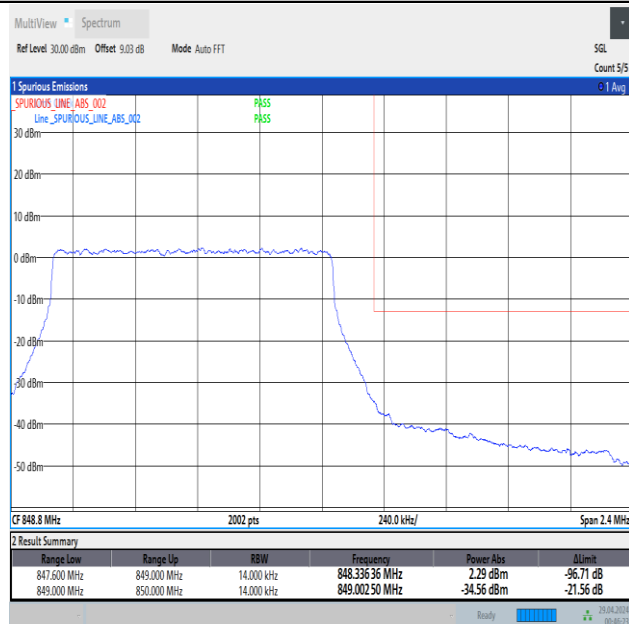
Band5_1.4MHz_16QAM_20643_6RB#0
