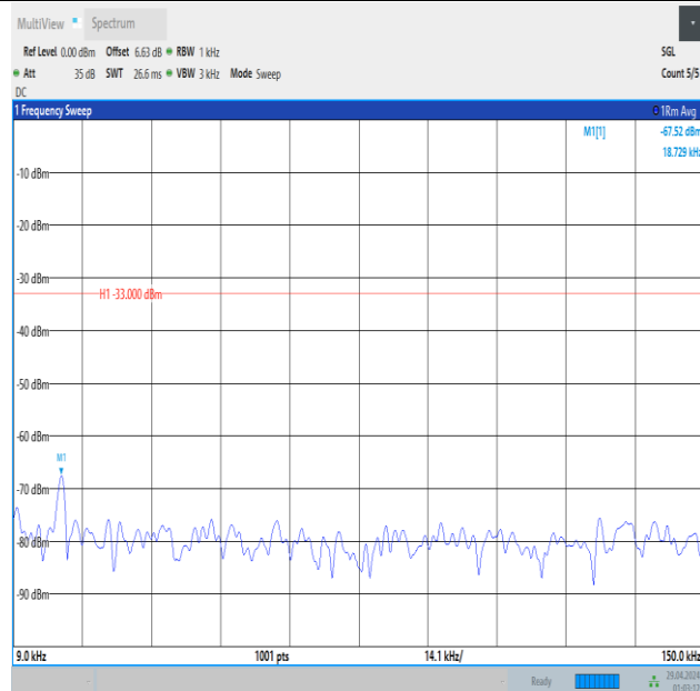
Band5_1.4MHz_16QAM_20525_1RB#0_0.009~0.15_0.009~0.15
