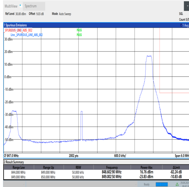
Band5_5MHz_QPSK_20625_1RB#24
