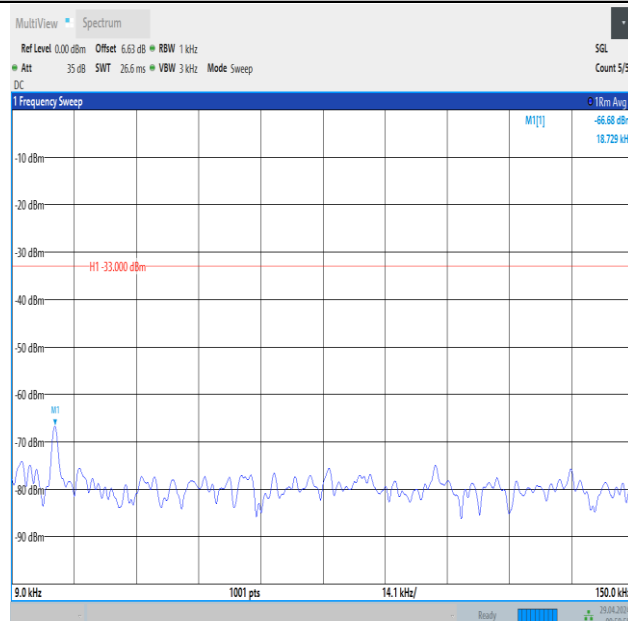
Band5_1.4MHz_16QAM_20407_1RB#5_0.009~0.15_0.009~0.15
