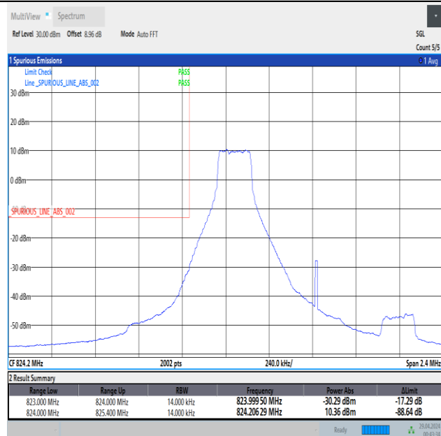
Band5_1.4MHz_16QAM_20407_1RB#0
