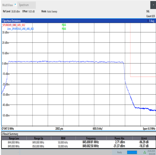
Band5_5MHz_QPSK_20625_25RB#0
