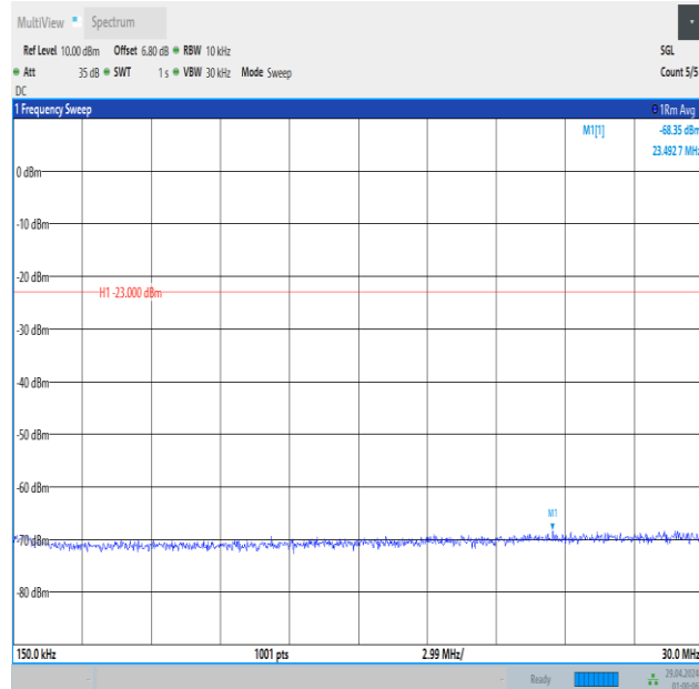
Band5_1.4MHz_16QAM_20407_1RB#5_0.15~30_0.15~30
