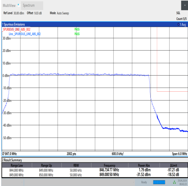
Band5_5MHz_16QAM_20625_25RB#0
