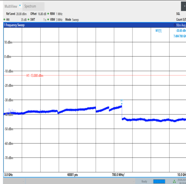
Band5_1.4MHz_16QAM_20407_1RB#0_3000~10000_3000~10000
