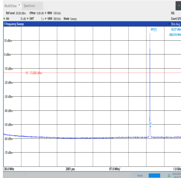
Band5_1.4MHz_QPSK_20407_1RB#5_30~1000_30~1000
