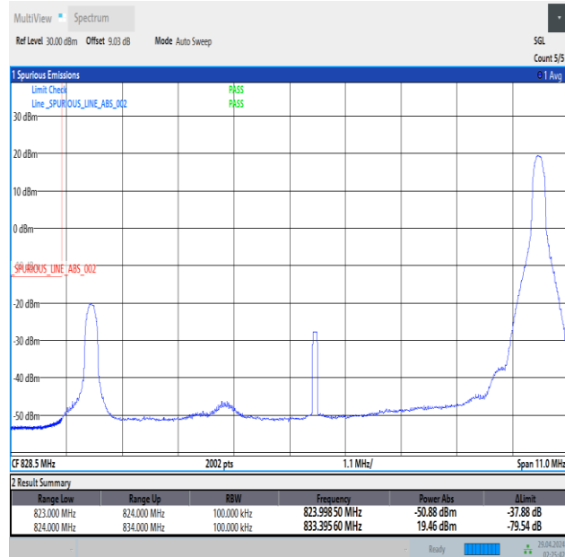
Band5_10MHz_QPSK_20450_1RB#49
