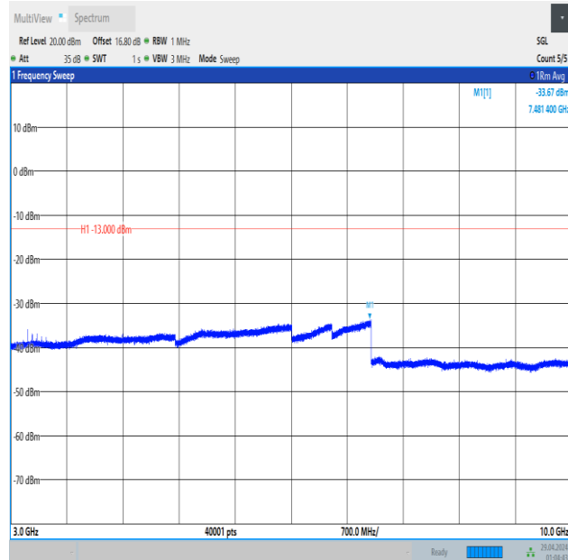
Band5_1.4MHz_QPSK_20525_1RB#5_3000~10000_3000~10000
