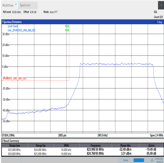
Band5_1.4MHz_QPSK_20407_6RB#0
