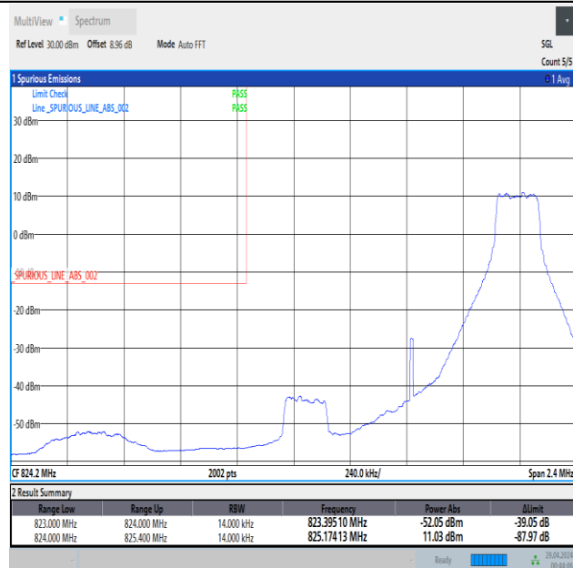
Band5_1.4MHz_16QAM_20407_1RB#5
