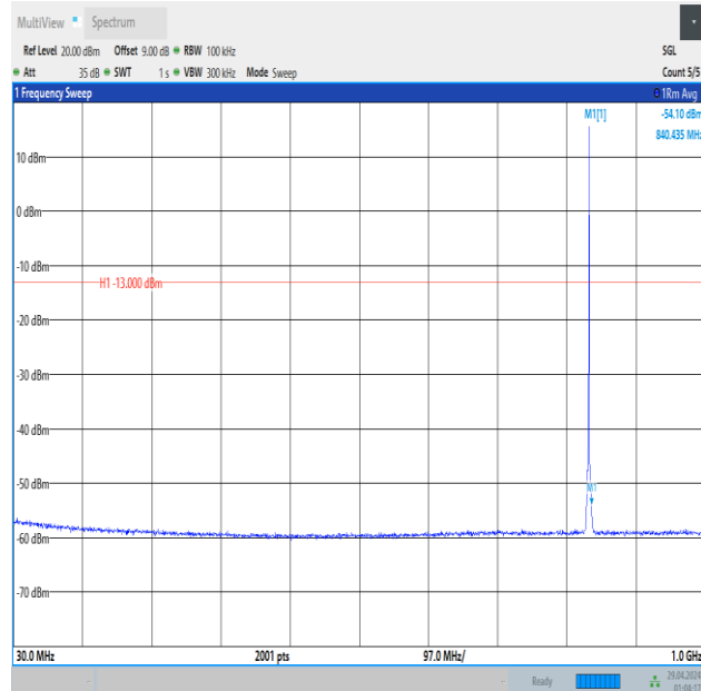
Band5_1.4MHz_QPSK_20525_1RB#5_30~1000_30~1000
