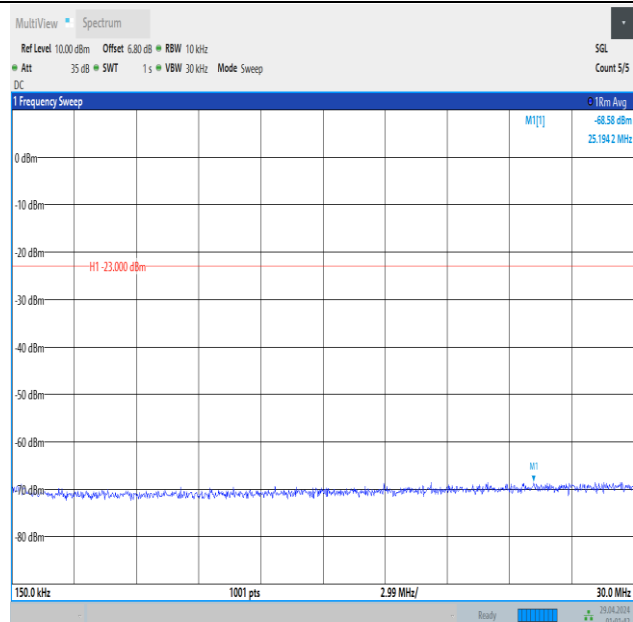
Band5_1.4MHz_16QAM_20407_6RB#0_0.15~30_0.15~30
