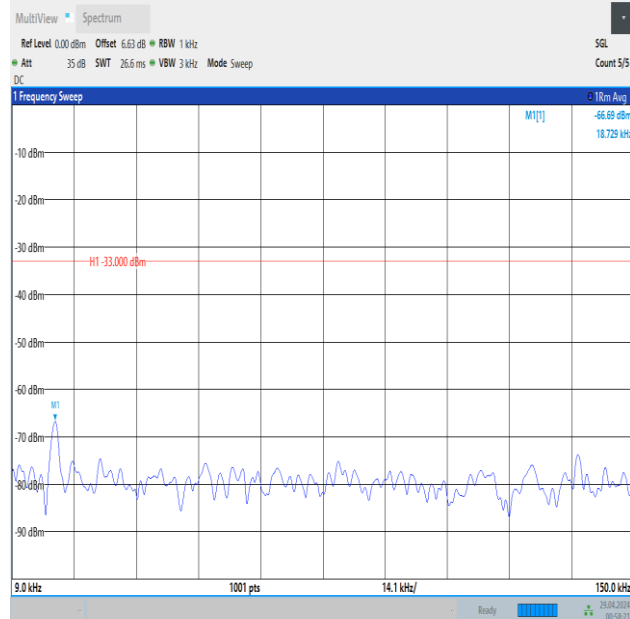
Band5_1.4MHz_16QAM_20407_1RB#0_0.009~0.15_0.009~0.15
