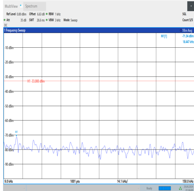
Band5_1.4MHz_QPSK_20525_1RB#5_0.009~0.15_0.009~0.15
