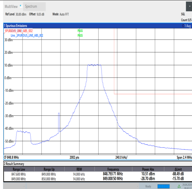
Band5_1.4MHz_16QAM_20643_1RB#5
