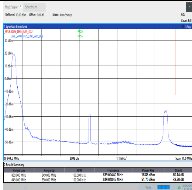
Band5_10MHz_16QAM_20600_1RB#0
