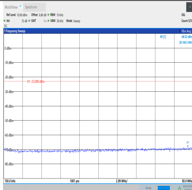
Band5_1.4MHz_16QAM_20525_6RB#0_0.15~30_0.15~30
