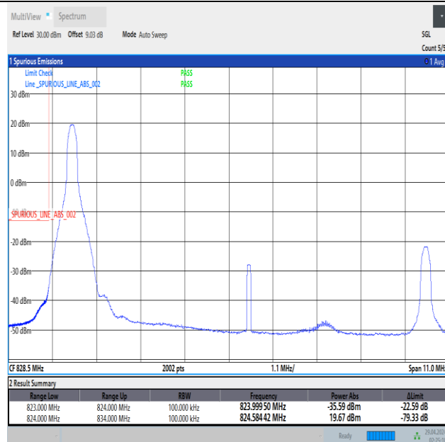
Band5_10MHz_QPSK_20450_1RB#0
