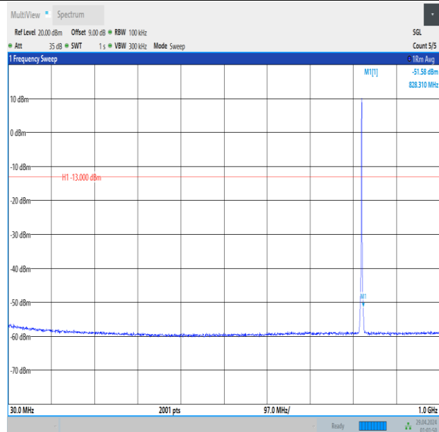
Band5_1.4MHz_16QAM_20407_6RB#0_30~1000_30~1000
