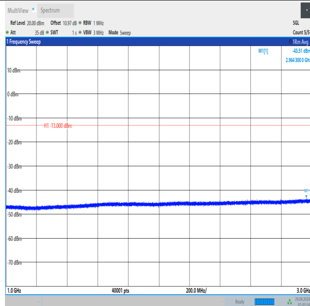
Band5_1.4MHz_QPSK_20525_1RB#0_1000~3000_1000~3000
