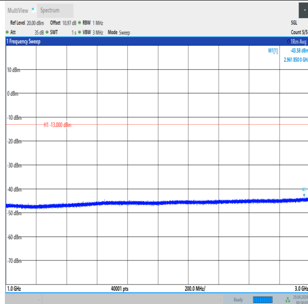
Band5_1.4MHz_QPSK_20407_1RB#0_1000~3000_1000~3000
