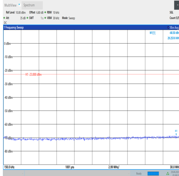
Band5_1.4MHz_QPSK_20407_6RB#0_0.15~30_0.15~30
