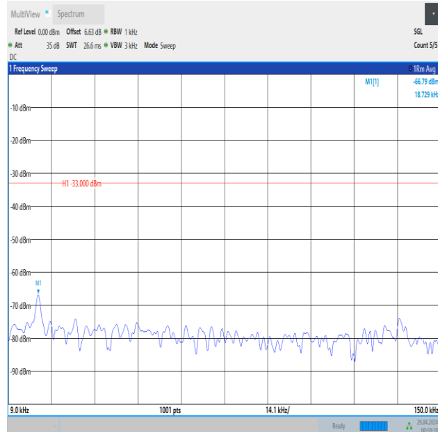
Band5_1.4MHz_QPSK_20407_1RB#5_0.009~0.15_0.009~0.15
