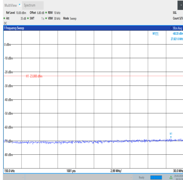
Band5_1.4MHz_QPSK_20407_1RB#5_0.15~30_0.15~30
