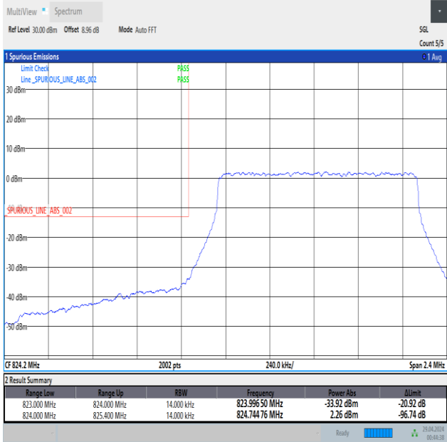
Band5_1.4MHz_16QAM_20407_6RB#0
