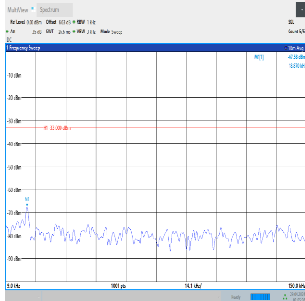
Band5_1.4MHz_QPSK_20525_6RB#0_0.009~0.15_0.009~0.15
