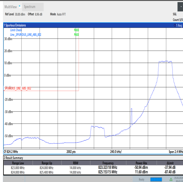
Band5_1.4MHz_QPSK_20407_1RB#5
