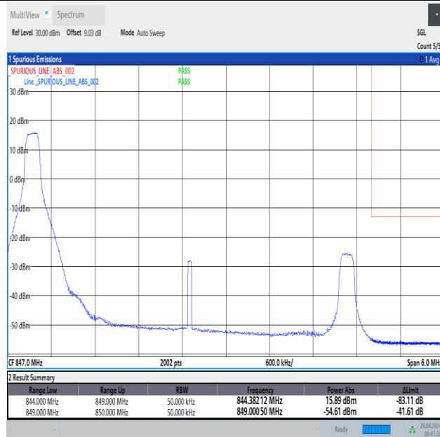
Band5_5MHz_16QAM_20625_1RB#0
