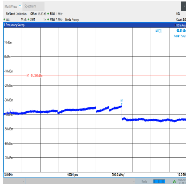
Band5_1.4MHz_16QAM_20407_6RB#0_3000~10000_3000~10000
