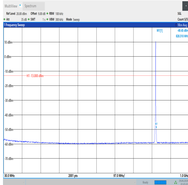
Band5_1.4MHz_QPSK_20407_6RB#0_30~1000_30~1000
