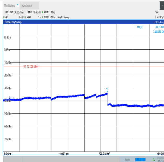
Band5_1.4MHz_16QAM_20525_1RB#0_3000~10000_3000~10000
