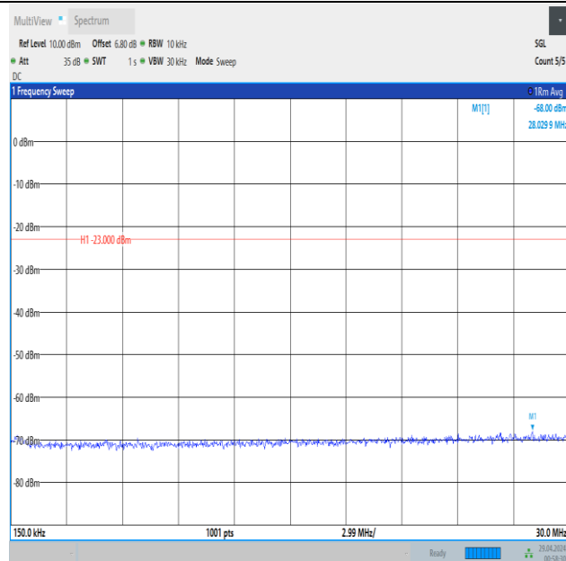
Band5_1.4MHz_16QAM_20407_1RB#0_0.15~30_0.15~30
