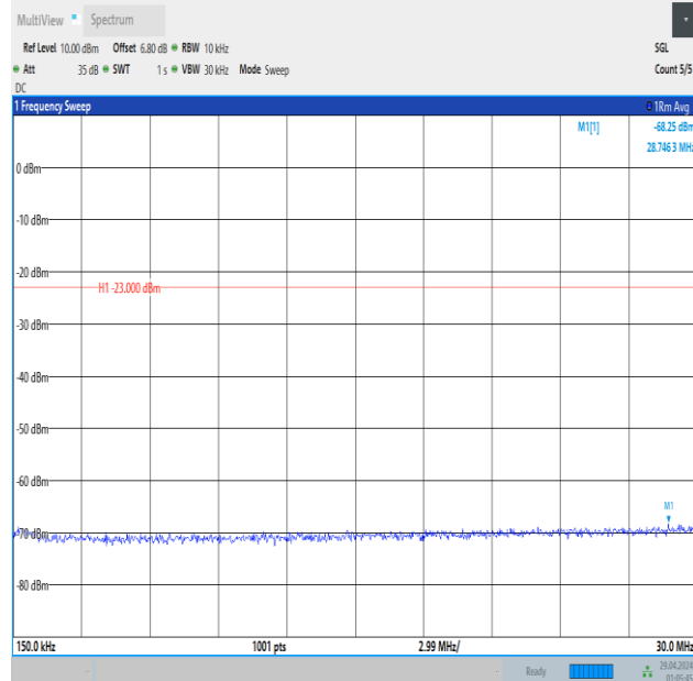
Band5_1.4MHz_QPSK_20525_6RB#0_0.15~30_0.15~30
