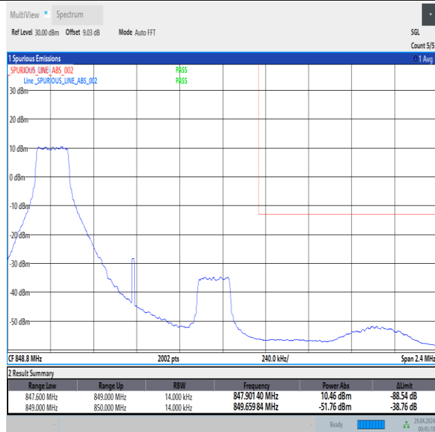
Band5_1.4MHz_16QAM_20643_1RB#0
