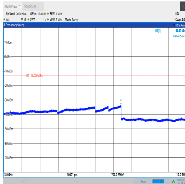
Band5_1.4MHz_16QAM_20407_1RB#5_3000~10000_3000~10000
