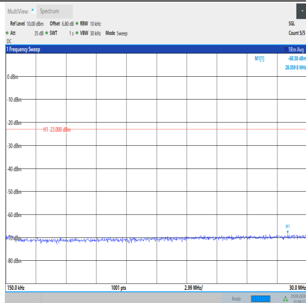
Band5_1.4MHz_16QAM_20525_1RB#5_0.15~30_0.15~30
