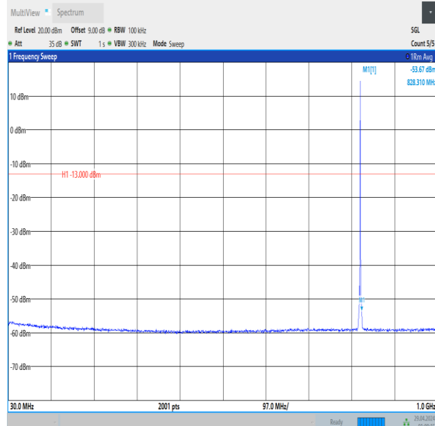
Band5_1.4MHz_16QAM_20407_1RB#5_30~1000_30~1000
