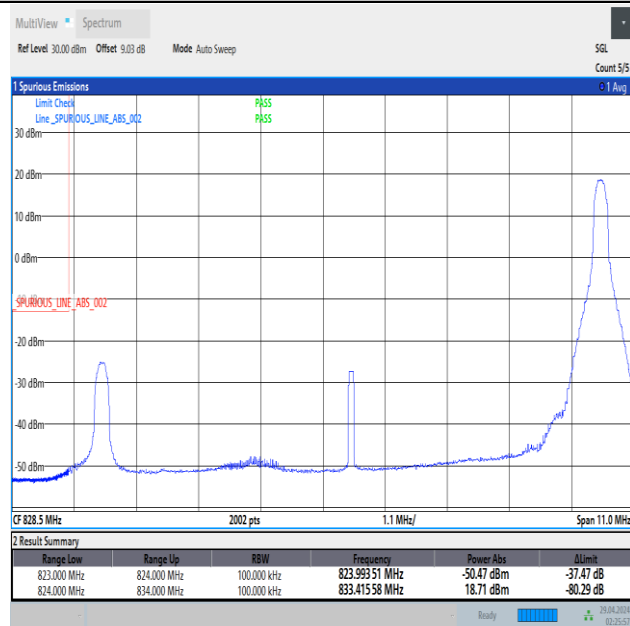
Band5_10MHz_16QAM_20450_1RB#49
