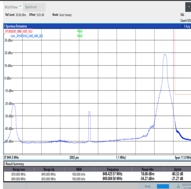
Band5_10MHz_16QAM_20600_1RB#49
