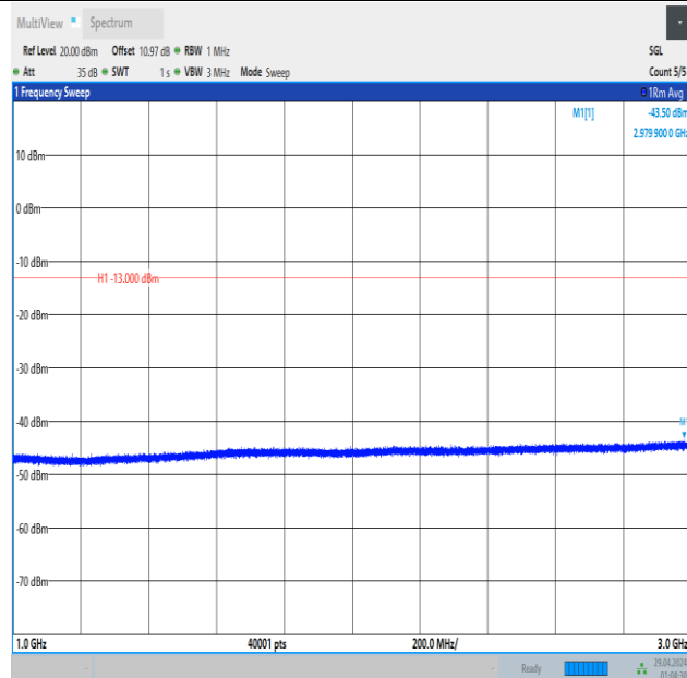
Band5_1.4MHz_QPSK_20525_1RB#5_1000~3000_1000~3000
