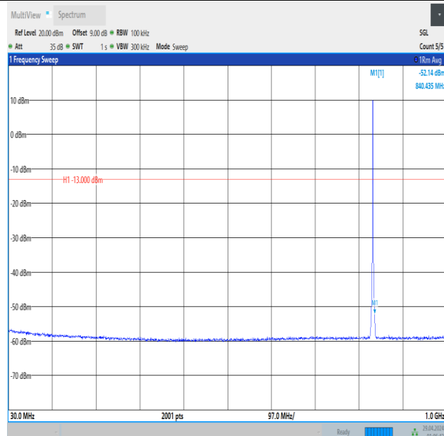
Band5_1.4MHz_16QAM_20525_6RB#0_30~1000_30~1000
