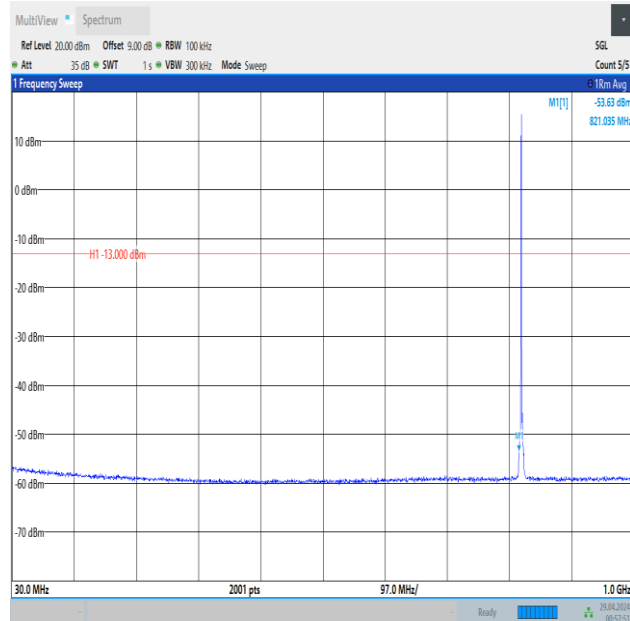
Band5_1.4MHz_QPSK_20407_1RB#0_30~1000_30~1000
