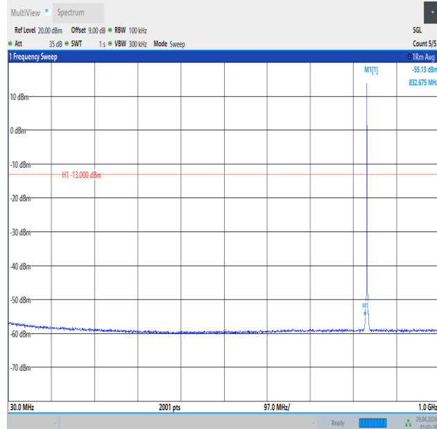
Band5_1.4MHz_16QAM_20525_1RB#0_30~1000_30~1000
