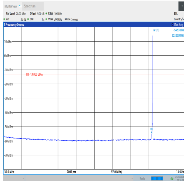
Band5_1.4MHz_16QAM_20407_1RB#0_30~1000_30~1000
