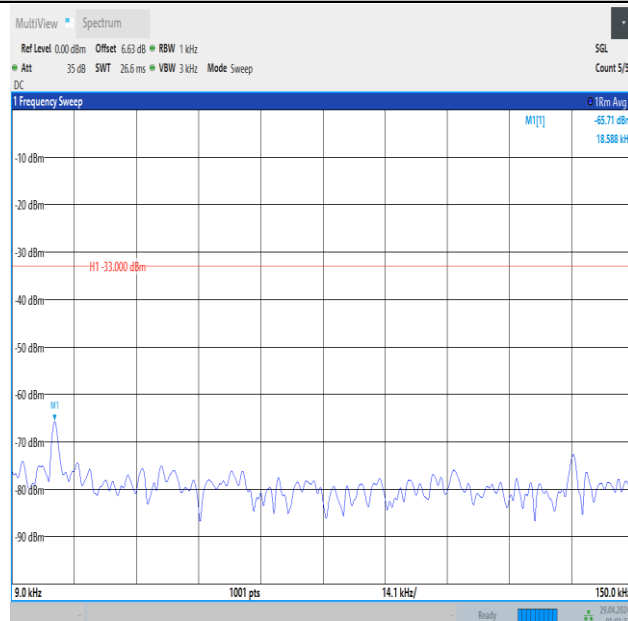
Band5_1.4MHz_16QAM_20407_6RB#0_0.009~0.15_0.009~0.15
