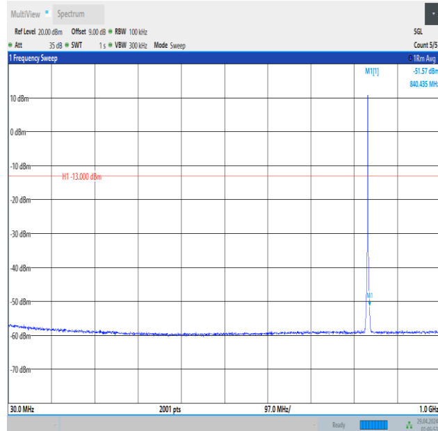
Band5_1.4MHz_QPSK_20525_6RB#0_30~1000_30~1000
