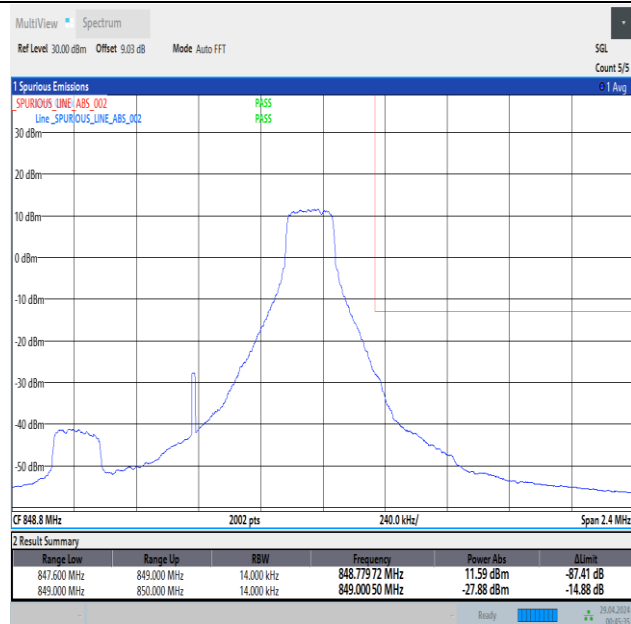
Band5_1.4MHz_QPSK_20643_1RB#5
