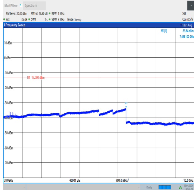
Band5_3MHz_16QAM_20415_1RB#0_3000~10000_3000~10000
