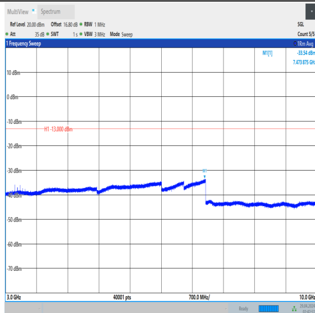
Band5_10MHz_16QAM_20600_1RB#0_3000~10000_3000~10000
