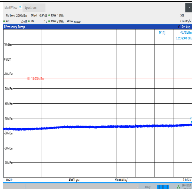
Band5_3MHz_16QAM_20415_1RB#0_1000~3000_1000~3000
