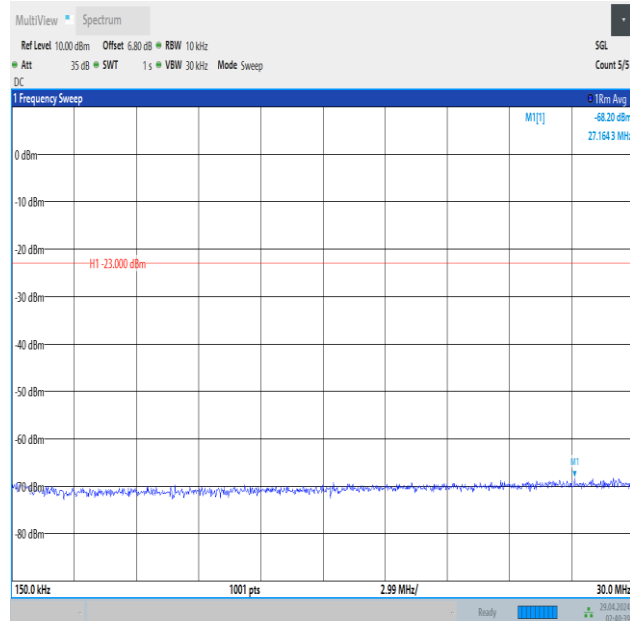
Band5_10MHz_16QAM_20525_1RB#49_0.15~30_0.15~30
