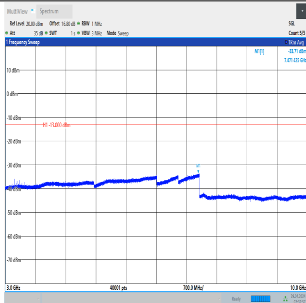
Band5_10MHz_16QAM_20450_1RB#49_3000~10000_3000~10000
