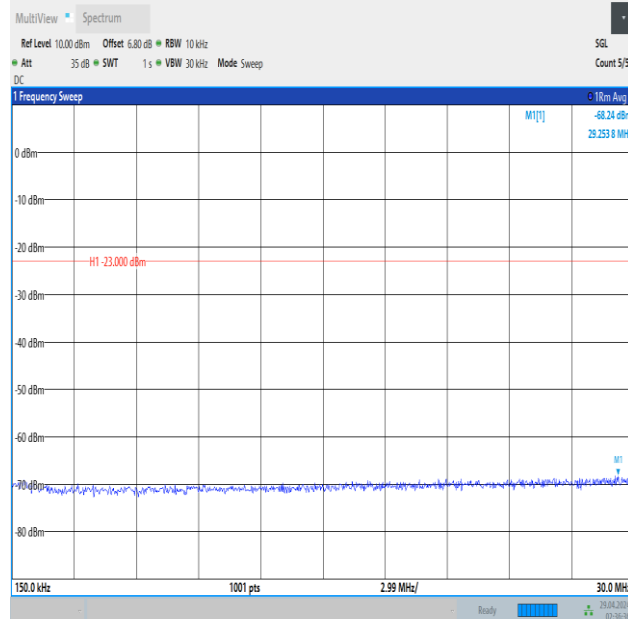
Band5_10MHz_QPSK_20450_1RB#49_0.15~30_0.15~30
