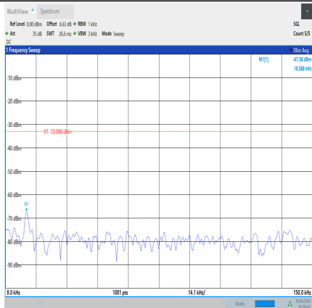
Band5_1.4MHz_16QAM_20643_1RB#5_0.009~0.15_0.009~0.15
