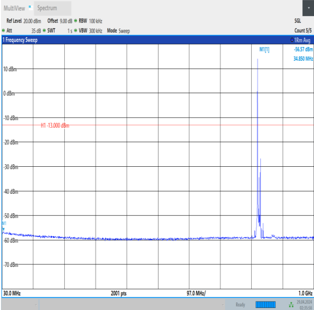
Band5_10MHz_16QAM_20450_1RB#0_30~1000_30~1000
