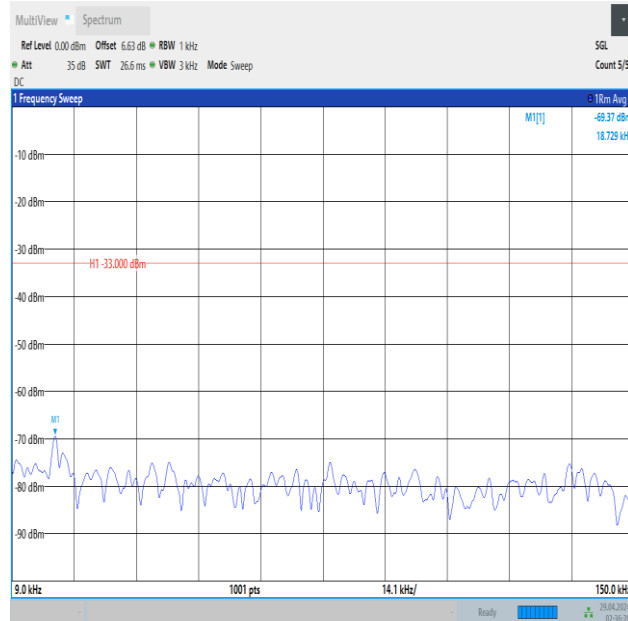
Band5_10MHz_QPSK_20450_1RB#49_0.009~0.15_0.009~0.15
