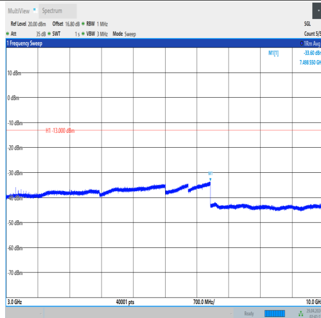
Band5_10MHz_16QAM_20525_1RB#49_3000~10000_3000~10000
