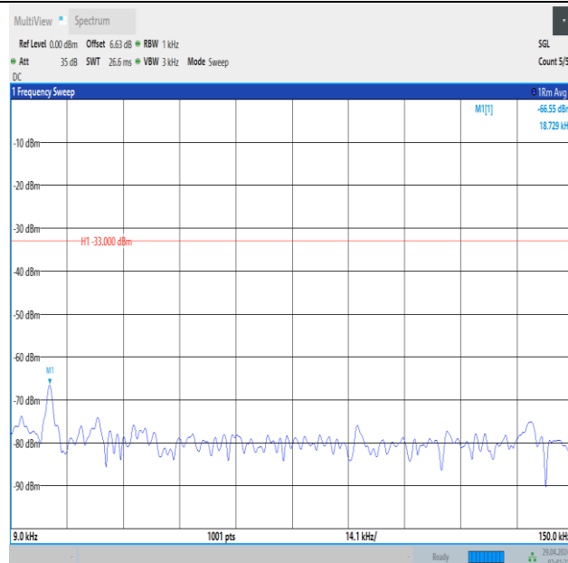
Band5_10MHz_QPSK_20600_1RB#0_0.009~0.15_0.009~0.15
