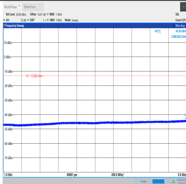
Band5_3MHz_QPSK_20415_1RB#0_1000~3000_1000~3000
