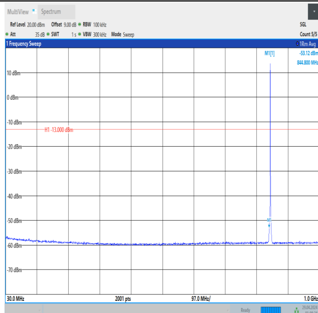
Band5_1.4MHz_16QAM_20643_1RB#0_30~1000_30~1000
