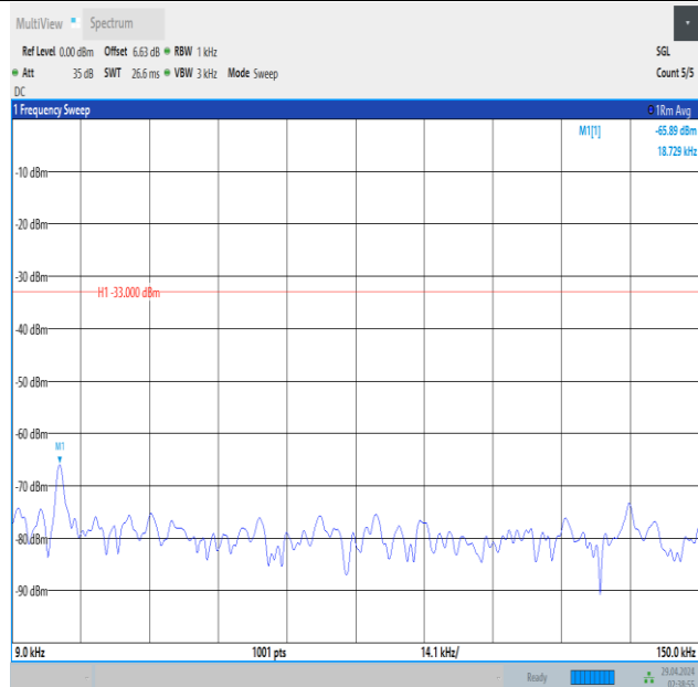
Band5_10MHz_16QAM_20525_1RB#0_0.009~0.15_0.009~0.15
