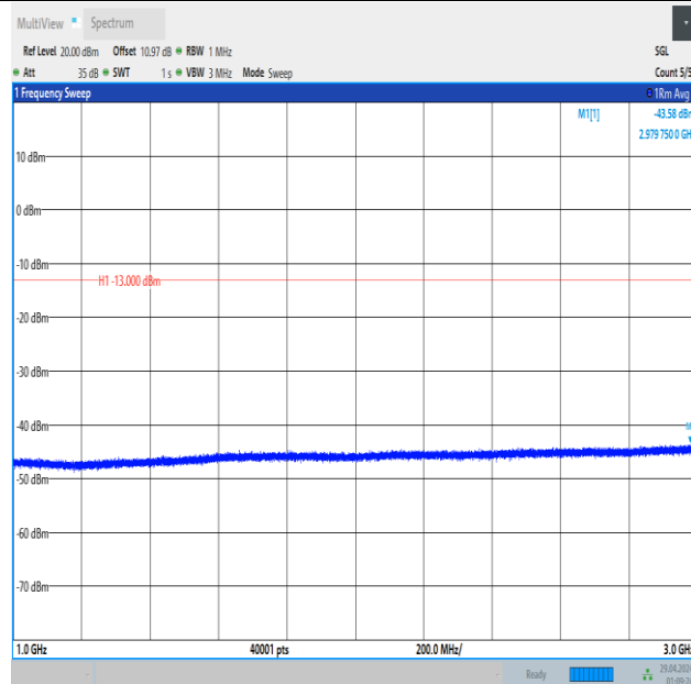
Band5_1.4MHz_QPSK_20643_1RB#5_1000~3000_1000~3000
