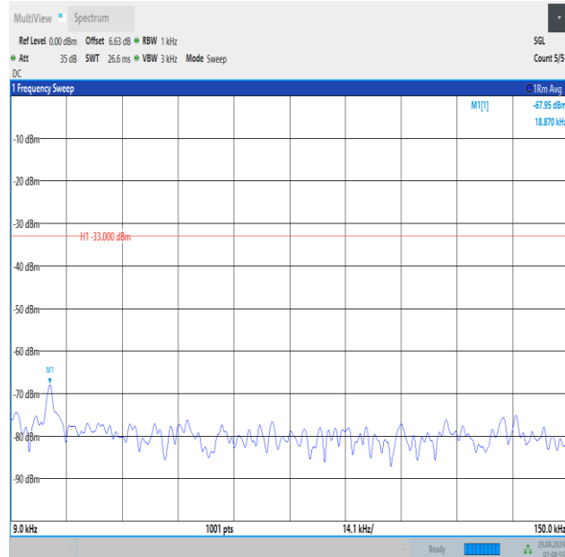
Band5_1.4MHz_QPSK_20643_1RB#5_0.009~0.15_0.009~0.15
