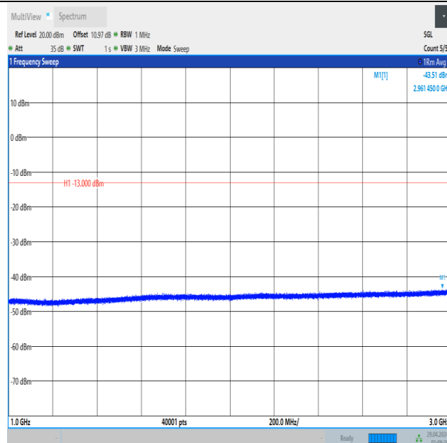
Band5_1.4MHz_16QAM_20643_1RB#0_1000~3000_1000~3000
