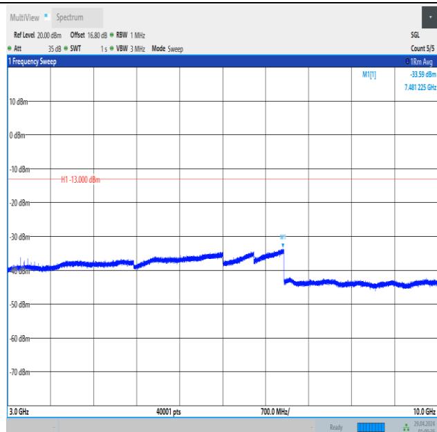
Band5_1.4MHz_QPSK_20643_1RB#5_3000~10000_3000~10000
