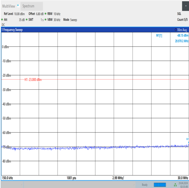
Band5_10MHz_16QAM_20450_1RB#0_0.15~30_0.15~30
