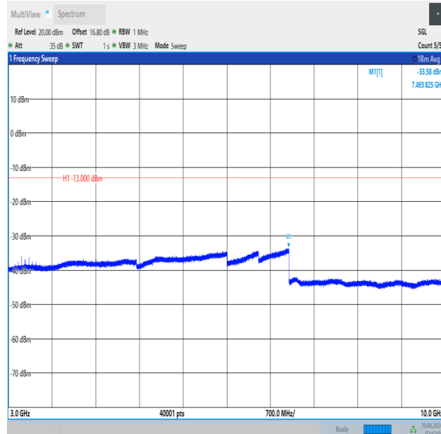
Band5_10MHz_QPSK_20600_1RB#0_3000~10000_3000~10000
