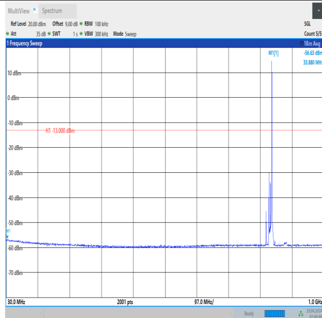
Band5_10MHz_16QAM_20525_1RB#49_30~1000_30~1000
