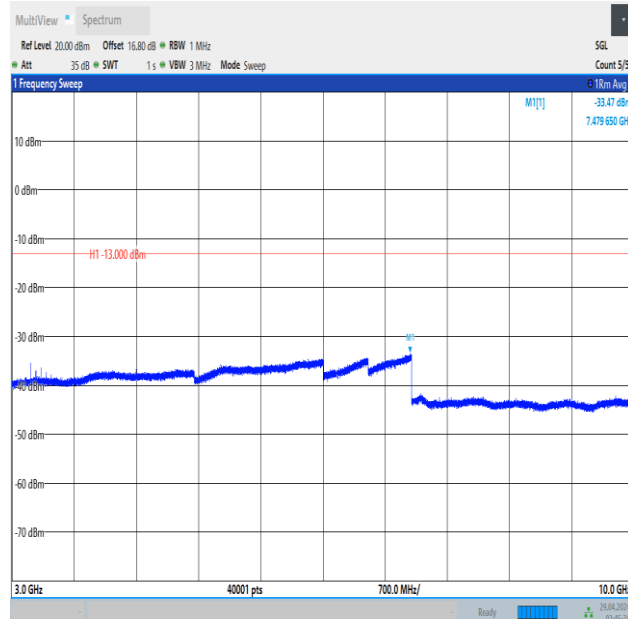
Band5_3MHz_QPSK_20415_1RB#0_3000~10000_3000~10000
