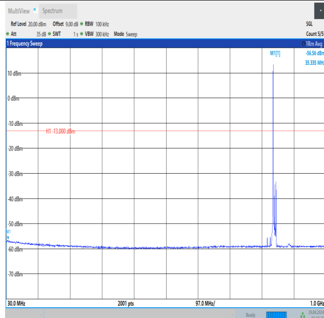
Band5_10MHz_16QAM_20600_1RB#0_30~1000_30~1000
