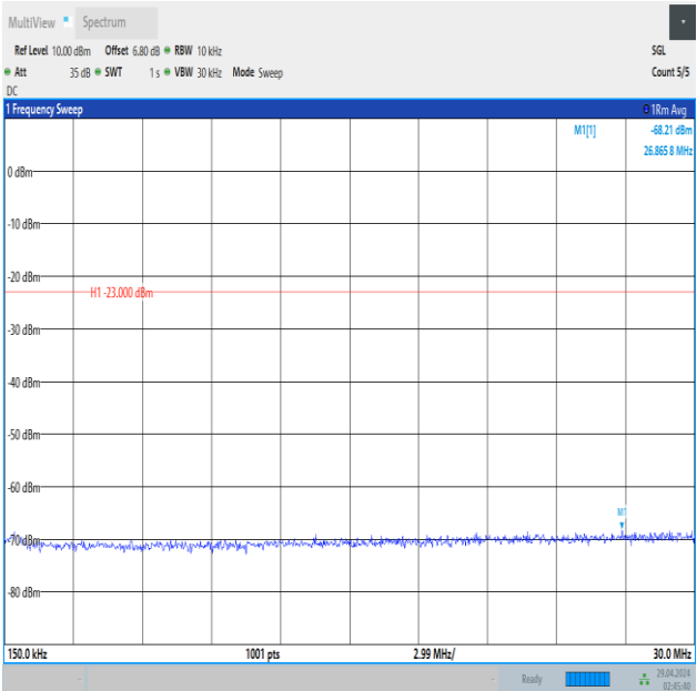
Band5_3MHz_16QAM_20415_1RB#0_0.15~30_0.15~30
