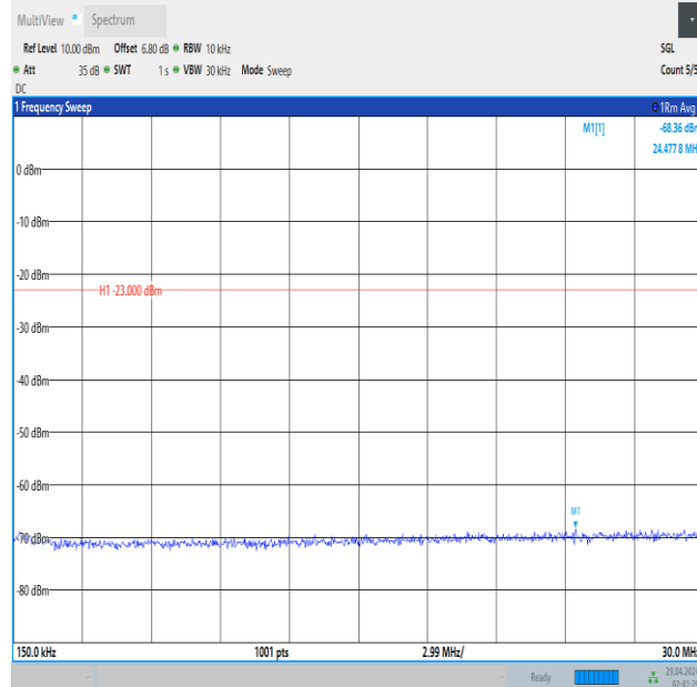
Band5_10MHz_QPSK_20600_1RB#0_0.15~30_0.15~30
