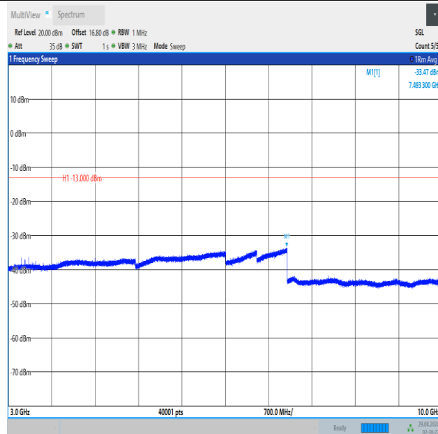
Band5_10MHz_16QAM_20450_1RB#0_3000~10000_3000~10000
