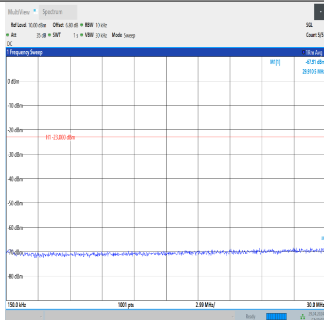
Band5_10MHz_16QAM_20525_1RB#0_0.15~30_0.15~30
