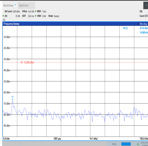
Band5_1.4MHz_16QAM_20643_1RB#0_0.009~0.15_0.009~0.15
