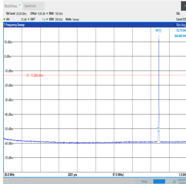
Band5_1.4MHz_QPSK_20643_1RB#0_30~1000_30~1000
