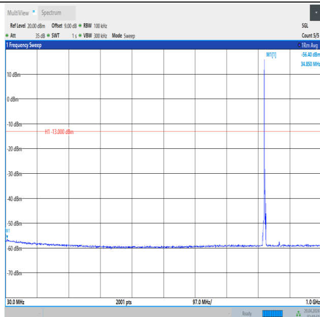
Band5_3MHz_QPSK_20415_1RB#0_30~1000_30~1000
