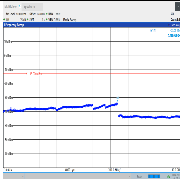
Band5_1.4MHz_16QAM_20643_6RB#0_3000~10000_3000~10000
