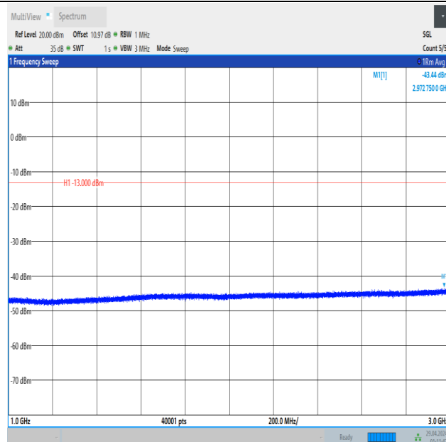
Band5_1.4MHz_16QAM_20643_6RB#0_1000~3000_1000~3000
