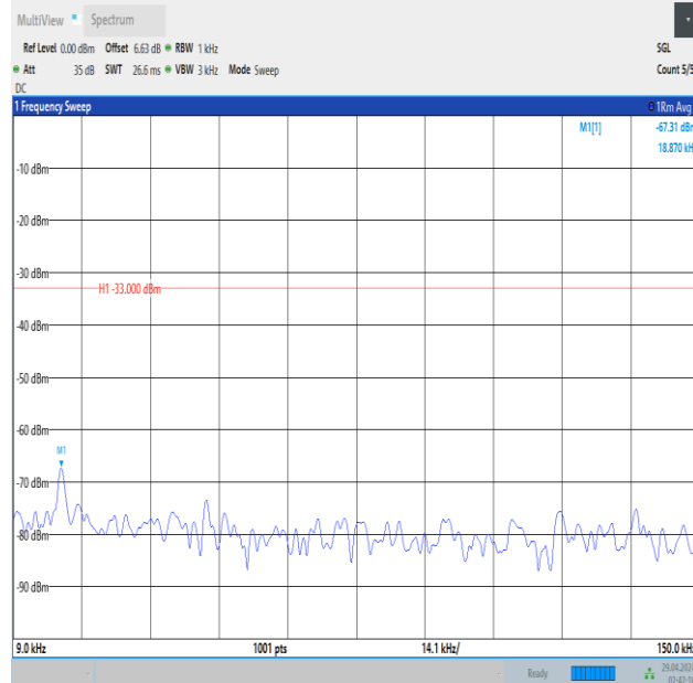
Band5_10MHz_16QAM_20600_1RB#0_0.009~0.15_0.009~0.15
