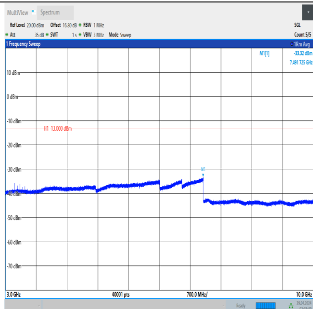
Band5_10MHz_QPSK_20525_1RB#0_3000~10000_3000~10000
