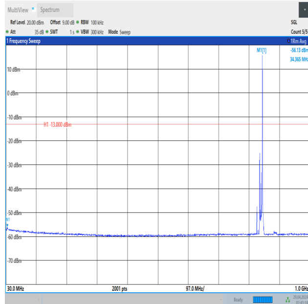
Band5_10MHz_QPSK_20600_1RB#49_30~1000_30~1000
