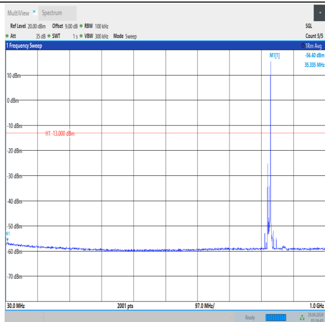
Band5_10MHz_QPSK_20450_1RB#49_30~1000_30~1000
