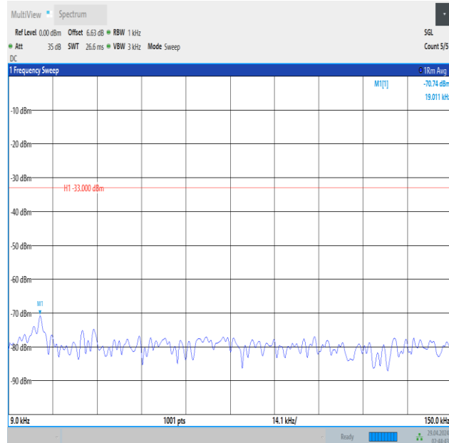
Band5_3MHz_QPSK_20415_1RB#0_0.009~0.15_0.009~0.15
