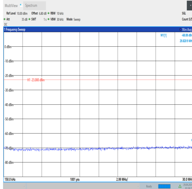
Band5_10MHz_QPSK_20525_1RB#0_0.15~30_0.15~30
