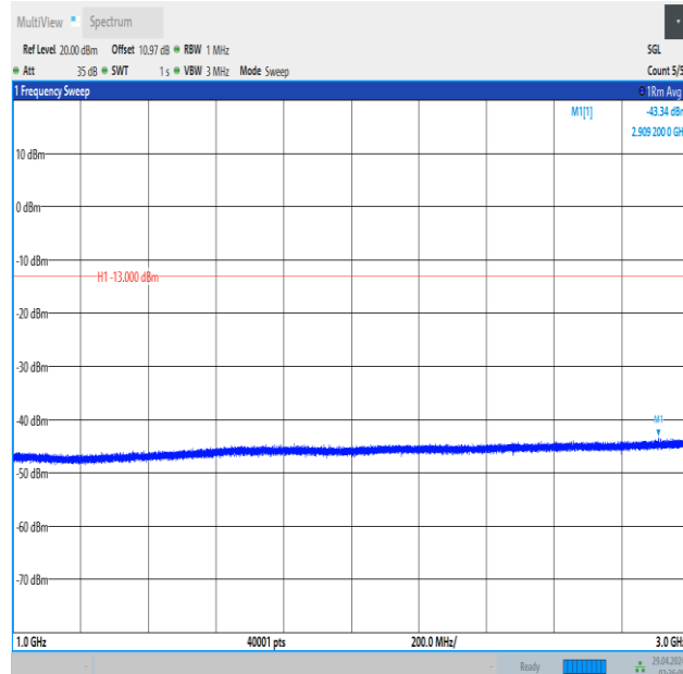
Band5_10MHz_16QAM_20450_1RB#0_1000~3000_1000~3000
