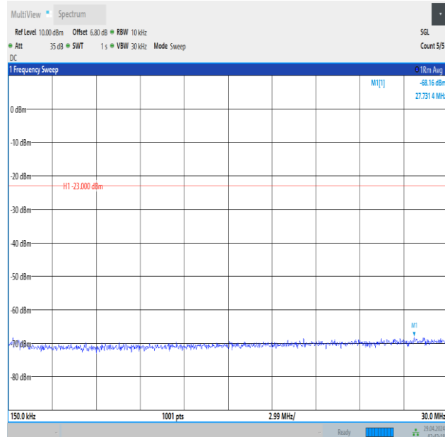
Band5_10MHz_16QAM_20600_1RB#0_0.15~30_0.15~30
