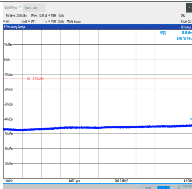
Band5_10MHz_16QAM_20450_1RB#49_1000~3000_1000~3000
