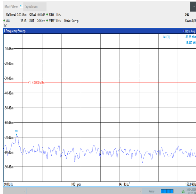
Band5_10MHz_16QAM_20450_1RB#0_0.009~0.15_0.009~0.15
