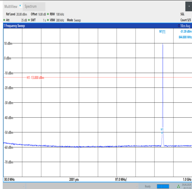
Band5_1.4MHz_16QAM_20643_6RB#0_30~1000_30~1000
