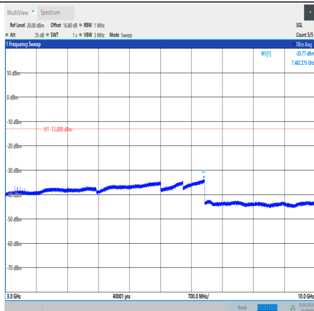
Band5_1.4MHz_QPSK_20643_1RB#0_3000~10000_3000~10000
