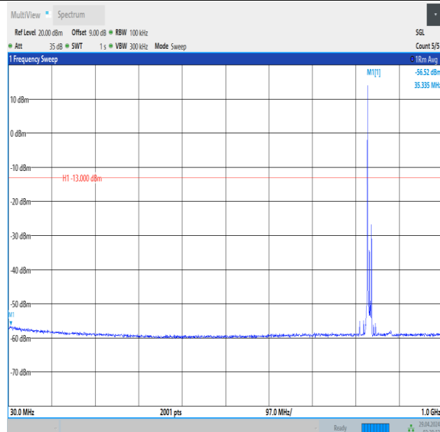
Band5_10MHz_16QAM_20525_1RB#0_30~1000_30~1000
