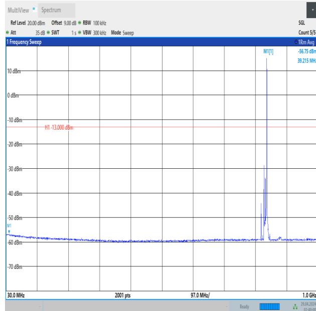
Band5_10MHz_QPSK_20525_1RB#49_30~1000_30~1000
