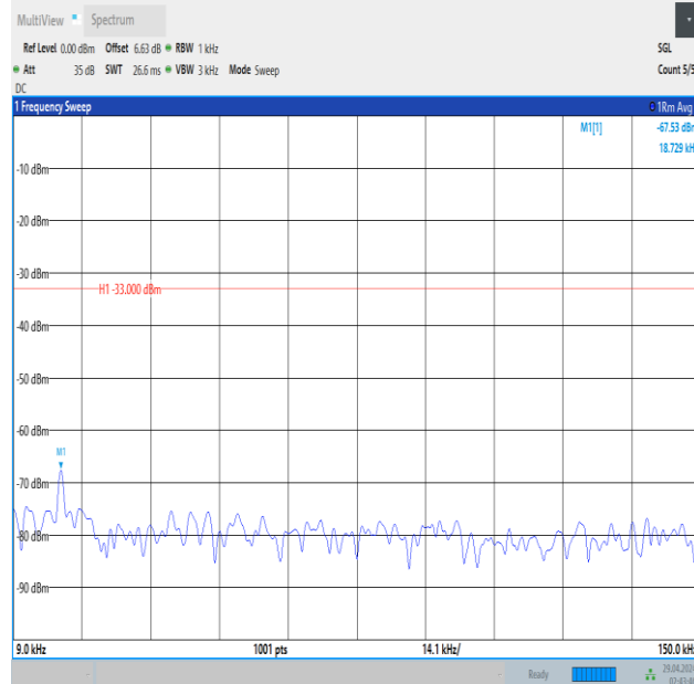
Band5_10MHz_16QAM_20600_1RB#49_0.009~0.15_0.009~0.15
