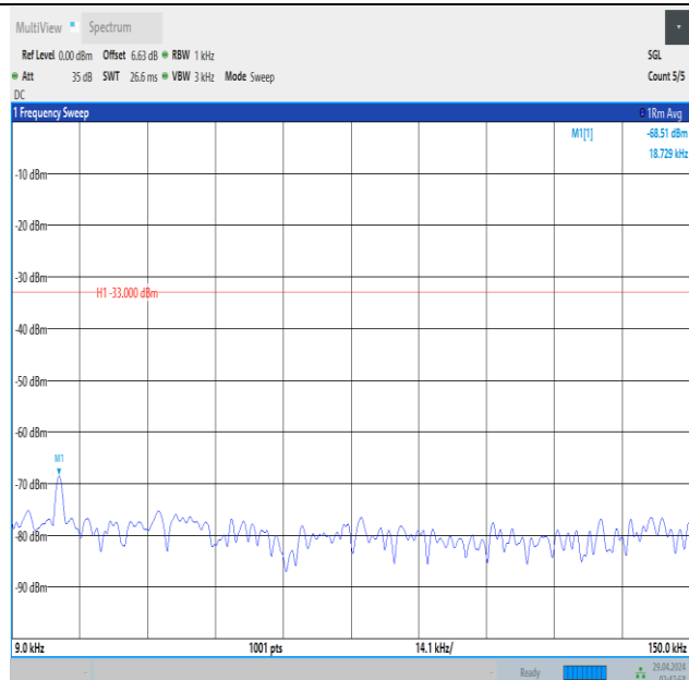
Band5_3MHz_QPSK_20415_15RB#0_0.009~0.15_0.009~0.15
