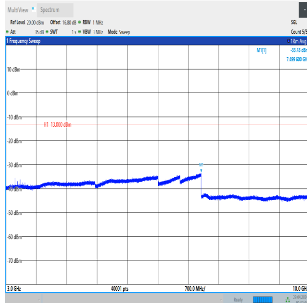
Band5_3MHz_QPSK_20525_1RB#14_3000~10000_3000~10000
