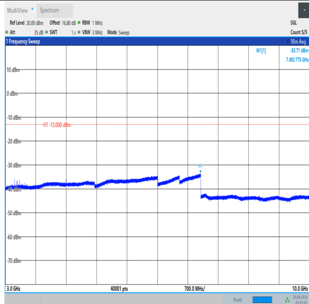
Band5_10MHz_QPSK_20525_50RB#0_3000~10000_3000~10000
