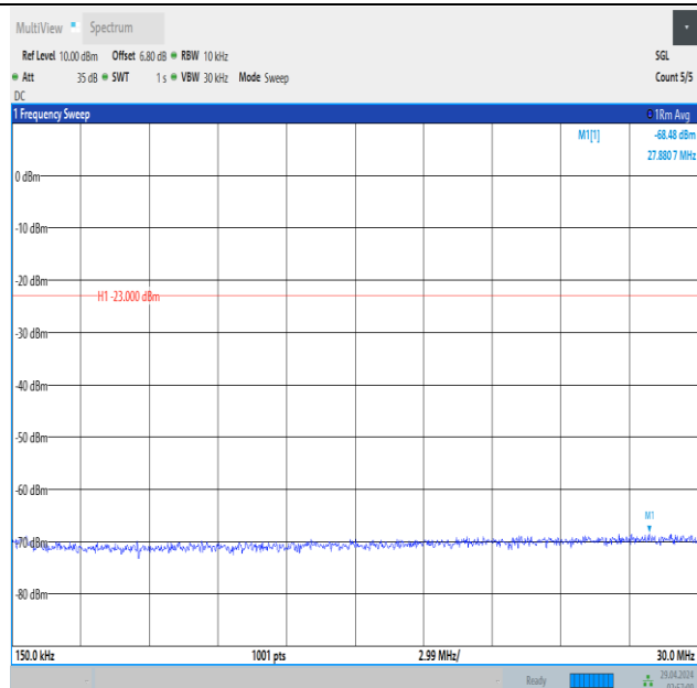
Band5_3MHz_16QAM_20635_1RB#14_0.15~30_0.15~30
