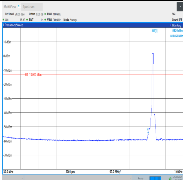
Band5_10MHz_QPSK_20525_50RB#0_30~1000_30~1000
