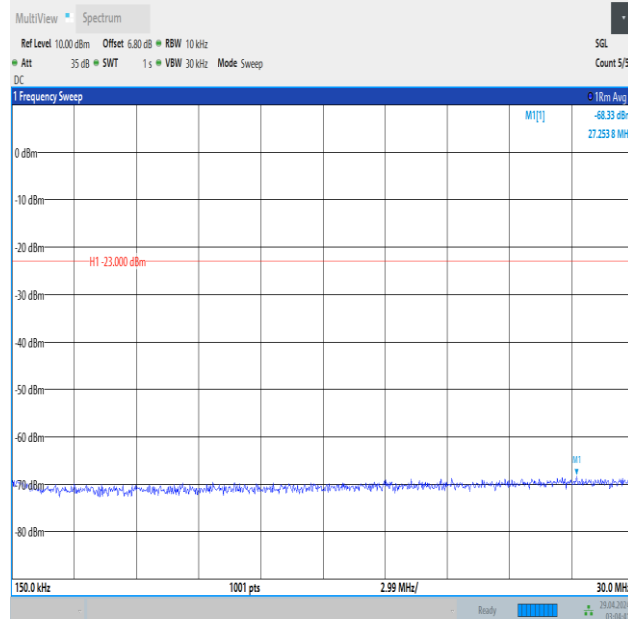
Band5_5MHz_16QAM_20425_1RB#0_0.15~30_0.15~30
