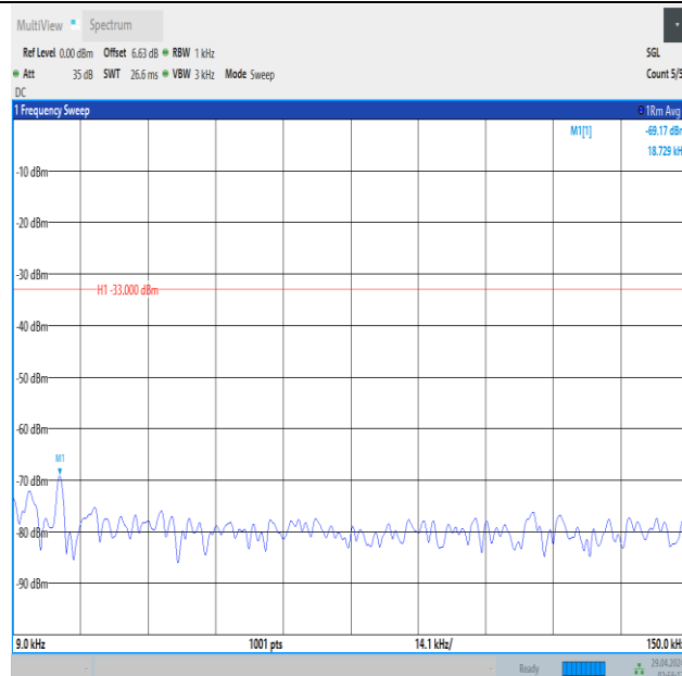
Band5_3MHz_QPSK_20635_1RB#14_0.009~0.15_0.009~0.15
