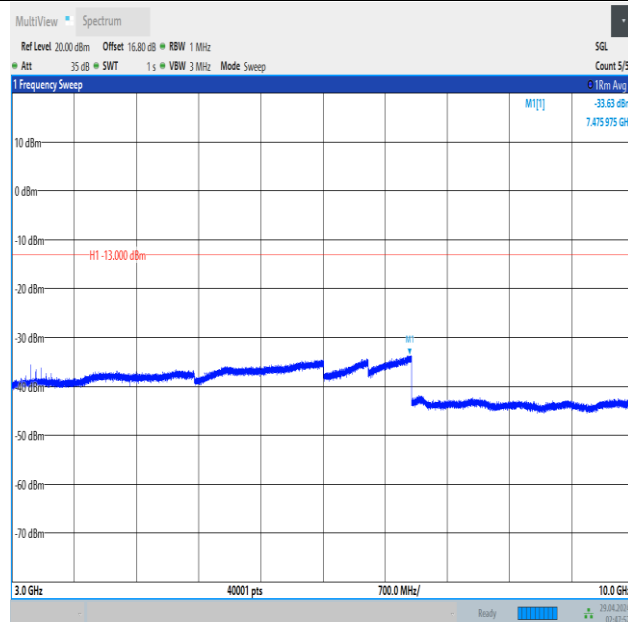
Band5_3MHz_16QAM_20415_1RB#14_3000~10000_3000~10000
