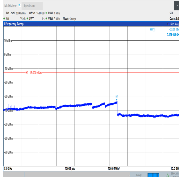
Band5_3MHz_QPSK_20415_1RB#14_3000~10000_3000~10000
