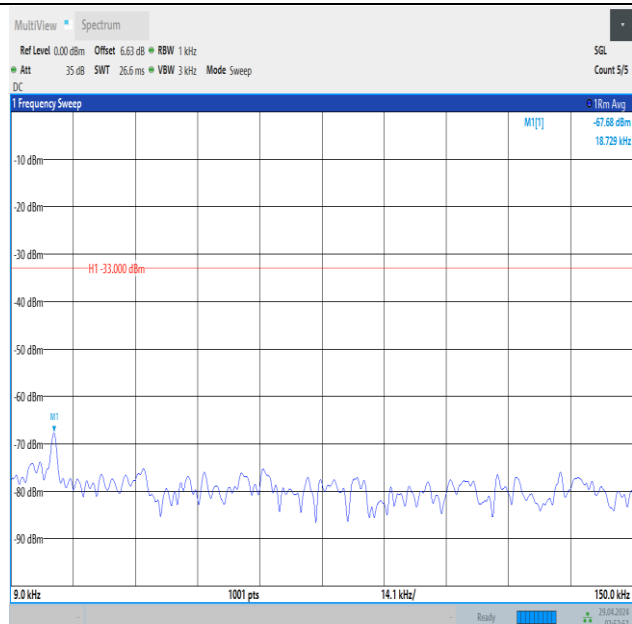
Band5_3MHz_QPSK_20525_15RB#0_0.009~0.15_0.009~0.15
