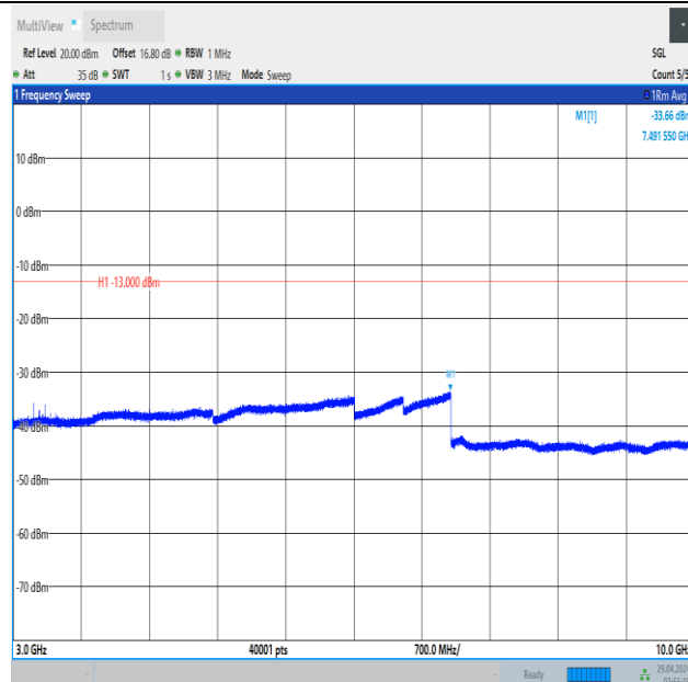
Band5_3MHz_QPSK_20635_1RB#0_3000~10000_3000~10000
