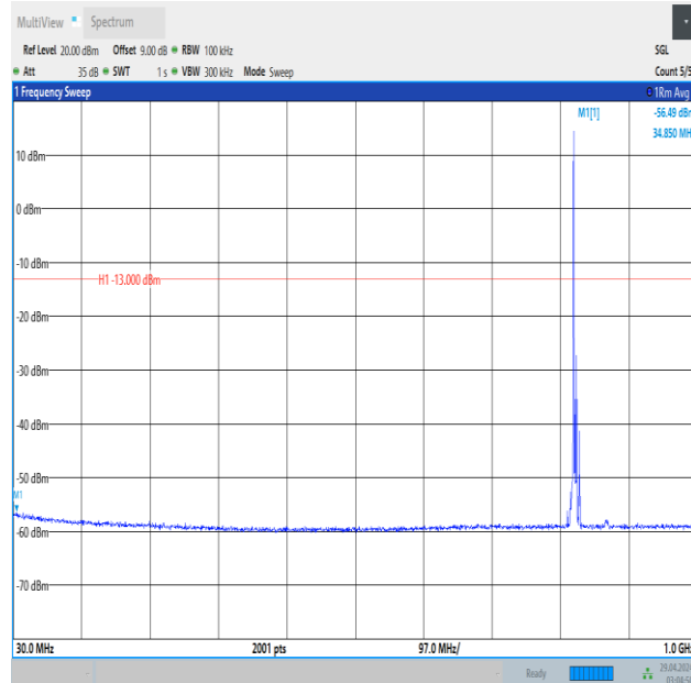
Band5_5MHz_16QAM_20425_1RB#0_30~1000_30~1000
