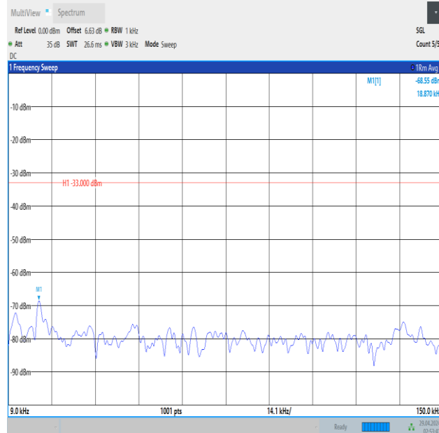
Band5_3MHz_16QAM_20525_15RB#0_0.009~0.15_0.009~0.15
