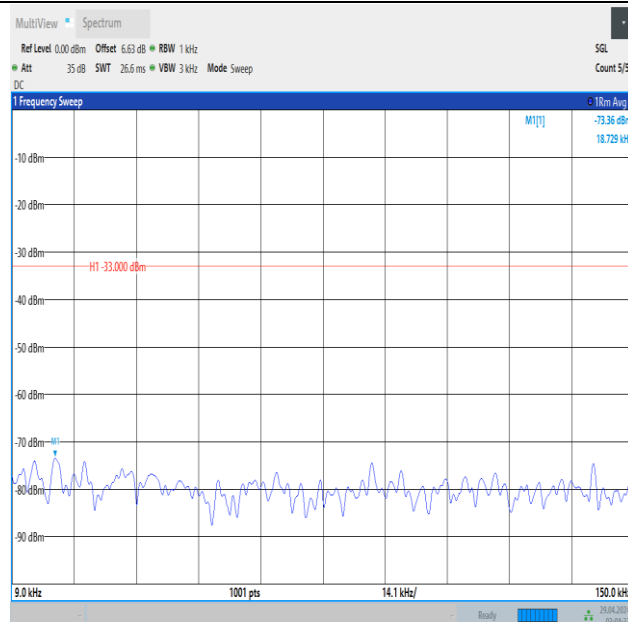
Band5_5MHz_16QAM_20425_1RB#0_0.009~0.15_0.009~0.15
