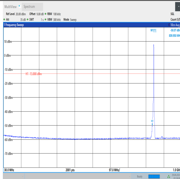
Band5_3MHz_QPSK_20635_15RB#0_30~1000_30~1000
