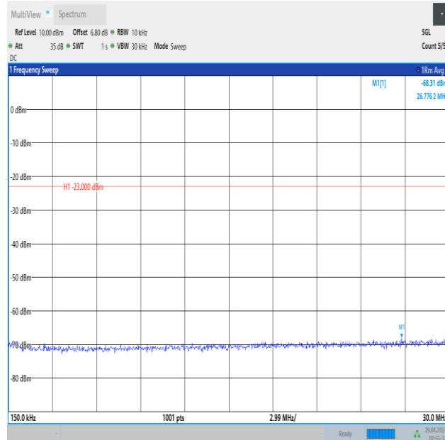
Band5_3MHz_16QAM_20635_1RB#0_0.15~30_0.15~30
