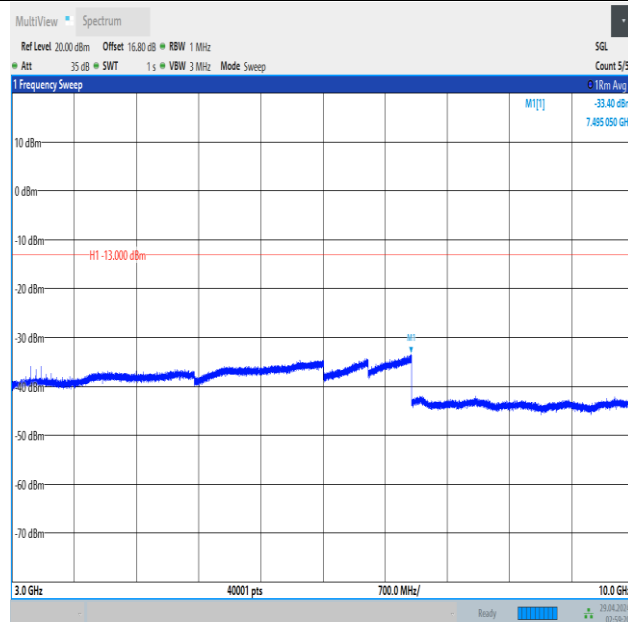
Band5_3MHz_16QAM_20635_15RB#0_3000~10000_3000~10000
