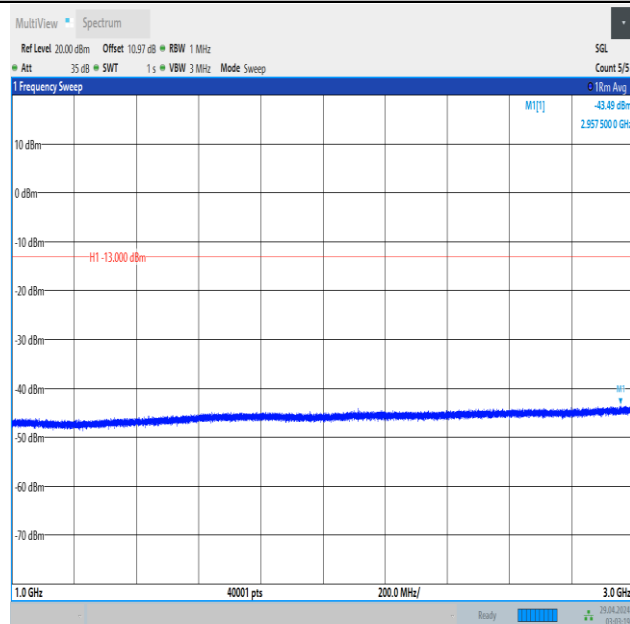
Band5_10MHz_QPSK_20600_50RB#0_1000~3000_1000~3000
