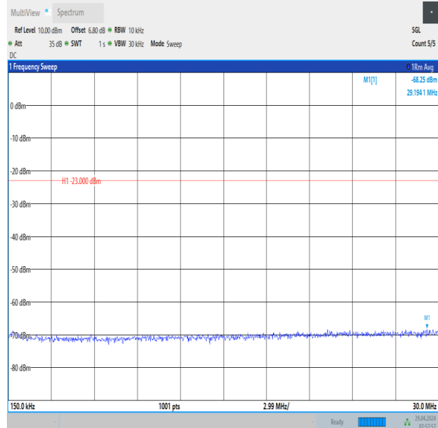
Band5_3MHz_QPSK_20635_15RB#0_0.15~30_0.15~30
