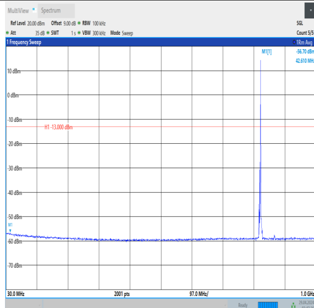
Band5_3MHz_16QAM_20415_1RB#14_30~1000_30~1000
