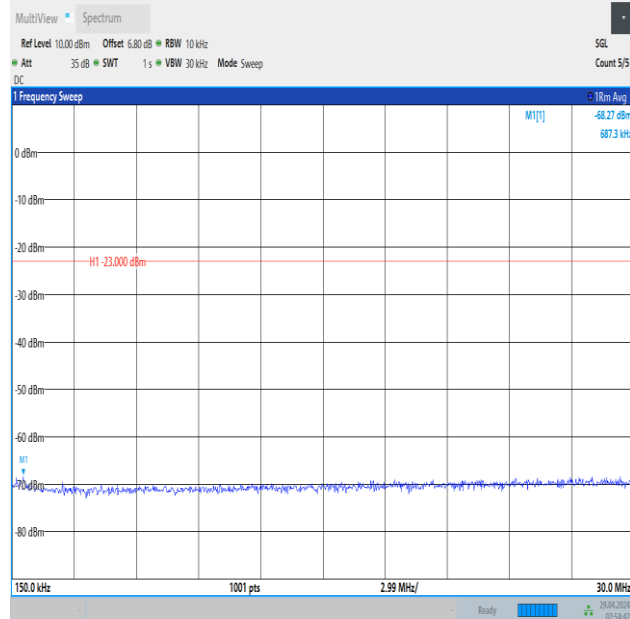
Band5_3MHz_QPSK_20635_1RB#0_0.15~30_0.15~30
