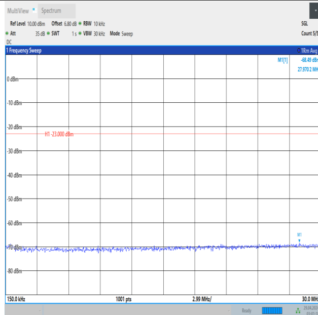
Band5_10MHz_QPSK_20450_50RB#0_0.15~30_0.15~30
