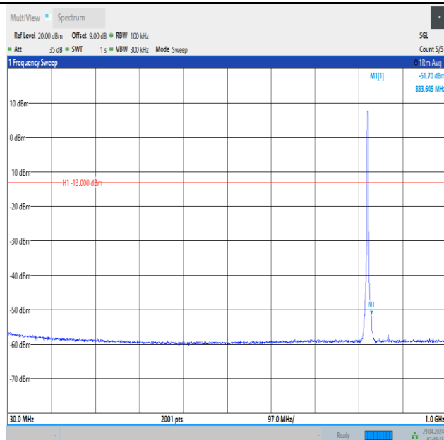
Band5_3MHz_QPSK_20415_15RB#0_30~1000_30~1000
