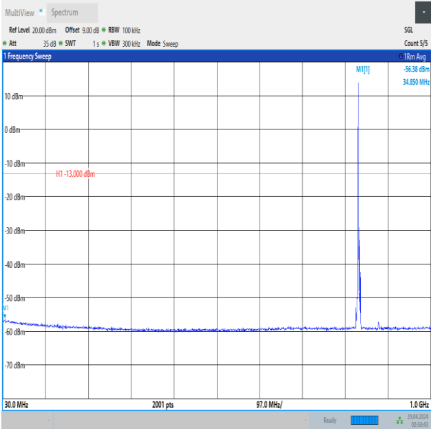
Band5_3MHz_16QAM_20525_1RB#0_30~1000_30~1000
