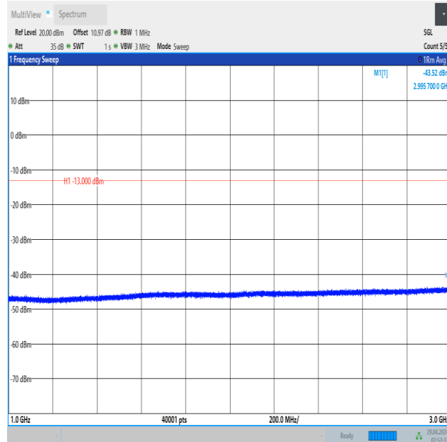
Band5_3MHz_16QAM_20525_1RB#14_1000~3000_1000~3000
