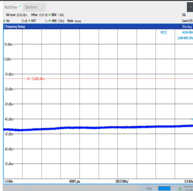
Band5_3MHz_QPSK_20525_1RB#0_1000~3000_1000~3000
