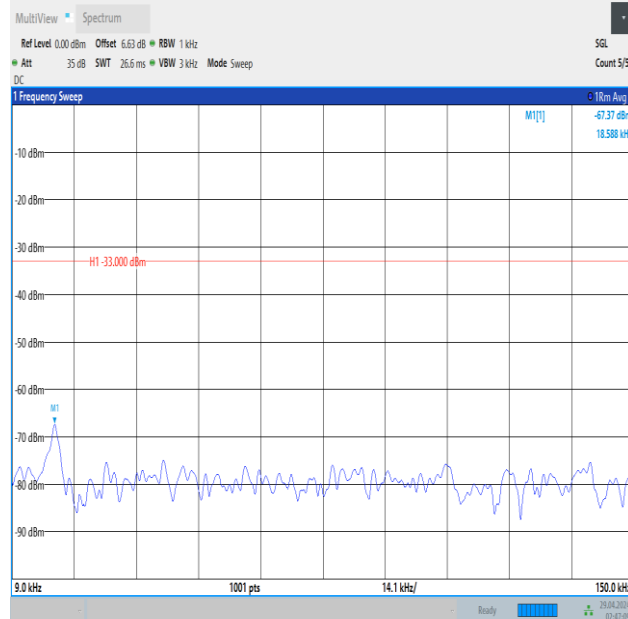
Band5_3MHz_16QAM_20415_1RB#14_0.009~0.15_0.009~0.15
