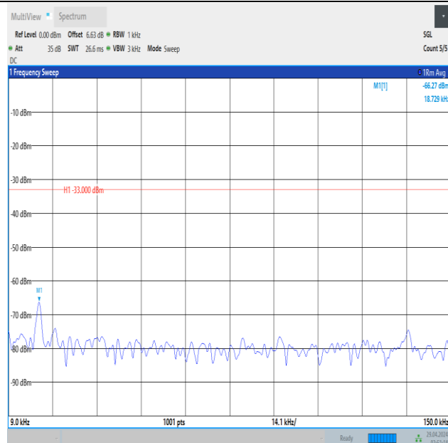
Band5_3MHz_QPSK_20525_1RB#14_0.009~0.15_0.009~0.15
