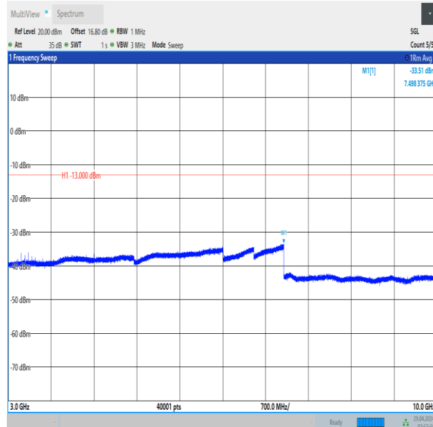
Band5_3MHz_QPSK_20525_15RB#0_3000~10000_3000~10000
