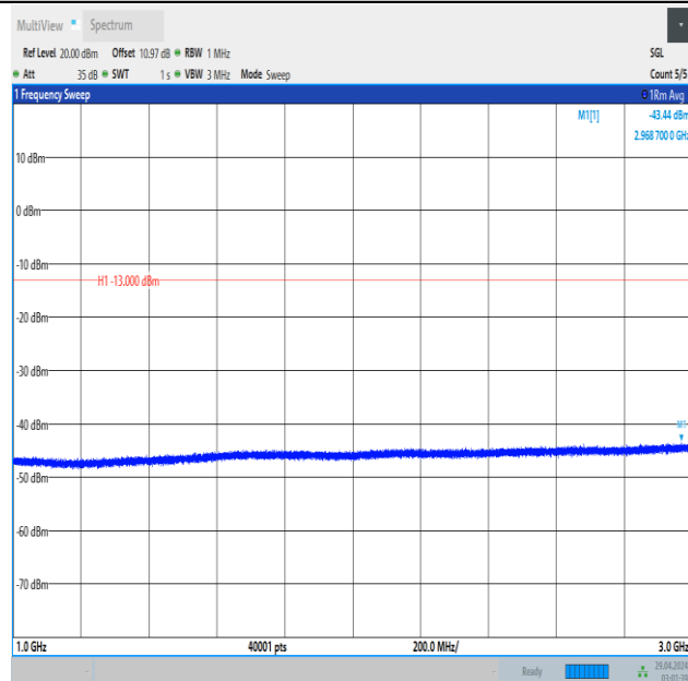
Band5_10MHz_QPSK_20450_50RB#0_1000~3000_1000~3000
