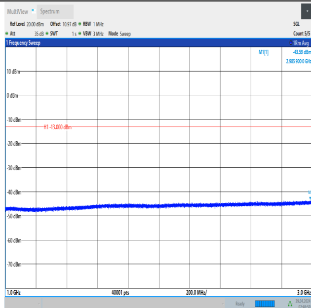
Band5_3MHz_QPSK_20415_1RB#14_1000~3000_1000~3000
