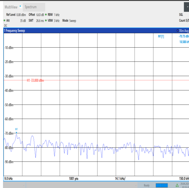
Band5_3MHz_16QAM_20635_1RB#0_0.009~0.15_0.009~0.15
