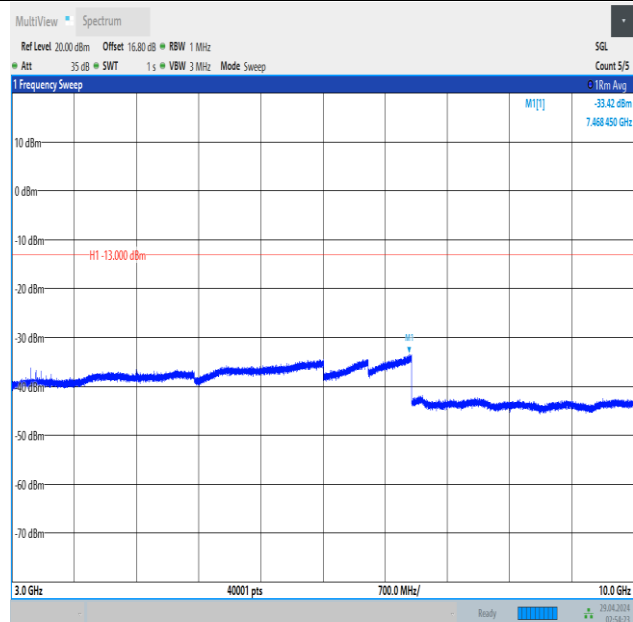
Band5_3MHz_16QAM_20525_15RB#0_3000~10000_3000~10000
