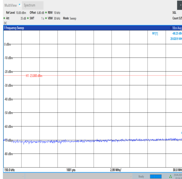
Band5_3MHz_QPSK_20635_1RB#14_0.15~30_0.15~30
