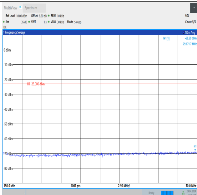
Band5_10MHz_QPSK_20525_50RB#0_0.15~30_0.15~30
