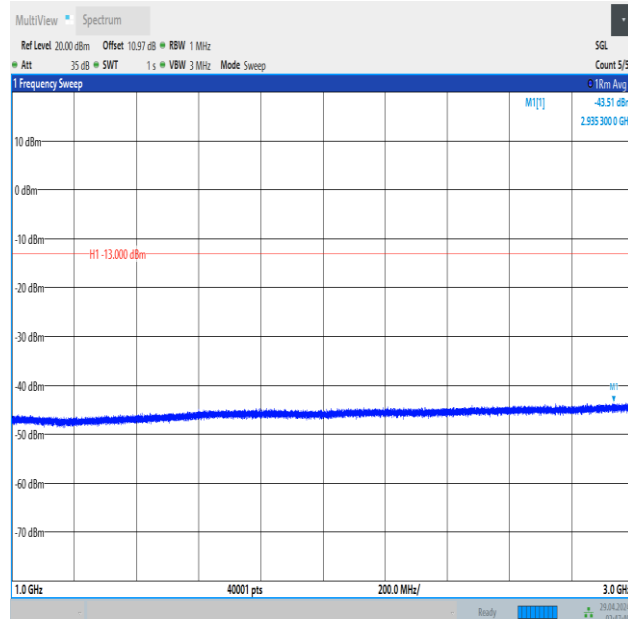
Band5_3MHz_16QAM_20415_1RB#14_1000~3000_1000~3000
