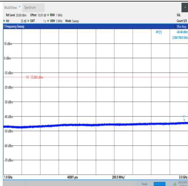
Band5_5MHz_QPSK_20425_1RB#0_1000~3000_1000~3000
