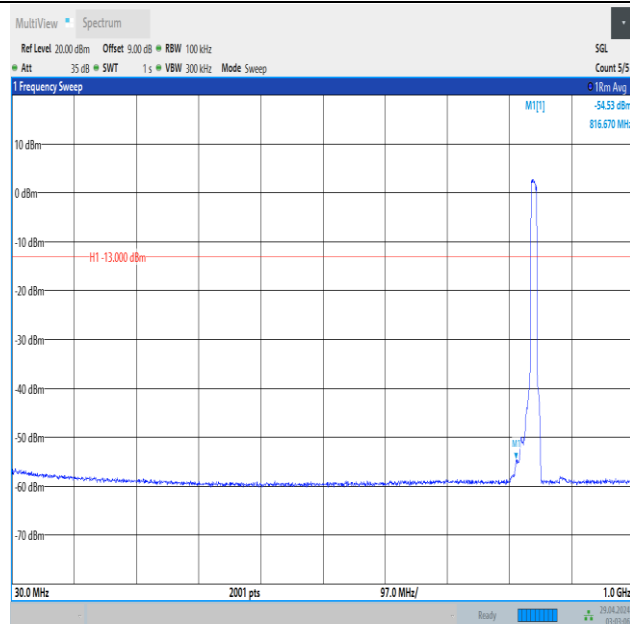
Band5_10MHz_QPSK_20600_50RB#0_30~1000_30~1000
