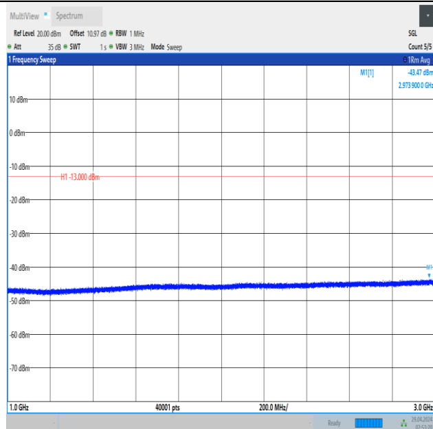
Band5_3MHz_QPSK_20525_15RB#0_1000~3000_1000~3000
