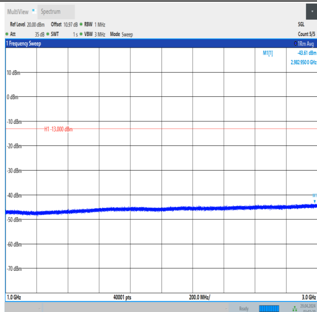
Band5_10MHz_QPSK_20525_50RB#0_1000~3000_1000~3000
