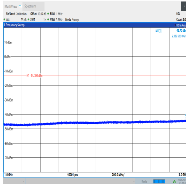
Band5_5MHz_16QAM_20425_1RB#0_1000~3000_1000~3000
