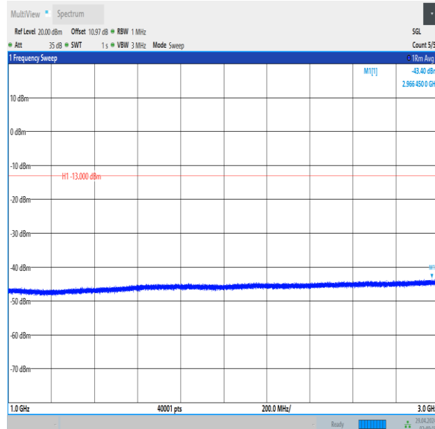
Band5_3MHz_16QAM_20415_15RB#0_1000~3000_1000~3000
