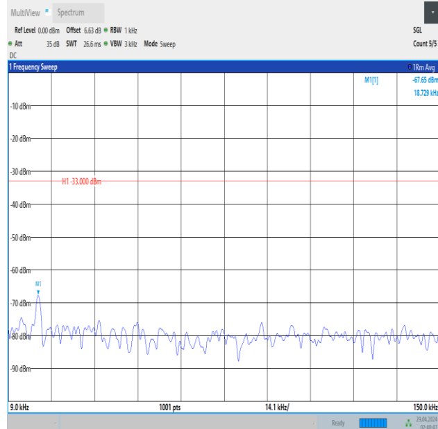
Band5_3MHz_16QAM_20415_15RB#0_0.009~0.15_0.009~0.15
