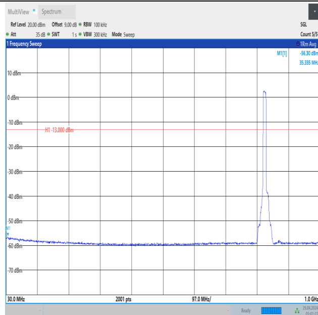
Band5_10MHz_QPSK_20450_50RB#0_30~1000_30~1000
