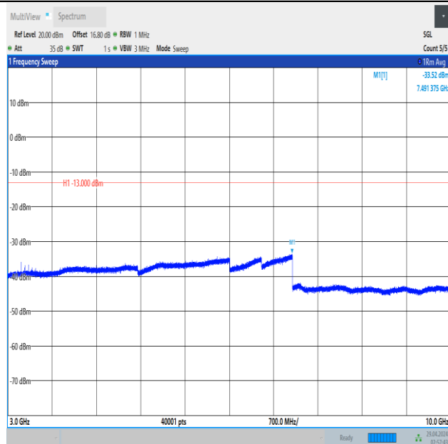
Band5_3MHz_16QAM_20635_1RB#14_3000~10000_3000~10000
