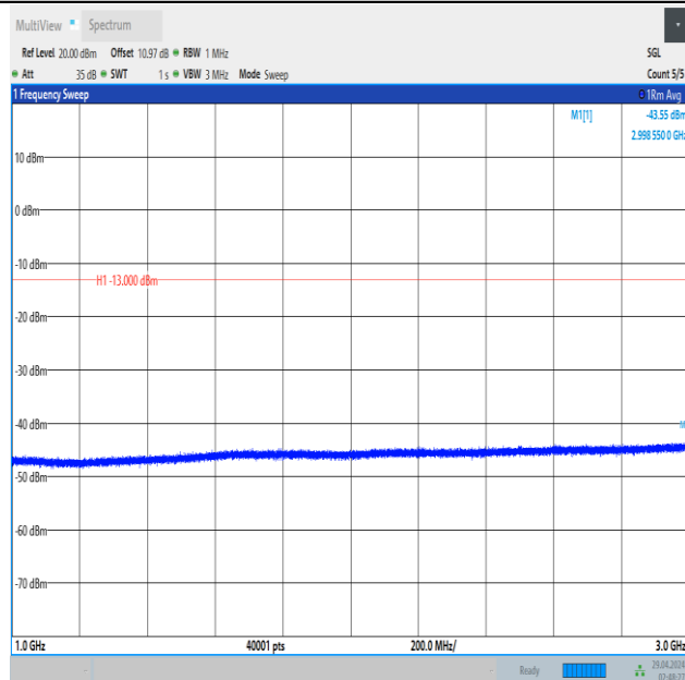
Band5_3MHz_QPSK_20415_15RB#0_1000~3000_1000~3000
