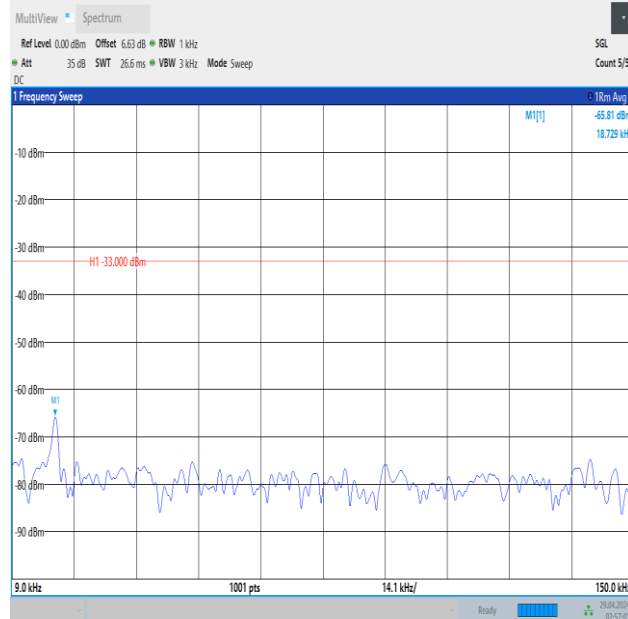
Band5_3MHz_16QAM_20635_1RB#14_0.009~0.15_0.009~0.15
