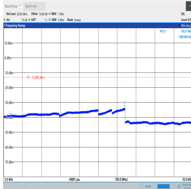
Band5_3MHz_QPSK_20635_1RB#14_3000~10000_3000~10000
