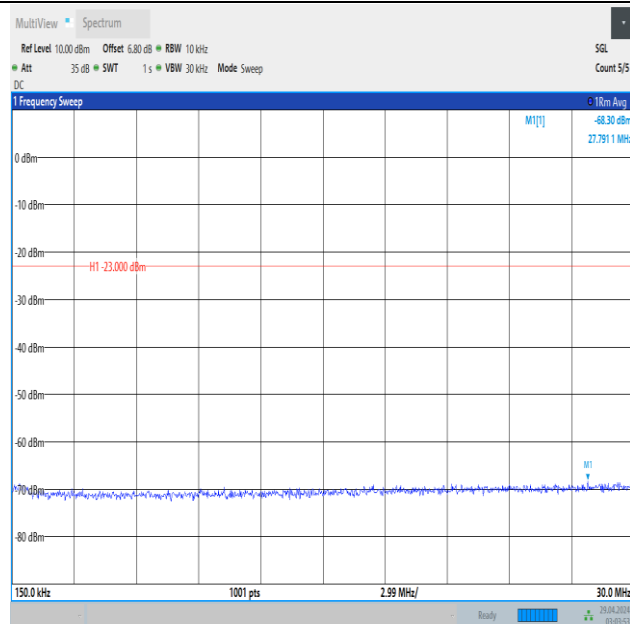
Band5_5MHz_QPSK_20425_1RB#0_0.15~30_0.15~30
