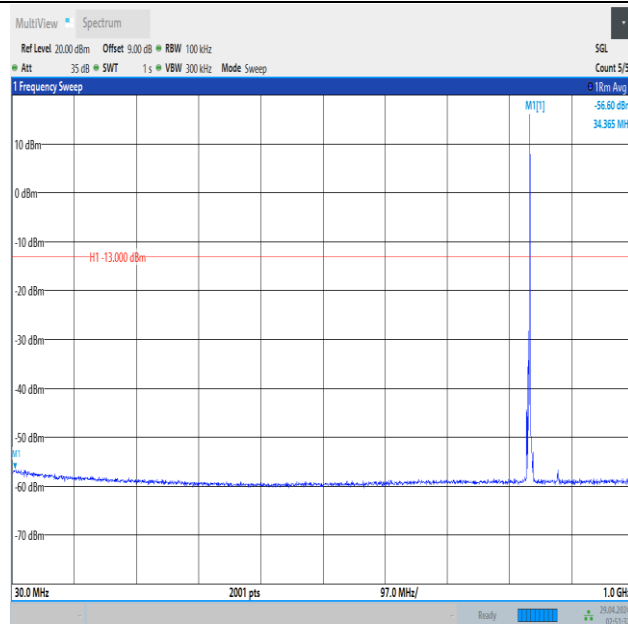
Band5_3MHz_QPSK_20525_1RB#14_30~1000_30~1000
