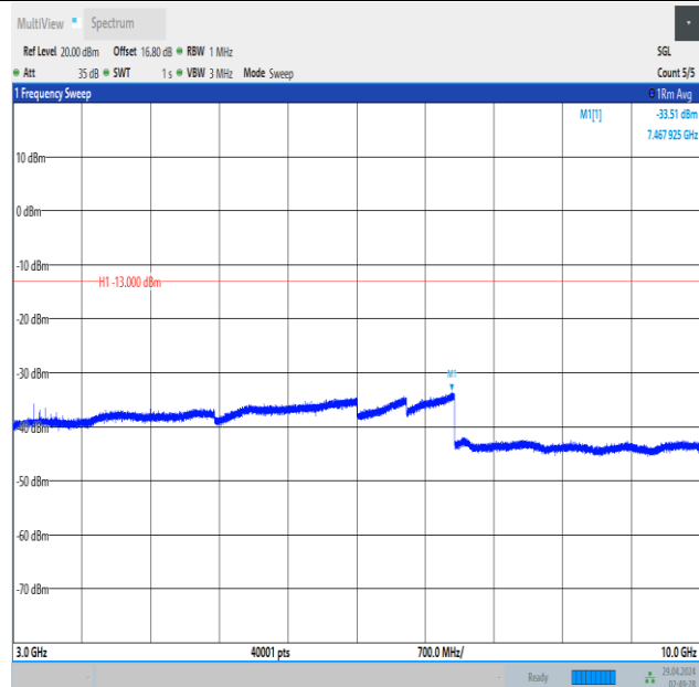
Band5_3MHz_16QAM_20415_15RB#0_3000~10000_3000~10000
