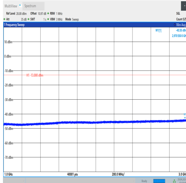
Band5_3MHz_16QAM_20635_15RB#0_1000~3000_1000~3000
