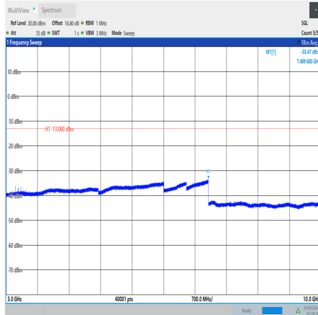
Band5_3MHz_QPSK_20635_15RB#0_3000~10000_3000~10000
