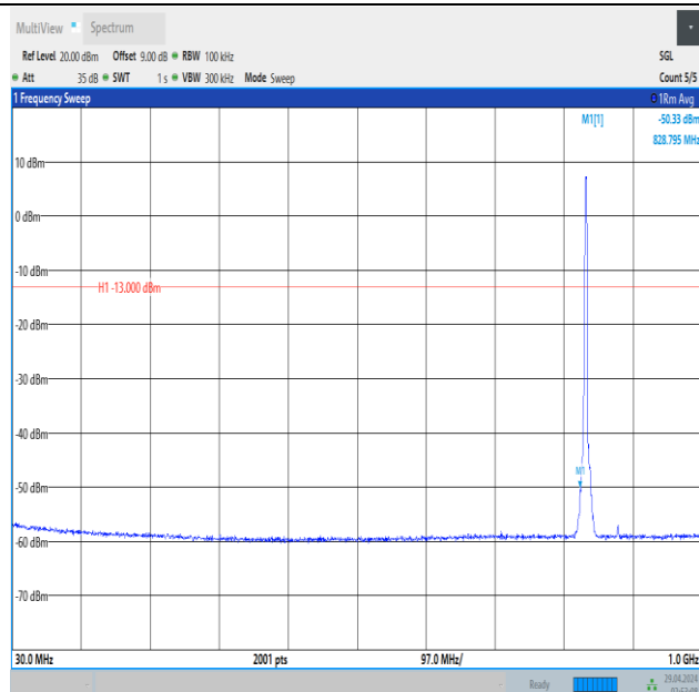
Band5_3MHz_QPSK_20525_15RB#0_30~1000_30~1000
