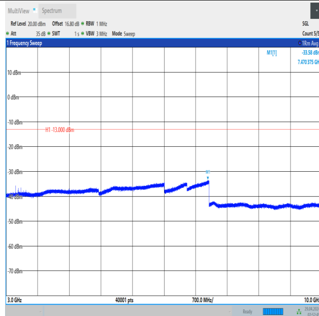
Band5_3MHz_16QAM_20525_1RB#14_3000~10000_3000~10000
