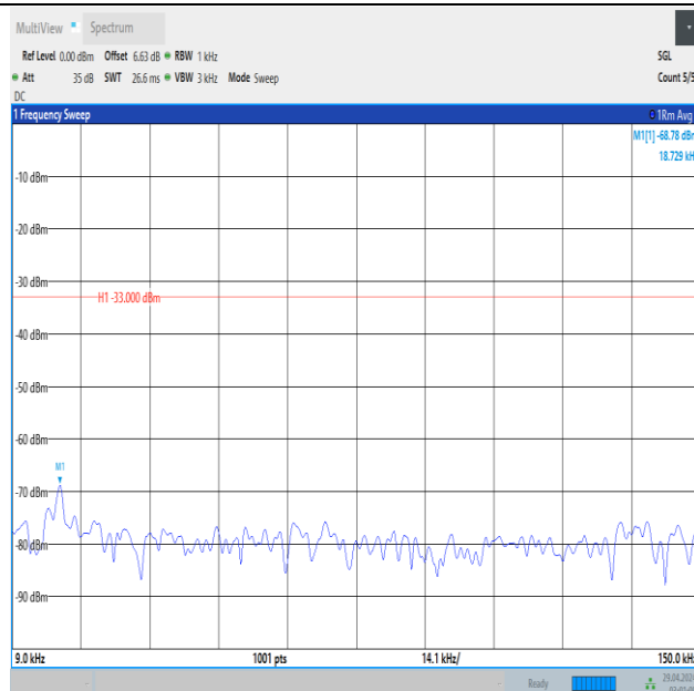
Band5_10MHz_QPSK_20450_50RB#0_0.009~0.15_0.009~0.15
