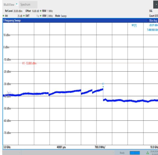
Band5_3MHz_16QAM_20635_1RB#0_3000~10000_3000~10000
