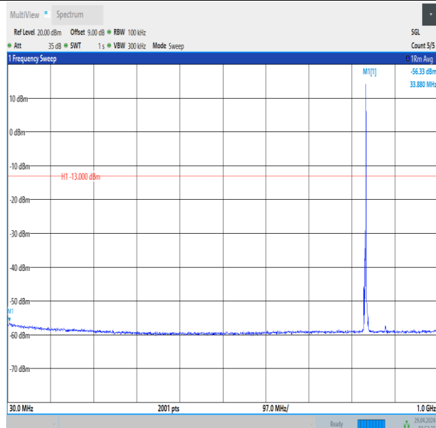
Band5_3MHz_16QAM_20525_1RB#14_30~1000_30~1000
