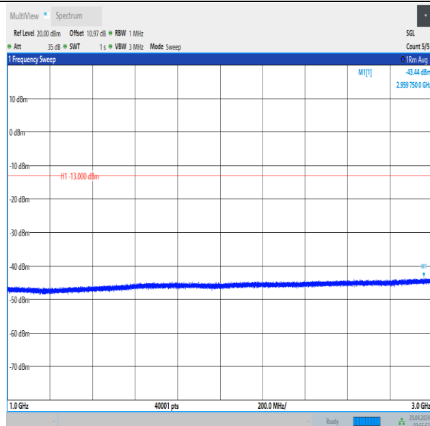
Band5_3MHz_16QAM_20635_1RB#0_1000~3000_1000~3000
