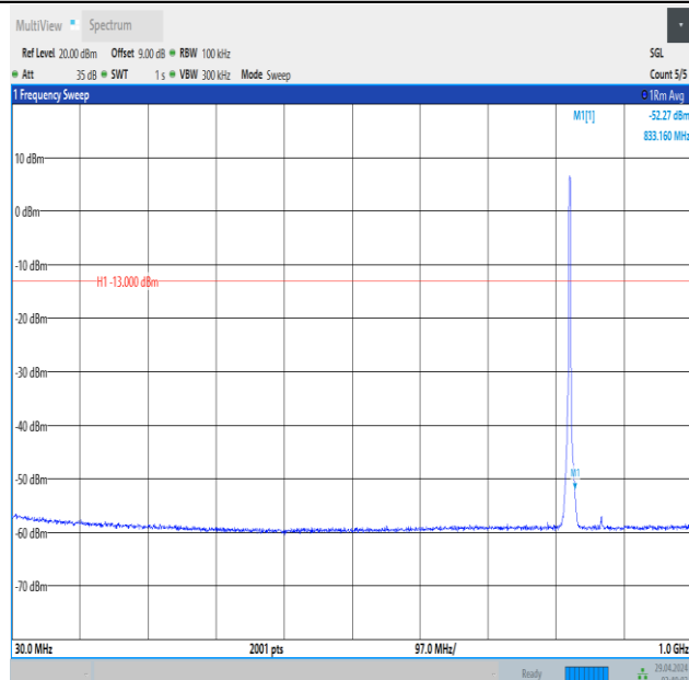
Band5_3MHz_16QAM_20415_15RB#0_30~1000_30~1000
