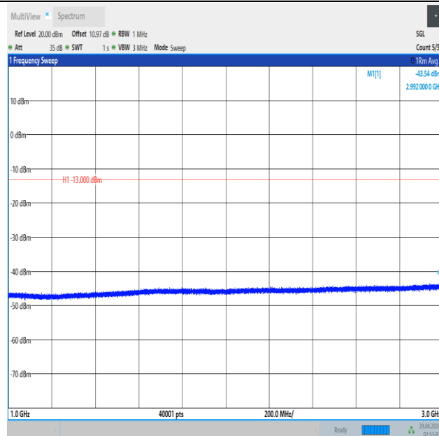
Band5_3MHz_QPSK_20635_1RB#0_1000~3000_1000~3000
