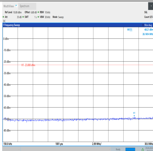
Band5_3MHz_16QAM_20525_1RB#14_0.15~30_0.15~30
