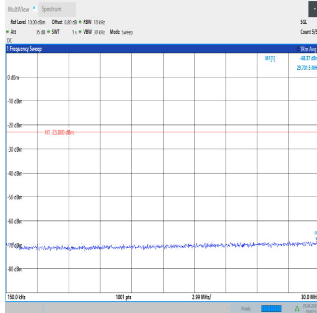
Band5_10MHz_QPSK_20600_50RB#0_0.15~30_0.15~30
