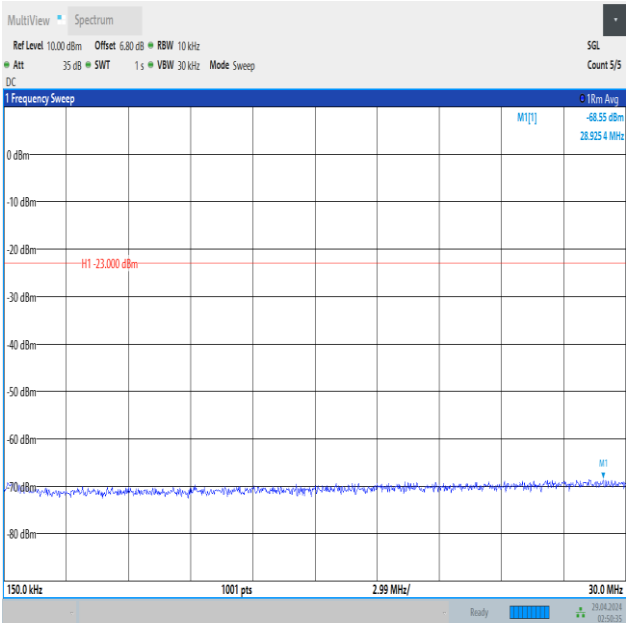
Band5_3MHz_16QAM_20525_1RB#0_0.15~30_0.15~30
