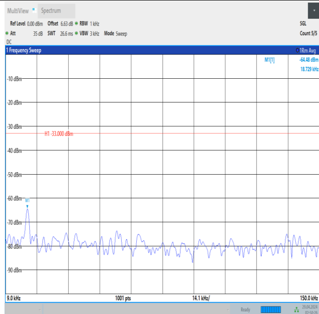
Band5_3MHz_16QAM_20525_1RB#0_0.009~0.15_0.009~0.15
