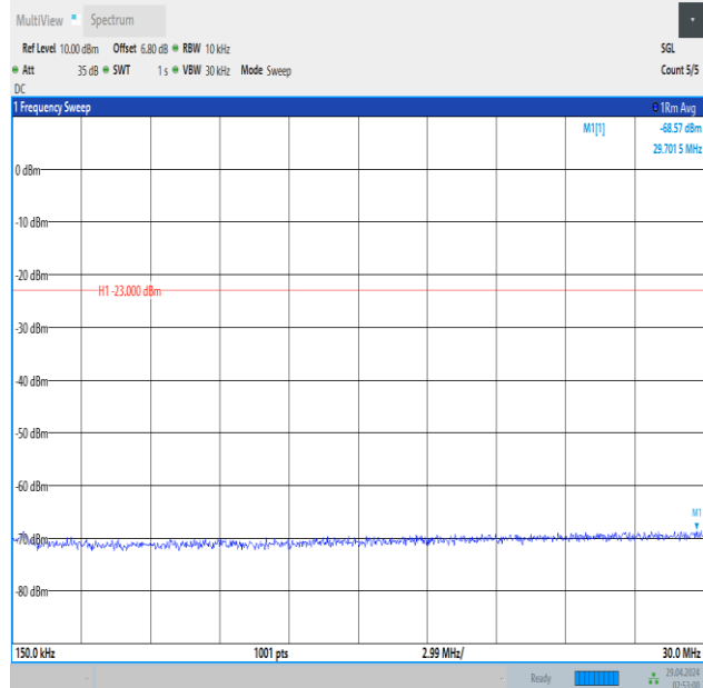
Band5_3MHz_QPSK_20525_15RB#0_0.15~30_0.15~30
