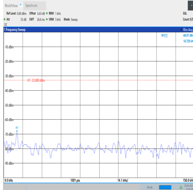
Band5_10MHz_QPSK_20525_50RB#0_0.009~0.15_0.009~0.15
