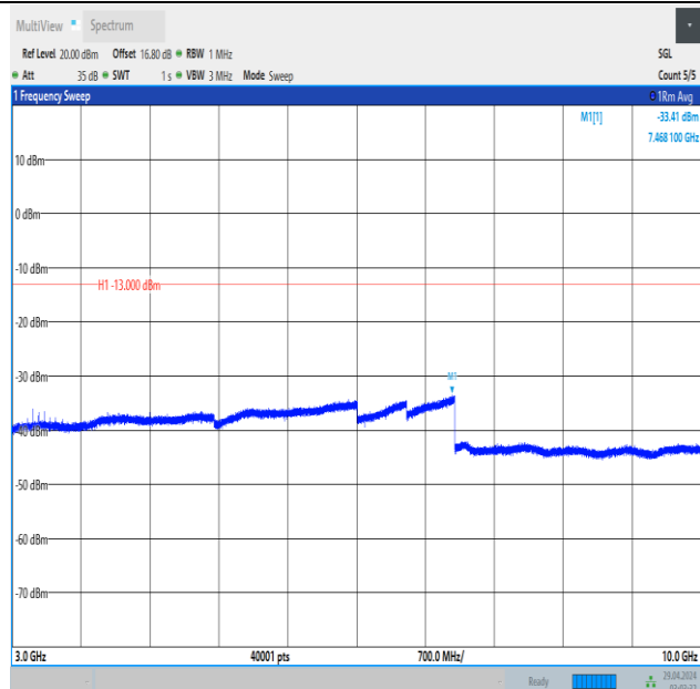
Band5_10MHz_QPSK_20600_50RB#0_3000~10000_3000~10000
