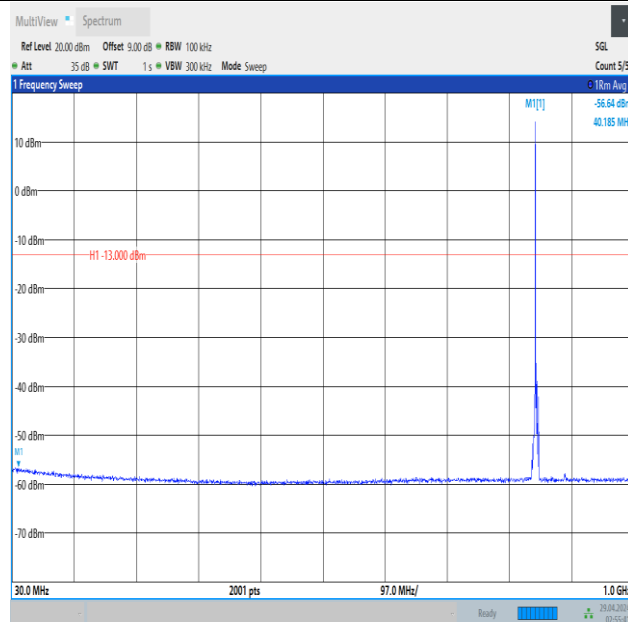
Band5_3MHz_16QAM_20635_1RB#0_30~1000_30~1000
