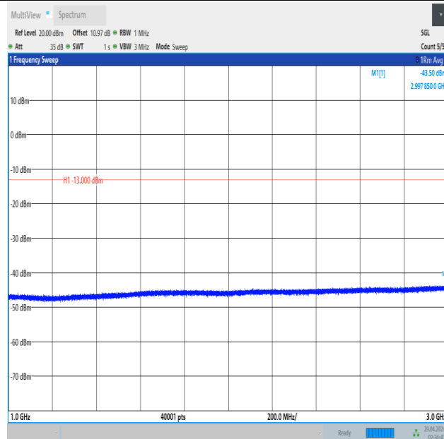
Band5_3MHz_QPSK_20635_1RB#14_1000~3000_1000~3000
