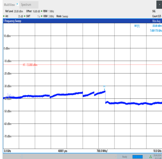
Band5_3MHz_16QAM_20525_1RB#0_3000~10000_3000~10000
