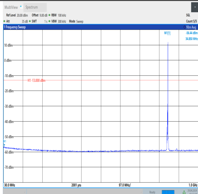
Band5_3MHz_16QAM_20635_1RB#14_30~1000_30~1000
