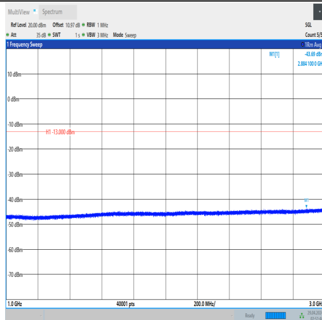
Band5_3MHz_QPSK_20525_1RB#14_1000~3000_1000~3000
