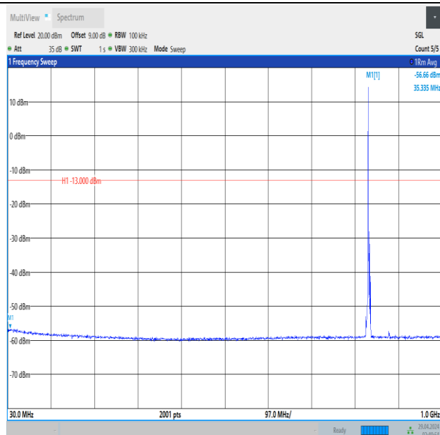
Band5_3MHz_QPSK_20525_1RB#0_30~1000_30~1000
