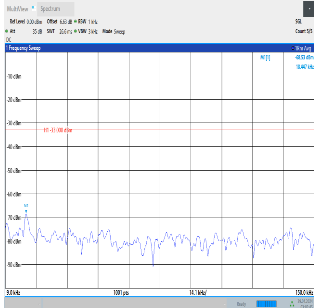
Band5_5MHz_QPSK_20425_1RB#0_0.009~0.15_0.009~0.15
