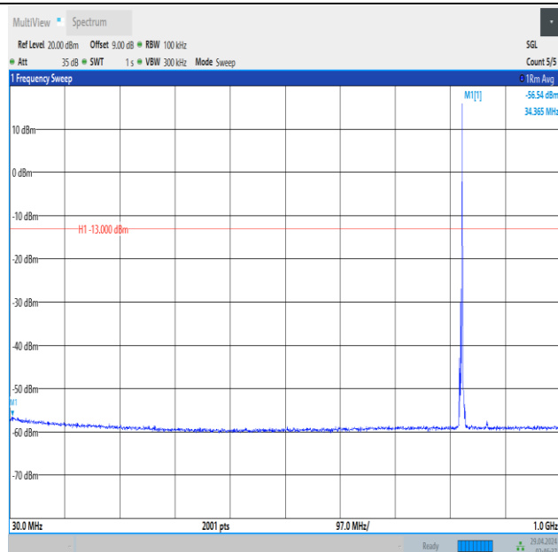
Band5_3MHz_QPSK_20415_1RB#14_30~1000_30~1000
