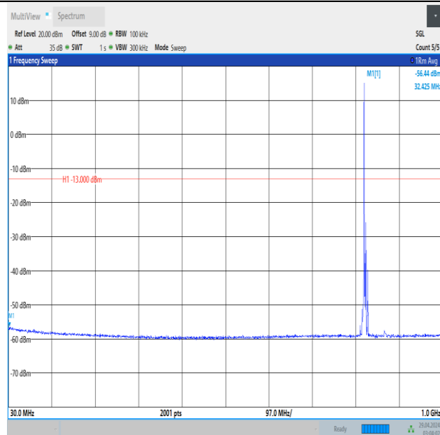
Band5_5MHz_QPSK_20425_1RB#0_30~1000_30~1000
