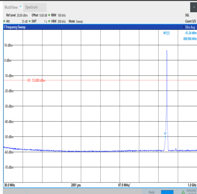
Band5_3MHz_16QAM_20635_15RB#0_30~1000_30~1000
