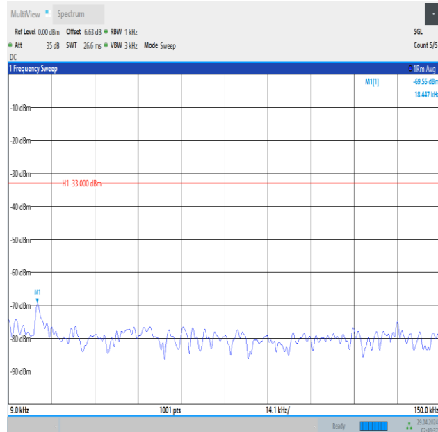
Band5_3MHz_QPSK_20525_1RB#0_0.009~0.15_0.009~0.15
