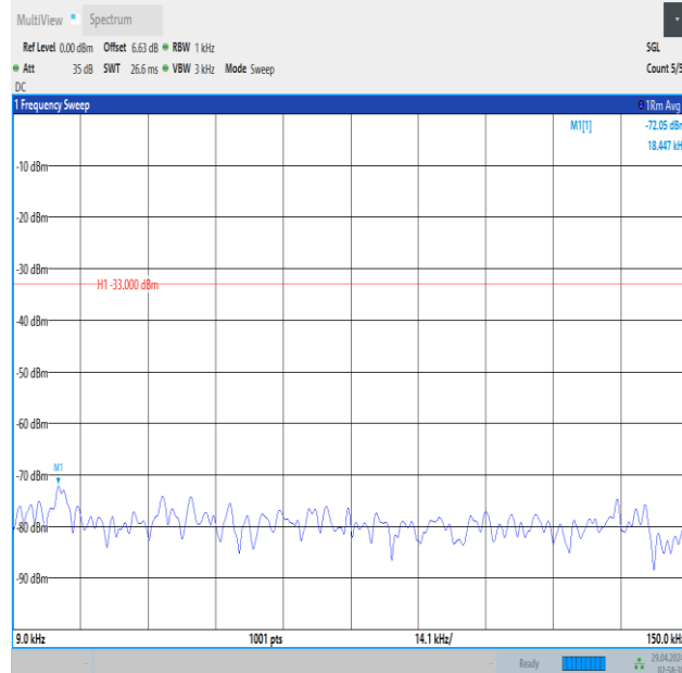
Band5_3MHz_16QAM_20635_15RB#0_0.009~0.15_0.009~0.15
