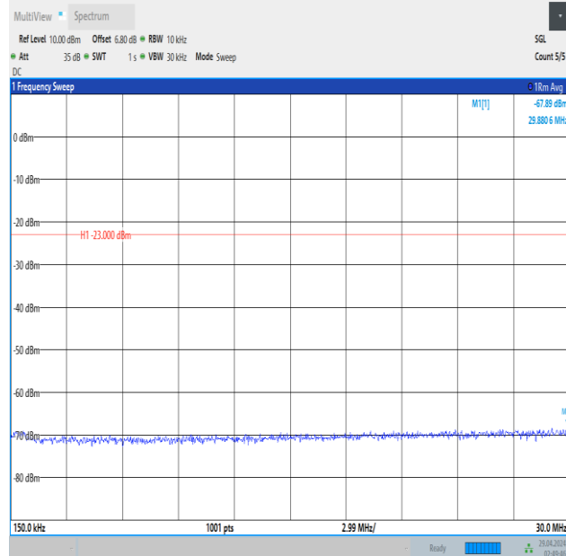
Band5_3MHz_QPSK_20525_1RB#0_0.15~30_0.15~30
