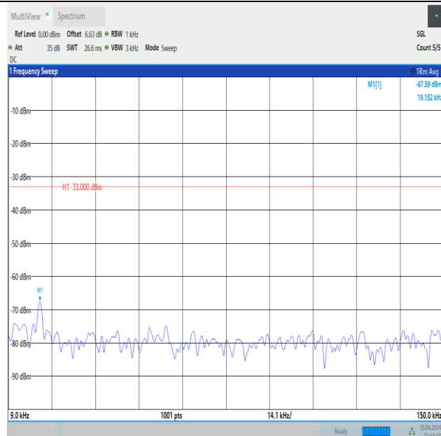
Band5_3MHz_QPSK_20635_1RB#0_0.009~0.15_0.009~0.15
