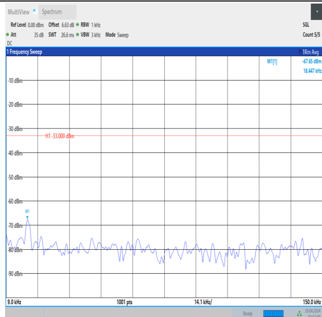
Band5_3MHz_QPSK_20635_15RB#0_0.009~0.15_0.009~0.15
