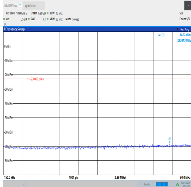
Band5_3MHz_QPSK_20415_15RB#0_0.15~30_0.15~30
