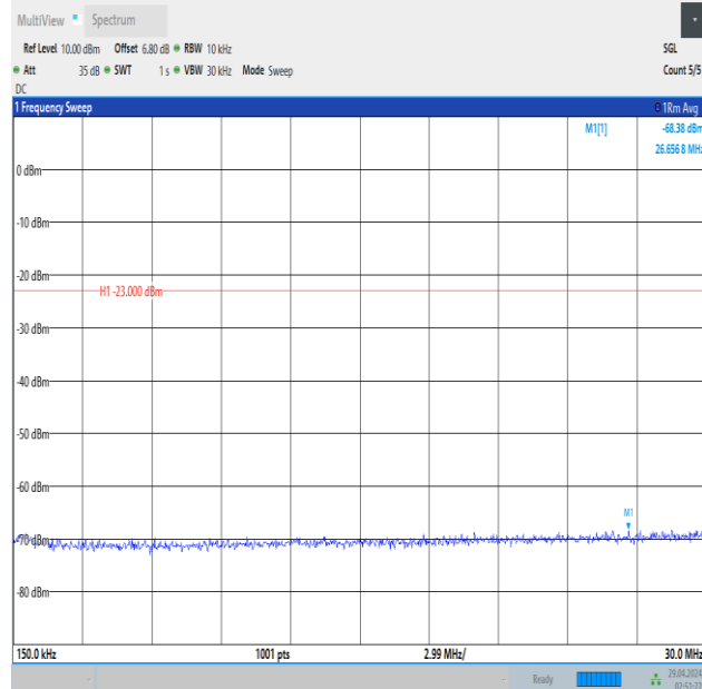
Band5_3MHz_QPSK_20525_1RB#14_0.15~30_0.15~30
