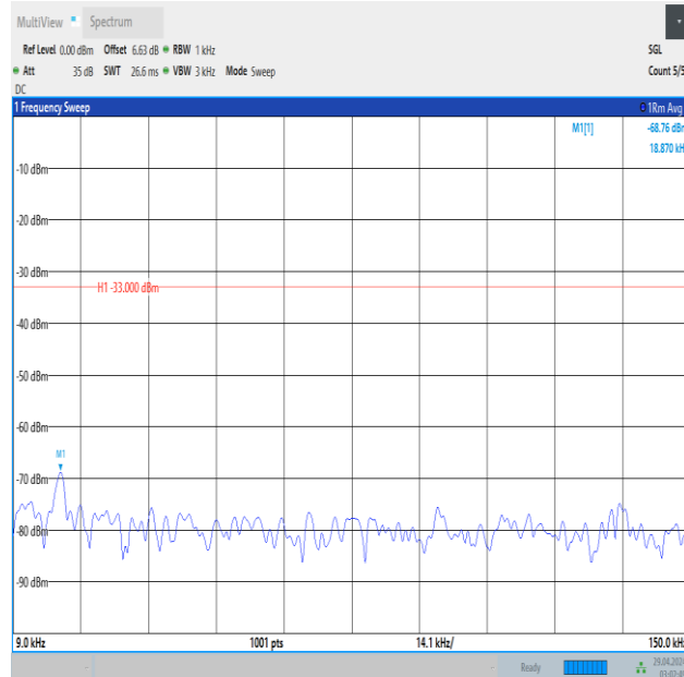
Band5_10MHz_QPSK_20600_50RB#0_0.009~0.15_0.009~0.15
