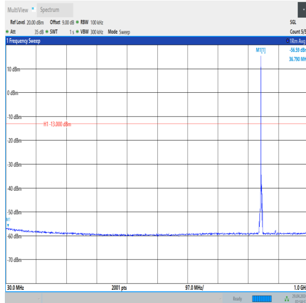
Band5_3MHz_QPSK_20635_1RB#0_30~1000_30~1000
