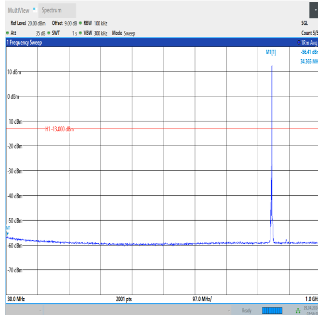
Band5_3MHz_QPSK_20635_1RB#14_30~1000_30~1000
