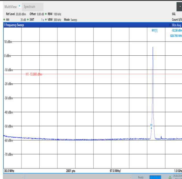
Band5_3MHz_16QAM_20525_15RB#0_30~1000_30~1000
