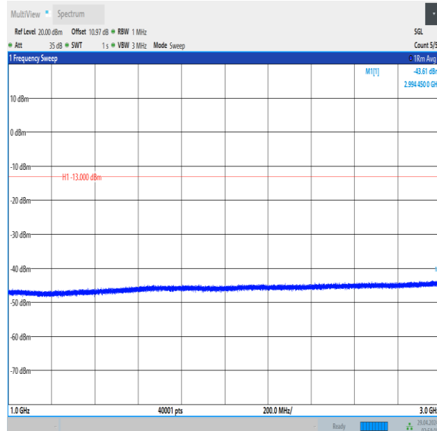
Band5_3MHz_16QAM_20525_15RB#0_1000~3000_1000~3000
