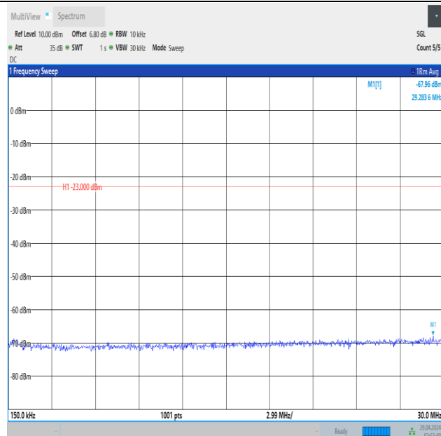
Band5_3MHz_16QAM_20525_15RB#0_0.15~30_0.15~30
