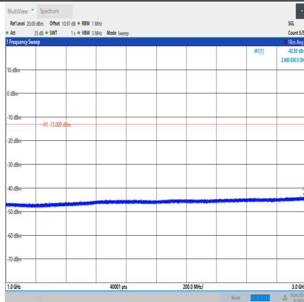
Band5_3MHz_QPSK_20635_15RB#0_1000~3000_1000~3000
