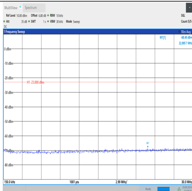
Band5_3MHz_16QAM_20415_15RB#0_0.15~30_0.15~30
