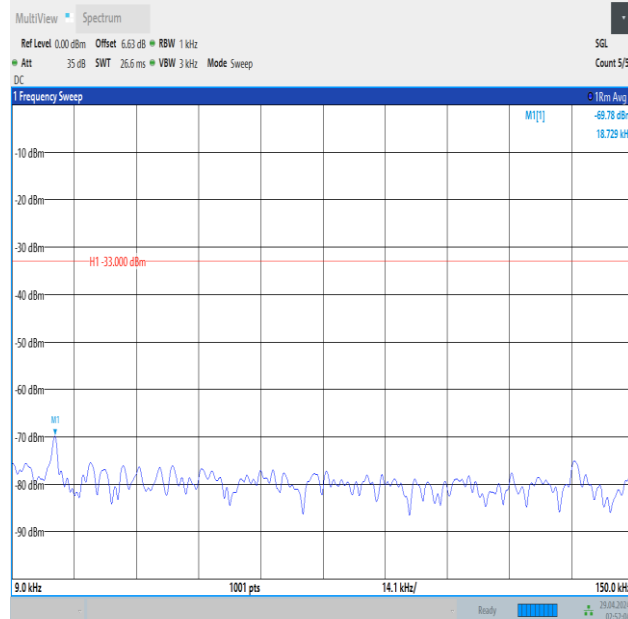
Band5_3MHz_16QAM_20525_1RB#14_0.009~0.15_0.009~0.15
