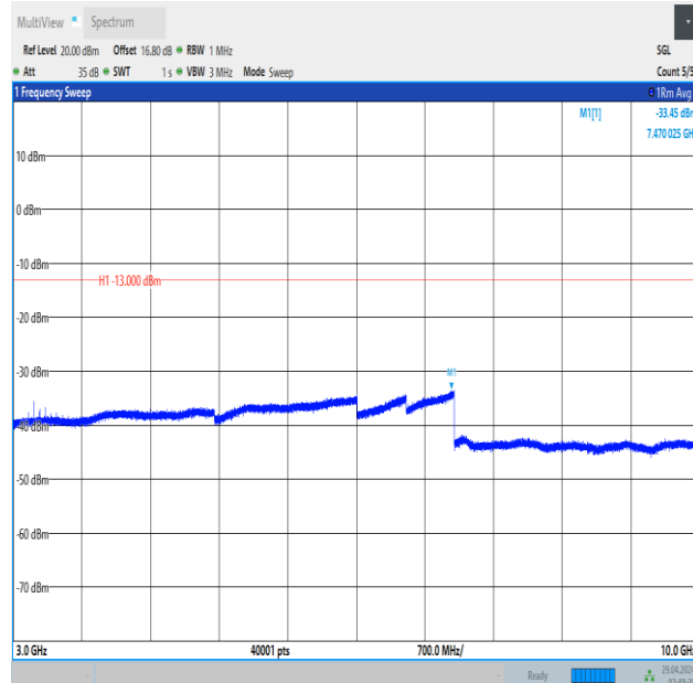
Band5_3MHz_QPSK_20415_15RB#0_3000~10000_3000~10000
