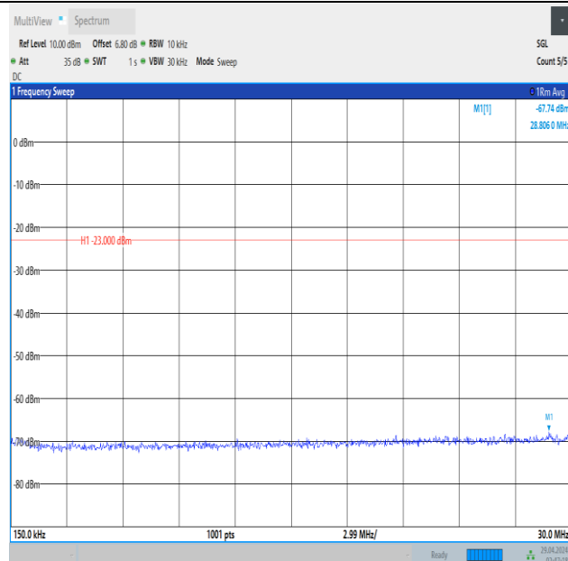
Band5_3MHz_16QAM_20415_1RB#14_0.15~30_0.15~30
