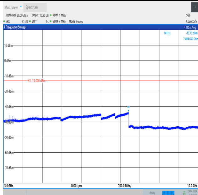
Band5_3MHz_QPSK_20525_1RB#0_3000~10000_3000~10000
