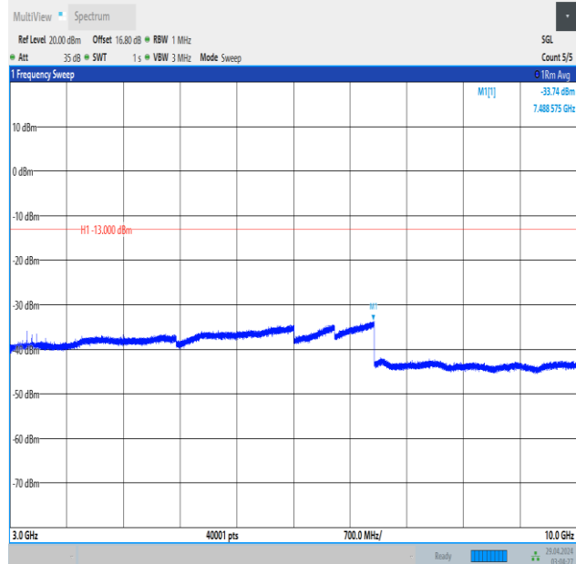
Band5_5MHz_QPSK_20425_1RB#0_3000~10000_3000~10000
