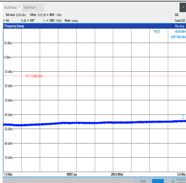
Band5_5MHz_QPSK_20425_1RB#24_1000~3000_1000~3000
