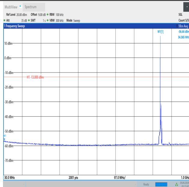
Band5_5MHz_QPSK_20625_1RB#0_30~1000_30~1000
