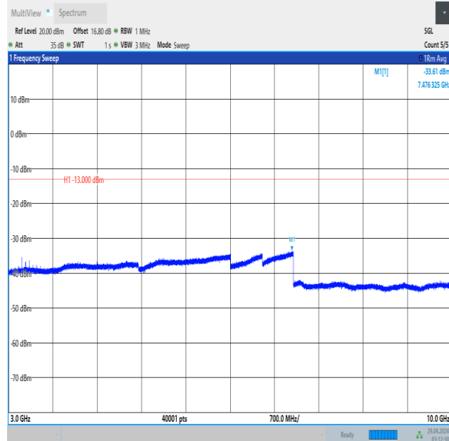
Band5_5MHz_QPSK_20525_25RB#0_3000~10000_3000~10000
