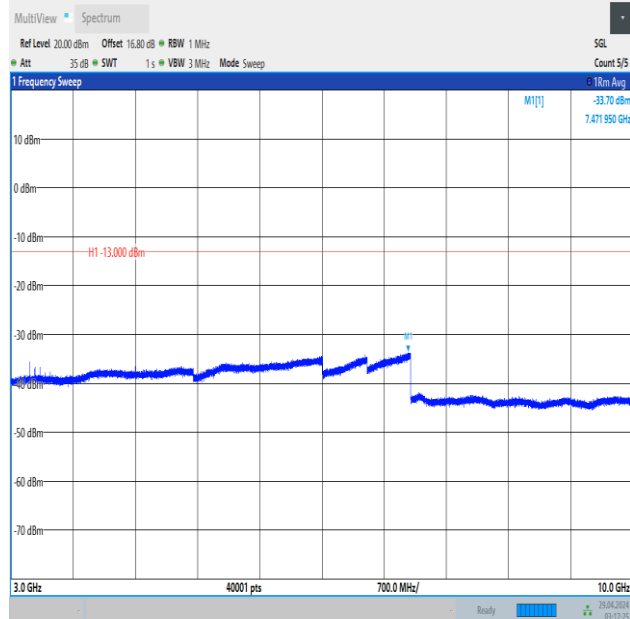
Band5_5MHz_QPSK_20625_25RB#0_3000~10000_3000~10000
