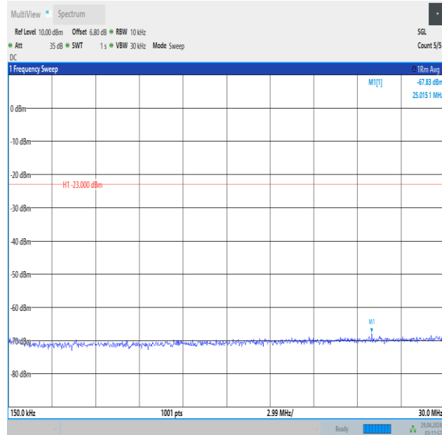
Band5_5MHz_QPSK_20525_25RB#0_0.15~30_0.15~30
