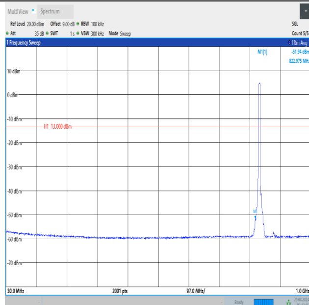
Band5_5MHz_QPSK_20525_25RB#0_30~1000_30~1000
