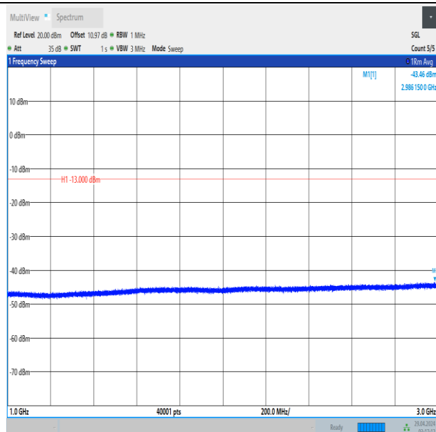
Band5_5MHz_QPSK_20625_25RB#0_1000~3000_1000~3000
