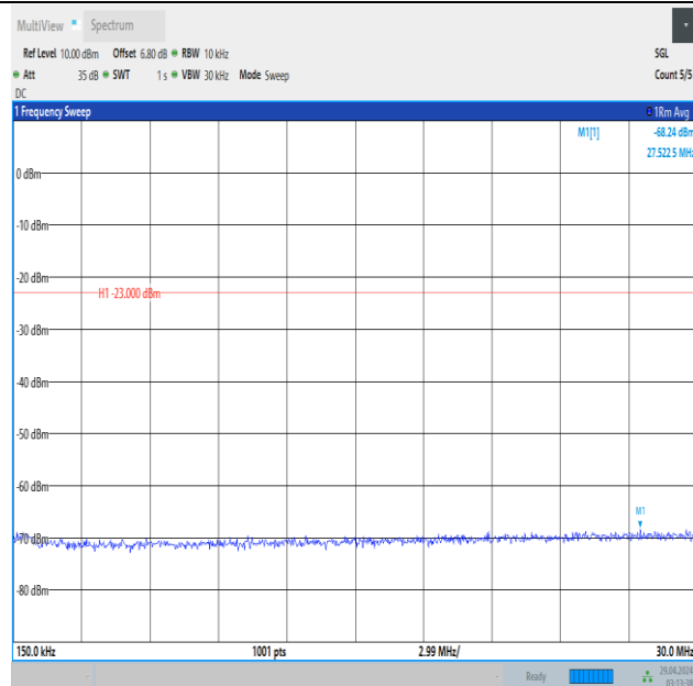
Band5_5MHz_QPSK_20625_1RB#0_0.15~30_0.15~30
