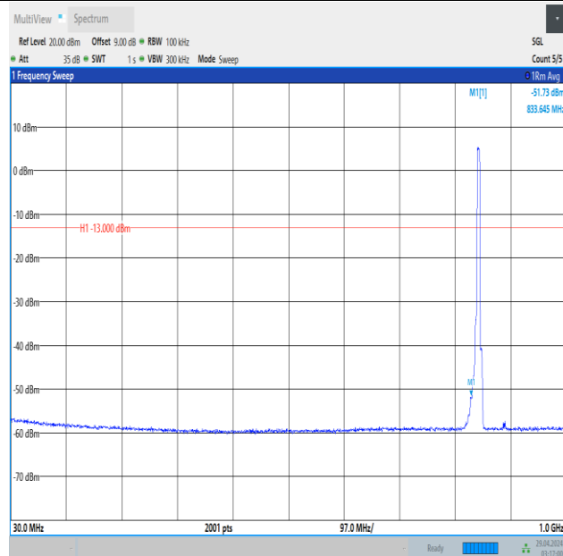
Band5_5MHz_QPSK_20625_25RB#0_30~1000_30~1000
