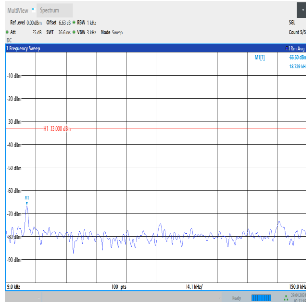
Band5_5MHz_QPSK_20525_25RB#0_0.009~0.15_0.009~0.15
