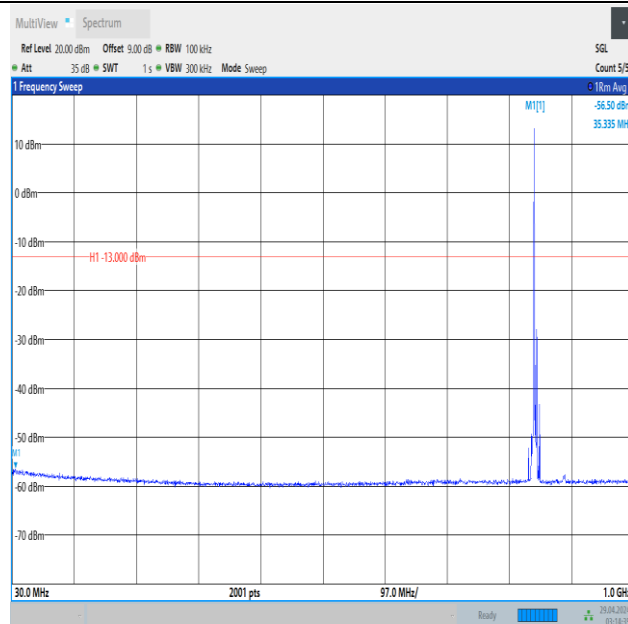
Band5_5MHz_16QAM_20625_1RB#0_30~1000_30~1000
