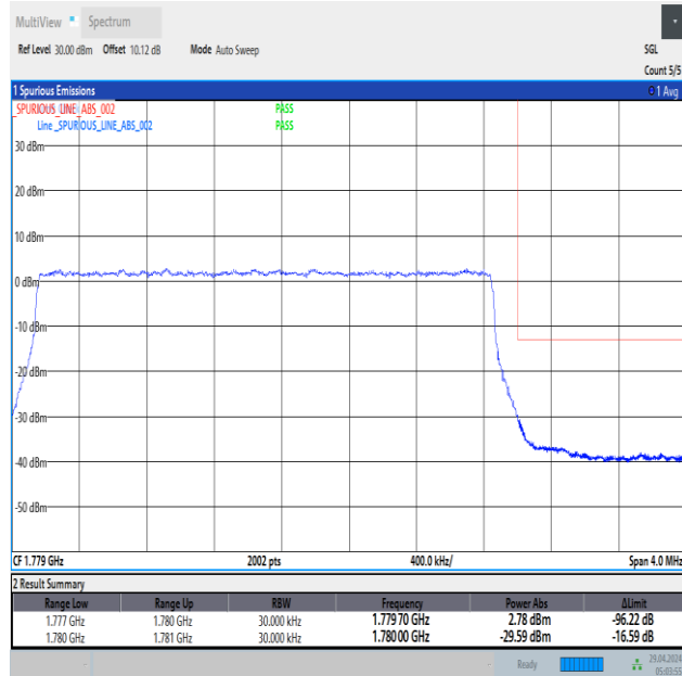
Band66_3MHz_QPSK_132657_15RB#0
