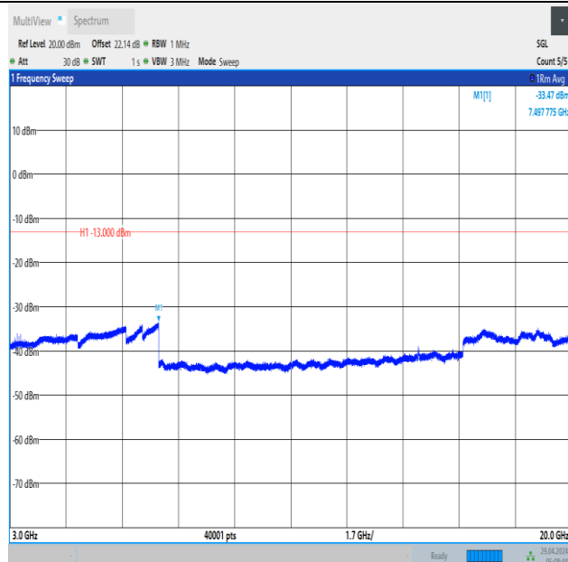
Band66_1.4MHz_QPSK_131979_1RB#0_3000~20000_3000~20000
