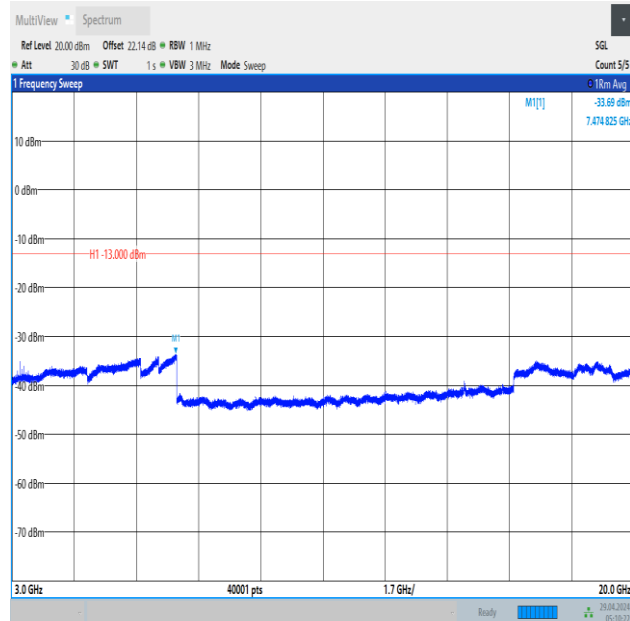
Band66_1.4MHz_QPSK_131979_1RB#5_3000~20000_3000~20000
