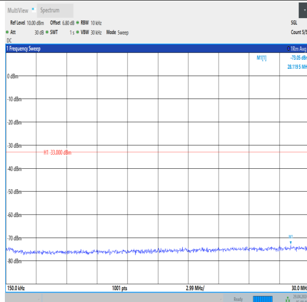
Band66_1.4MHz_QPSK_131979_1RB#5_0.15~30_0.15~30
