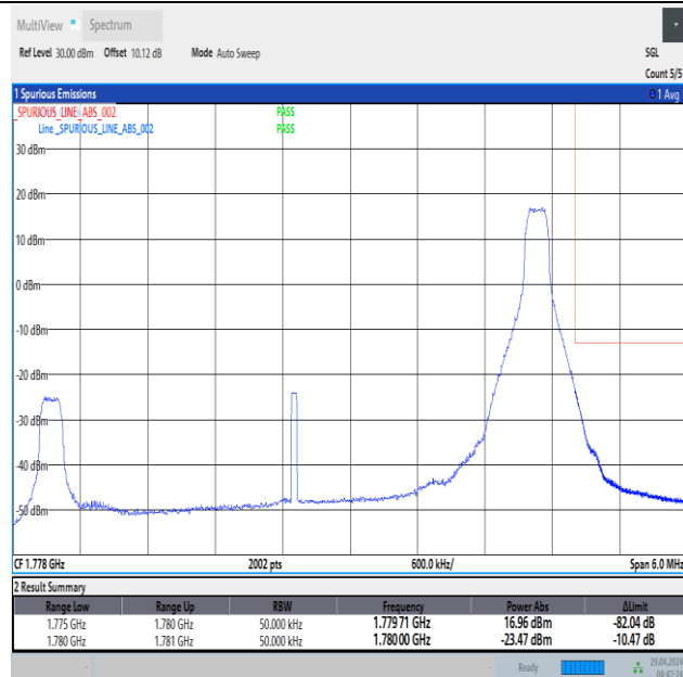
Band66_5MHz_QPSK_132647_1RB#24
