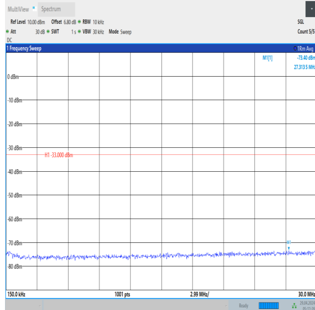
Band66_1.4MHz_QPSK_131979_6RB#0_0.15~30_0.15~30
