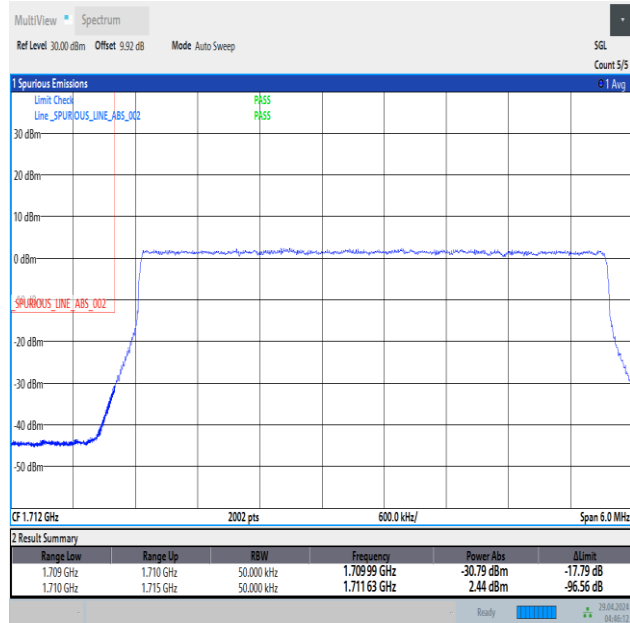
Band66_5MHz_QPSK_131997_25RB#0
