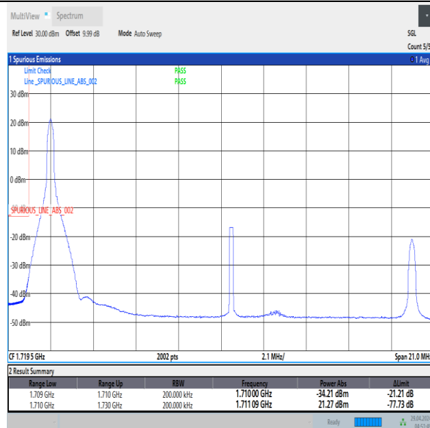
Band66_20MHz_16QAM_132072_1RB#0
