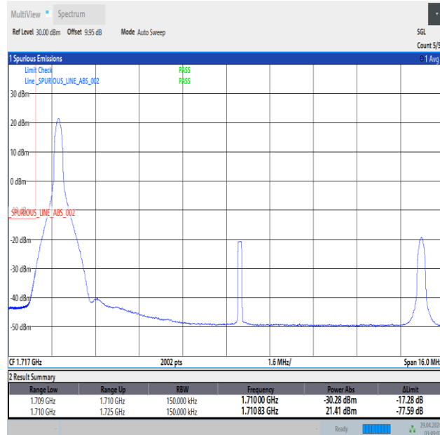
Band66_15MHz_QPSK_132047_1RB#0
