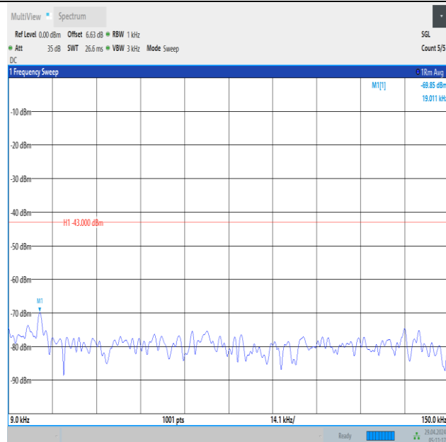
Band66_1.4MHz_QPSK_131979_6RB#0_0.009~0.15_0.009~0.15
