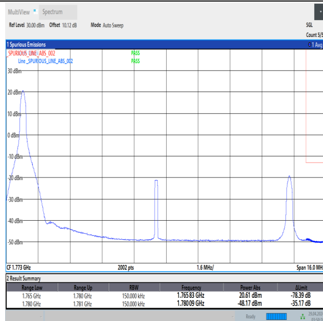
Band66_15MHz_QPSK_132597_1RB#0
