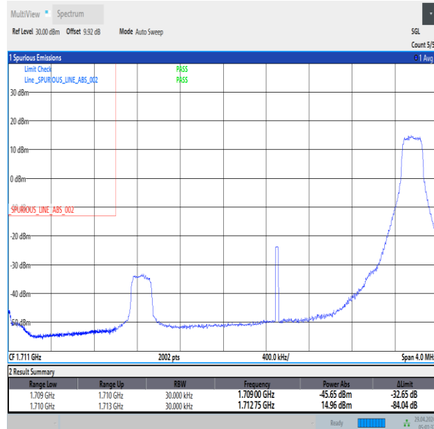
Band66_3MHz_QPSK_131987_1RB#14
