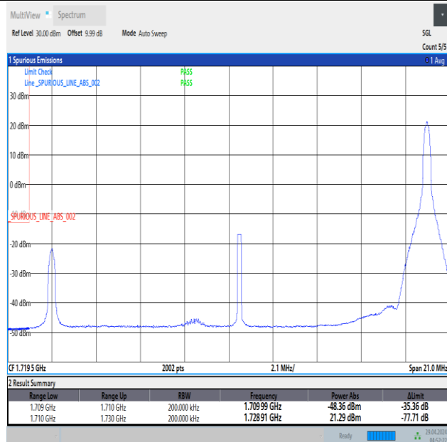
Band66_20MHz_16QAM_132072_1RB#99
