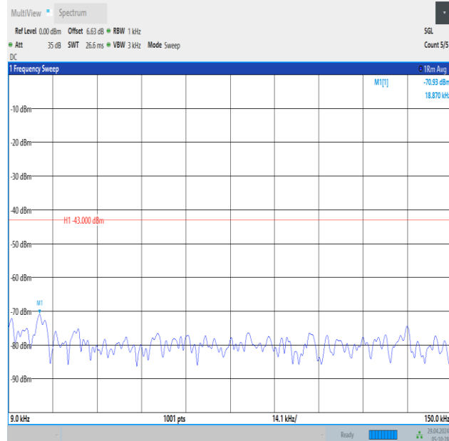
Band66_1.4MHz_16QAM_131979_1RB#5_0.009~0.15_0.009~0.15
