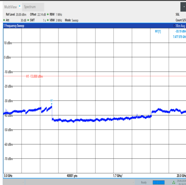
Band66_1.4MHz_16QAM_132322_1RB#0_3000~20000_3000~20000
