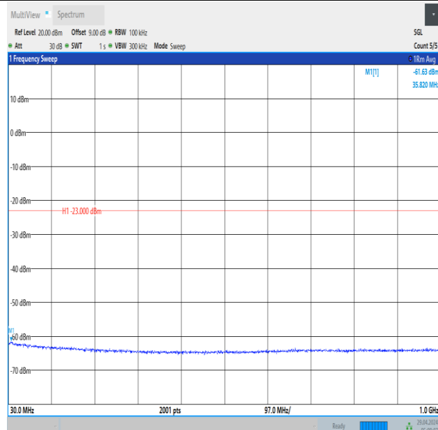
Band66_1.4MHz_16QAM_131979_1RB#0_30~1000_30~1000
