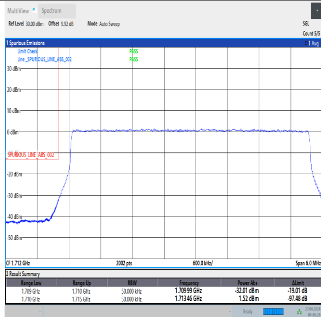
Band66_5MHz_16QAM_131997_25RB#0
