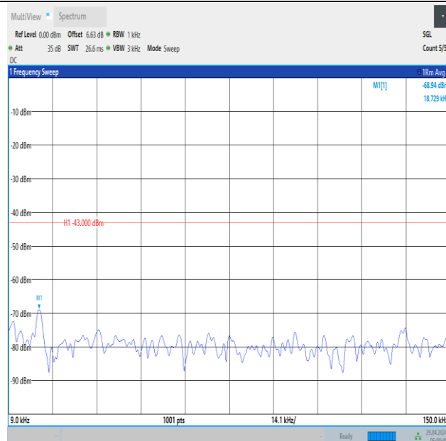
Band66_1.4MHz_QPSK_131979_1RB#5_0.009~0.15_0.009~0.15
