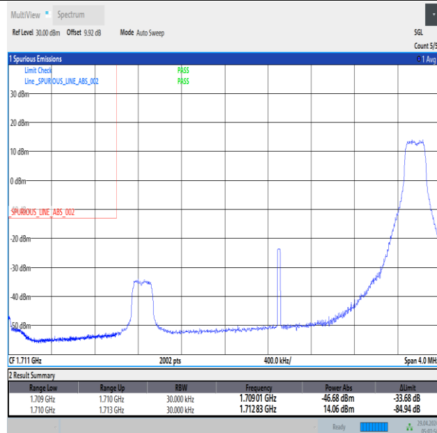
Band66_3MHz_16QAM_131987_1RB#14
