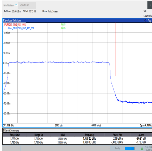
Band66_3MHz_16QAM_132657_15RB#0
