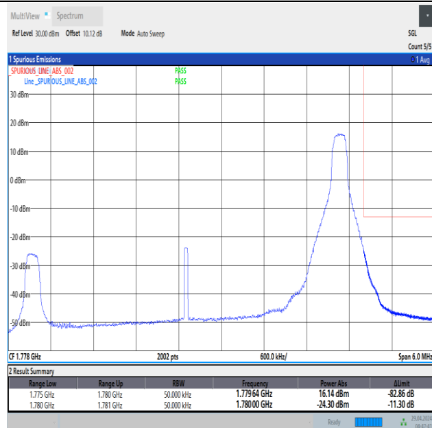
Band66_5MHz_16QAM_132647_1RB#24
