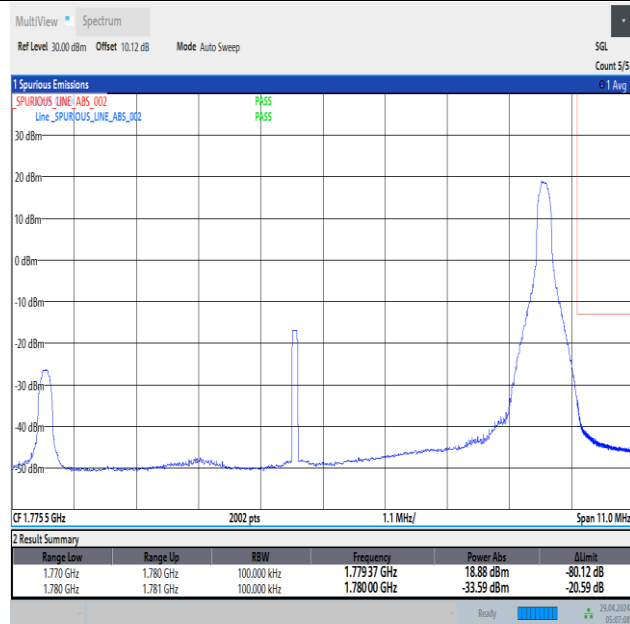
Band66_10MHz_16QAM_132622_1RB#49
