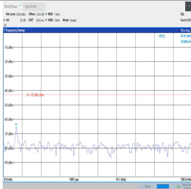
Band66_1.4MHz_16QAM_131979_1RB#0_0.009~0.15_0.009~0.15
