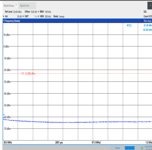
Band66_1.4MHz_QPSK_132322_1RB#5_30~1000_30~1000
