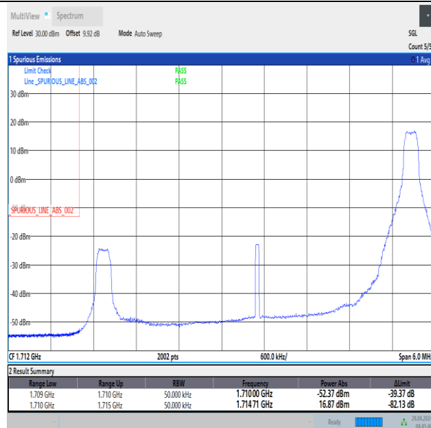
Band66_5MHz_QPSK_131997_1RB#24
