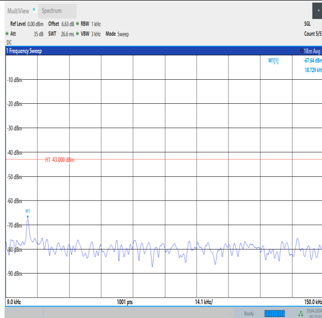
Band66_1.4MHz_16QAM_132322_1RB#0_0.009~0.15_0.009~0.15
