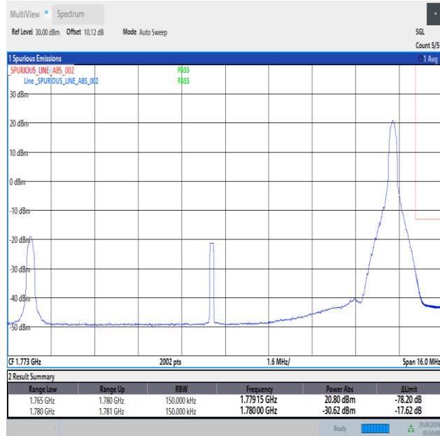
Band66_15MHz_QPSK_132597_1RB#74
