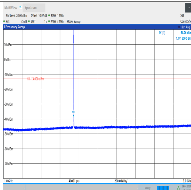
Band66_1.4MHz_16QAM_132322_1RB#0_1000~3000_1000~3000
