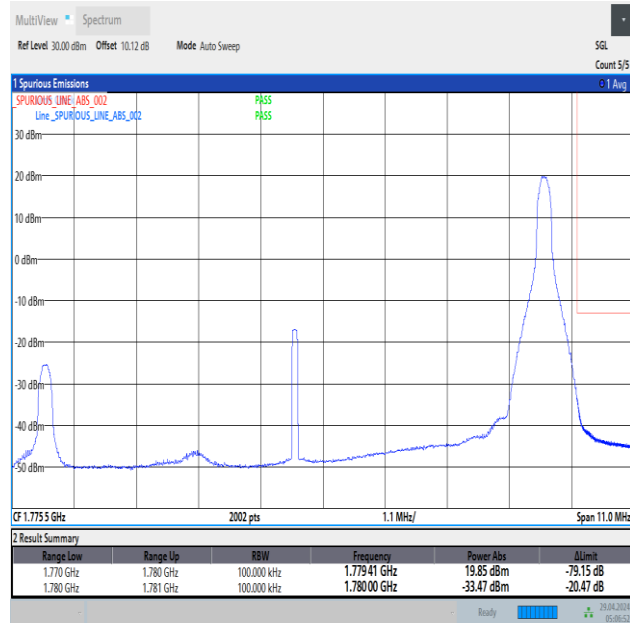
Band66_10MHz_QPSK_132622_1RB#49
