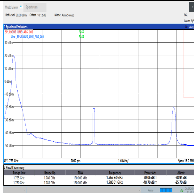
Band66_15MHz_16QAM_132597_1RB#0
