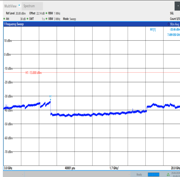
Band66_1.4MHz_16QAM_131979_1RB#0_3000~20000_3000~20000
