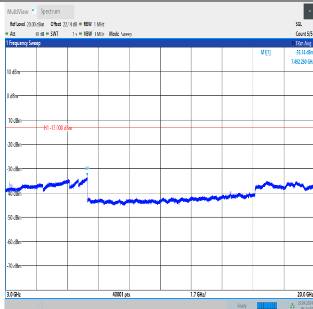
Band66_1.4MHz_QPSK_132322_1RB#0_3000~20000_3000~20000
