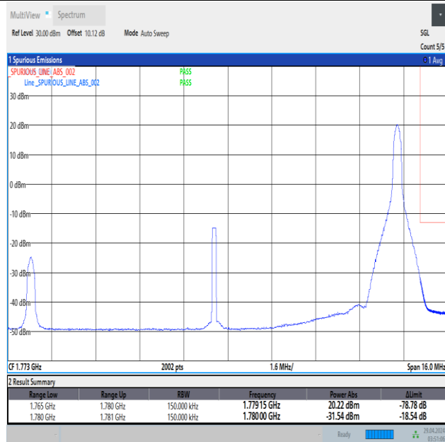
Band66_15MHz_16QAM_132597_1RB#74
