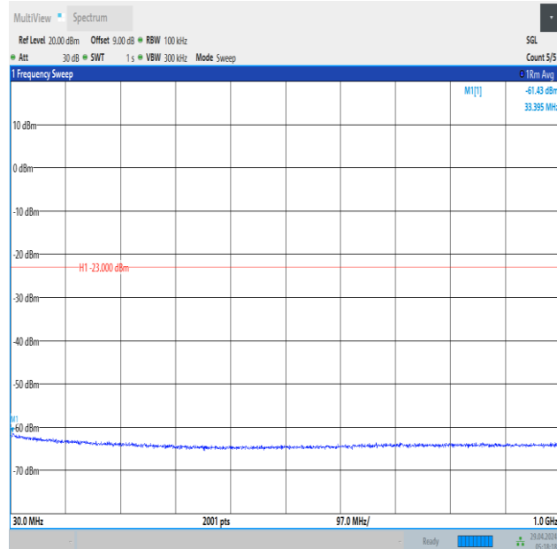
Band66_1.4MHz_QPSK_132665_1RB#0_30~1000_30~1000
