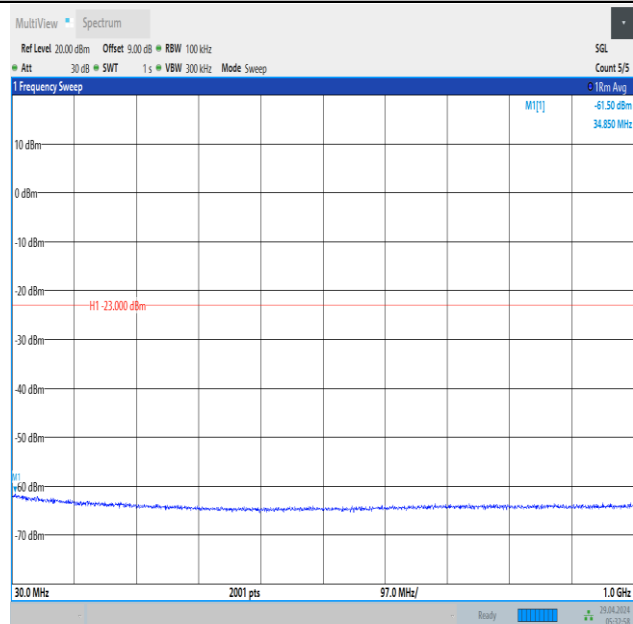
Band66_3MHz_16QAM_132322_15RB#0_30~1000_30~1000
