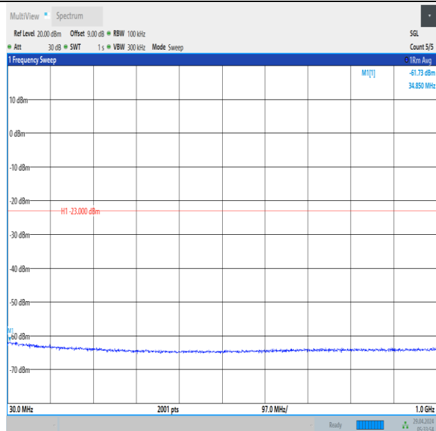
Band66_3MHz_QPSK_132657_1RB#0_30~1000_30~1000
