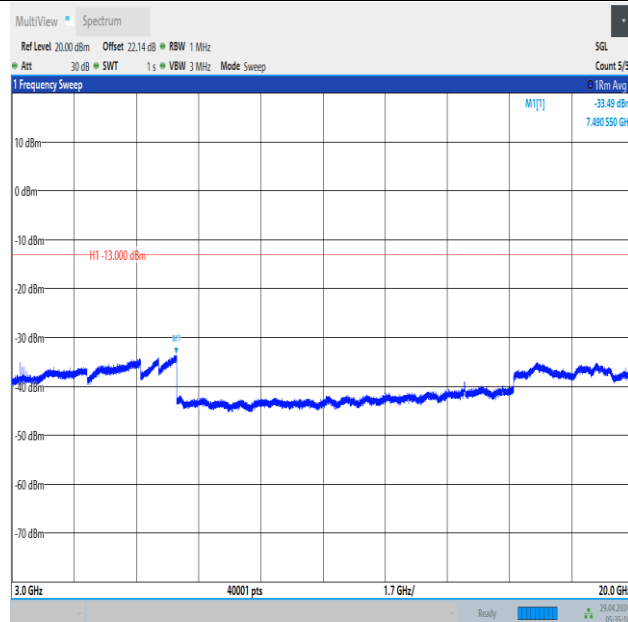
Band66_3MHz_16QAM_132657_1RB#0_3000~20000_3000~20000
