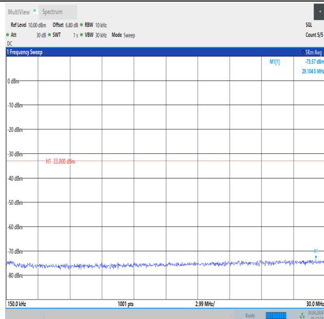
Band66_1.4MHz_16QAM_132322_6RB#0_0.15~30_0.15~30
