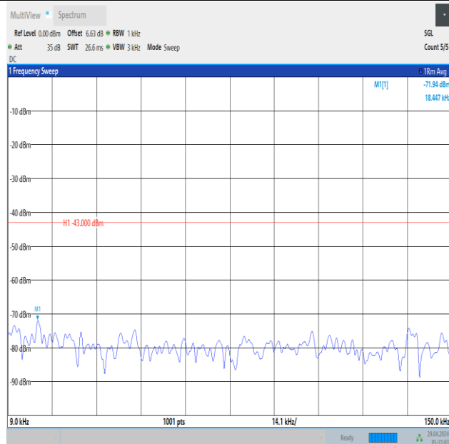
Band66_3MHz_16QAM_132322_1RB#14_0.009~0.15_0.009~0.15
