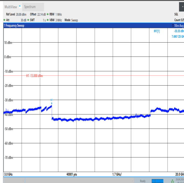
Band66_3MHz_QPSK_132322_15RB#0_3000~20000_3000~20000
