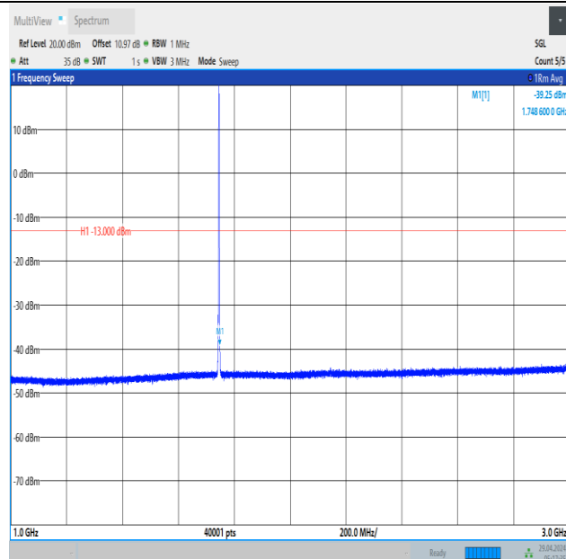
Band66_1.4MHz_16QAM_132322_6RB#0_1000~3000_1000~3000
