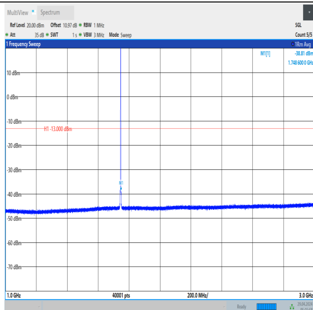
Band66_1.4MHz_16QAM_132322_1RB#5_1000~3000_1000~3000
