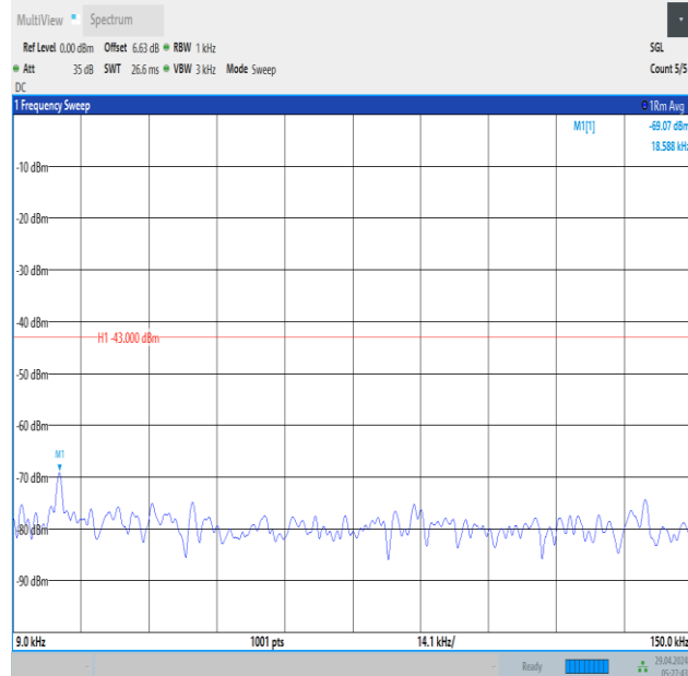
Band66_3MHz_16QAM_131987_15RB#0_0.009~0.15_0.009~0.15
