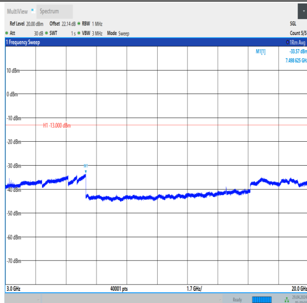
Band66_3MHz_QPSK_132322_1RB#14_3000~20000_3000~20000
