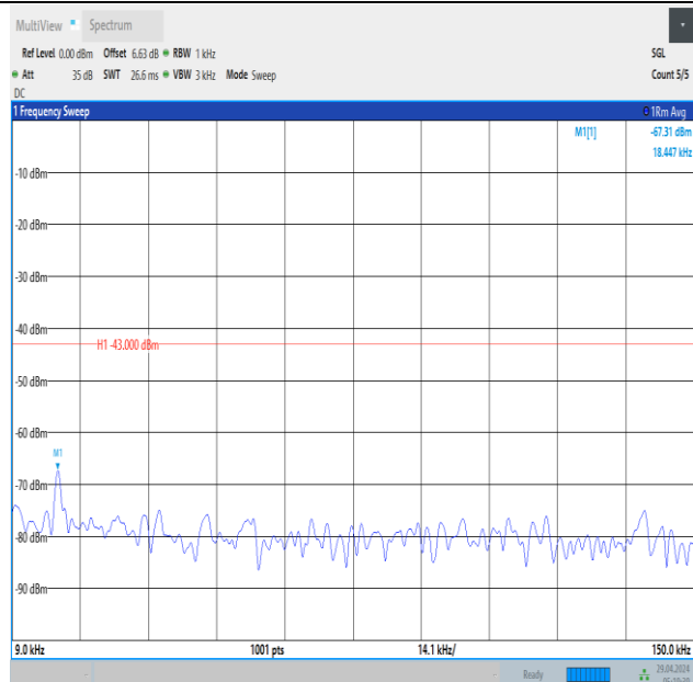
Band66_1.4MHz_QPSK_132665_1RB#5_0.009~0.15_0.009~0.15
