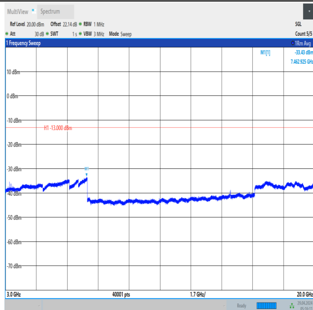
Band66_1.4MHz_16QAM_132322_1RB#5_3000~20000_3000~20000
