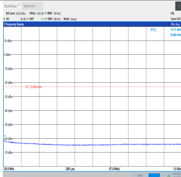
Band66_3MHz_16QAM_131987_1RB#0_30~1000_30~1000
