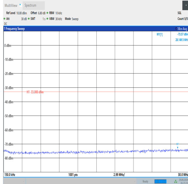
Band66_1.4MHz_QPSK_132665_6RB#0_0.15~30_0.15~30
