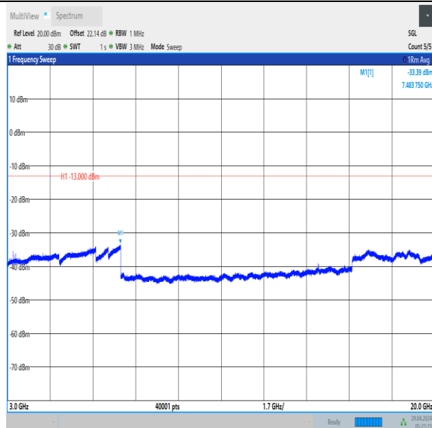
Band66_1.4MHz_16QAM_132665_1RB#5_3000~20000_3000~20000
