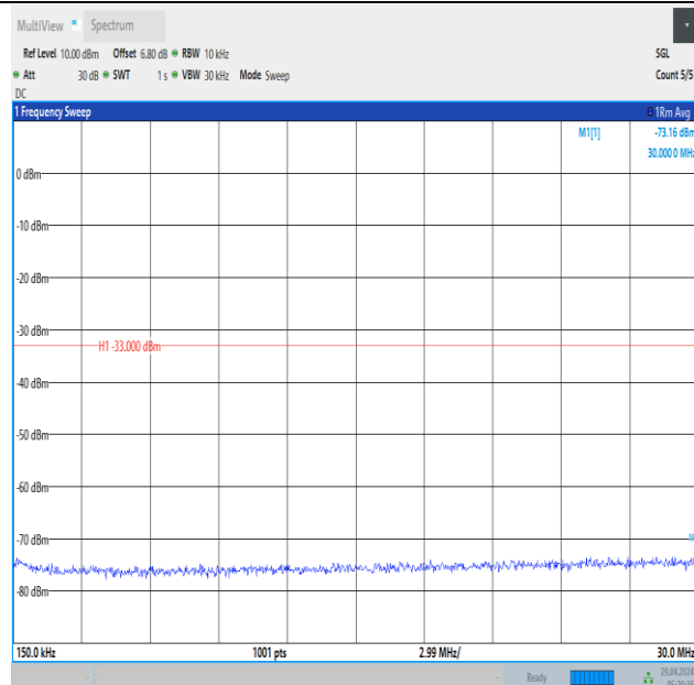
Band66_1.4MHz_16QAM_132665_1RB#5_0.15~30_0.15~30
