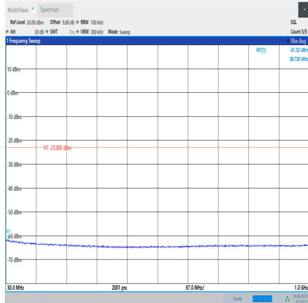
Band66_3MHz_QPSK_132322_1RB#0_30~1000_30~1000
