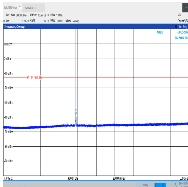
Band66_1.4MHz_16QAM_132665_1RB#5_1000~3000_1000~3000
