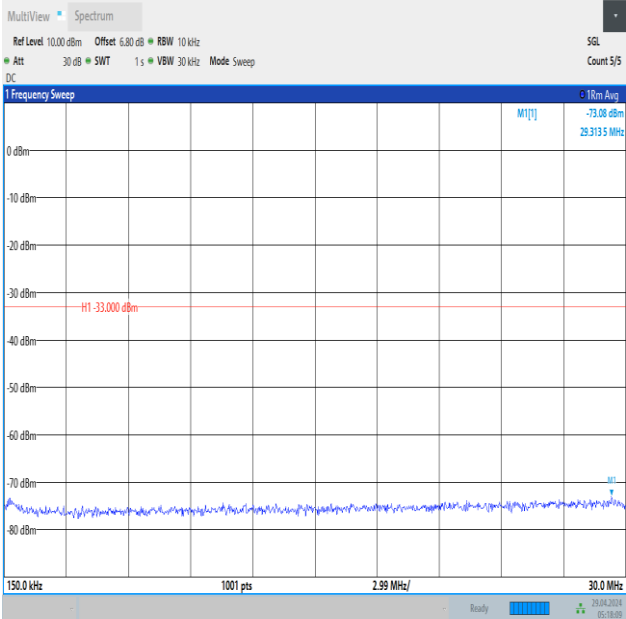
Band66_1.4MHz_QPSK_132665_1RB#0_0.15~30_0.15~30
