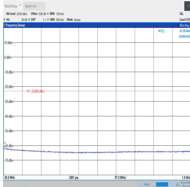
Band66_3MHz_QPSK_131987_15RB#0_30~1000_30~1000
