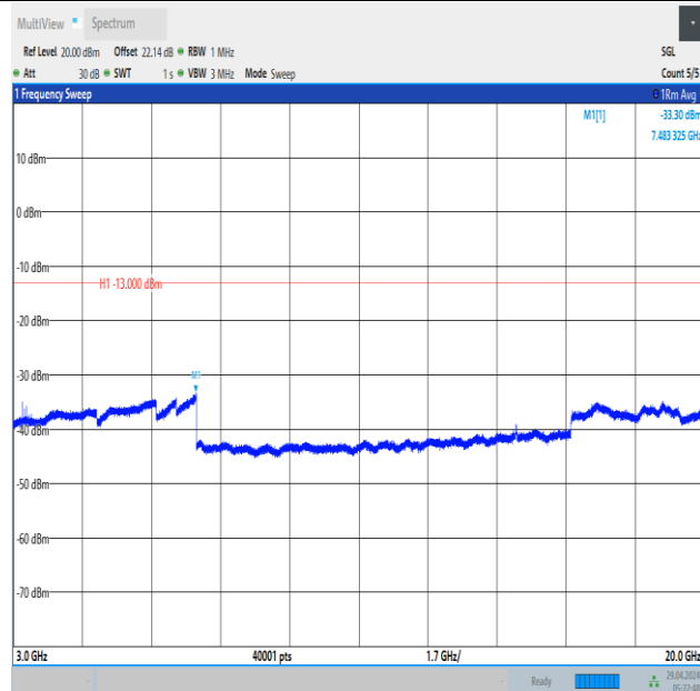
Band66_1.4MHz_16QAM_132665_6RB#0_3000~20000_3000~20000
