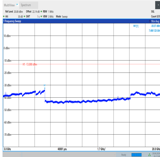
Band66_1.4MHz_QPSK_132322_6RB#0_3000~20000_3000~20000
