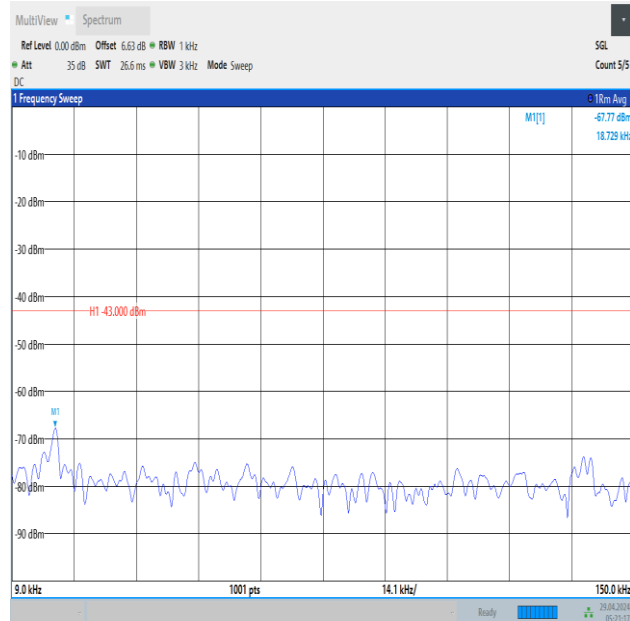
Band66_1.4MHz_QPSK_132665_6RB#0_0.009~0.15_0.009~0.15
