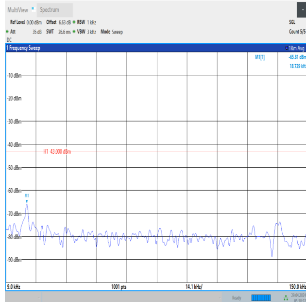
Band66_3MHz_QPSK_132322_1RB#14_0.009~0.15_0.009~0.15
