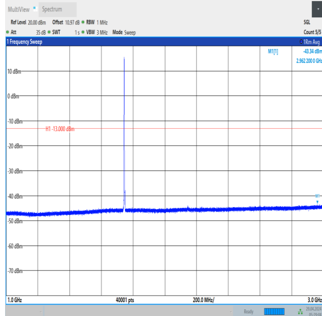
Band66_3MHz_QPSK_132322_1RB#0_1000~3000_1000~3000
