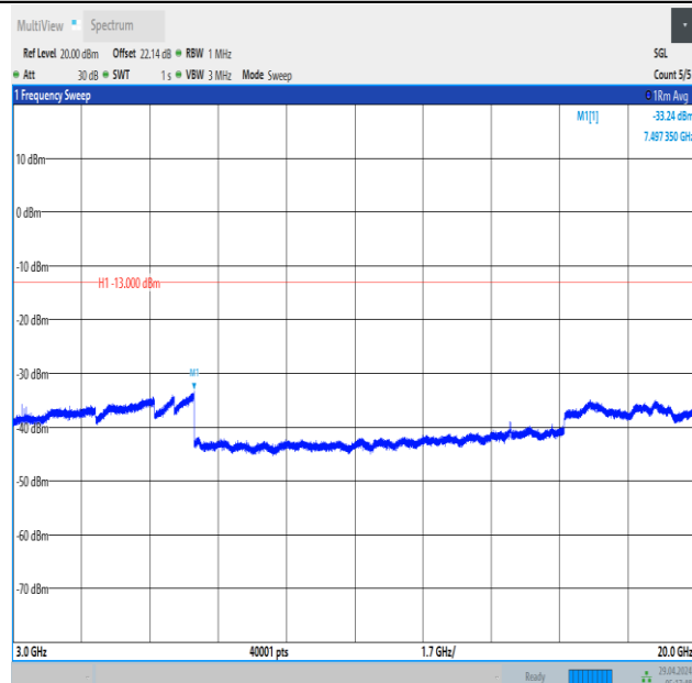
Band66_1.4MHz_16QAM_132322_6RB#0_3000~20000_3000~20000
