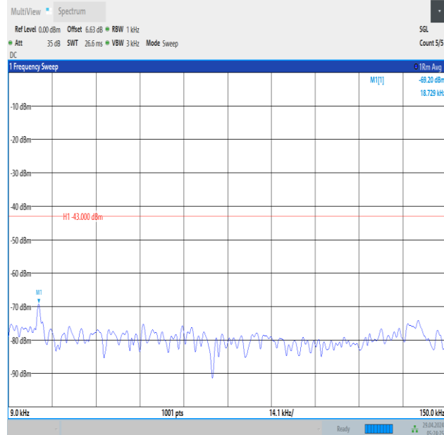
Band66_3MHz_16QAM_131987_1RB#0_0.009~0.15_0.009~0.15
