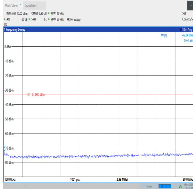
Band66_3MHz_QPSK_132322_1RB#14_0.15~30_0.15~30
