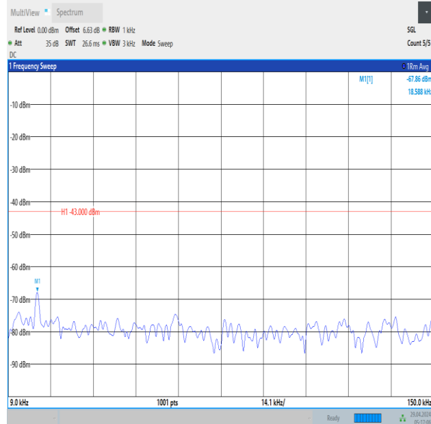
Band66_1.4MHz_16QAM_132322_6RB#0_0.009~0.15_0.009~0.15
