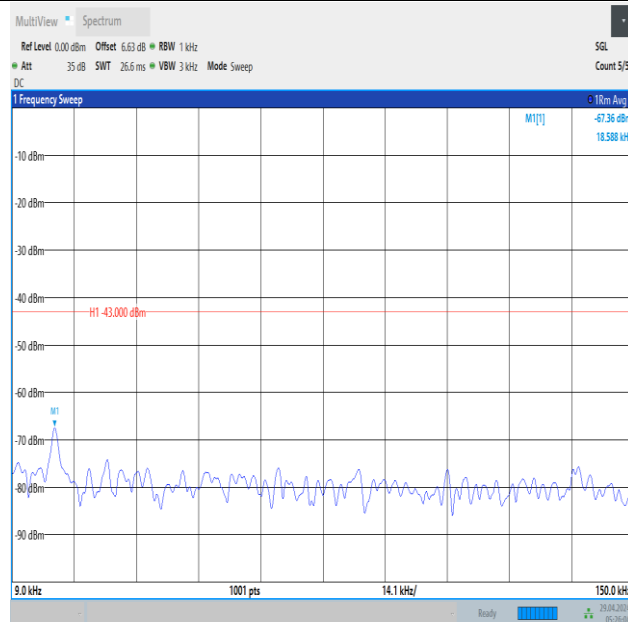
Band66_3MHz_16QAM_131987_1RB#14_0.009~0.15_0.009~0.15
