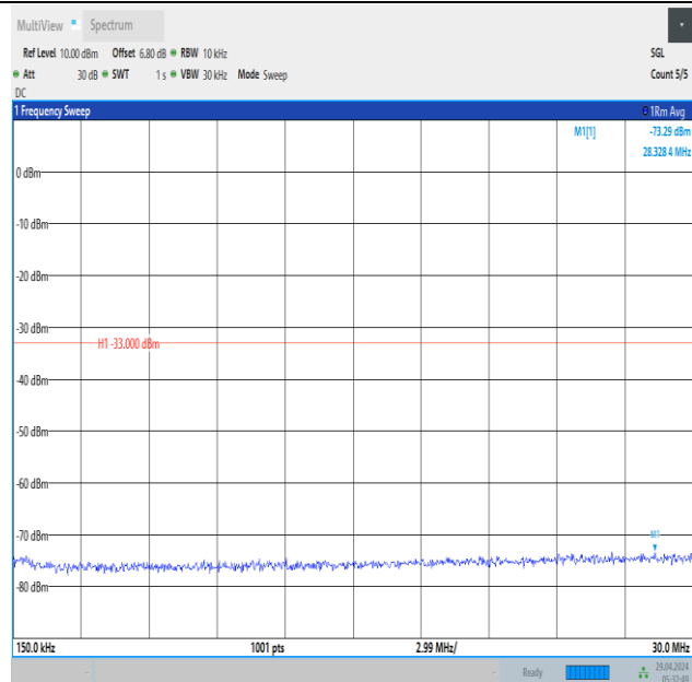
Band66_3MHz_16QAM_132322_15RB#0_0.15~30_0.15~30
