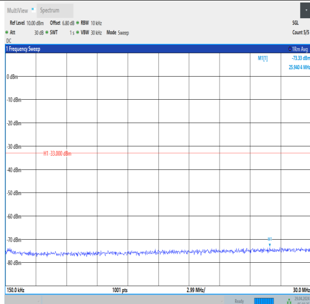
Band66_1.4MHz_QPSK_132322_6RB#0_0.15~30_0.15~30
