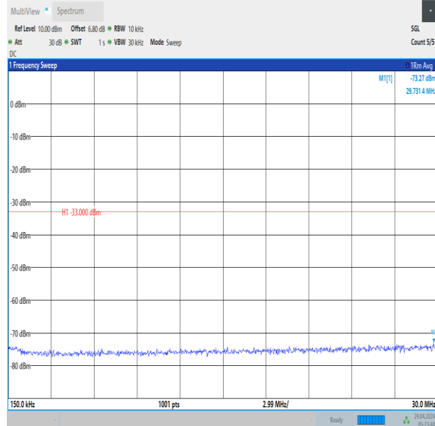
Band66_3MHz_QPSK_131987_1RB#0_0.15~30_0.15~30
