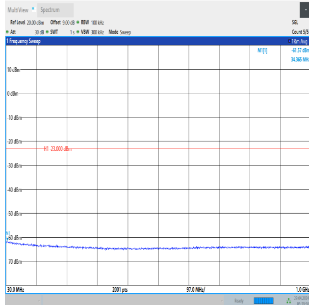
Band66_1.4MHz_QPSK_132665_1RB#5_30~1000_30~1000
