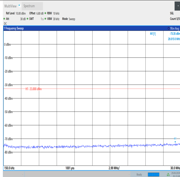
Band66_3MHz_QPSK_132322_15RB#0_0.15~30_0.15~30
