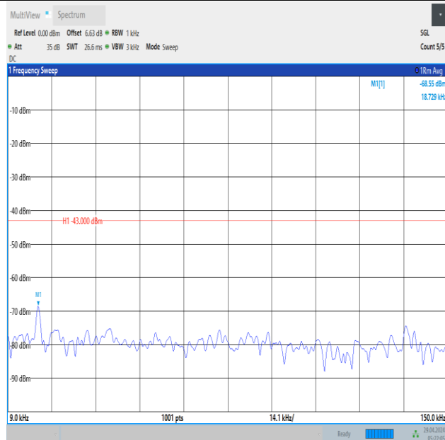
Band66_1.4MHz_16QAM_132665_6RB#0_0.009~0.15_0.009~0.15
