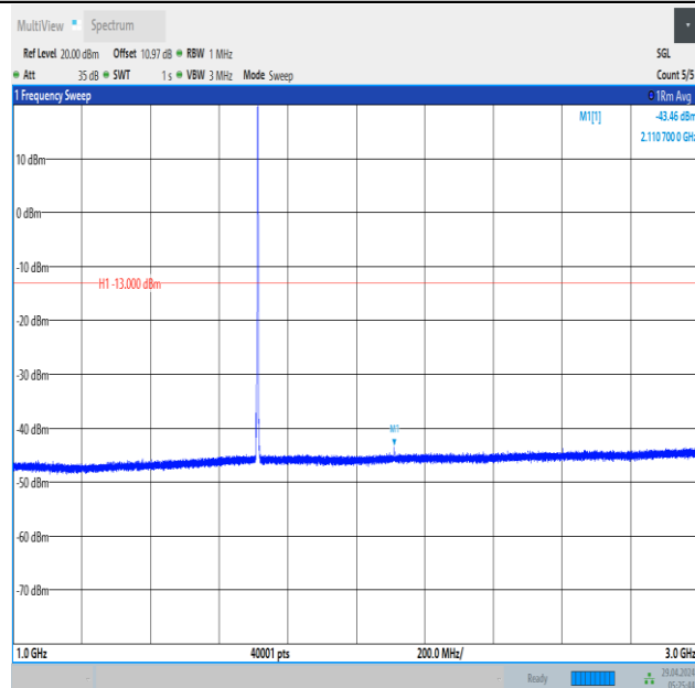
Band66_3MHz_QPSK_131987_1RB#14_1000~3000_1000~3000
