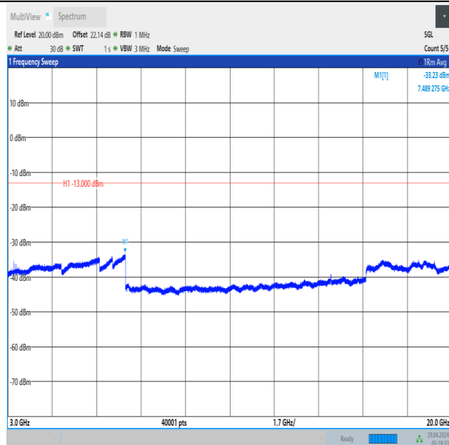
Band66_1.4MHz_16QAM_132665_1RB#0_3000~20000_3000~20000
