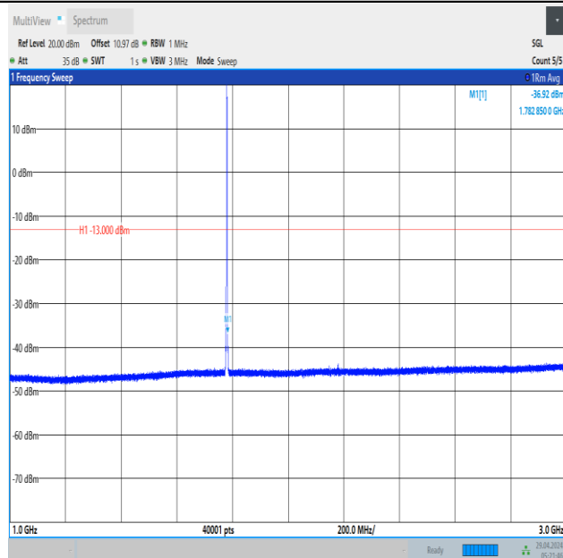
Band66_1.4MHz_QPSK_132665_6RB#0_1000~3000_1000~3000
