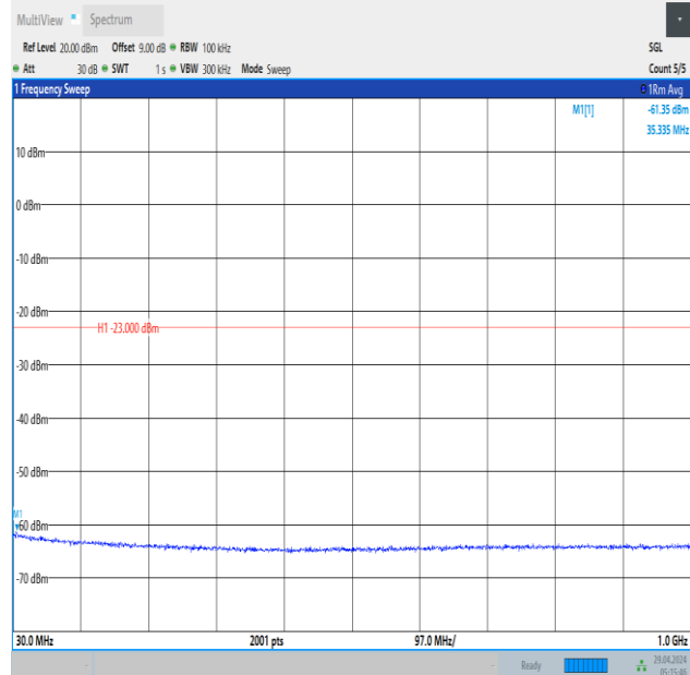
Band66_1.4MHz_16QAM_132322_1RB#5_30~1000_30~1000
