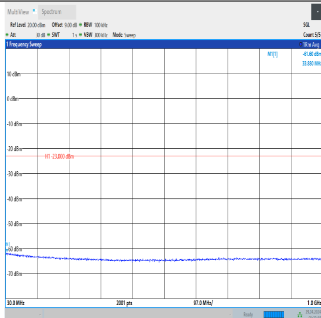
Band66_1.4MHz_QPSK_132665_6RB#0_30~1000_30~1000
