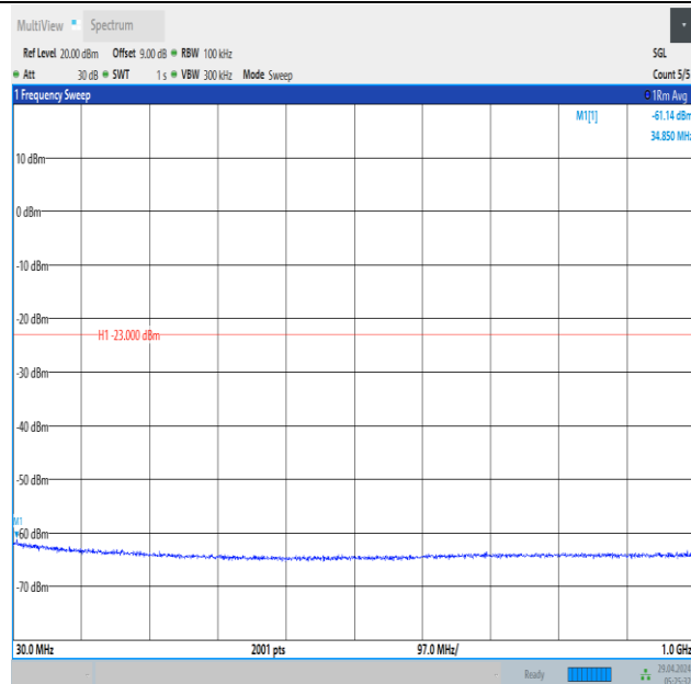
Band66_3MHz_QPSK_131987_1RB#14_30~1000_30~1000
