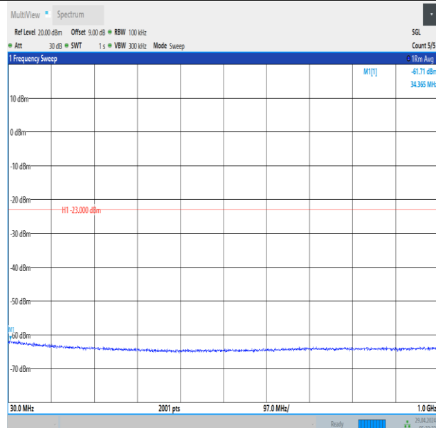
Band66_1.4MHz_16QAM_132665_6RB#0_30~1000_30~1000
