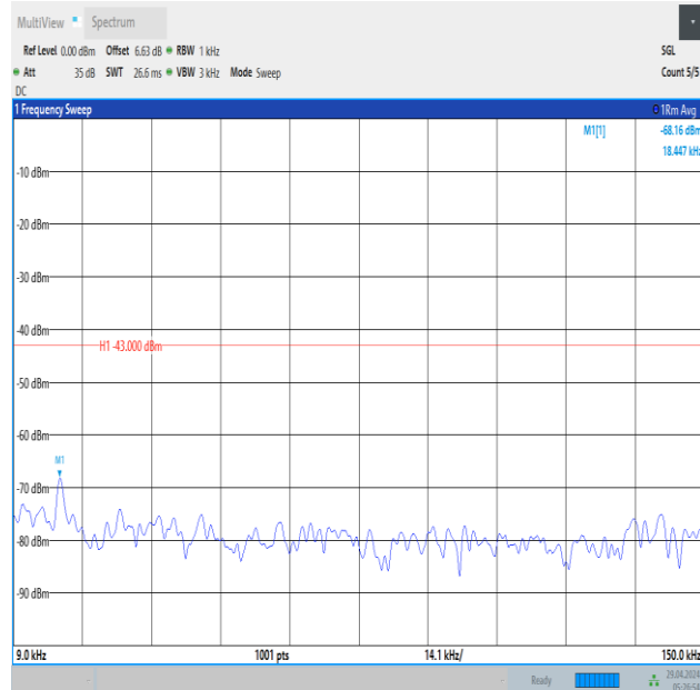
Band66_3MHz_QPSK_131987_15RB#0_0.009~0.15_0.009~0.15
