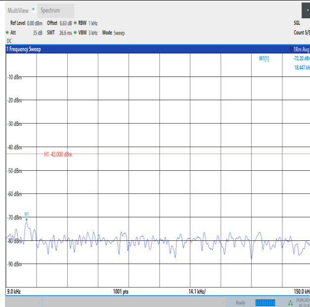
Band66_3MHz_16QAM_132322_15RB#0_0.009~0.15_0.009~0.15
