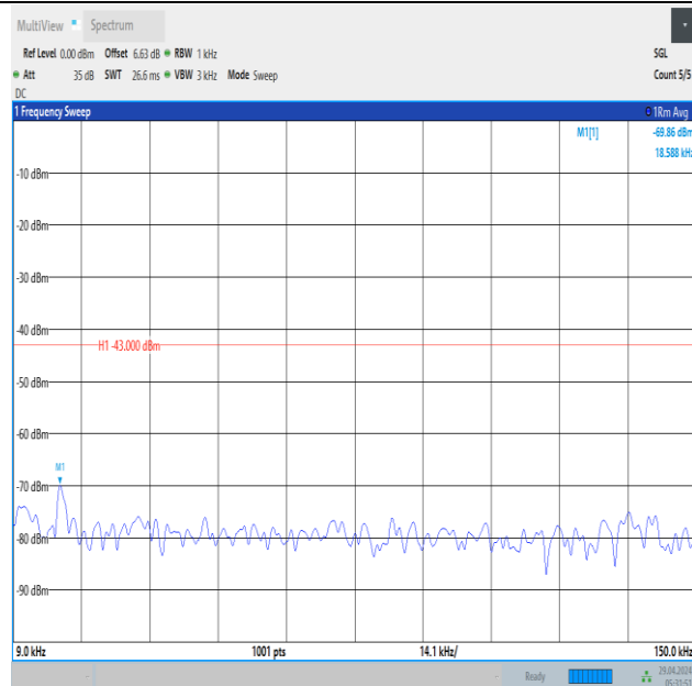
Band66_3MHz_QPSK_132322_15RB#0_0.009~0.15_0.009~0.15
