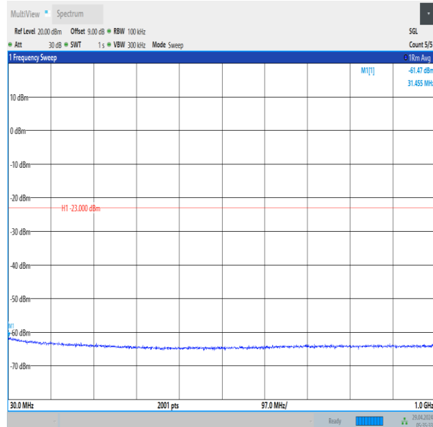
Band66_3MHz_QPSK_132657_1RB#14_30~1000_30~1000
