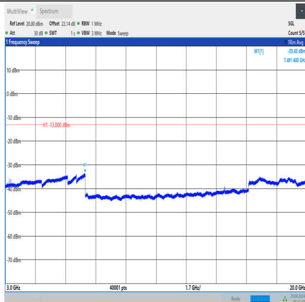
Band66_1.4MHz_QPSK_132665_6RB#0_3000~20000_3000~20000
