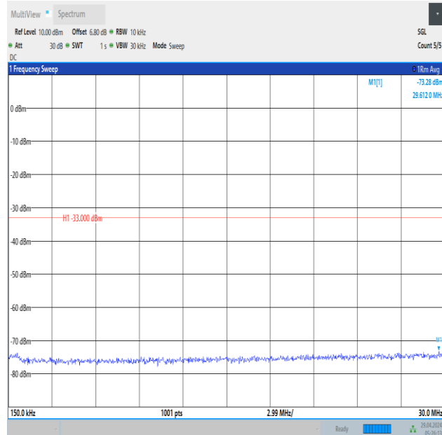
Band66_3MHz_16QAM_131987_1RB#14_0.15~30_0.15~30
