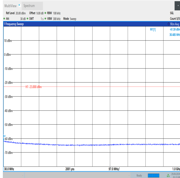
Band66_3MHz_QPSK_132322_15RB#0_30~1000_30~1000
