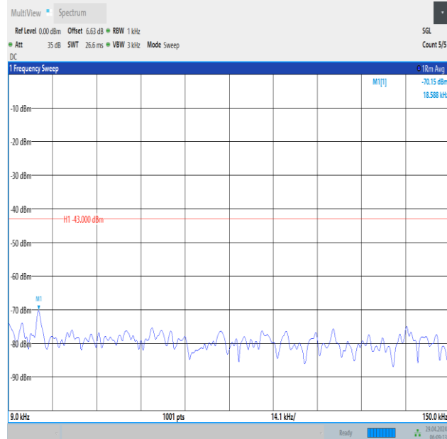
Band66_15MHz_QPSK_132047_1RB#74_0.009~0.15_0.009~0.15
