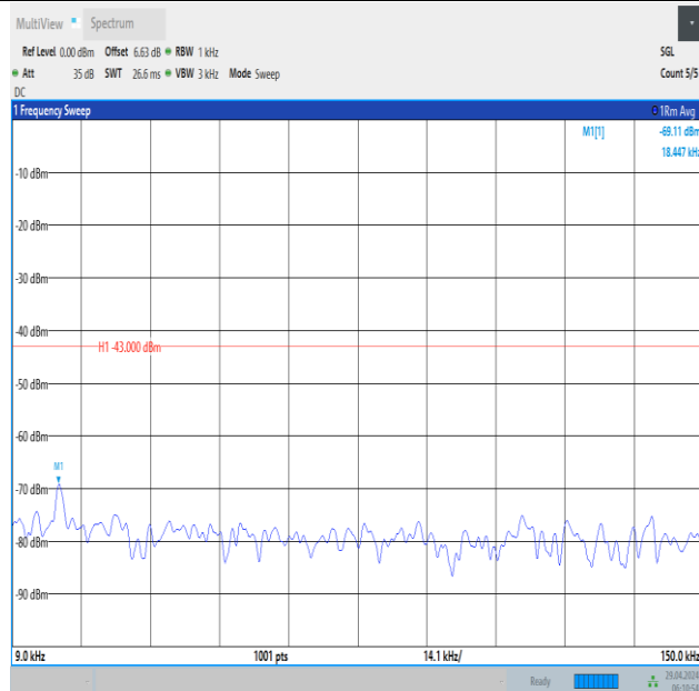
Band66_15MHz_QPSK_132322_1RB#0_0.009~0.15_0.009~0.15
