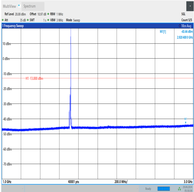
Band66_10MHz_16QAM_132022_1RB#49_1000~3000_1000~3000
