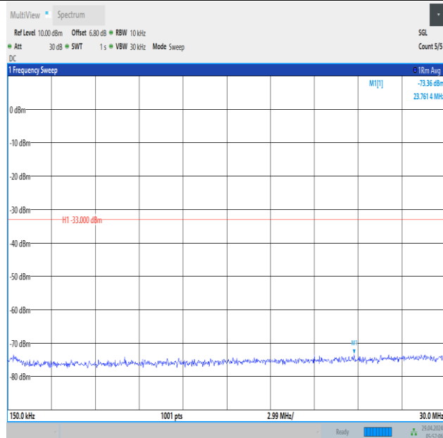
Band66_10MHz_QPSK_132322_1RB#0_0.15~30_0.15~30
