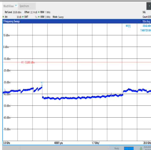
Band66_15MHz_16QAM_132047_1RB#74_3000~20000_3000~20000
