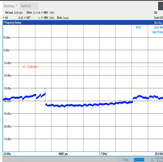
Band66_15MHz_QPSK_132597_1RB#74_3000~20000_3000~20000
