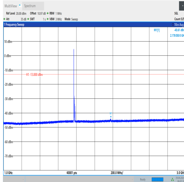
Band66_10MHz_16QAM_132622_1RB#0_1000~3000_1000~3000
