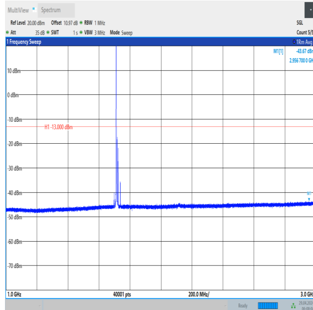
Band66_15MHz_QPSK_132047_1RB#0_1000~3000_1000~3000
