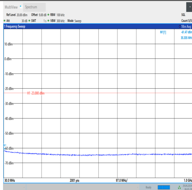
Band66_10MHz_QPSK_132622_50RB#0_30~1000_30~1000
