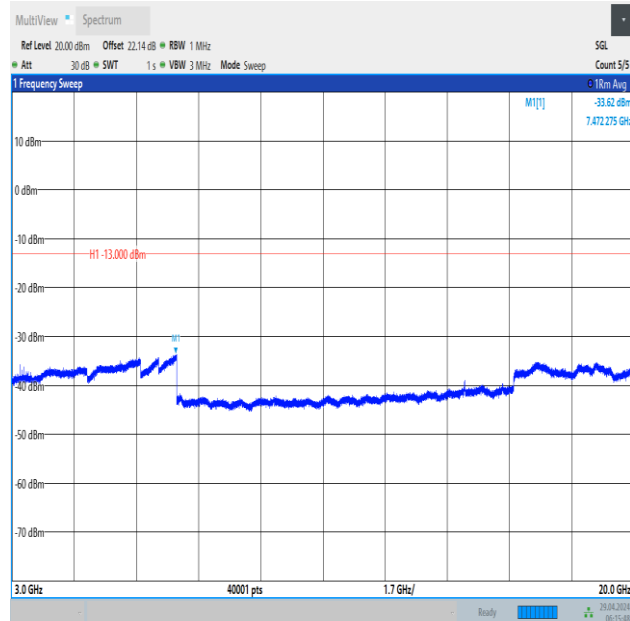
Band66_15MHz_16QAM_132597_1RB#0_3000~20000_3000~20000
