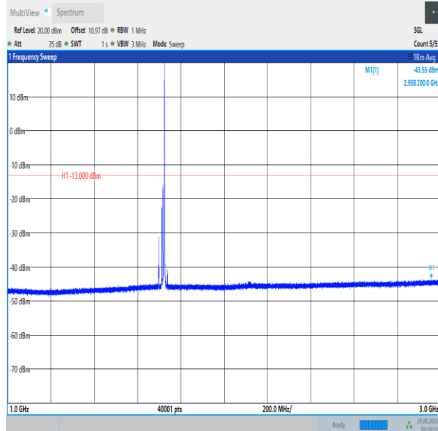
Band66_15MHz_16QAM_132047_1RB#74_1000~3000_1000~3000
