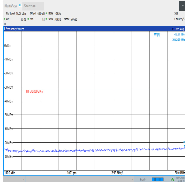
Band66_15MHz_QPSK_132047_1RB#74_0.15~30_0.15~30
