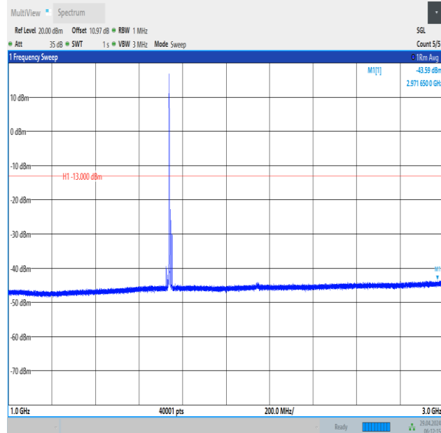
Band66_15MHz_16QAM_132322_1RB#0_1000~3000_1000~3000
