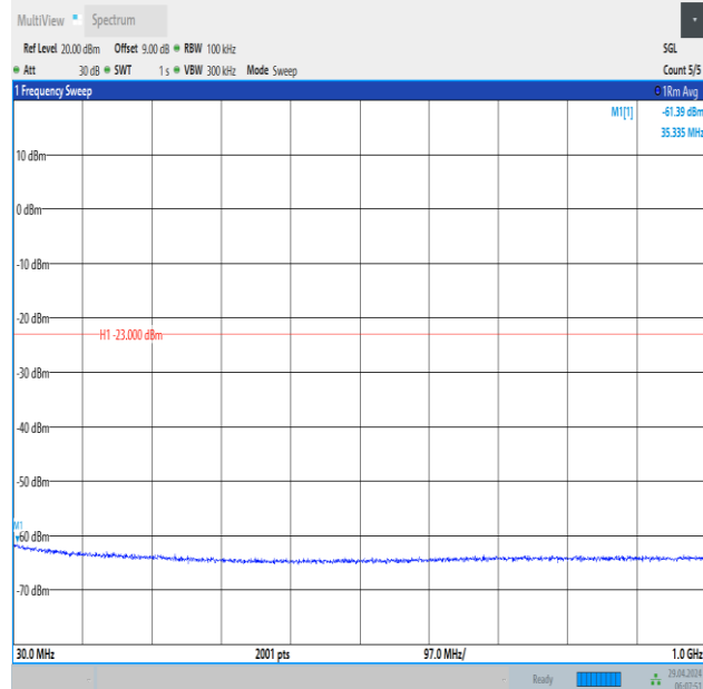
Band66_15MHz_QPSK_132047_1RB#0_30~1000_30~1000
