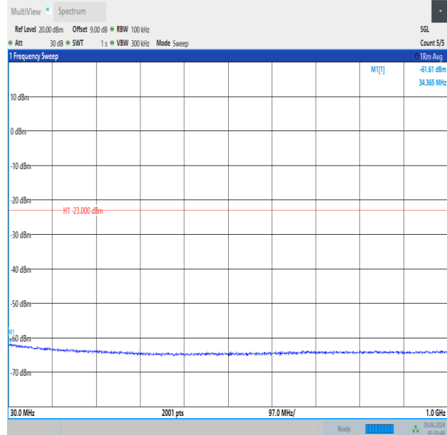
Band66_10MHz_16QAM_132322_1RB#49_30~1000_30~1000
