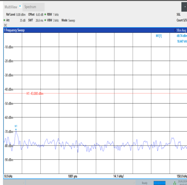
Band66_10MHz_QPSK_132022_50RB#0_0.009~0.15_0.009~0.15
