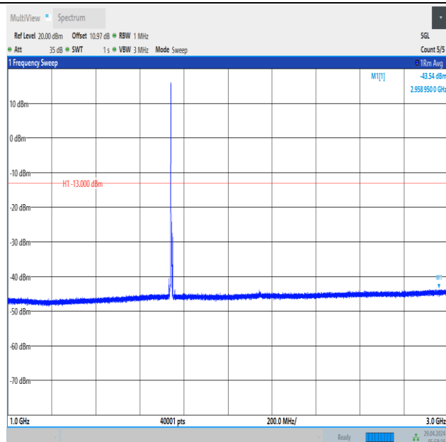
Band66_10MHz_16QAM_132322_1RB#0_1000~3000_1000~3000
