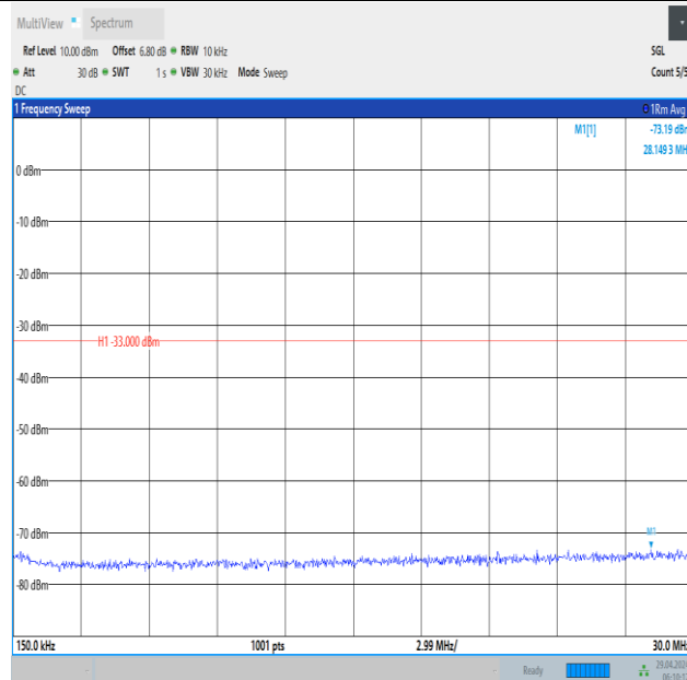
Band66_15MHz_16QAM_132047_1RB#74_0.15~30_0.15~30
