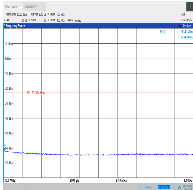
Band66_15MHz_QPSK_132597_1RB#74_30~1000_30~1000
