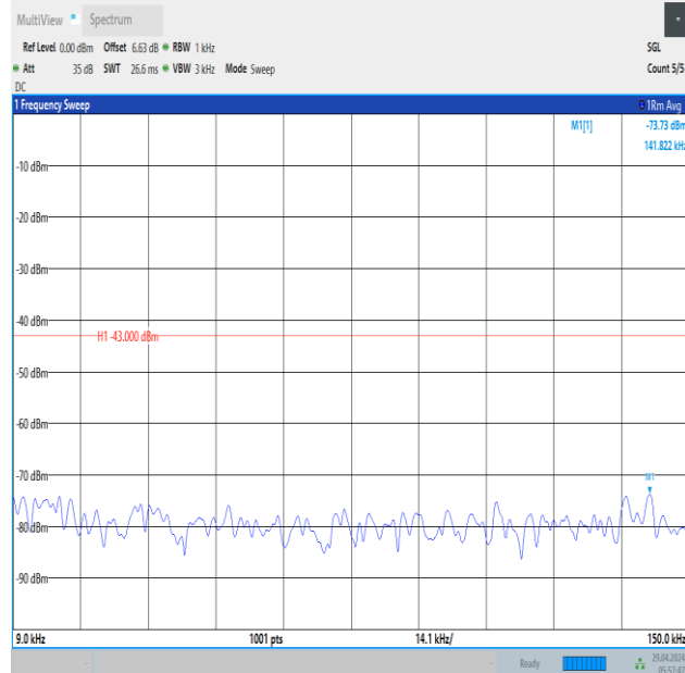
Band66_10MHz_16QAM_132322_1RB#0_0.009~0.15_0.009~0.15
