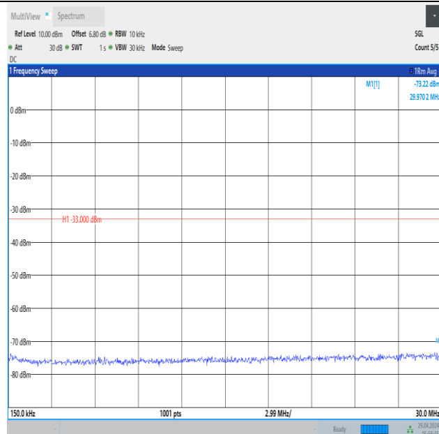
Band66_10MHz_16QAM_132022_1RB#49_0.15~30_0.15~30
