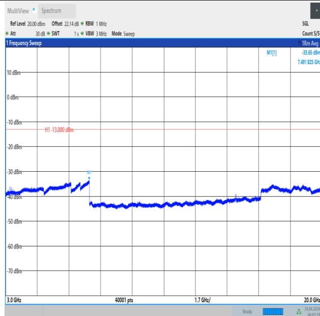
Band66_10MHz_16QAM_132622_1RB#49_3000~20000_3000~20000
