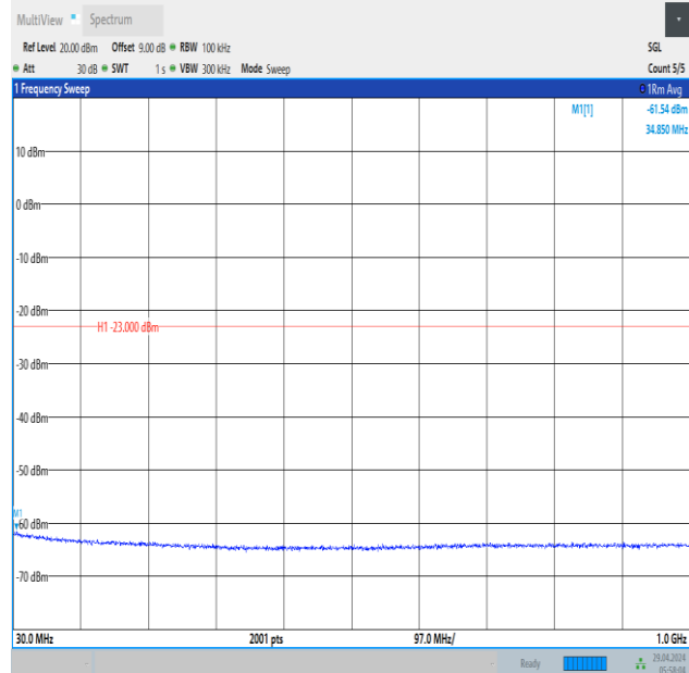
Band66_10MHz_16QAM_132322_1RB#0_30~1000_30~1000
