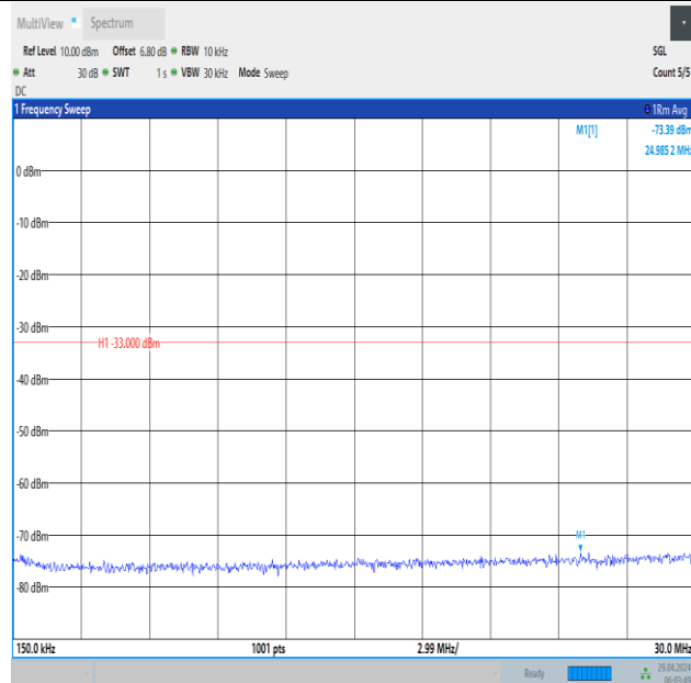
Band66_10MHz_QPSK_132022_50RB#0_0.15~30_0.15~30
