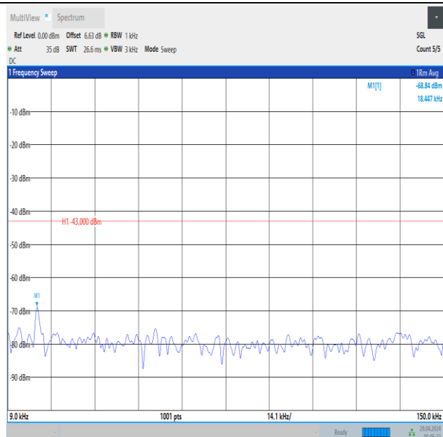
Band66_10MHz_QPSK_132622_50RB#0_0.009~0.15_0.009~0.15
