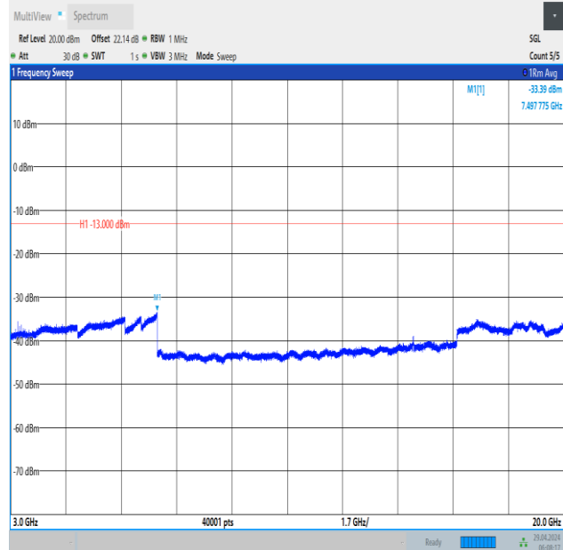
Band66_15MHz_QPSK_132047_1RB#0_3000~20000_3000~20000
