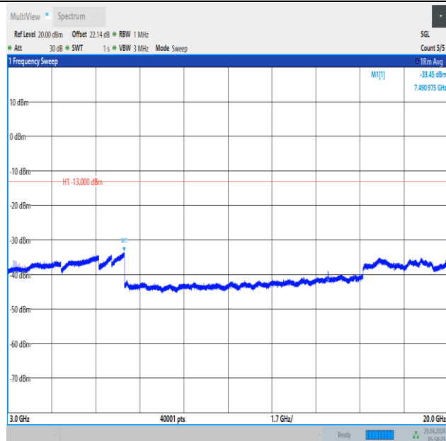
Band66_10MHz_16QAM_132322_1RB#0_3000~20000_3000~20000
