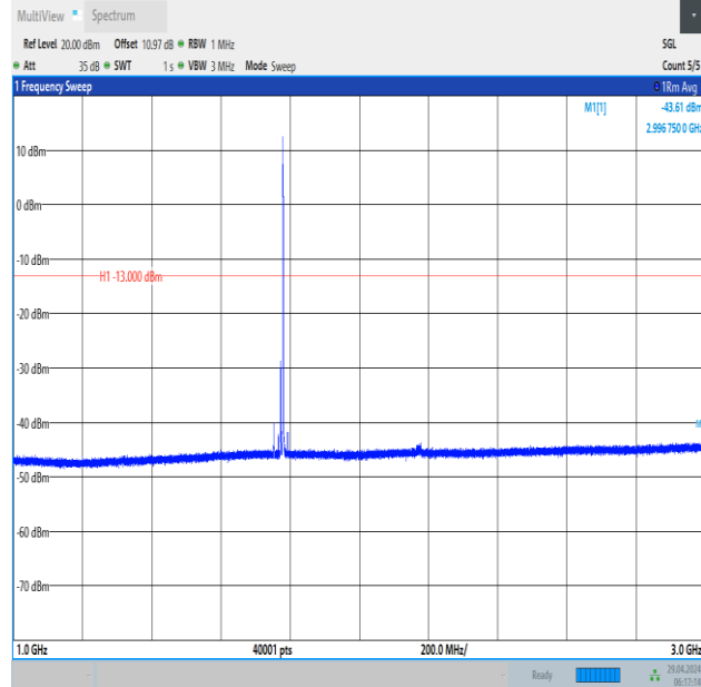
Band66_15MHz_16QAM_132597_1RB#74_1000~3000_1000~3000
