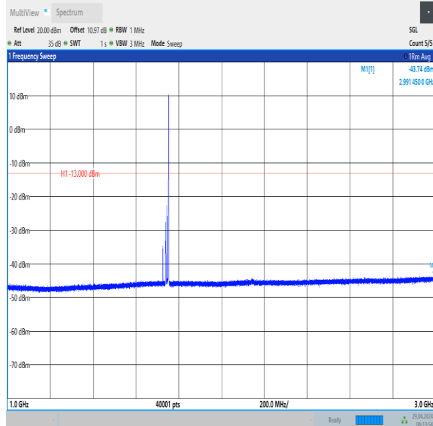
Band66_15MHz_16QAM_132322_1RB#74_1000~3000_1000~3000
