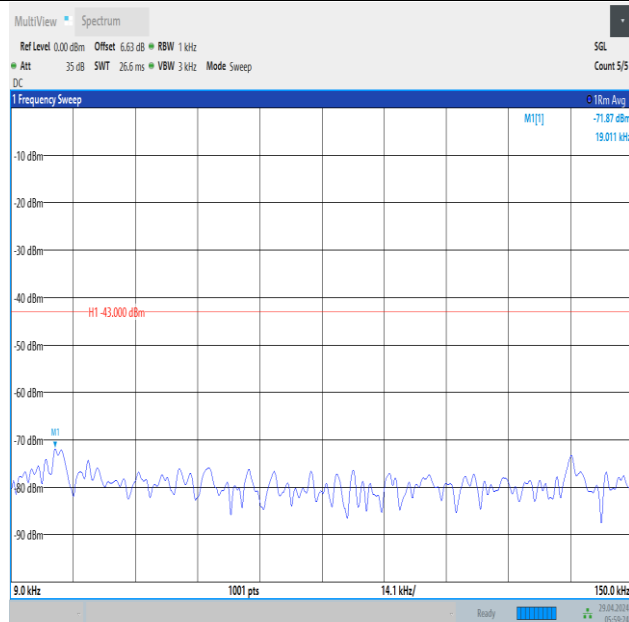
Band66_10MHz_16QAM_132322_1RB#49_0.009~0.15_0.009~0.15
