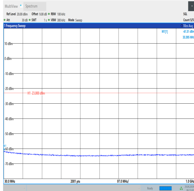
Band66_15MHz_16QAM_132322_1RB#0_30~1000_30~1000
