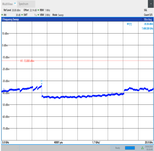
Band66_10MHz_16QAM_132022_1RB#49_3000~20000_3000~20000
