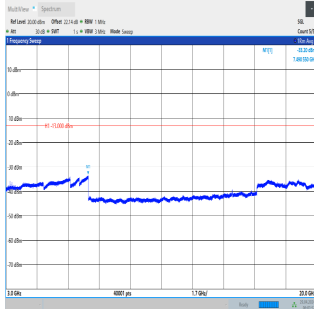
Band66_10MHz_16QAM_132622_1RB#0_3000~20000_3000~20000
