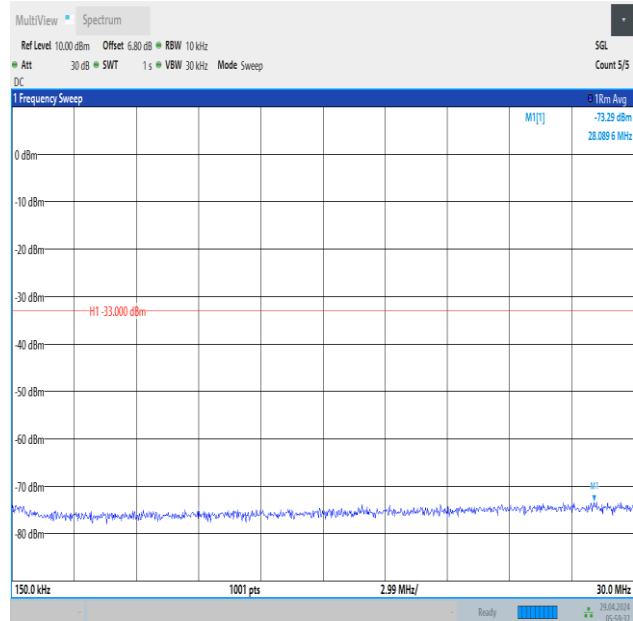
Band66_10MHz_16QAM_132322_1RB#49_0.15~30_0.15~30
