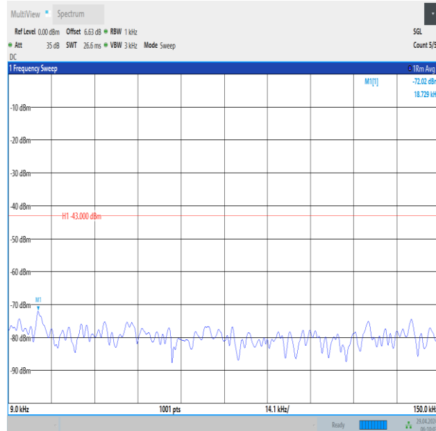
Band66_15MHz_16QAM_132047_1RB#74_0.009~0.15_0.009~0.15
