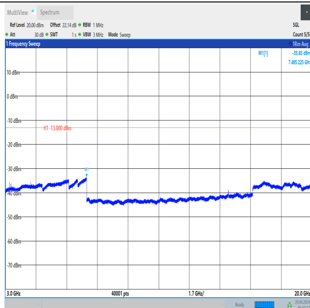
Band66_10MHz_QPSK_132322_1RB#49_3000~20000_3000~20000
