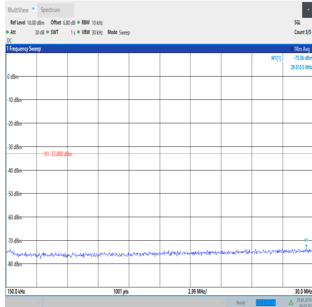
Band66_15MHz_QPSK_132047_1RB#0_0.15~30_0.15~30
