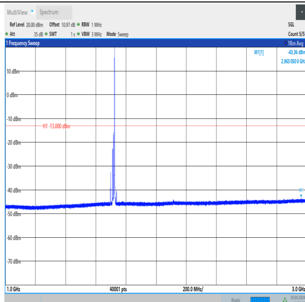
Band66_15MHz_QPSK_132047_1RB#74_1000~3000_1000~3000
