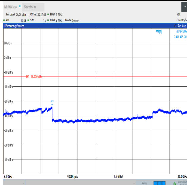
Band66_15MHz_QPSK_132047_1RB#74_3000~20000_3000~20000
