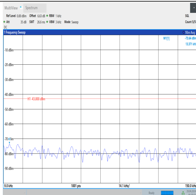
Band66_10MHz_QPSK_132322_1RB#49_0.009~0.15_0.009~0.15
