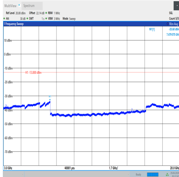
Band66_10MHz_QPSK_132322_1RB#0_3000~20000_3000~20000
