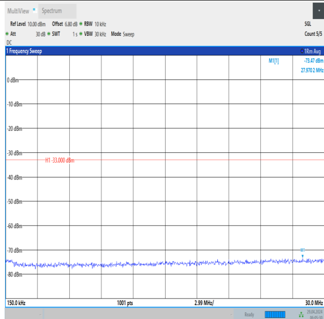
Band66_10MHz_QPSK_132622_50RB#0_0.15~30_0.15~30
