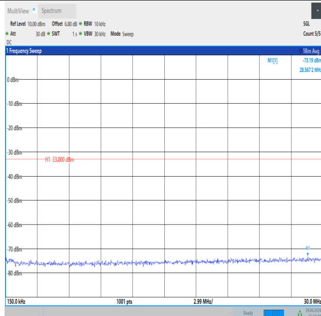
Band66_10MHz_QPSK_132322_1RB#49_0.15~30_0.15~30
