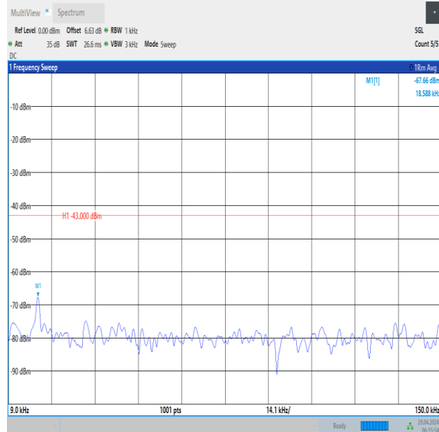
Band66_15MHz_QPSK_132597_1RB#74_0.009~0.15_0.009~0.15
