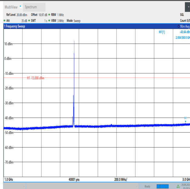
Band66_10MHz_16QAM_132322_1RB#49_1000~3000_1000~3000
