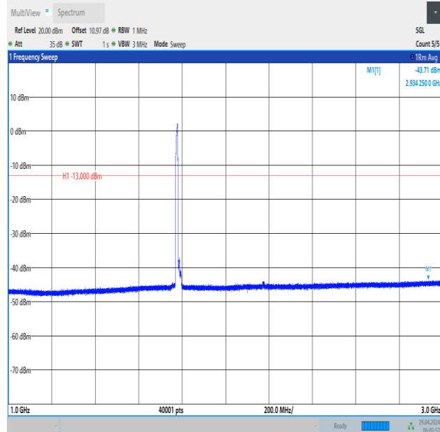
Band66_10MHz_QPSK_132622_50RB#0_1000~3000_1000~3000
