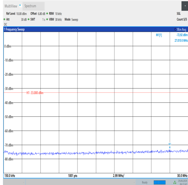
Band66_15MHz_QPSK_132322_1RB#74_0.15~30_0.15~30
