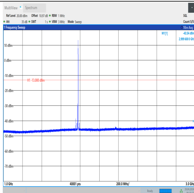
Band66_15MHz_QPSK_132597_1RB#74_1000~3000_1000~3000
