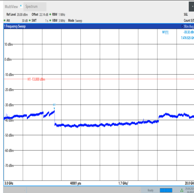
Band66_10MHz_16QAM_132322_1RB#49_3000~20000_3000~20000
