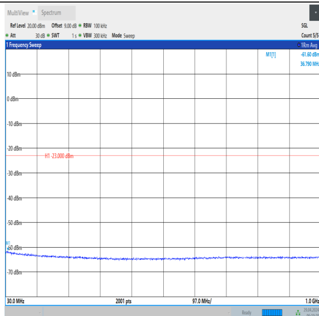
Band66_15MHz_16QAM_132047_1RB#74_30~1000_30~1000
