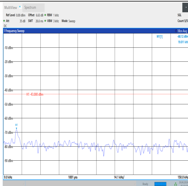
Band66_10MHz_QPSK_132322_1RB#0_0.009~0.15_0.009~0.15
