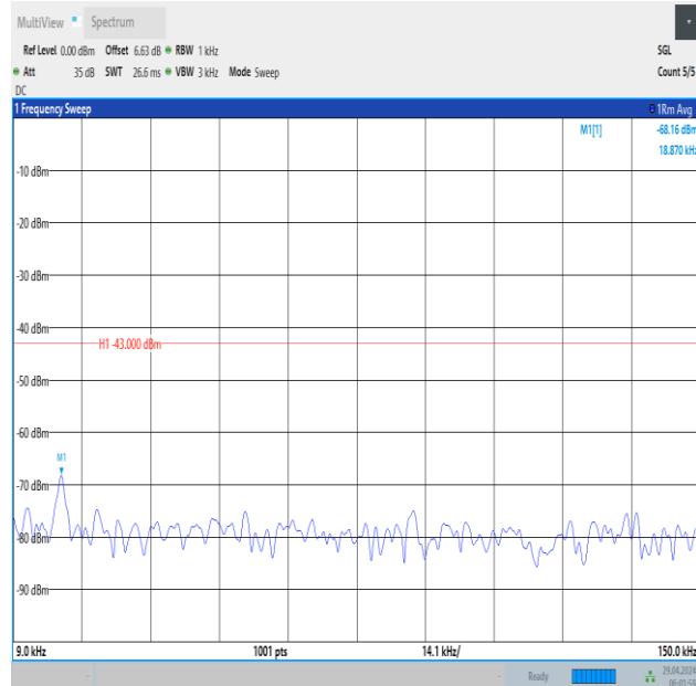
Band66_10MHz_QPSK_132622_1RB#49_0.009~0.15_0.009~0.15
