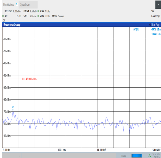
Band66_15MHz_QPSK_132322_1RB#74_0.009~0.15_0.009~0.15
