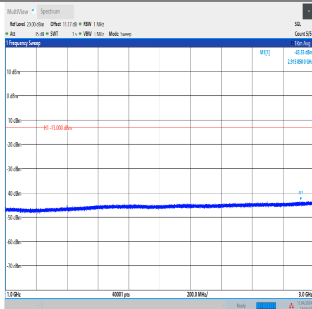
Band12_3MHz_16QAM_23025_1RB#0_1000~3000_1000~3000
