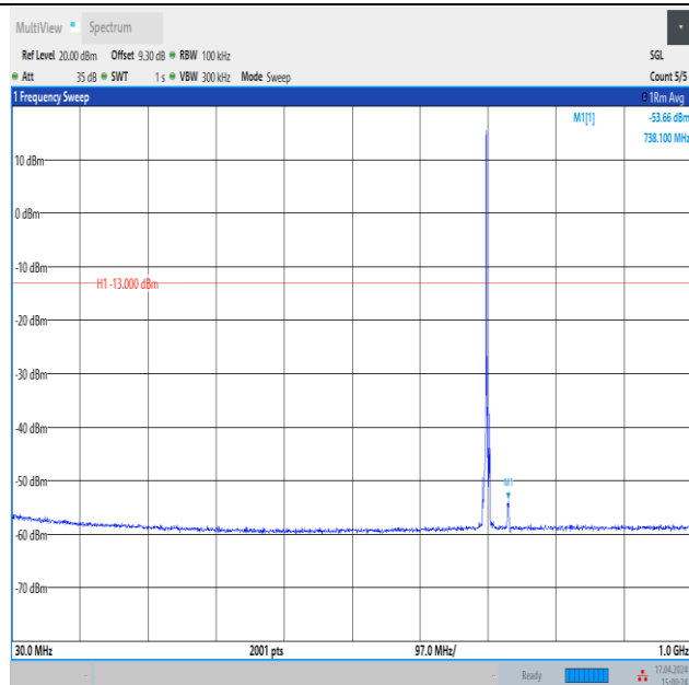
Band12_3MHz_QPSK_23095_1RB#0_30~1000_30~1000
