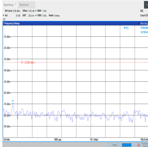
Band12_5MHz_QPSK_23155_1RB#0_0.009~0.15_0.009~0.15
