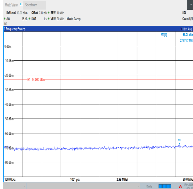
Band12_3MHz_QPSK_23025_1RB#0_0.15~30_0.15~30
