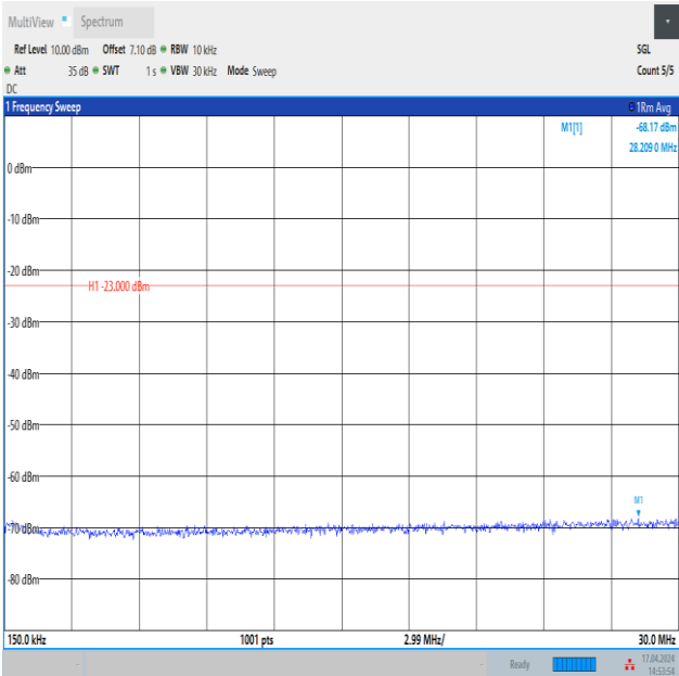
Band12_5MHz_16QAM_23155_25RB#0_0.15~30_0.15~30
