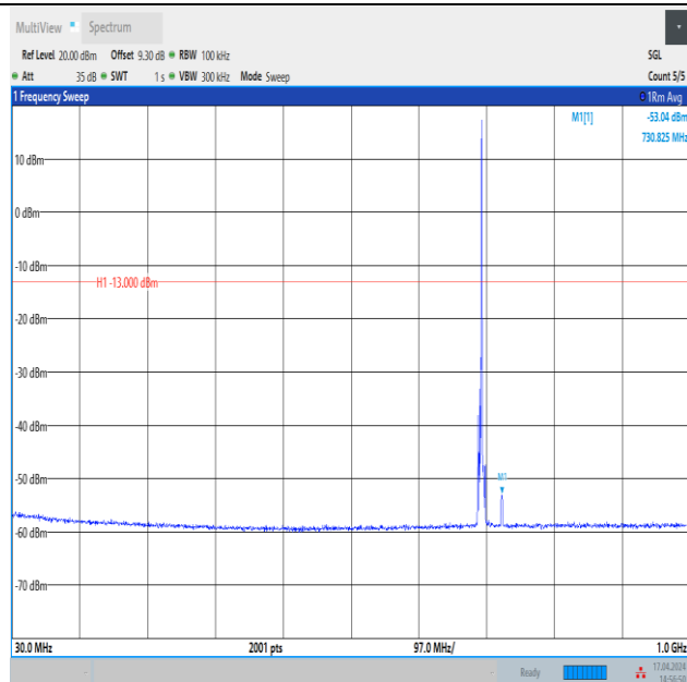
Band12_3MHz_QPSK_23025_1RB#14_30~1000_30~1000
