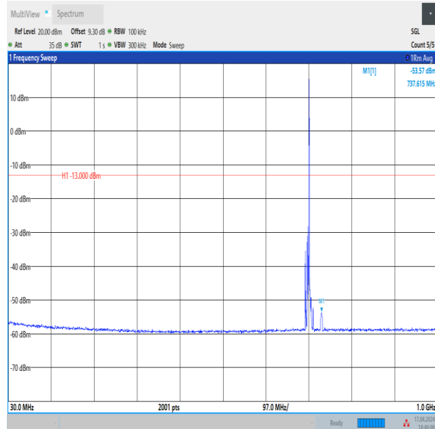
Band12_5MHz_QPSK_23095_1RB#24_30~1000_30~1000
