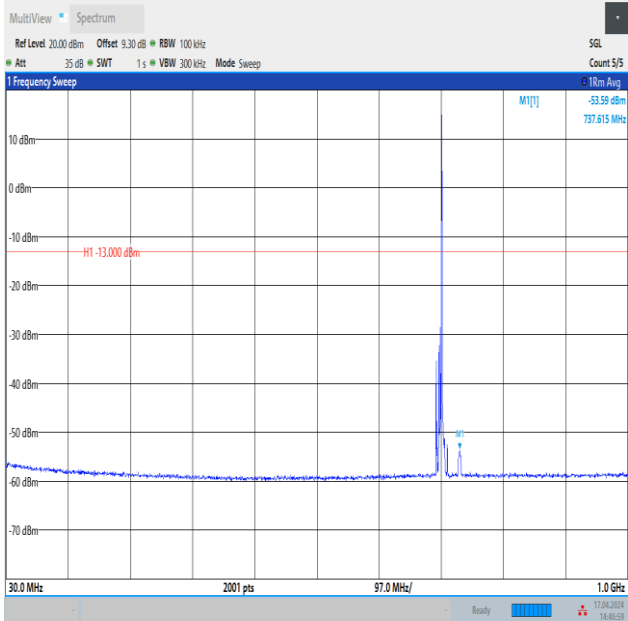
Band12_5MHz_16QAM_23095_1RB#24_30~1000_30~1000
