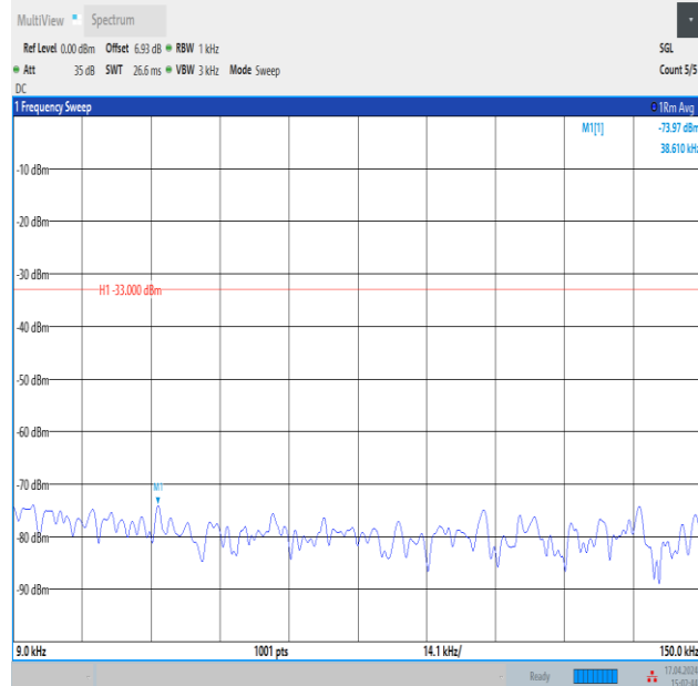
Band12_3MHz_16QAM_23095_1RB#14_0.009~0.15_0.009~0.15
