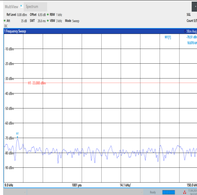
Band12_5MHz_16QAM_23155_1RB#24_0.009~0.15_0.009~0.15
