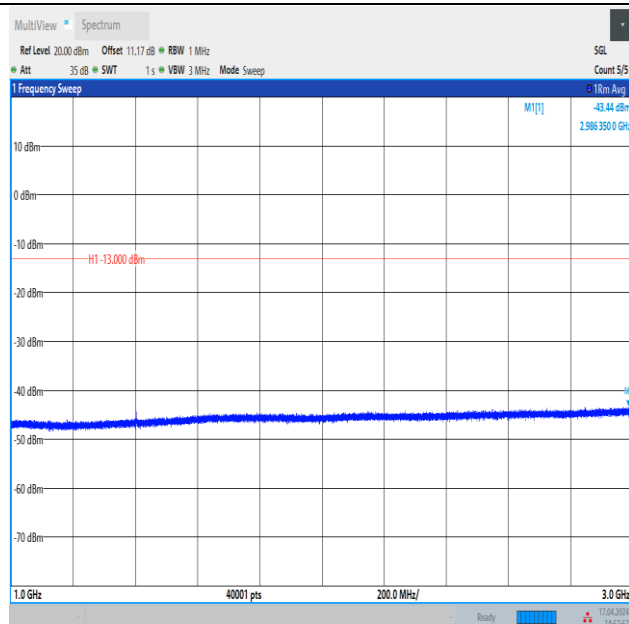
Band12_3MHz_16QAM_23025_1RB#14_1000~3000_1000~3000
