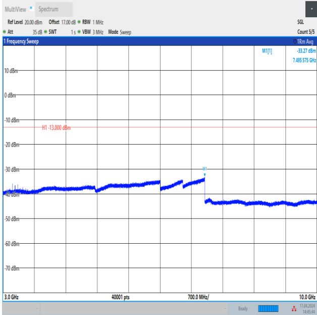
Band12_5MHz_16QAM_23095_1RB#0_3000~10000_3000~10000
