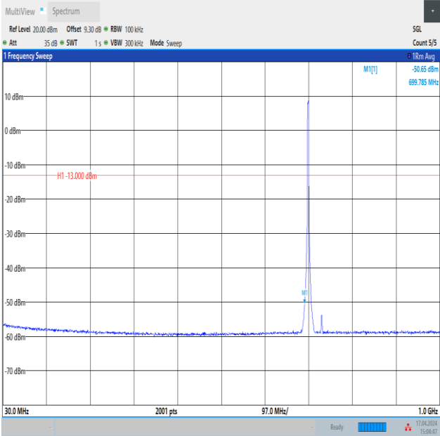
Band12_3MHz_16QAM_23095_15RB#0_30~1000_30~1000
