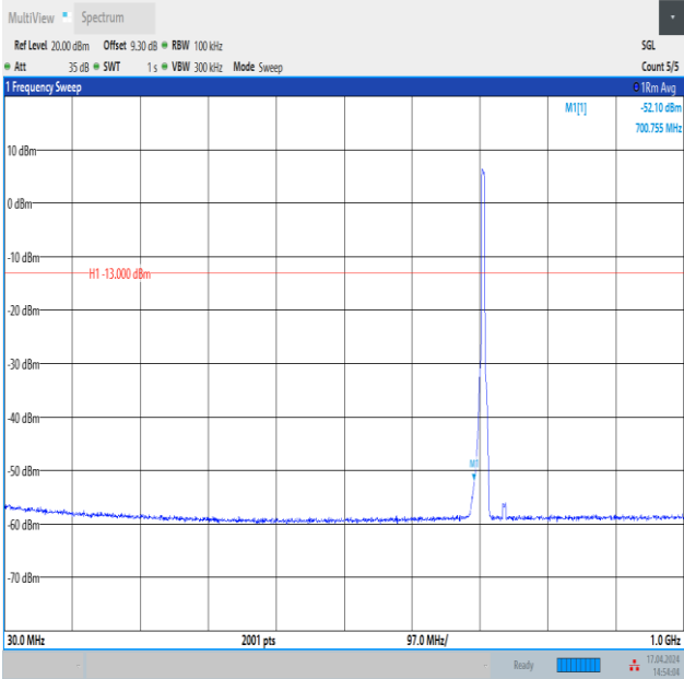
Band12_5MHz_16QAM_23155_25RB#0_30~1000_30~1000
