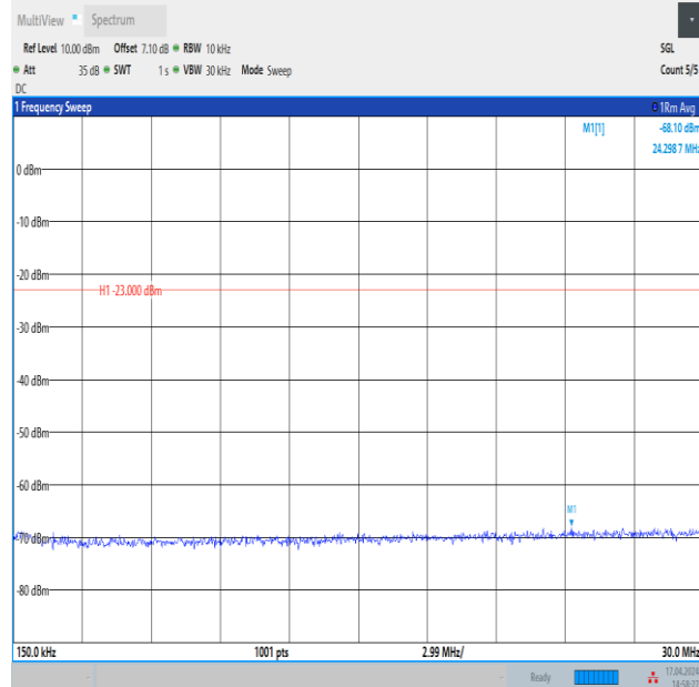
Band12_3MHz_QPSK_23025_15RB#0_0.15~30_0.15~30
