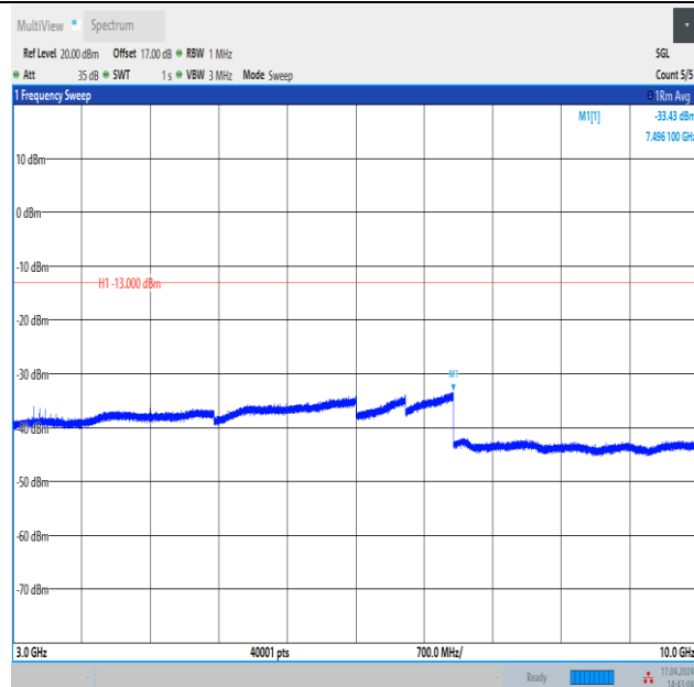
Band12_5MHz_QPSK_23035_25RB#0_3000~10000_3000~10000
