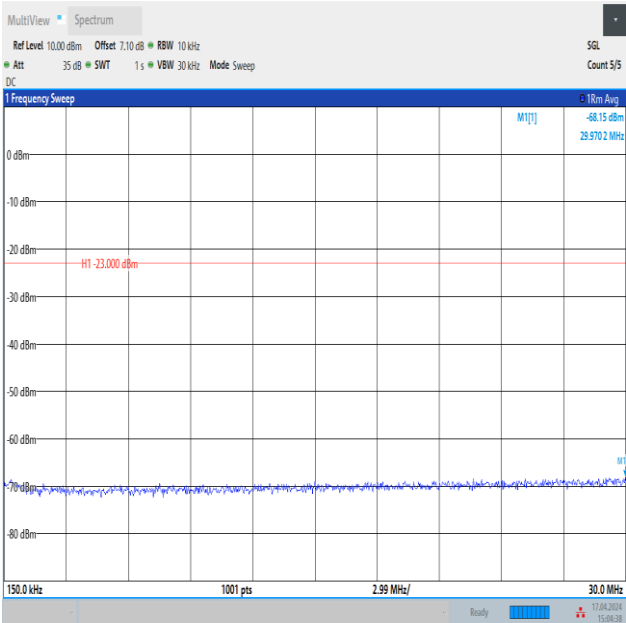
Band12_3MHz_16QAM_23095_15RB#0_0.15~30_0.15~30
