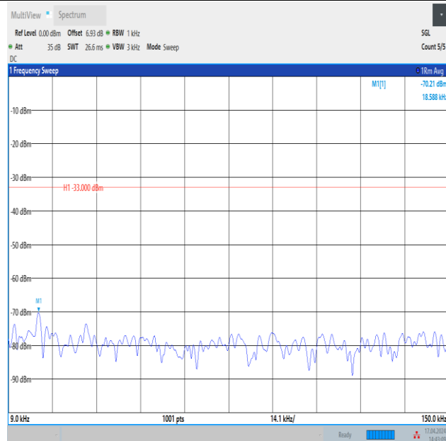
Band12_5MHz_16QAM_23035_25RB#0_0.009~0.15_0.009~0.15
