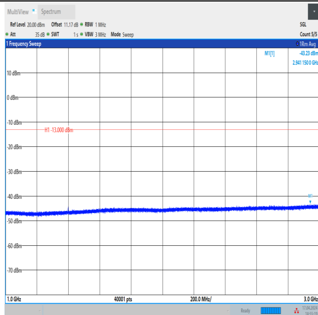
Band12_3MHz_QPSK_23025_1RB#0_1000~3000_1000~3000
