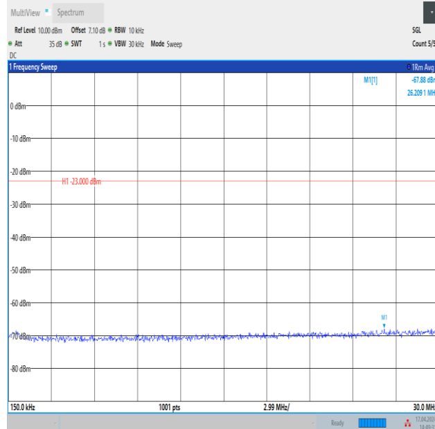
Band12_5MHz_QPSK_23155_1RB#0_0.15~30_0.15~30
