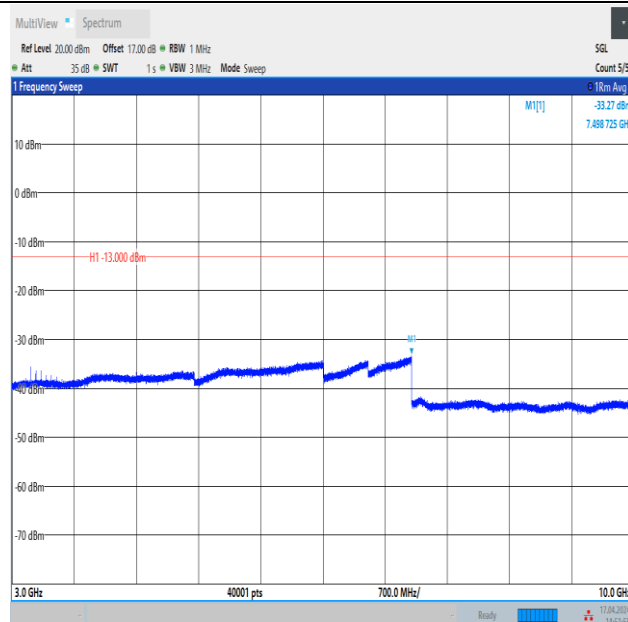
Band12_5MHz_QPSK_23155_1RB#24_3000~10000_3000~10000
