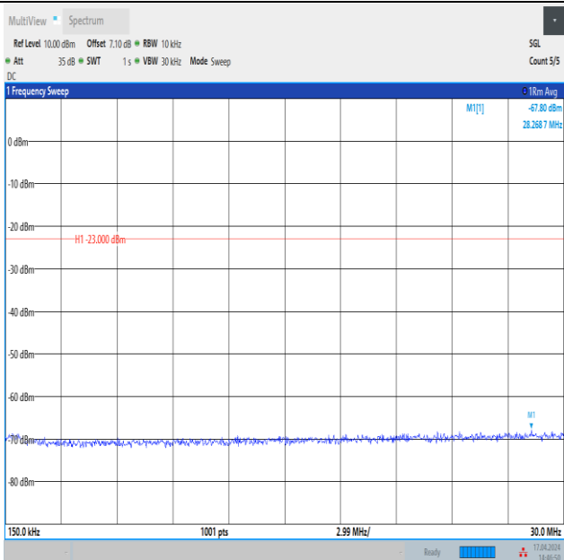
Band12_5MHz_16QAM_23095_1RB#24_0.15~30_0.15~30
