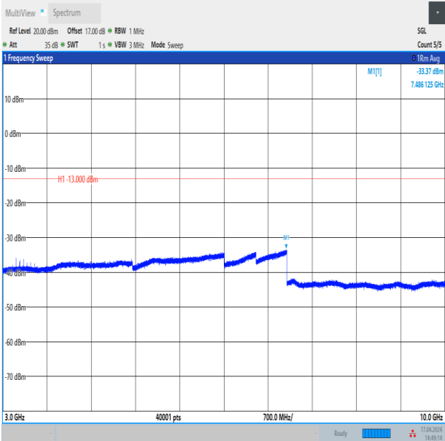
Band12_5MHz_16QAM_23095_25RB#0_3000~10000_3000~10000
