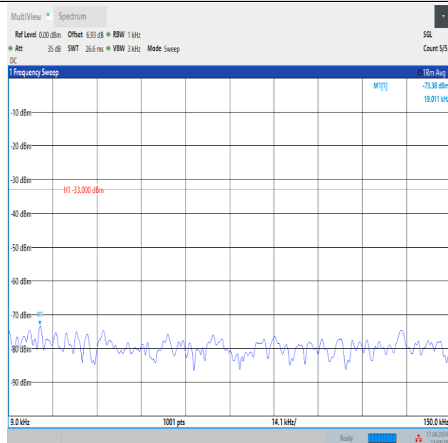
Band12_3MHz_QPSK_23025_15RB#0_0.009~0.15_0.009~0.15
