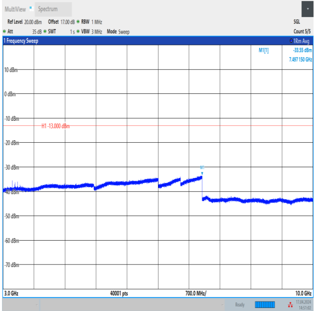
Band12_5MHz_16QAM_23155_1RB#0_3000~10000_3000~10000
