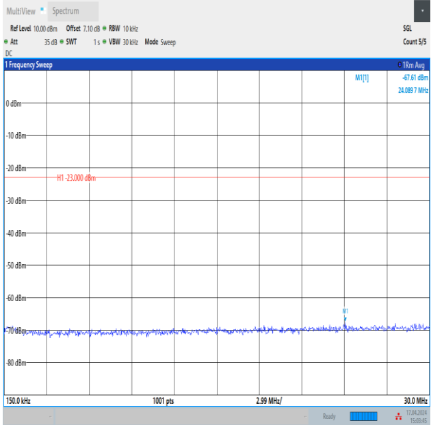
Band12_3MHz_QPSK_23095_15RB#0_0.15~30_0.15~30
