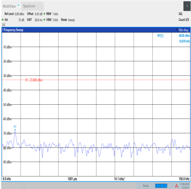
Band12_3MHz_QPSK_23095_15RB#0_0.009~0.15_0.009~0.15
