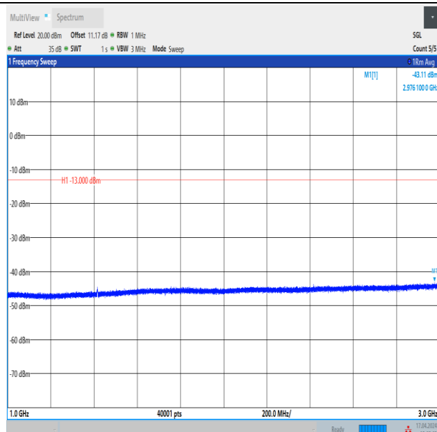
Band12_3MHz_16QAM_23095_15RB#0_1000~3000_1000~3000
