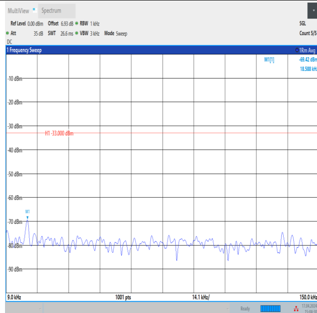
Band12_3MHz_16QAM_23095_15RB#0_0.009~0.15_0.009~0.15
