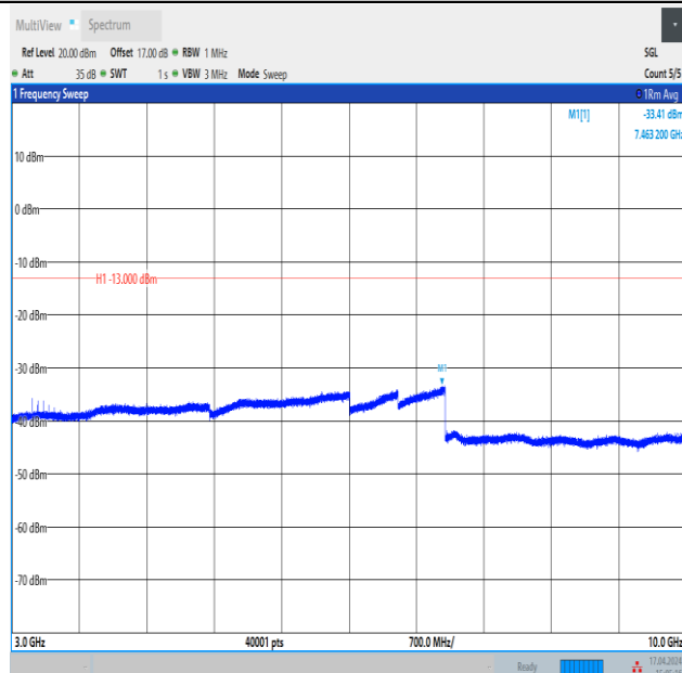
Band12_3MHz_16QAM_23095_15RB#0_3000~10000_3000~10000
