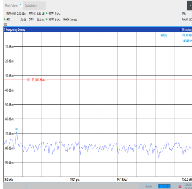
Band12_3MHz_16QAM_23025_1RB#0_0.009~0.15_0.009~0.15
