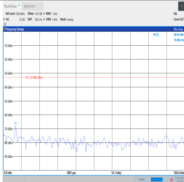
Band12_3MHz_16QAM_23025_15RB#0_0.009~0.15_0.009~0.15
