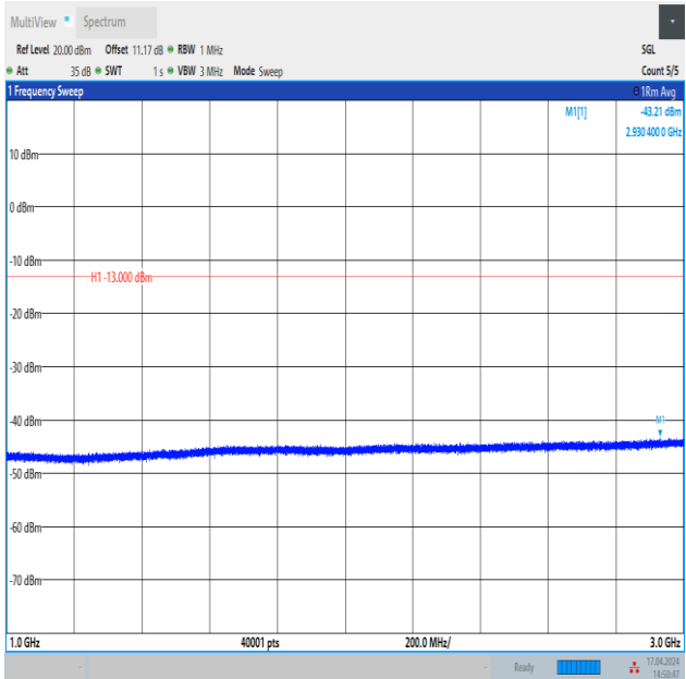
Band12_5MHz_16QAM_23155_1RB#0_1000~3000_1000~3000
