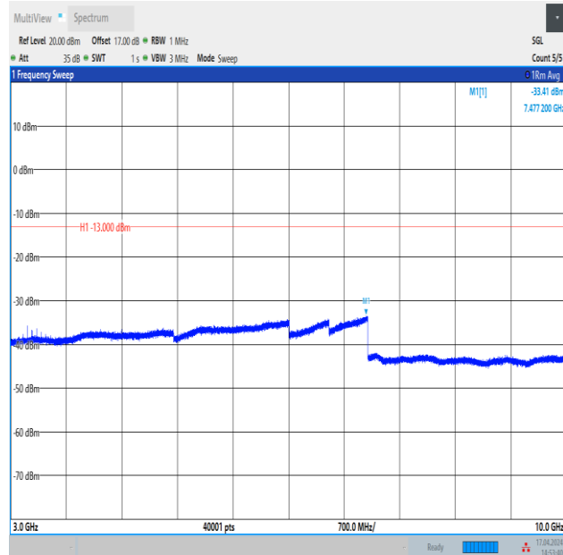
Band12_5MHz_QPSK_23155_25RB#0_3000~10000_3000~10000
