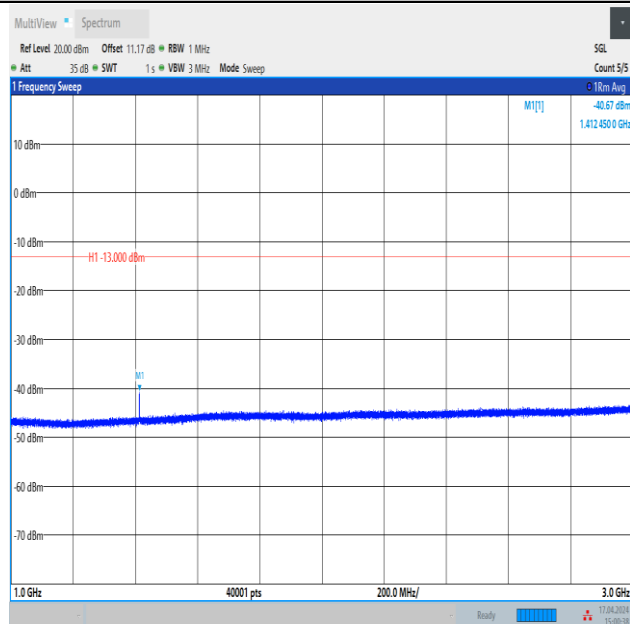
Band12_3MHz_QPSK_23095_1RB#0_1000~3000_1000~3000
