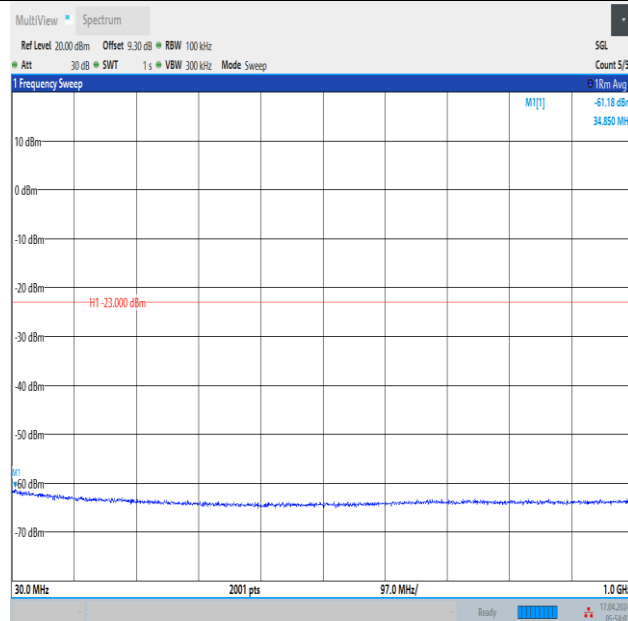
Band2_3MHz_QPSK_19185_15RB#0_30~1000_30~1000
