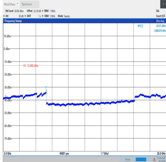
Band2_3MHz_16QAM_18900_15RB#0_3000~20000_3000~20000
