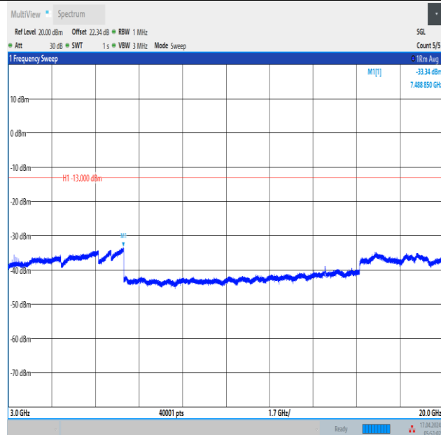
Band2_3MHz_QPSK_19185_1RB#0_3000~20000_3000~20000
