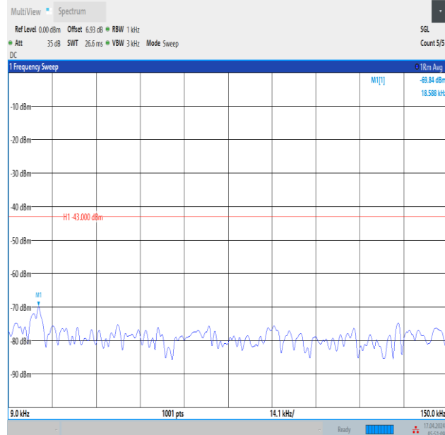
Band2_3MHz_16QAM_19185_1RB#0_0.009~0.15_0.009~0.15
