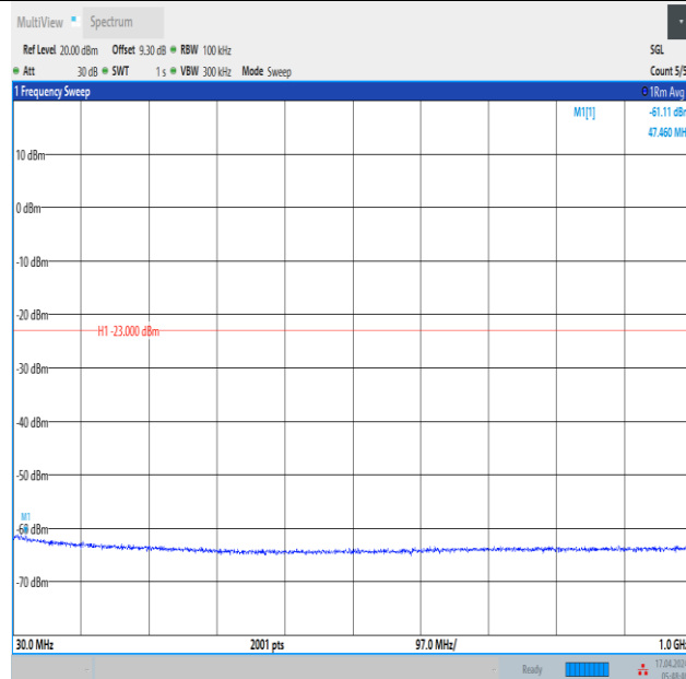
Band2_3MHz_QPSK_18900_15RB#0_30~1000_30~1000
