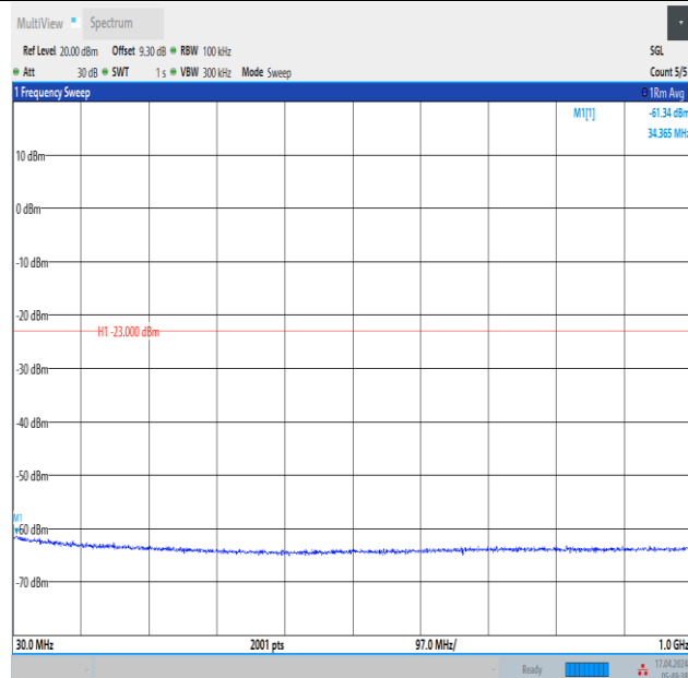
Band2_3MHz_16QAM_18900_15RB#0_30~1000_30~1000
