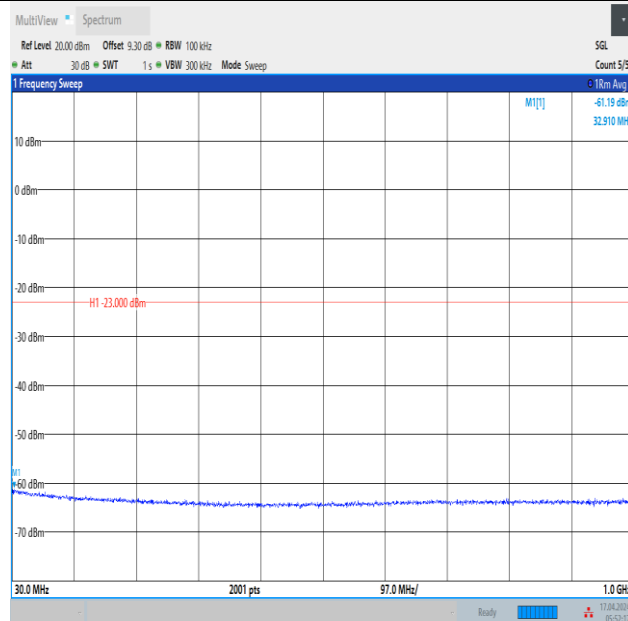
Band2_3MHz_QPSK_19185_1RB#14_30~1000_30~1000
