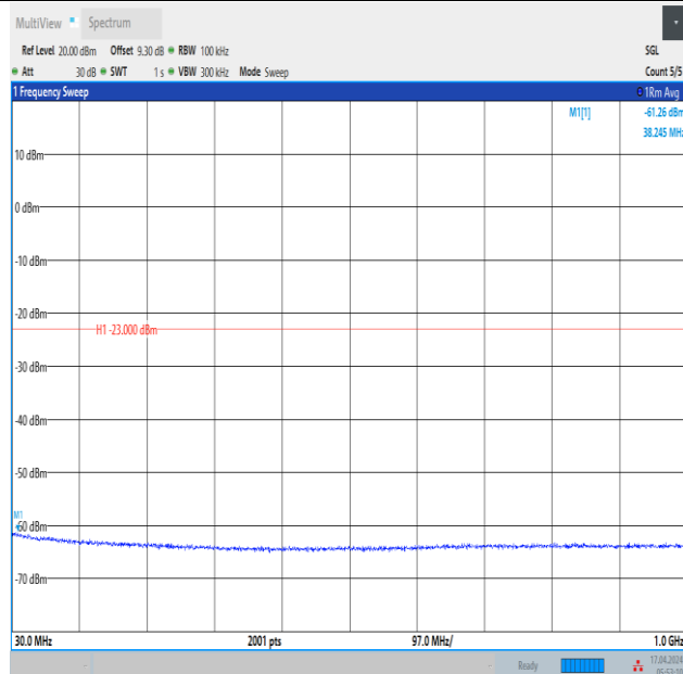
Band2_3MHz_16QAM_19185_1RB#14_30~1000_30~1000
