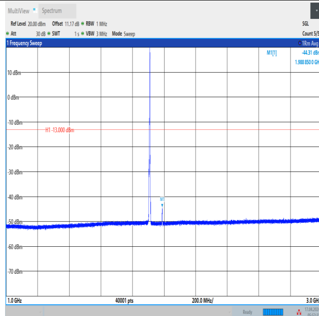
Band2_3MHz_QPSK_19185_1RB#14_1000~3000_1000~3000
