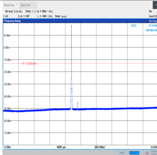
Band2_3MHz_16QAM_18900_15RB#0_1000~3000_1000~3000
