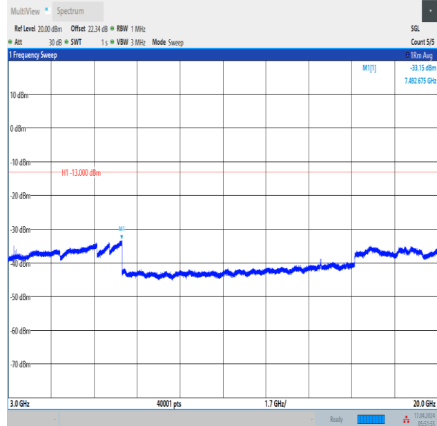
Band2_3MHz_16QAM_19185_1RB#0_3000~20000_3000~20000
