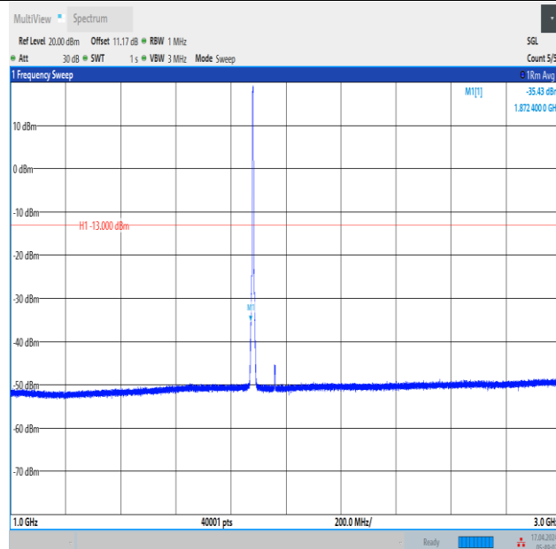
Band2_3MHz_QPSK_18900_15RB#0_1000~3000_1000~3000
