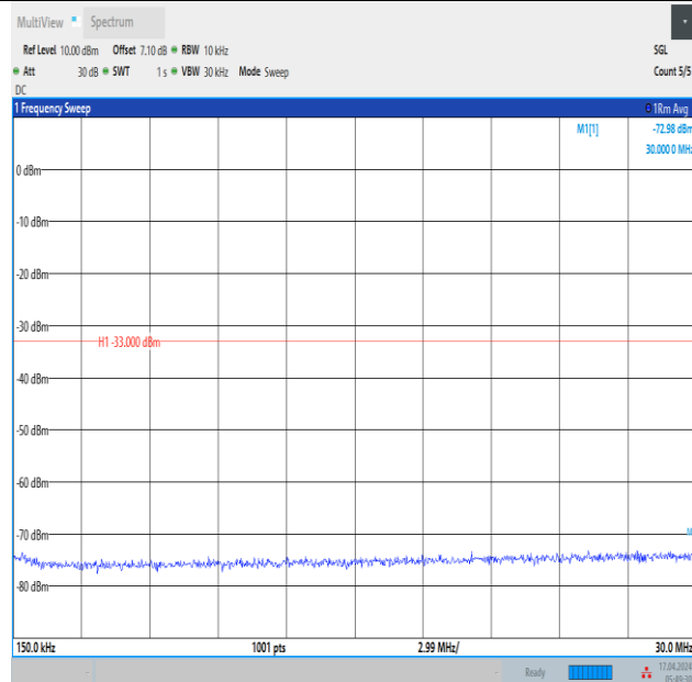
Band2_3MHz_16QAM_18900_15RB#0_0.15~30_0.15~30
