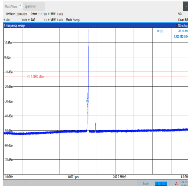
Band2_3MHz_QPSK_19185_15RB#0_1000~3000_1000~3000
