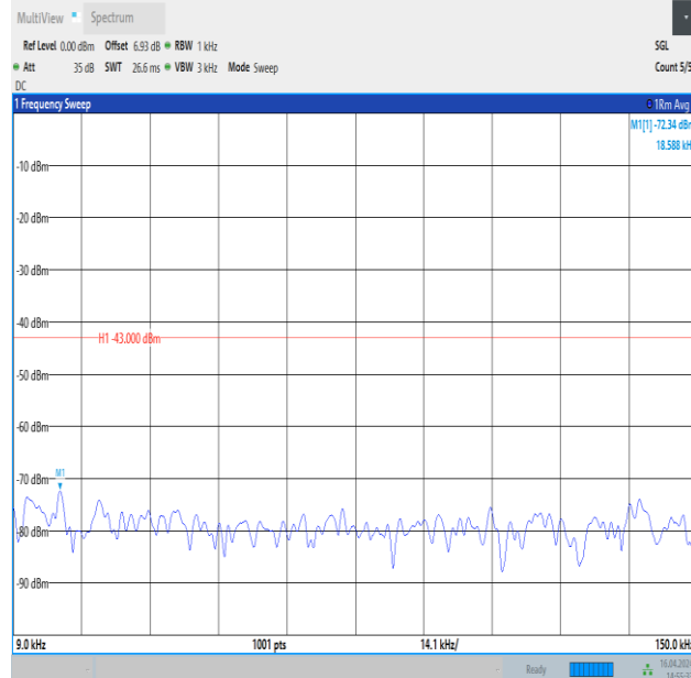
Band4_10MHz_QPSK_20000_1RB#0_0.009~0.15_0.009~0.15
