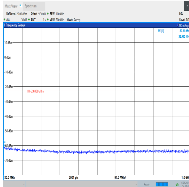
Band4_10MHz_QPSK_20350_50RB#0_30~1000_30~1000
