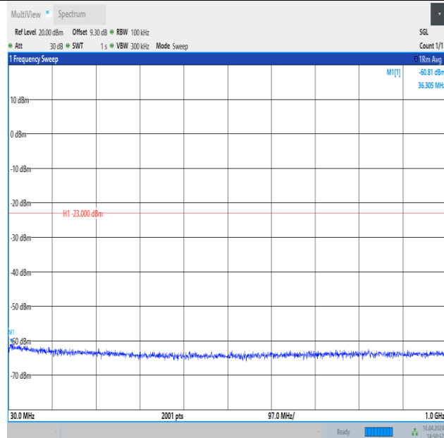
Band4_10MHz_QPSK_20000_50RB#0_30~1000_30~1000
