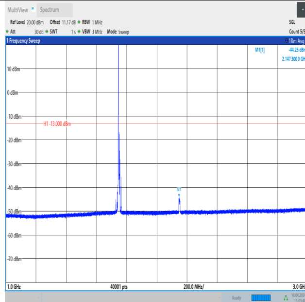
Band4_10MHz_QPSK_20350_1RB#0_1000~3000_1000~3000
