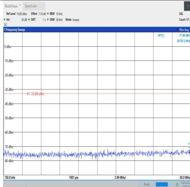
Band4_15MHz_16QAM_20175_1RB#74_0.15~30_0.15~30
