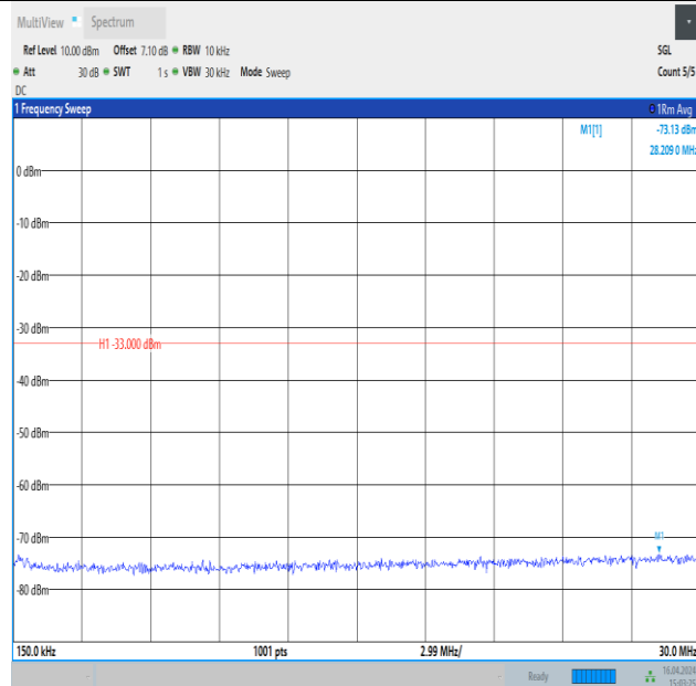
Band4_10MHz_QPSK_20350_1RB#0_0.15~30_0.15~30
