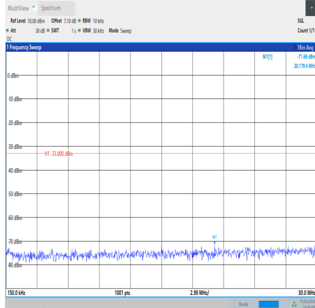
Band4_15MHz_QPSK_20175_1RB#0_0.15~30_0.15~30
