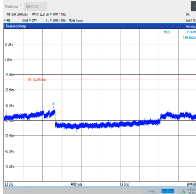
Band4_15MHz_QPSK_20175_1RB#74_3000~20000_3000~20000
