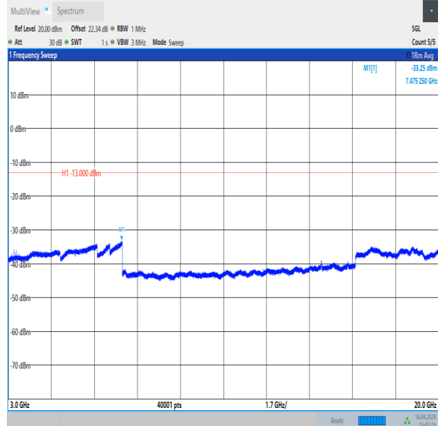
Band4_10MHz_QPSK_20175_1RB#49_3000~20000_3000~20000
