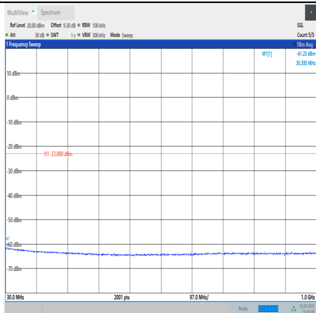
Band4_10MHz_16QAM_20000_1RB#49_30~1000_30~1000
