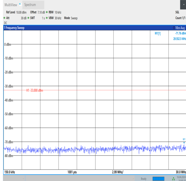
Band4_15MHz_QPSK_20325_1RB#0_0.15~30_0.15~30
