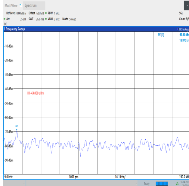
Band4_10MHz_QPSK_20175_1RB#49_0.009~0.15_0.009~0.15
