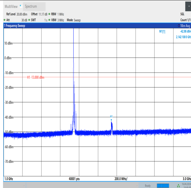
Band4_15MHz_QPSK_20325_1RB#0_1000~3000_1000~3000
