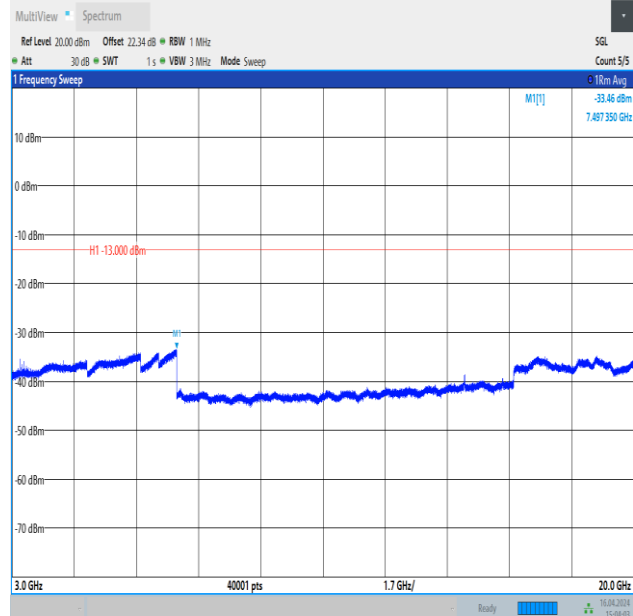
Band4_10MHz_QPSK_20350_1RB#0_3000~20000_3000~20000
