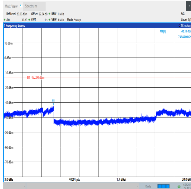
Band4_15MHz_QPSK_20325_1RB#0_3000~20000_3000~20000
