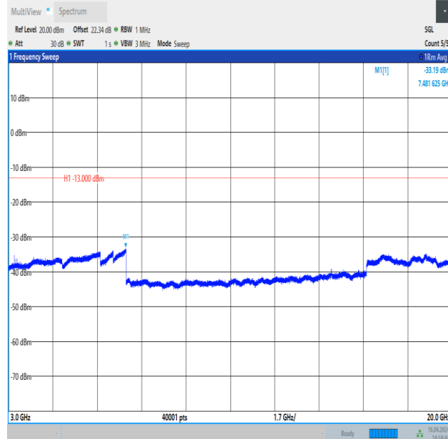
Band4_10MHz_QPSK_20000_1RB#49_3000~20000_3000~20000
