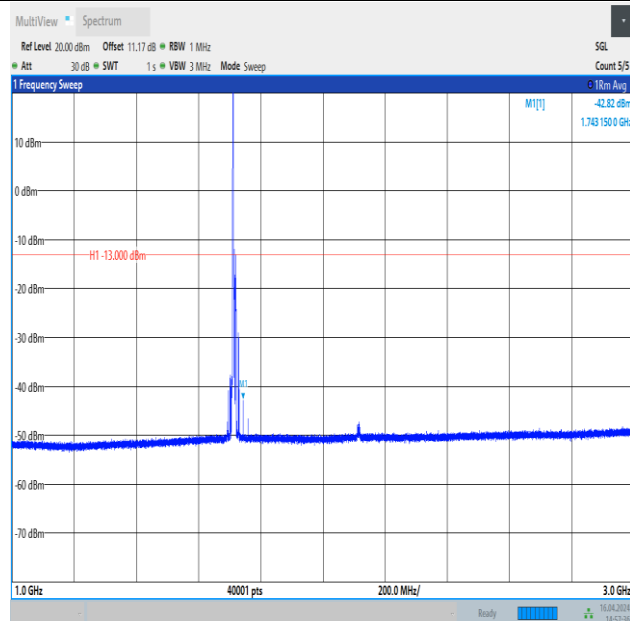
Band4_10MHz_16QAM_20000_1RB#0_1000~3000_1000~3000
