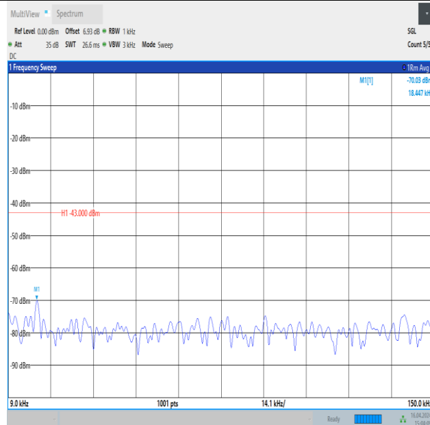
Band4_10MHz_16QAM_20350_1RB#0_0.009~0.15_0.009~0.15
