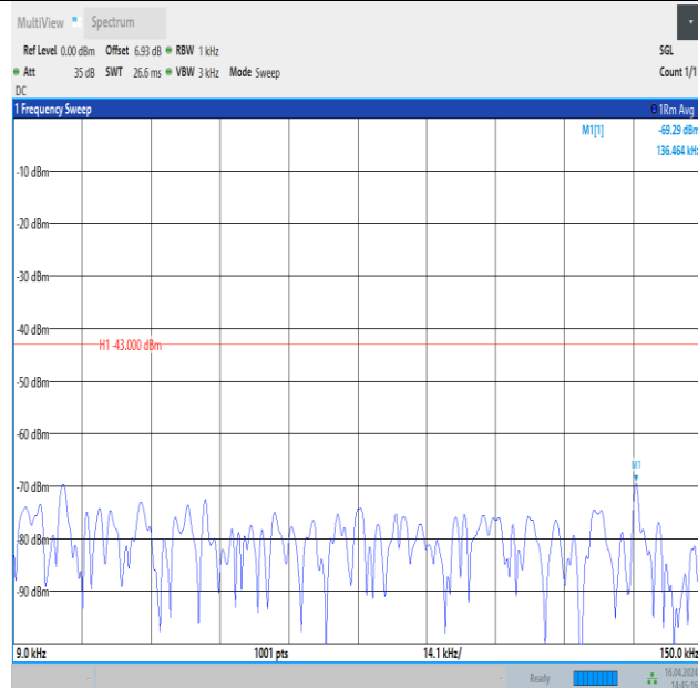
Band4_15MHz_QPSK_20175_1RB#74_0.009~0.15_0.009~0.15
