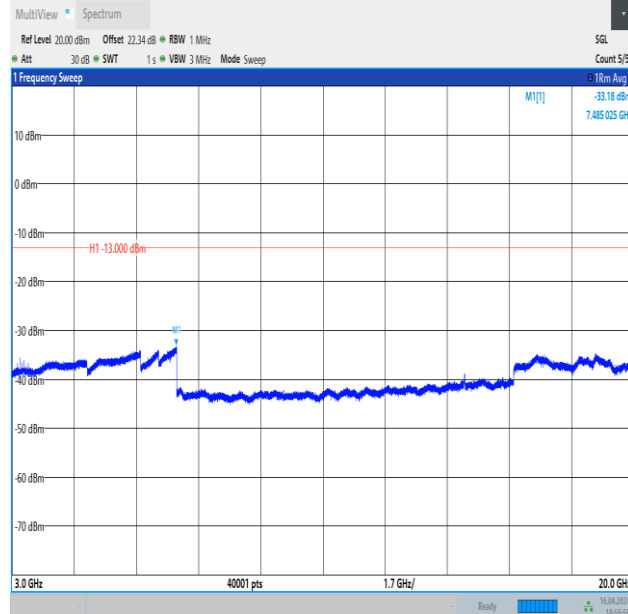
Band4_10MHz_QPSK_20000_1RB#0_3000~20000_3000~20000
