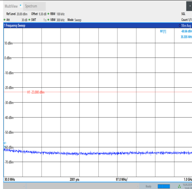
Band4_15MHz_QPSK_20325_1RB#0_30~1000_30~1000
