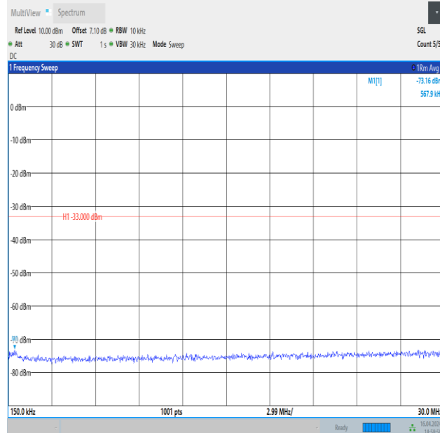
Band4_10MHz_16QAM_20000_1RB#49_0.15~30_0.15~30
