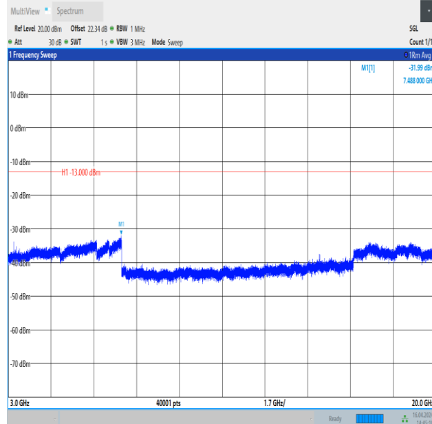
Band4_15MHz_16QAM_20175_1RB#0_3000~20000_3000~20000
