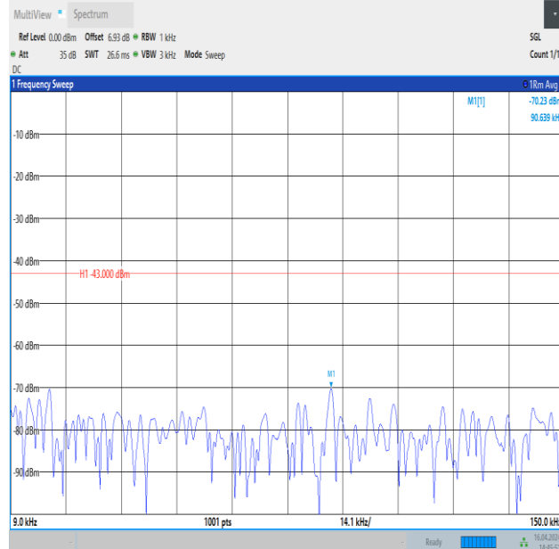
Band4_15MHz_16QAM_20175_1RB#74_0.009~0.15_0.009~0.15
