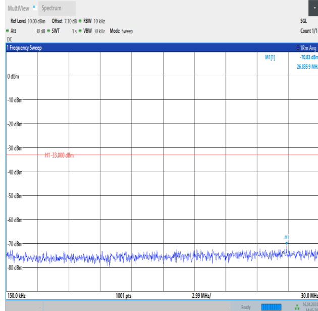
Band4_15MHz_QPSK_20175_1RB#74_0.15~30_0.15~30
