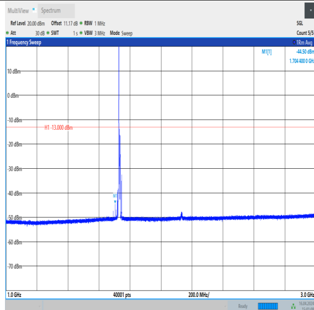
Band4_10MHz_16QAM_20175_1RB#0_1000~3000_1000~3000
