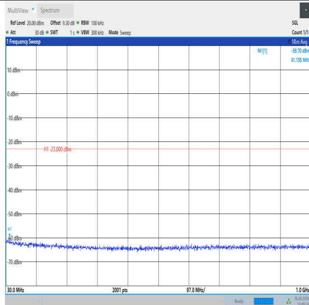
Band4_15MHz_16QAM_20325_1RB#74_30~1000_30~1000
