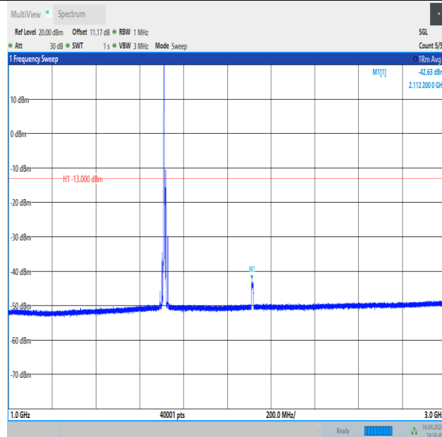
Band4_10MHz_QPSK_20000_1RB#0_1000~3000_1000~3000
