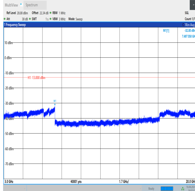
Band4_10MHz_QPSK_20175_50RB#0_3000~20000_3000~20000
