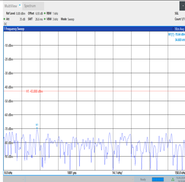
Band4_10MHz_QPSK_20000_50RB#0_0.009~0.15_0.009~0.15
