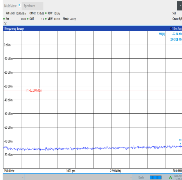
Band4_10MHz_QPSK_20000_1RB#0_0.15~30_0.15~30
