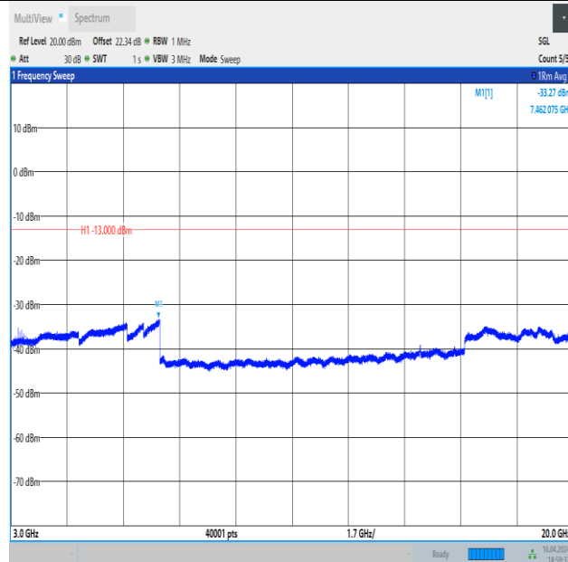
Band4_10MHz_16QAM_20000_1RB#49_3000~20000_3000~20000
