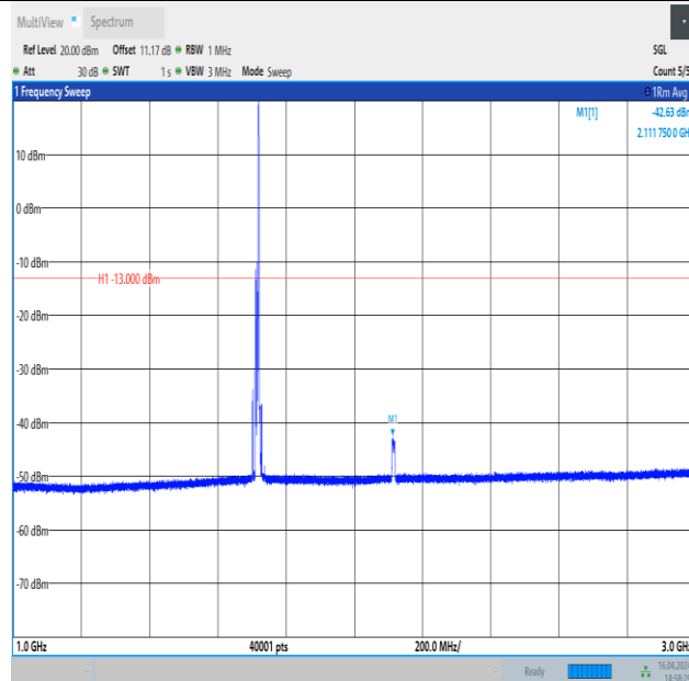
Band4_10MHz_QPSK_20000_1RB#49_1000~3000_1000~3000
