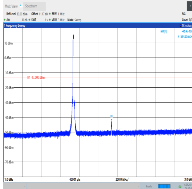
Band4_10MHz_QPSK_20175_50RB#0_1000~3000_1000~3000
