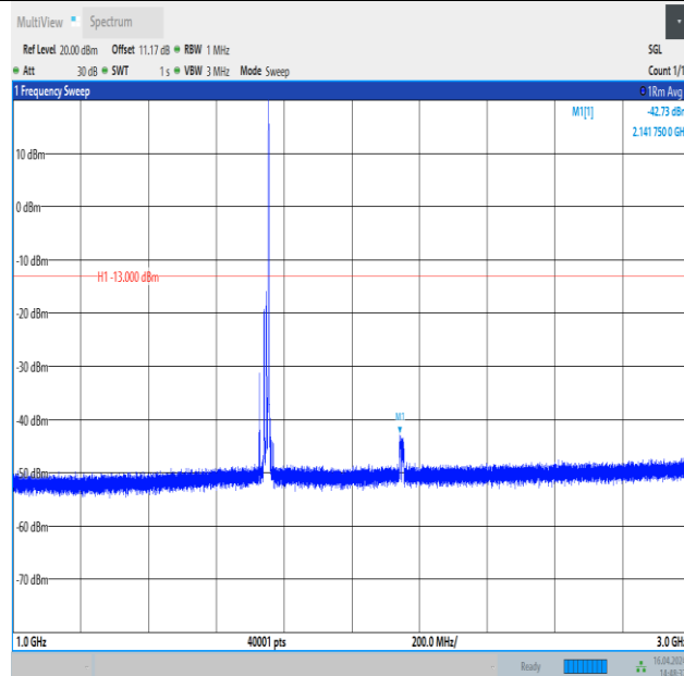
Band4_15MHz_16QAM_20325_1RB#74_1000~3000_1000~3000
