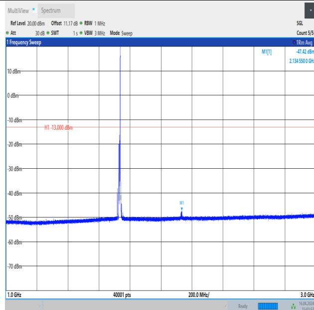
Band4_10MHz_16QAM_20175_1RB#49_1000~3000_1000~3000
