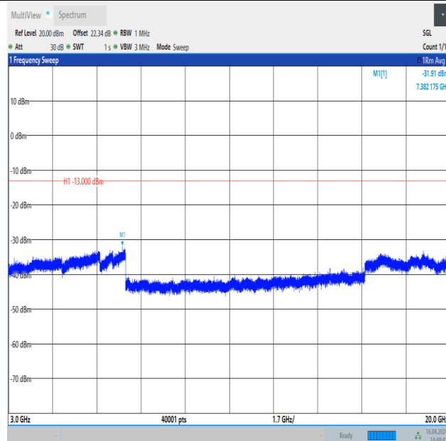
Band4_15MHz_16QAM_20325_1RB#74_3000~20000_3000~20000
