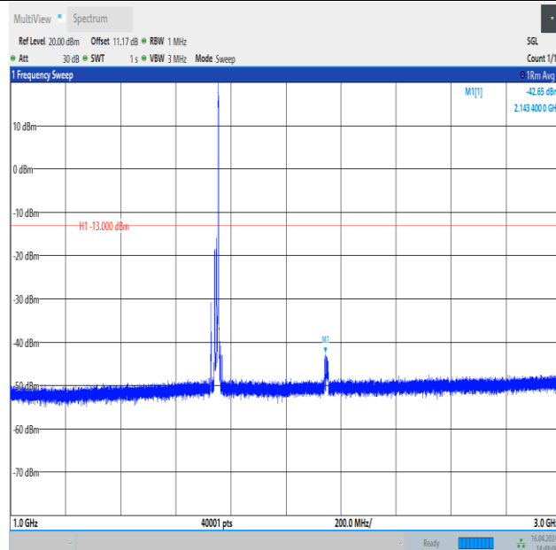
Band4_15MHz_QPSK_20325_1RB#74_1000~3000_1000~3000
