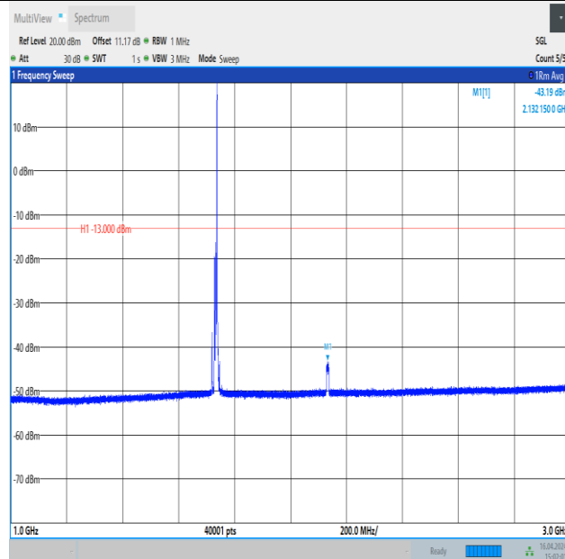
Band4_10MHz_QPSK_20175_1RB#49_1000~3000_1000~3000
