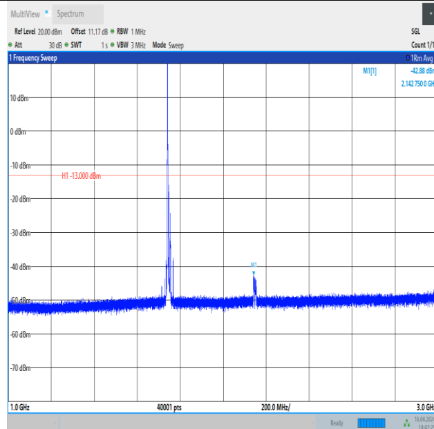
Band4_15MHz_16QAM_20325_1RB#0_1000~3000_1000~3000
