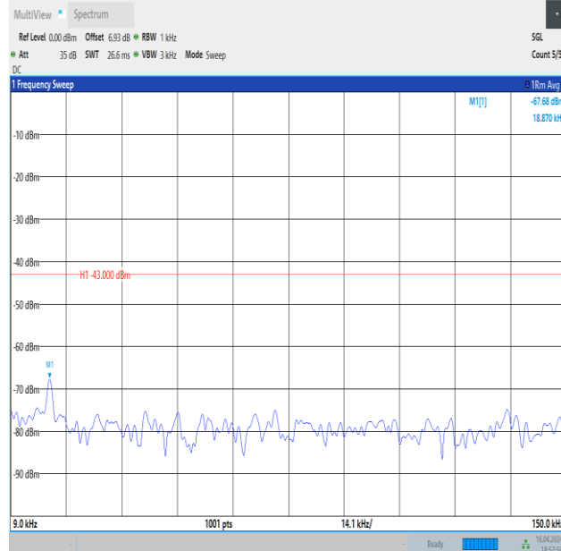
Band4_10MHz_QPSK_20000_1RB#49_0.009~0.15_0.009~0.15
