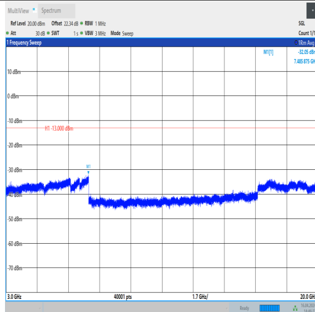
Band4_15MHz_16QAM_20175_1RB#74_3000~20000_3000~20000
