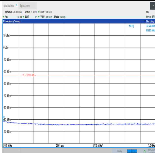
Band4_10MHz_QPSK_20000_1RB#49_30~1000_30~1000
