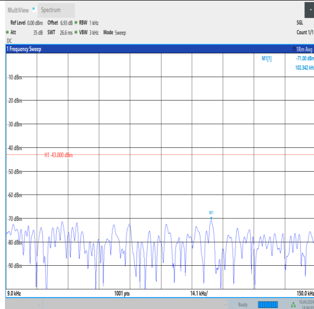
Band4_15MHz_QPSK_20175_1RB#0_0.009~0.15_0.009~0.15
