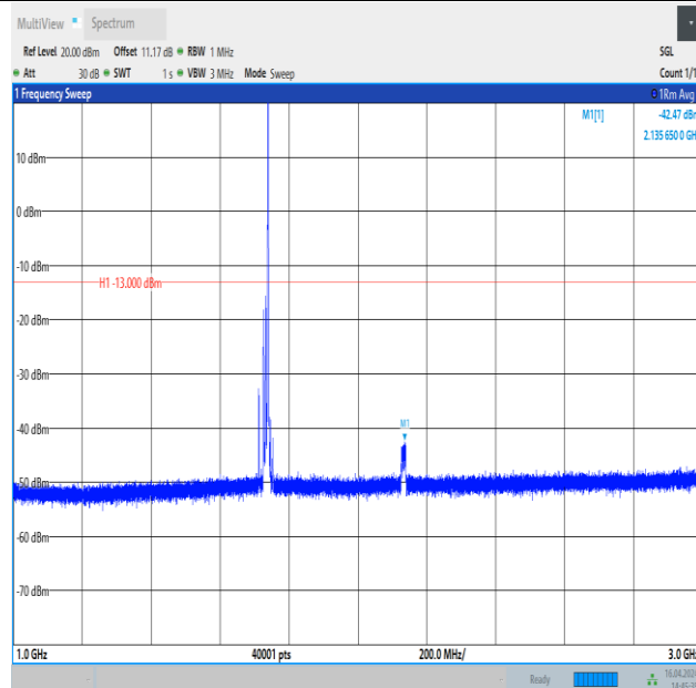
Band4_15MHz_QPSK_20175_1RB#74_1000~3000_1000~3000
