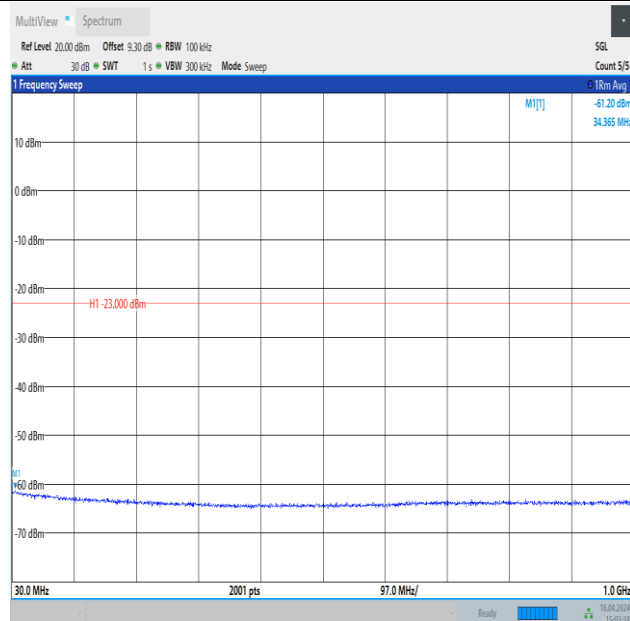
Band4_10MHz_QPSK_20350_1RB#0_30~1000_30~1000
