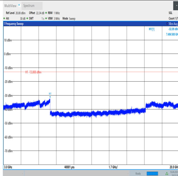
Band4_10MHz_QPSK_20350_50RB#0_3000~20000_3000~20000
