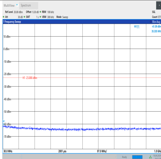
Band4_10MHz_QPSK_20175_50RB#0_30~1000_30~1000
