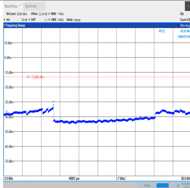
Band4_10MHz_16QAM_20175_1RB#0_3000~20000_3000~20000
