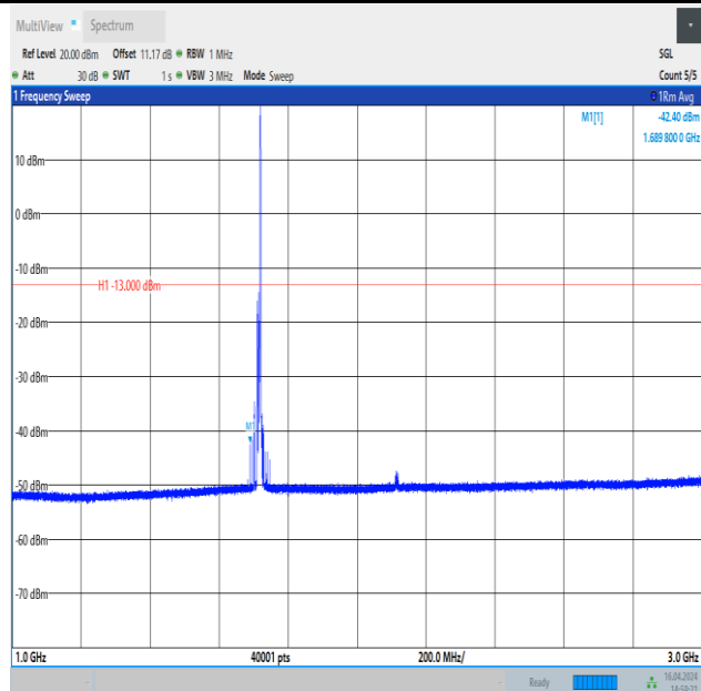
Band4_10MHz_16QAM_20000_1RB#49_1000~3000_1000~3000
