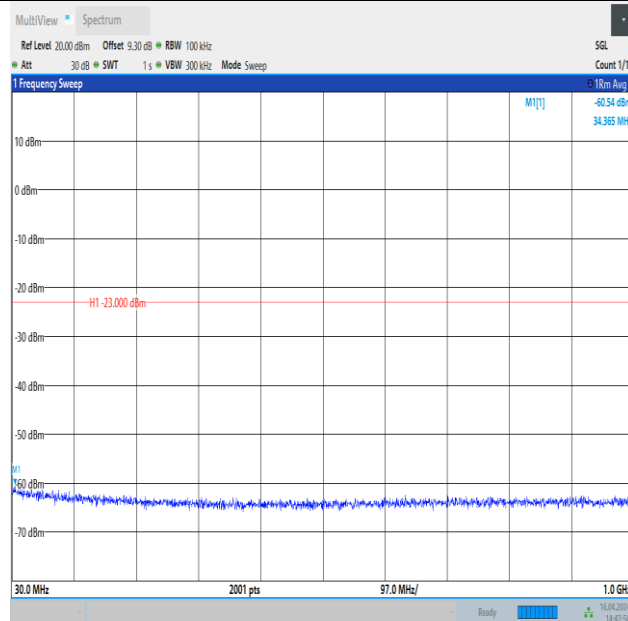
Band4_15MHz_QPSK_20325_1RB#74_30~1000_30~1000
