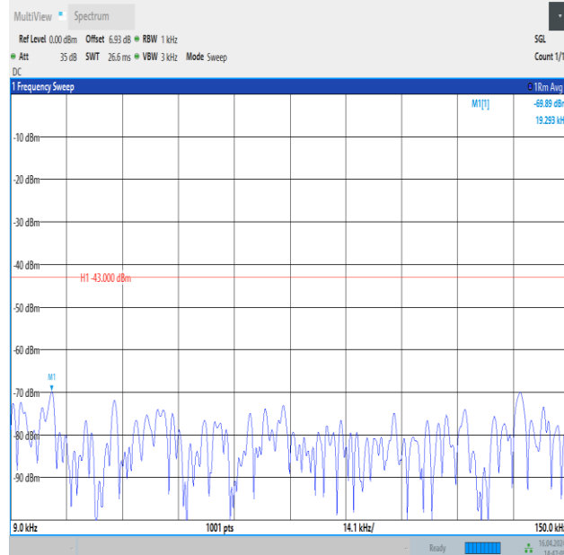
Band4_15MHz_16QAM_20325_1RB#0_0.009~0.15_0.009~0.15
