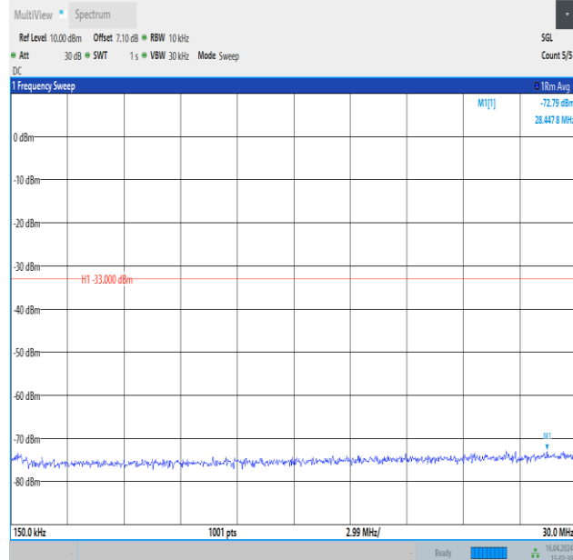
Band4_10MHz_16QAM_20175_1RB#49_0.15~30_0.15~30
