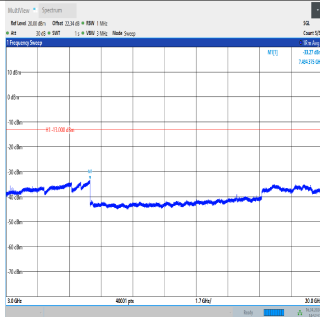
Band4_10MHz_16QAM_20000_1RB#0_3000~20000_3000~20000
