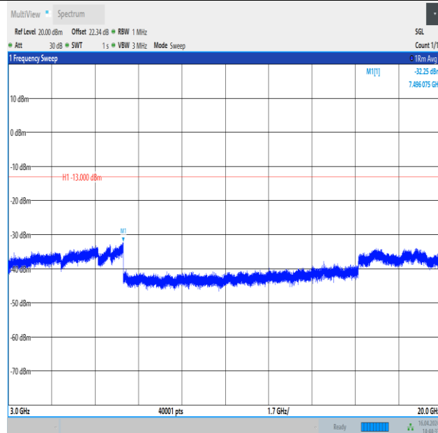
Band4_15MHz_QPSK_20175_1RB#0_3000~20000_3000~20000
