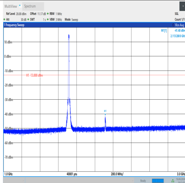
Band4_10MHz_QPSK_20000_50RB#0_1000~3000_1000~3000
