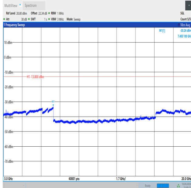
Band4_10MHz_QPSK_20175_1RB#0_3000~20000_3000~20000
