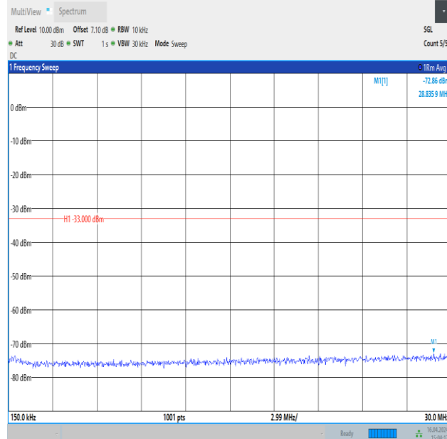
Band4_10MHz_16QAM_20350_1RB#0_0.15~30_0.15~30
