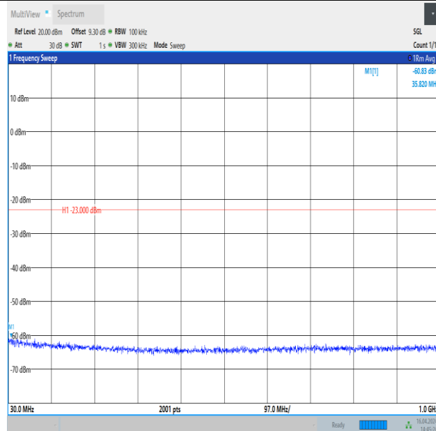
Band4_15MHz_QPSK_20175_1RB#74_30~1000_30~1000
