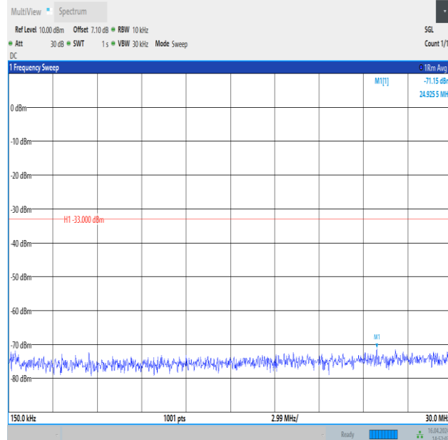
Band4_10MHz_QPSK_20350_50RB#0_0.15~30_0.15~30
