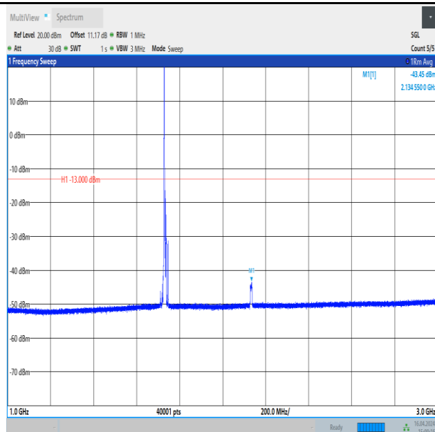
Band4_10MHz_QPSK_20175_1RB#0_1000~3000_1000~3000
