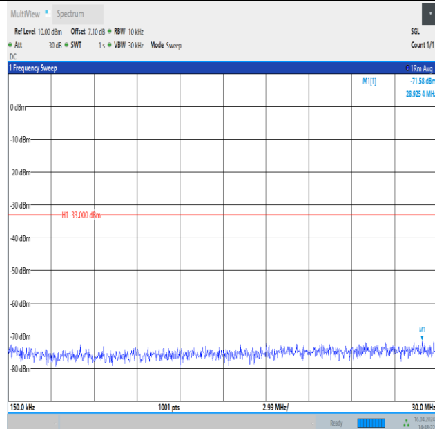
Band4_15MHz_16QAM_20325_1RB#74_0.15~30_0.15~30
