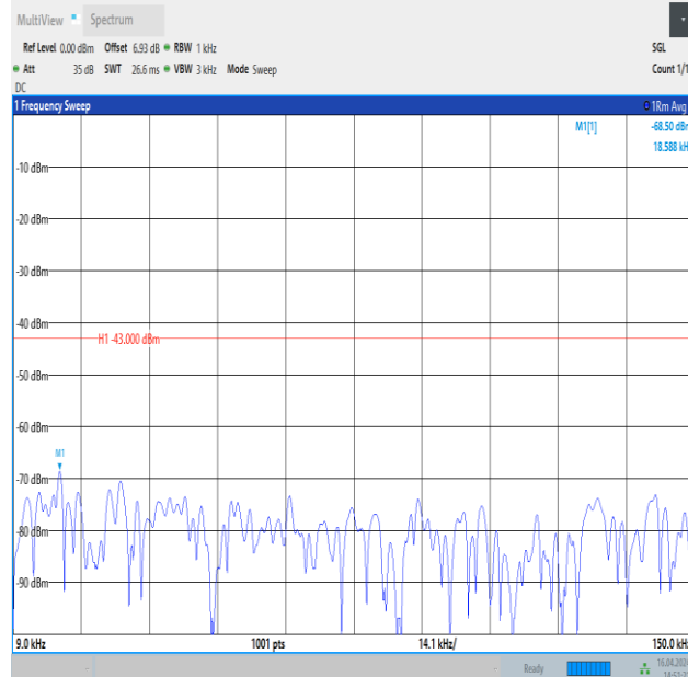
Band4_10MHz_QPSK_20175_50RB#0_0.009~0.15_0.009~0.15
