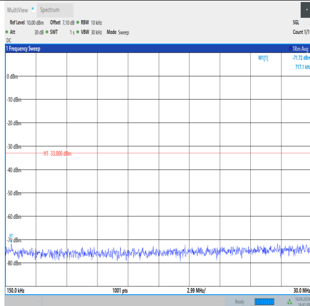
Band4_15MHz_16QAM_20325_1RB#0_0.15~30_0.15~30
