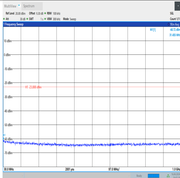
Band4_15MHz_16QAM_20325_1RB#0_30~1000_30~1000
