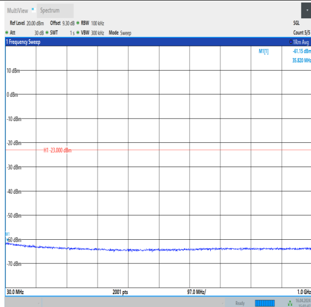
Band4_10MHz_QPSK_20175_1RB#49_30~1000_30~1000
