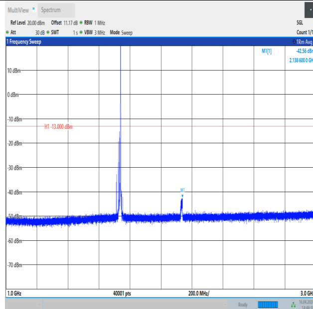
Band4_15MHz_16QAM_20175_1RB#74_1000~3000_1000~3000
