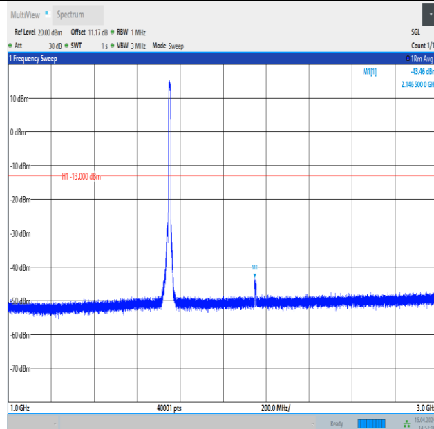
Band4_10MHz_QPSK_20350_50RB#0_1000~3000_1000~3000
