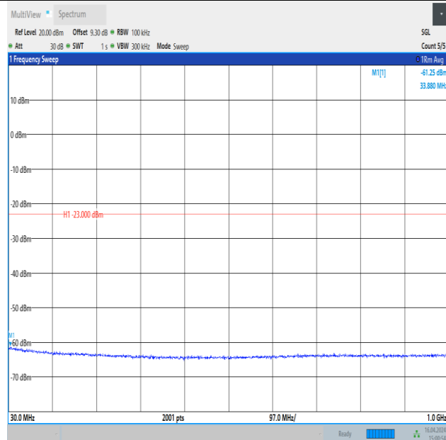
Band4_10MHz_16QAM_20175_1RB#0_30~1000_30~1000
