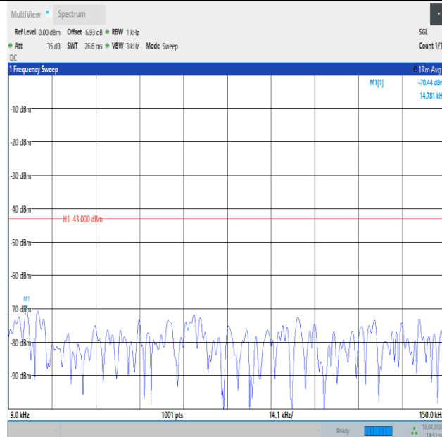
Band4_10MHz_QPSK_20350_50RB#0_0.009~0.15_0.009~0.15
