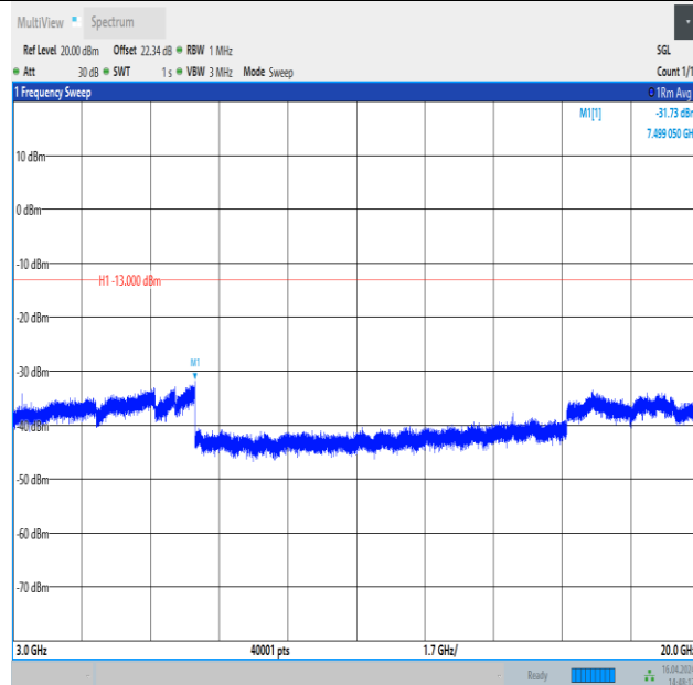
Band4_15MHz_QPSK_20325_1RB#74_3000~20000_3000~20000
