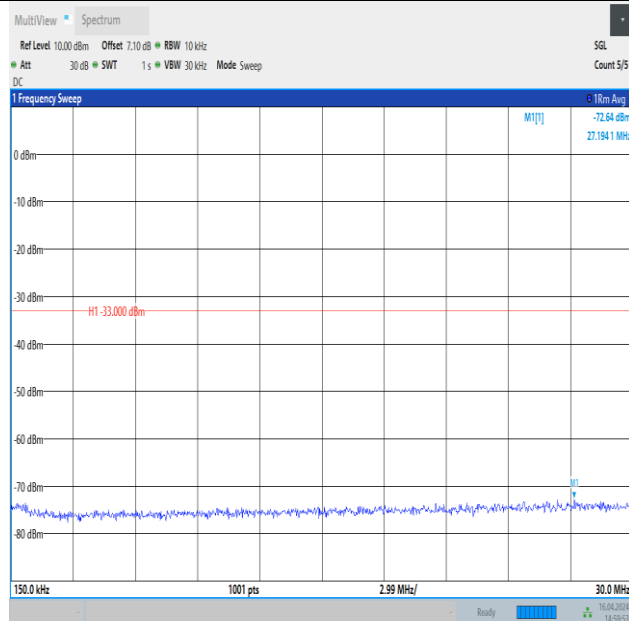
Band4_10MHz_QPSK_20175_1RB#0_0.15~30_0.15~30
