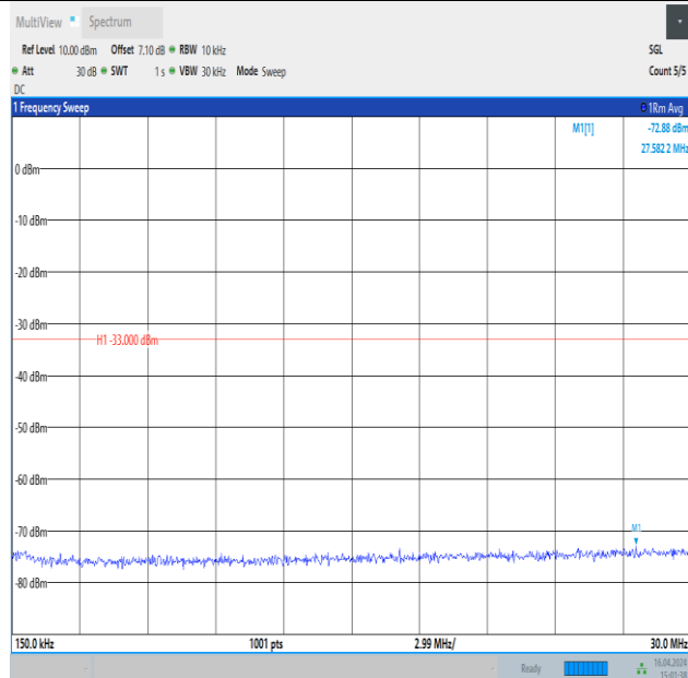
Band4_10MHz_QPSK_20175_1RB#49_0.15~30_0.15~30
