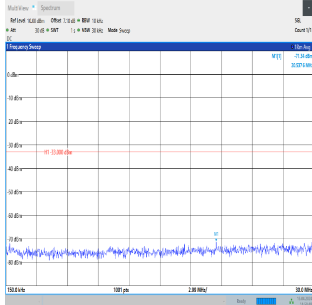
Band4_10MHz_QPSK_20000_50RB#0_0.15~30_0.15~30
