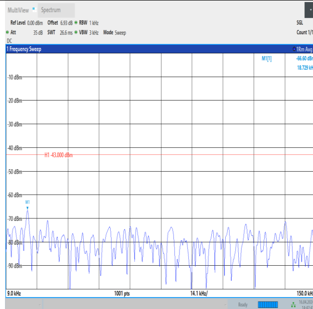
Band4_15MHz_QPSK_20325_1RB#74_0.009~0.15_0.009~0.15
