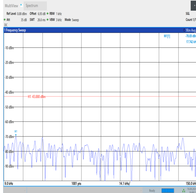
Band4_15MHz_16QAM_20325_1RB#74_0.009~0.15_0.009~0.15
