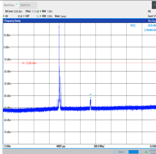
Band4_15MHz_16QAM_20175_1RB#0_1000~3000_1000~3000
