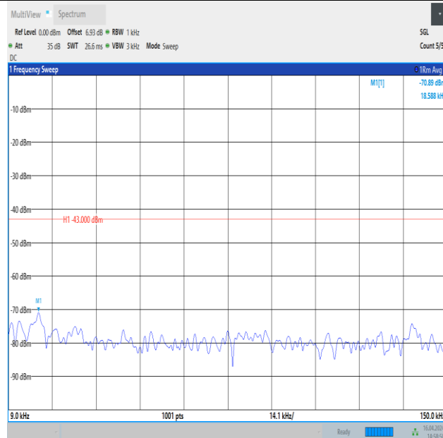
Band4_10MHz_16QAM_20000_1RB#49_0.009~0.15_0.009~0.15
