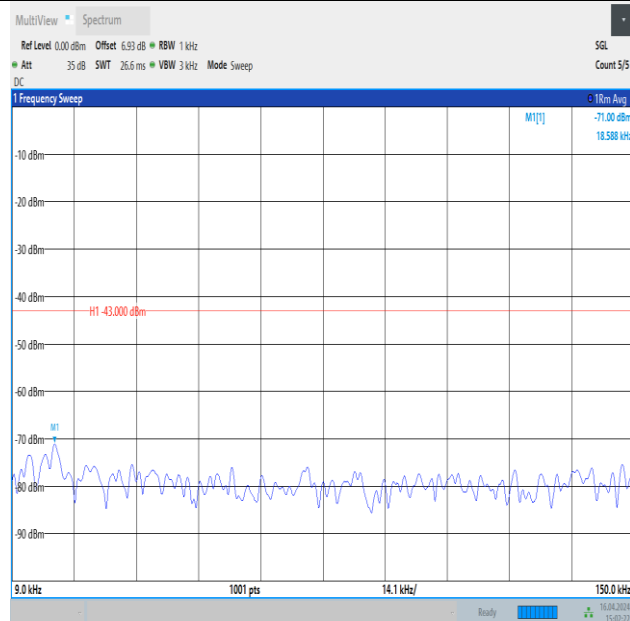
Band4_10MHz_16QAM_20175_1RB#49_0.009~0.15_0.009~0.15
