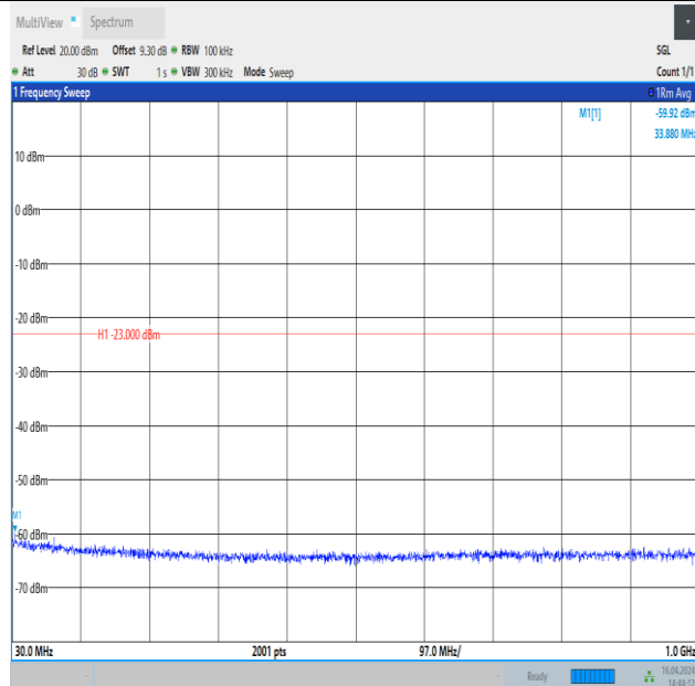
Band4_15MHz_QPSK_20175_1RB#0_30~1000_30~1000
