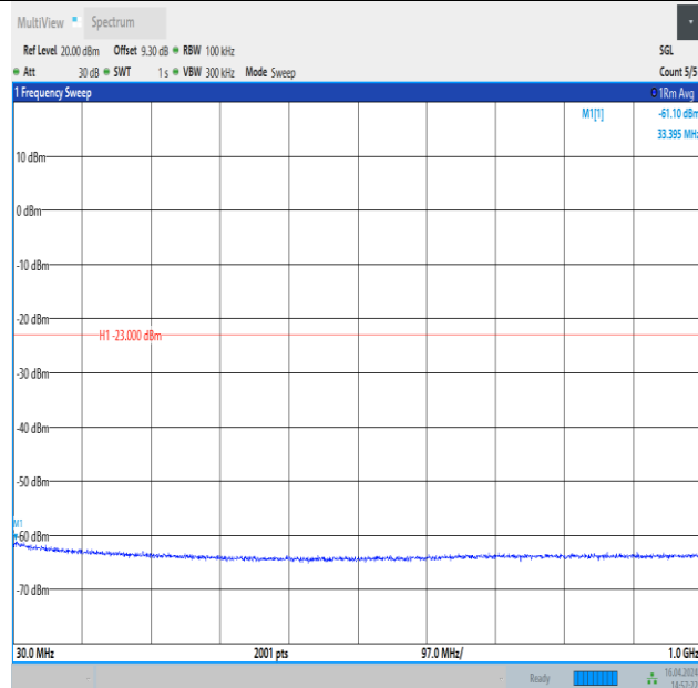
Band4_10MHz_16QAM_20000_1RB#0_30~1000_30~1000
