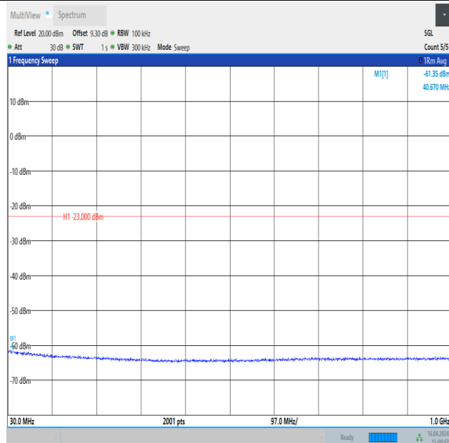
Band4_10MHz_QPSK_20175_1RB#0_30~1000_30~1000
