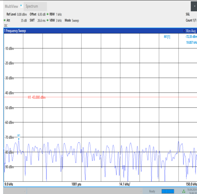
Band4_15MHz_QPSK_20325_1RB#0_0.009~0.15_0.009~0.15
