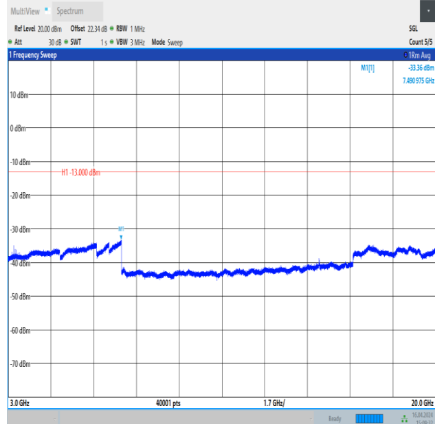
Band4_15MHz_QPSK_20325_75RB#0_3000~20000_3000~20000
