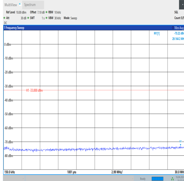
Band4_1.4MHz_16QAM_20175_6RB#0_0.15~30_0.15~30
