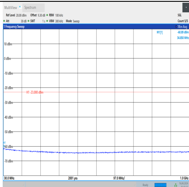
Band4_20MHz_QPSK_20300_100RB#0_30~1000_30~1000
