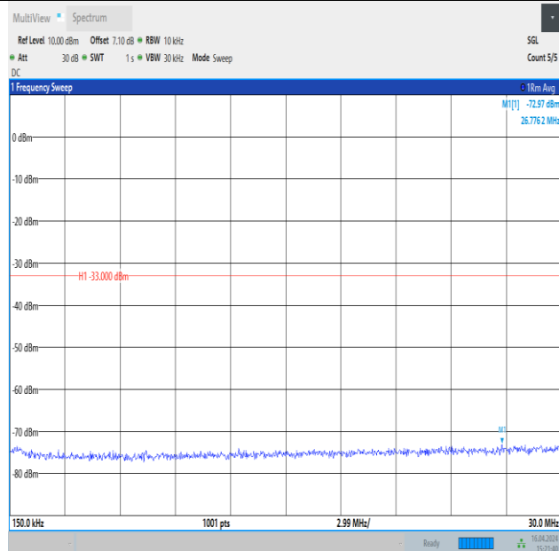
Band4_1.4MHz_QPSK_19957_1RB#0_0.15~30_0.15~30
