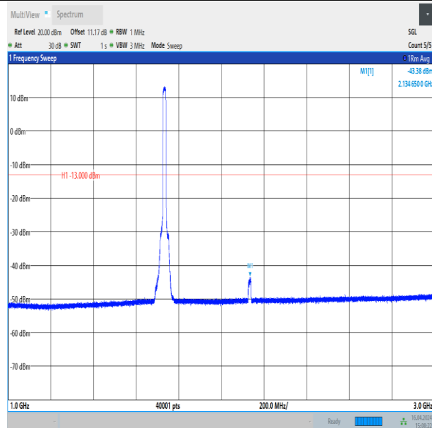
Band4_15MHz_QPSK_20175_75RB#0_1000~3000_1000~3000
