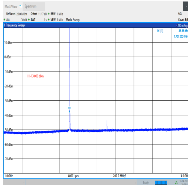
Band4_1.4MHz_16QAM_19957_6RB#0_1000~3000_1000~3000
