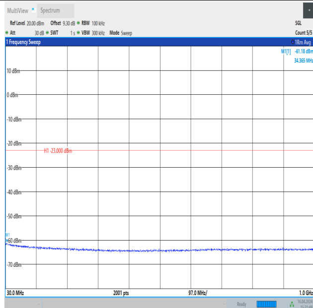
Band4_1.4MHz_QPSK_19957_1RB#0_30~1000_30~1000
