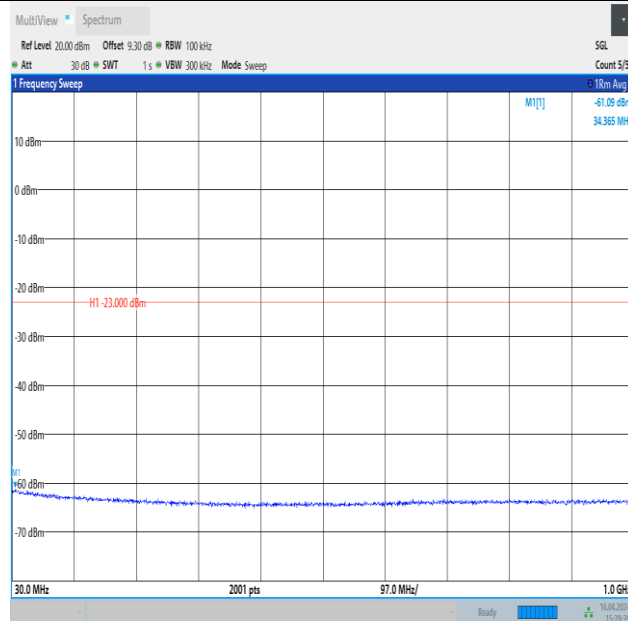
Band4_1.4MHz_16QAM_20175_1RB#5_30~1000_30~1000
