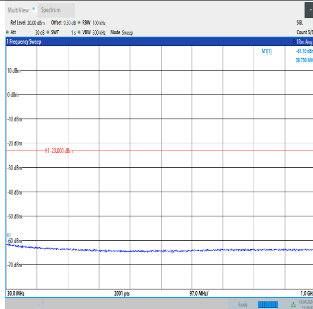
Band4_1.4MHz_16QAM_19957_6RB#0_30~1000_30~1000
