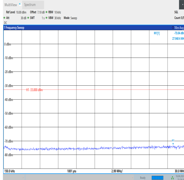
Band4_1.4MHz_16QAM_19957_1RB#5_0.15~30_0.15~30
