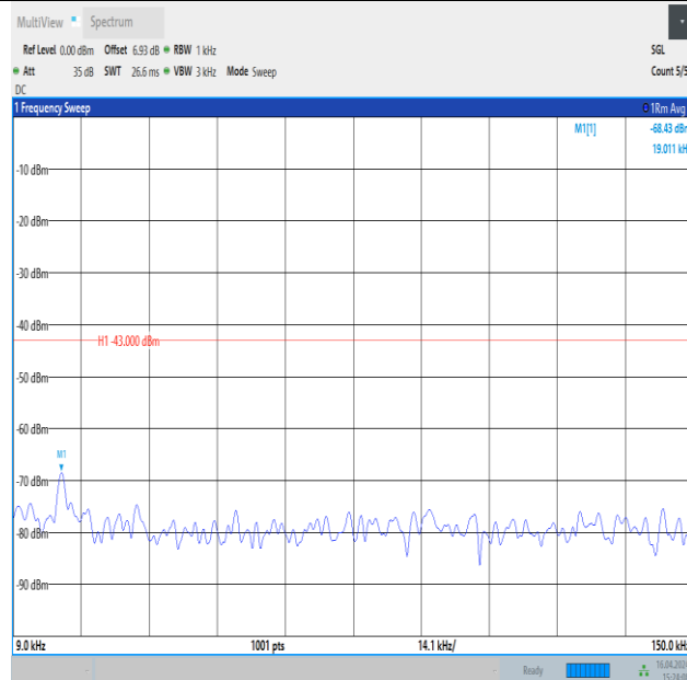
Band4_1.4MHz_16QAM_19957_1RB#5_0.009~0.15_0.009~0.15
