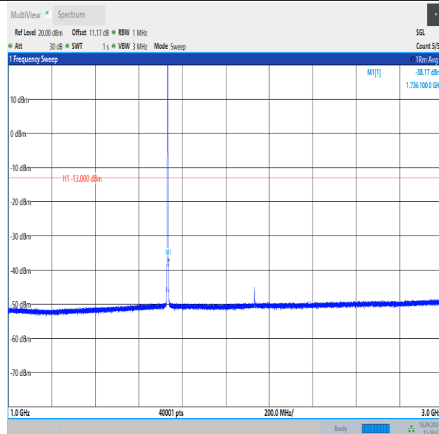
Band4_1.4MHz_16QAM_20175_1RB#5_1000~3000_1000~3000
