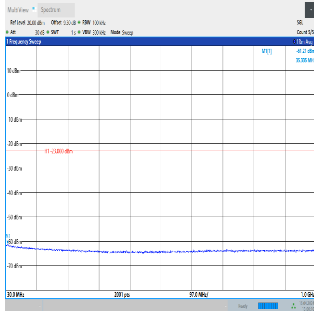
Band4_10MHz_16QAM_20350_1RB#49_30~1000_30~1000
