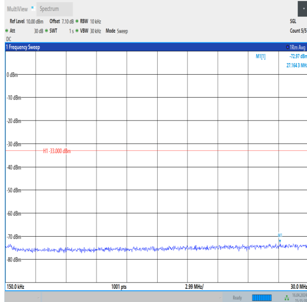
Band4_1.4MHz_QPSK_20393_6RB#0_0.15~30_0.15~30
