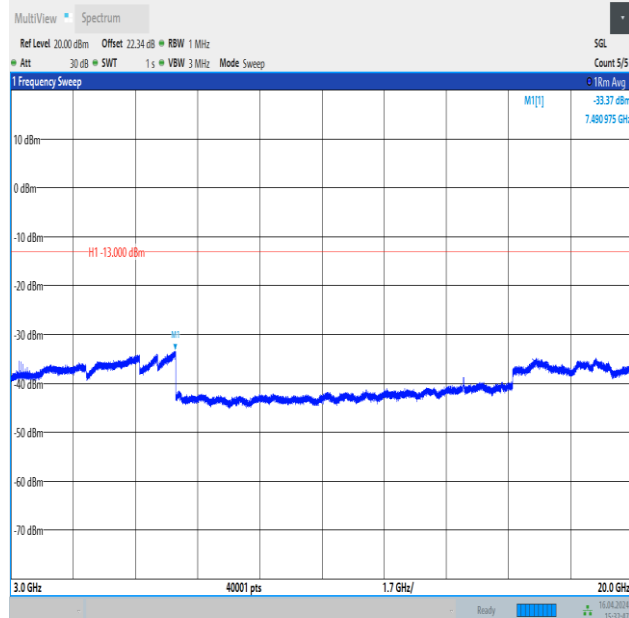
Band4_1.4MHz_QPSK_20393_1RB#0_3000~20000_3000~20000
