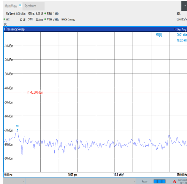
Band4_3MHz_16QAM_19965_1RB#0_0.009~0.15_0.009~0.15
