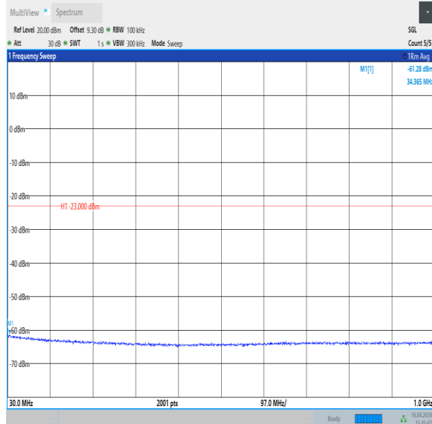
Band4_1.4MHz_QPSK_20393_6RB#0_30~1000_30~1000
