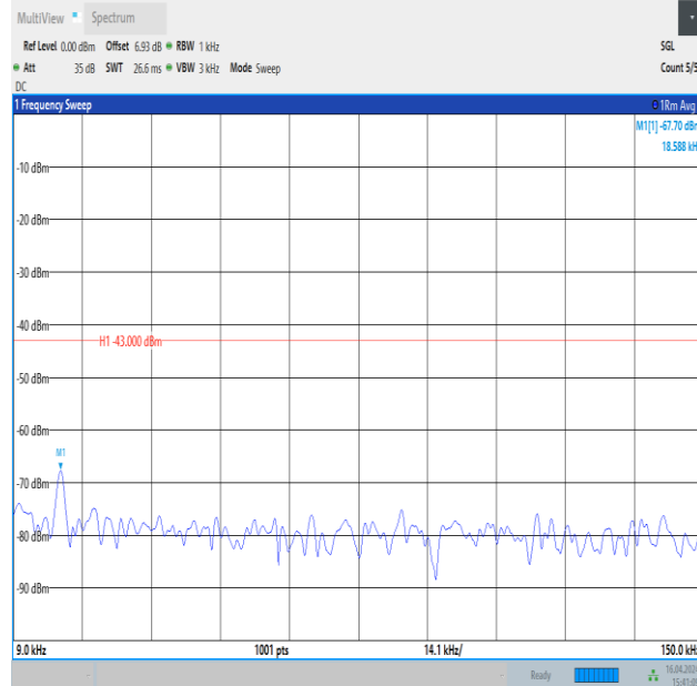
Band4_20MHz_QPSK_20050_1RB#0_0.009~0.15_0.009~0.15
