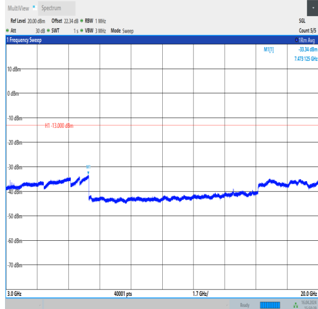
Band4_20MHz_QPSK_20300_1RB#99_3000~20000_3000~20000
