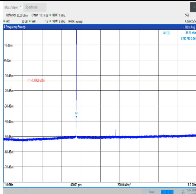
Band4_1.4MHz_QPSK_20393_1RB#0_1000~3000_1000~3000
