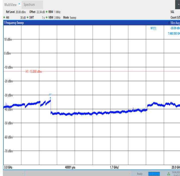
Band4_20MHz_QPSK_20175_1RB#99_3000~20000_3000~20000
