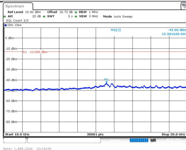
Band2-9262-3-10000~20000MHz
