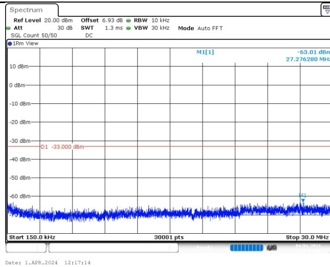
Band2-9400-2-0.009~0.15MHz
