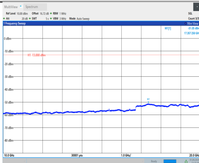
Band4-1312-3-10000~20000MHz
