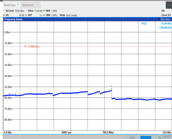
Band4-1513-4-3000~10000MHz
