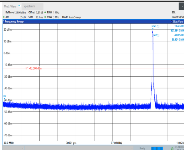
Band5-4132-4-1000~1500MHz
