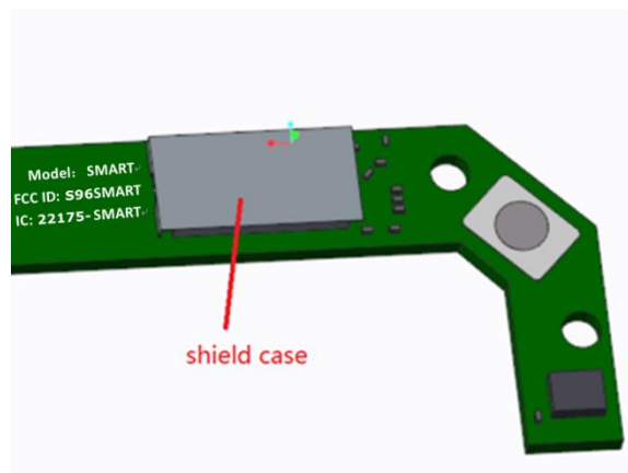
Figure 5-2: Add Shield Case view
