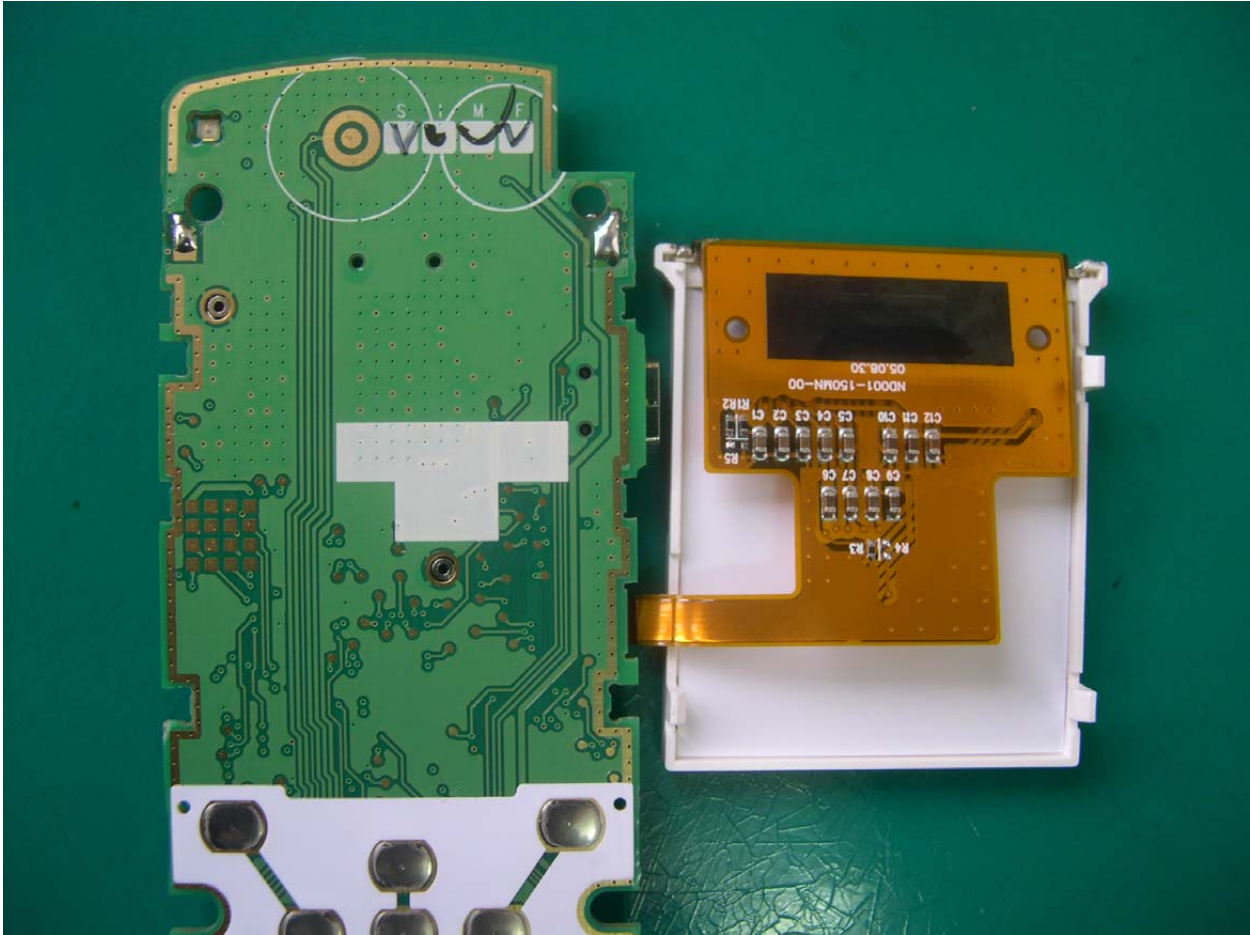
<Photograph 6: Internal Rear View – LCD Module >
