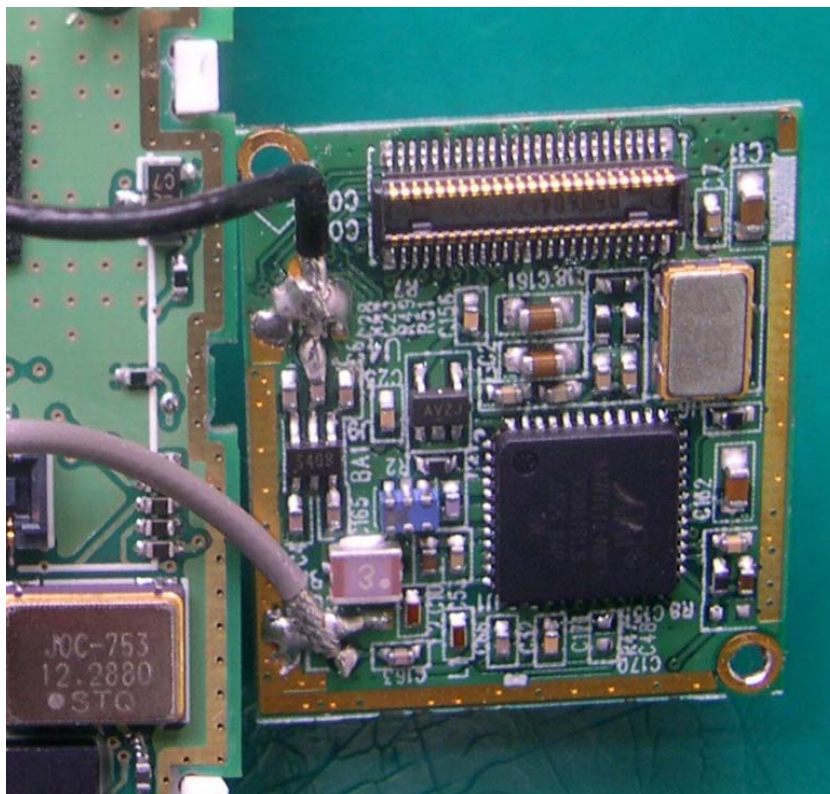
<Photograph 5: Internal Rear View – RF Module >
