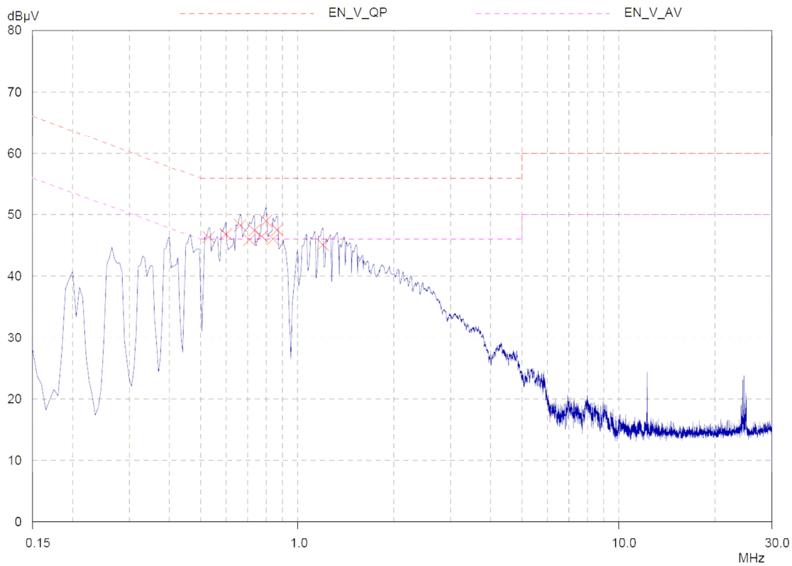
Figure 6. Plot of the Conducted Emissions
