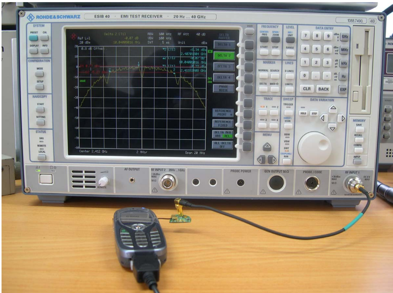
The antenna port of the EUT was connected to the spectrum analyzer using the RF cable
