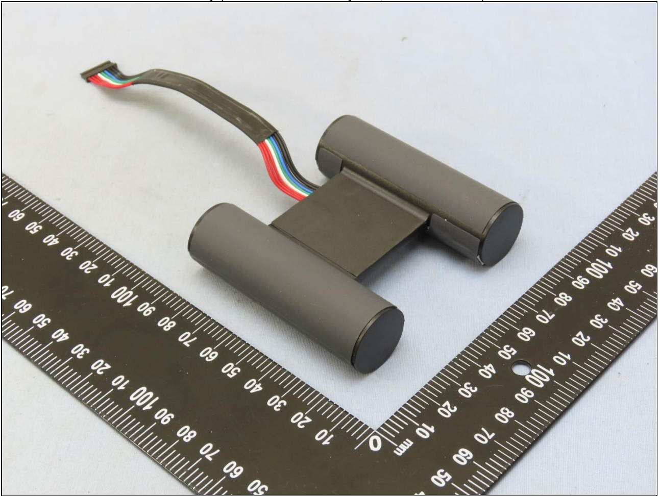
Battery (Brand: ETICA Battery Inc., Model: SGB-02)
