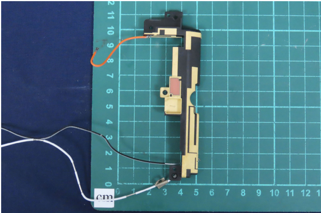
(35) EUT Photo
