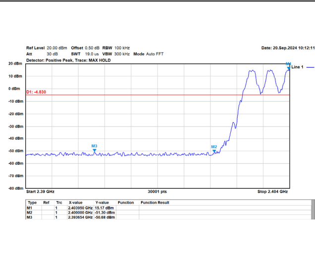
8DPSK(3DH5) (Band Edge Hopping) / 2402 MHz
