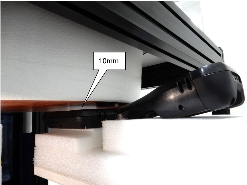
EUT Front - 10mm (Antenna 2)
