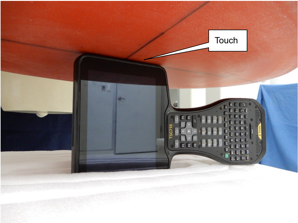
EUT Right-side -10mm (Main Antenna)
