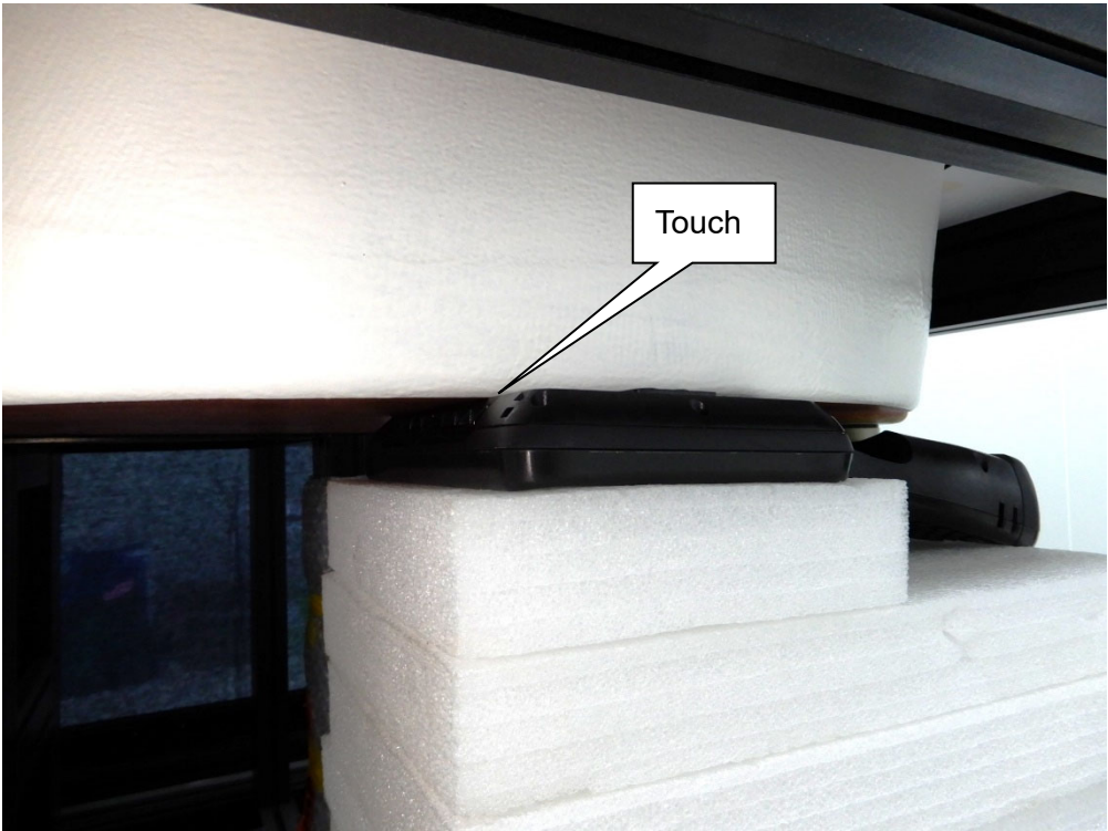
EUT Back - 15mm (Antenna 2)
