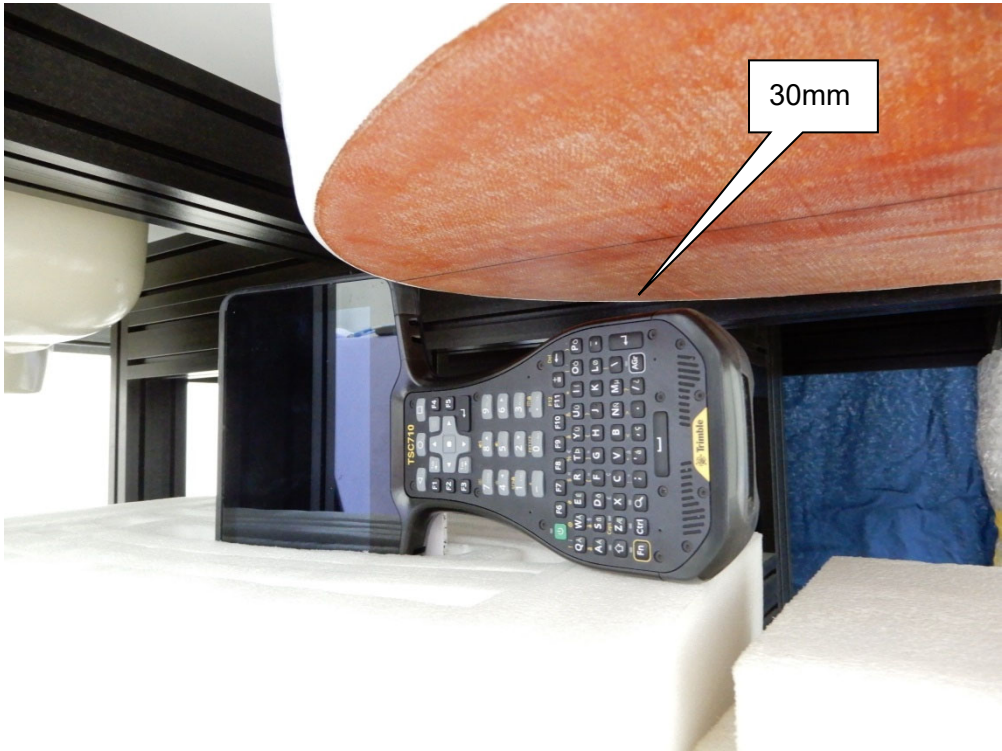
EUT Right-side - 30mm (Antenna 3)
