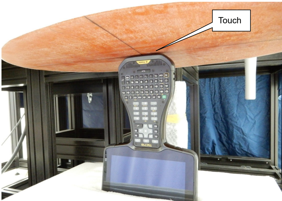
EUT Bottom - 0mm (Antenna 1, Antenna 3)
