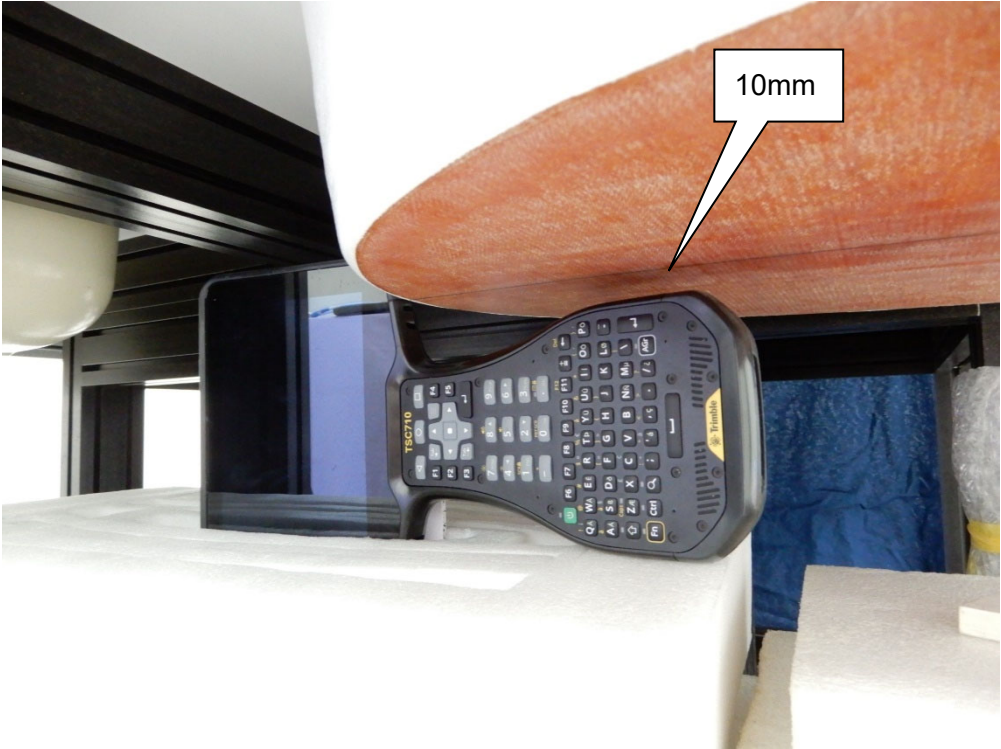
EUT Right-side - 10mm (Antenna 3)
