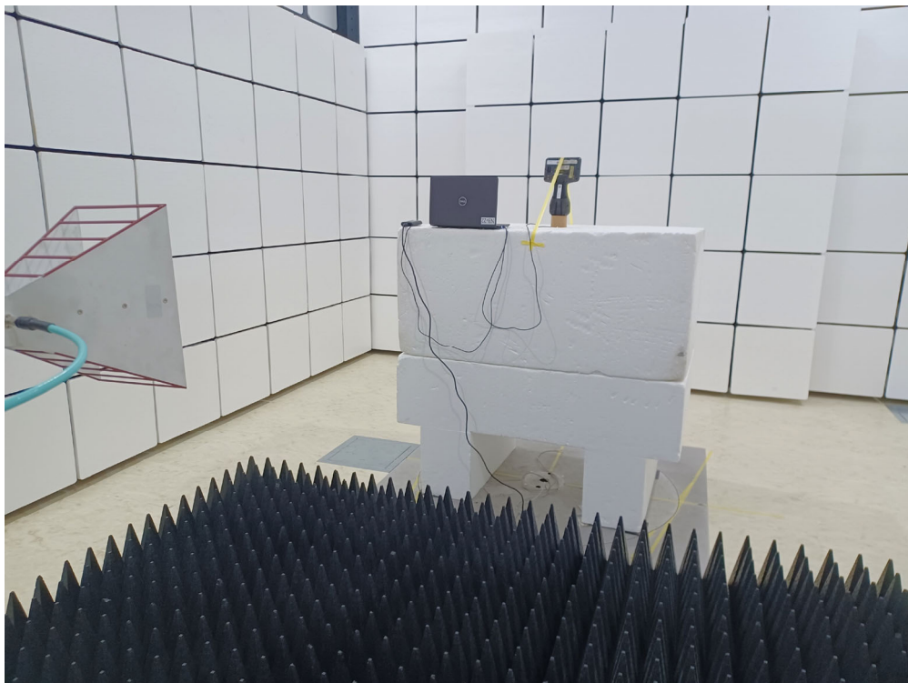
Radiated Test (Horn) (Above 1 GHz)
