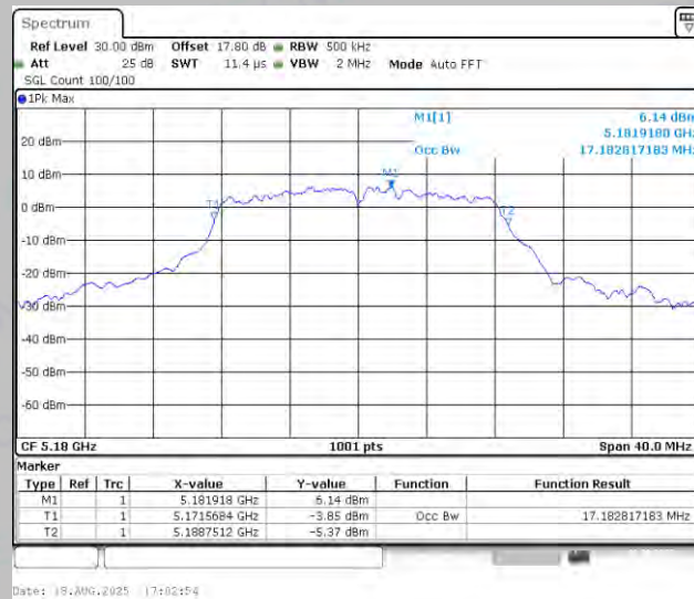
11A-Ant2-5180
