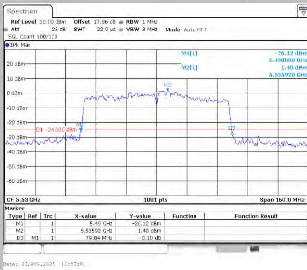
11AC80MIMO-Ant1-5530
