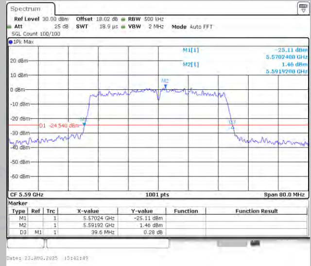
11AC40MIMO-Ant2-5590
