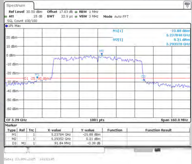
11AC80MIMO-Ant2-5290
