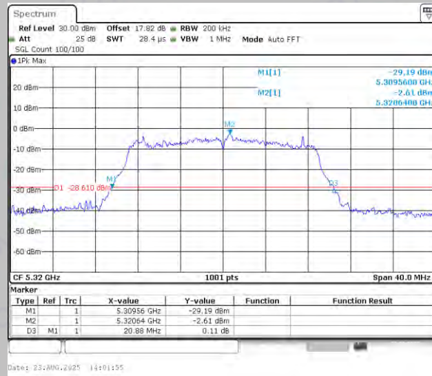
11AC20MIMO-Ant2-5320
