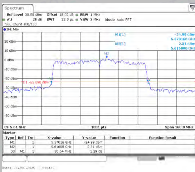
11AC80MIMO-Ant1-5610
