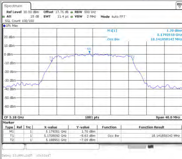
11N20MIMO-Ant1-5180
