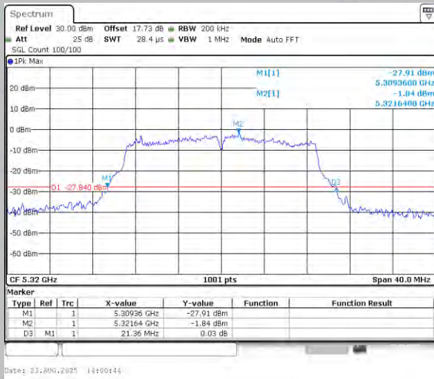
11AC20MIMO-Ant1-5320
