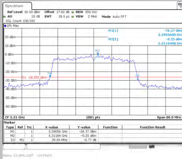
11N40MIMO-Ant2-5310
