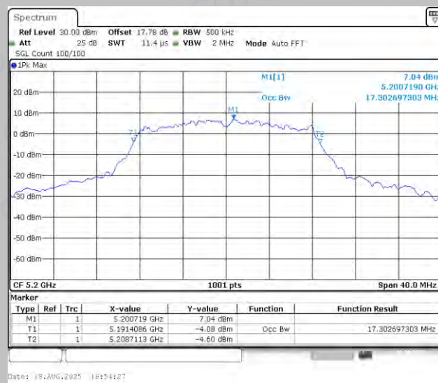
11A-Ant2-5200
