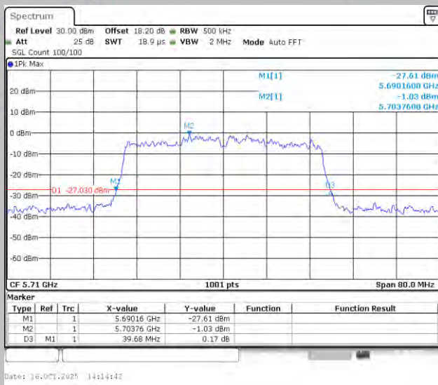
11AC40MIMO-Ant1-5710
