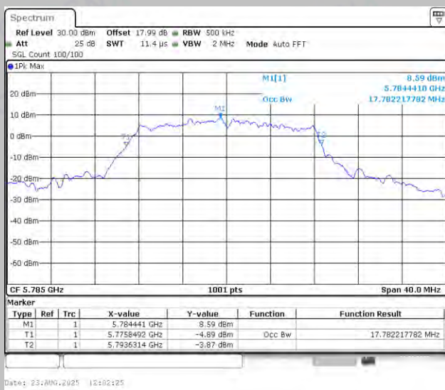
11A-Ant1-5785
