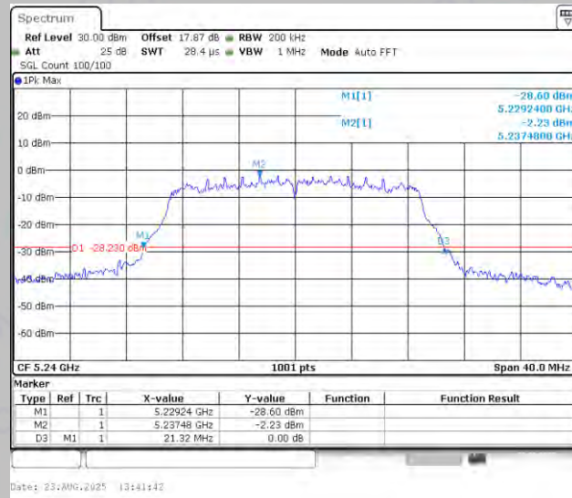
11AC20MIMO-Ant2-5240
