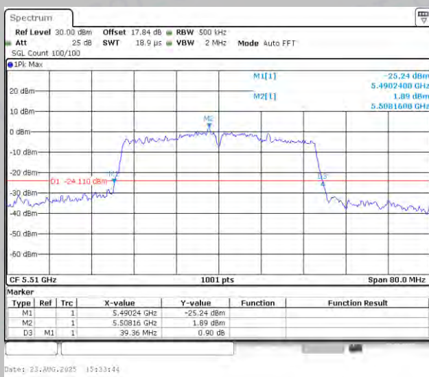
11AC40MIMO-Ant1-5510
