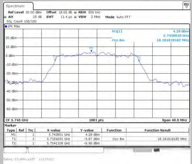
11N20MIMO-Ant2-5745
