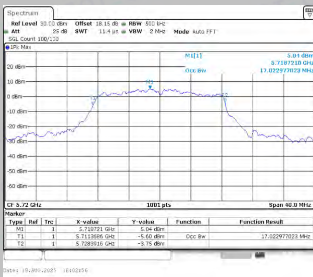
11A-Ant2-5720
