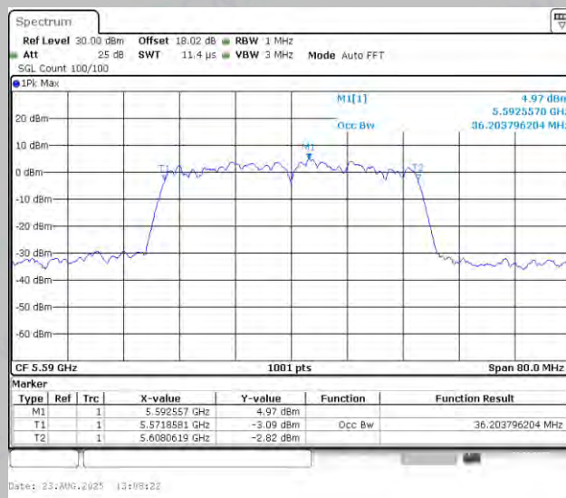
11N40MIMO-Ant2-5590
