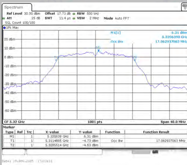
11A-Ant1-5320
