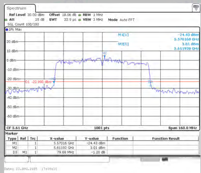
11AC80MIMO-Ant2-5610
