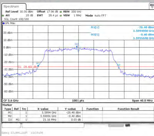
11AC20MIMO-Ant1-5600
