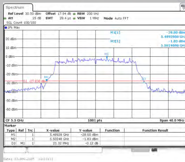
11AC20MIMO-Ant2-5500
