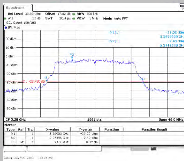
11AC20MIMO-Ant2-5280
