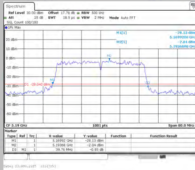
11N40MIMO-Ant2-5190
