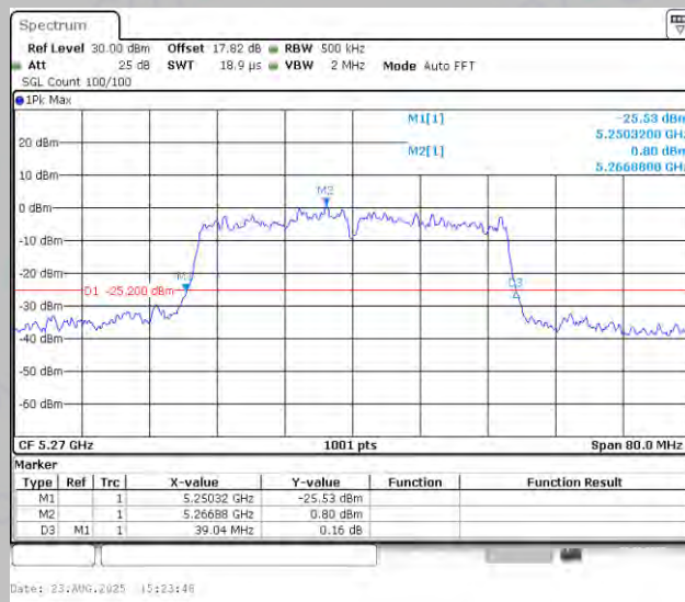
11AC40MIMO-Ant2-5270
