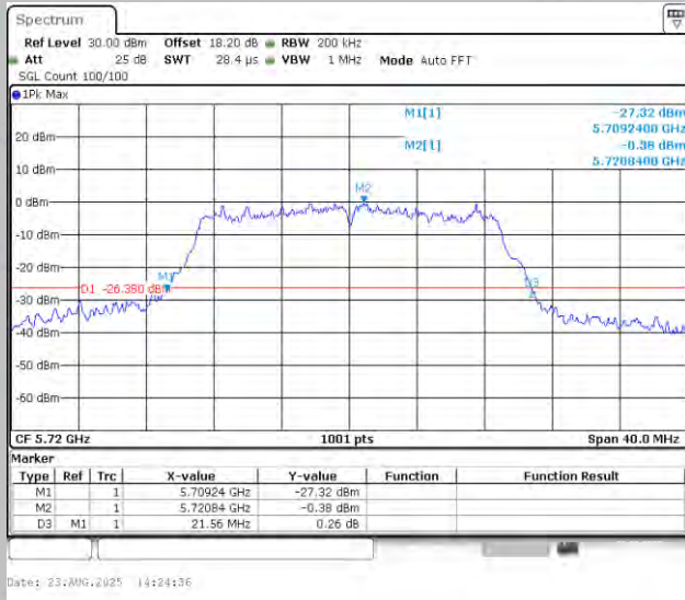
11AC20MIMO-Ant1-5720
