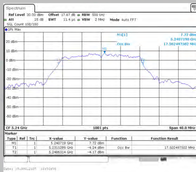
11A-Ant2-5240
