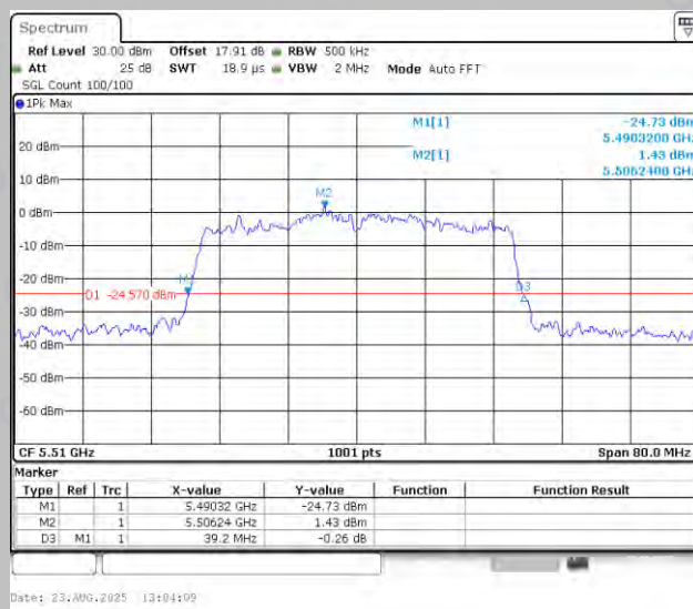
11N40MIMO-Ant2-5510
