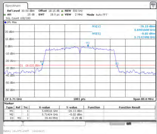
11AC40MIMO-Ant2-5710
