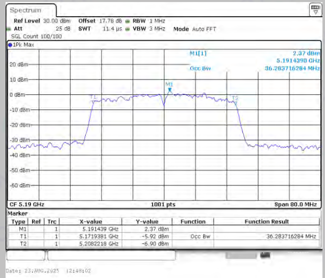
11N40MIMO-Ant2-5190
