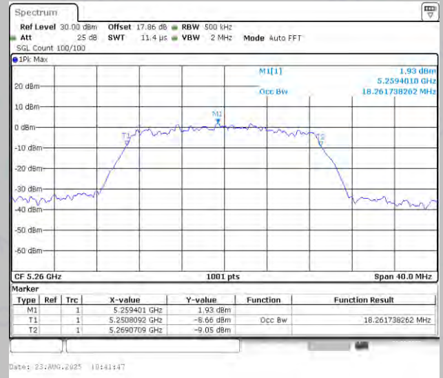
11N20MIMO-Ant2-5260
