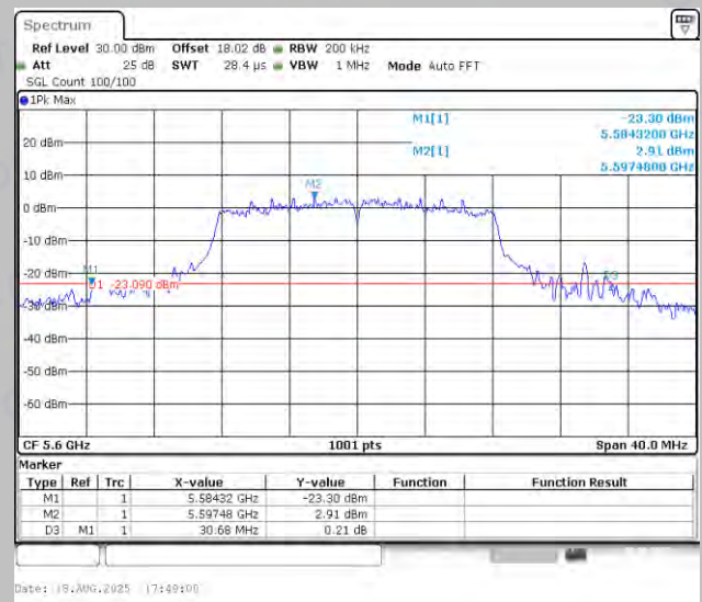
11A-Ant2-5600
