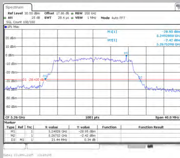
11AC20MIMO-Ant2-5260
