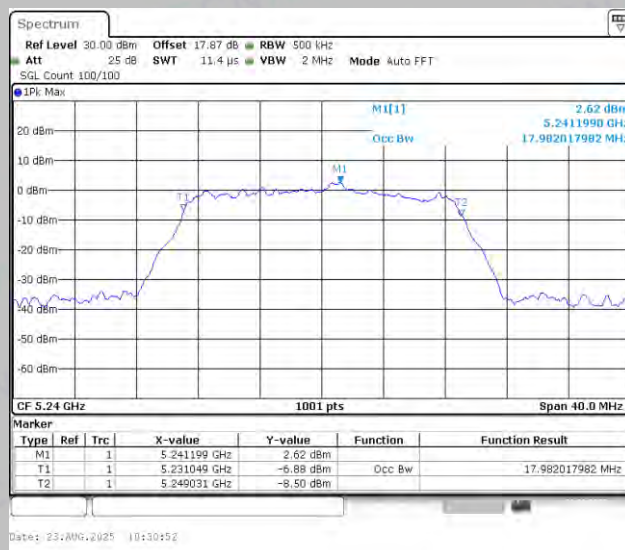
11N20MIMO-Ant2-5240
