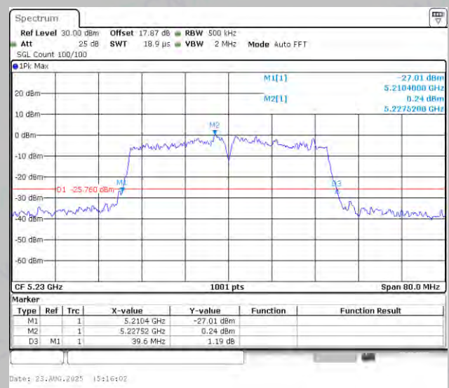
11AC40MIMO-Ant2-5230
