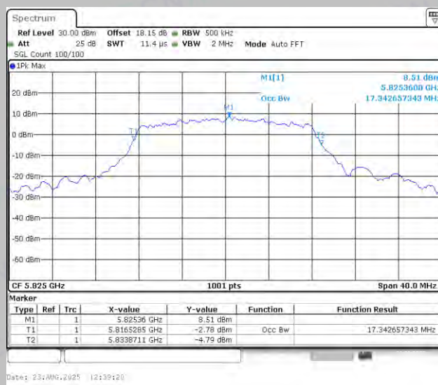
11A-Ant2-5825
