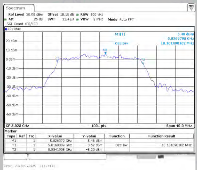
11N20MIMO-Ant2-5825
