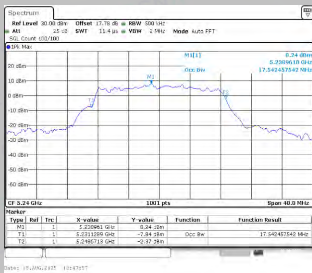
11A-Ant1-5240
