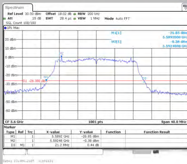
11N20MIMO-Ant2-5600
