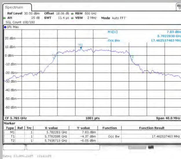
11A-Ant2-5785
