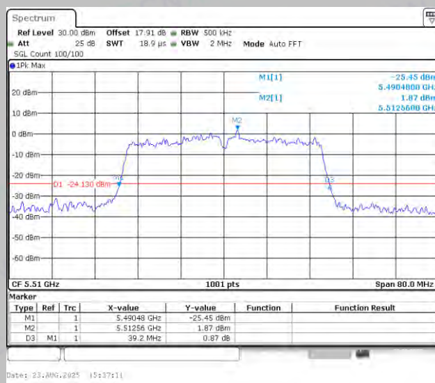
11AC40MIMO-Ant2-5510
