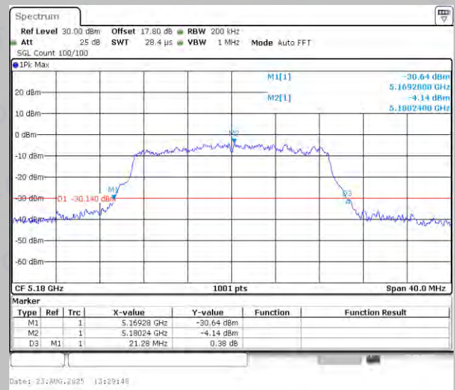
11AC20MIMO-Ant2-5180
