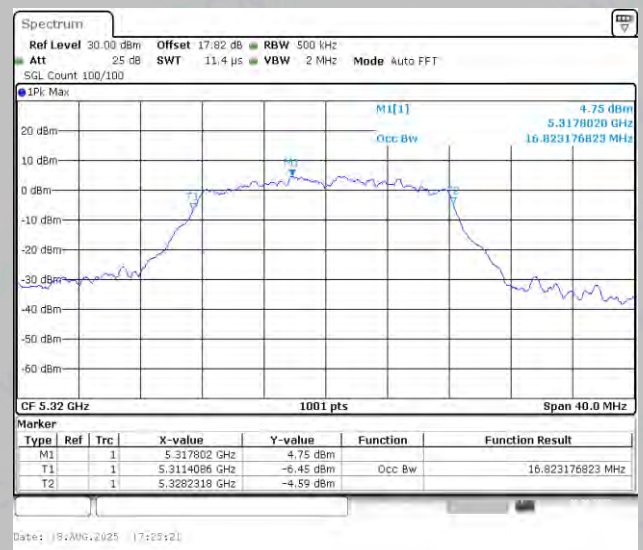
11A-Ant2-5320
