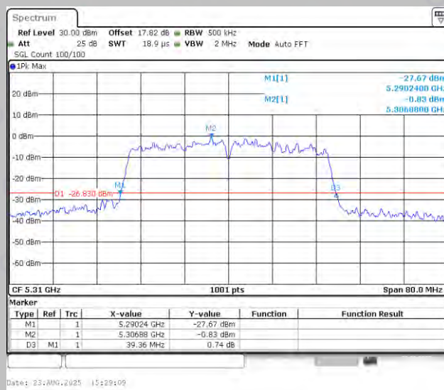
11AC40MIMO-Ant2-5310
