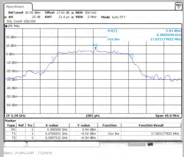
11A-Ant2-5280
