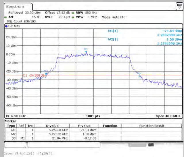
11A-Ant2-5280
