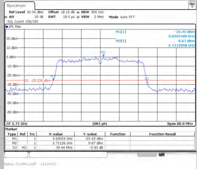
11N40MIMO-Ant2-5710
