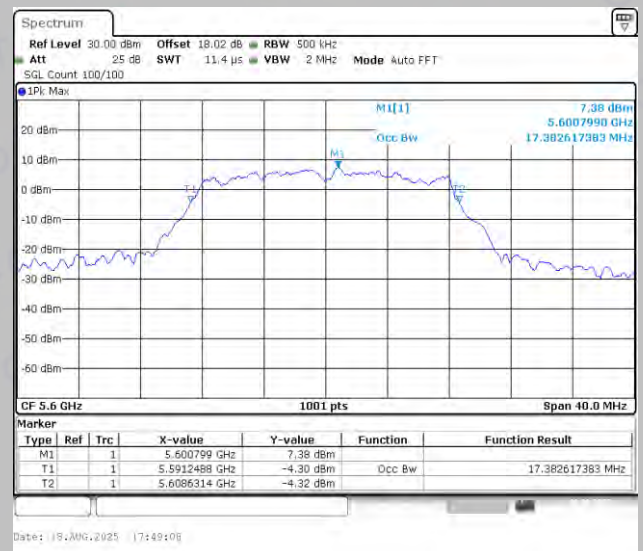
11A-Ant2-5600
