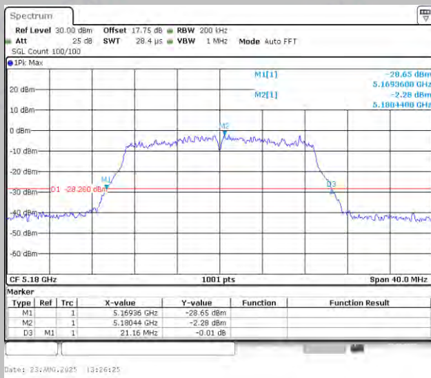
11AC20MIMO-Ant1-5180
