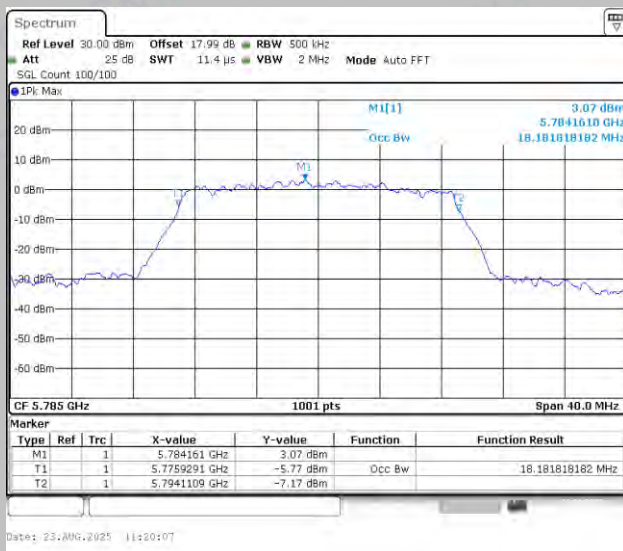
11N20MIMO-Ant1-5785
