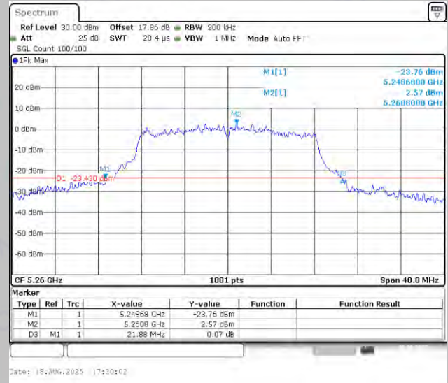
11A-Ant2-5260
