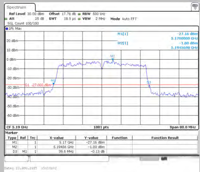
11AC40MIMO-Ant2-5190
