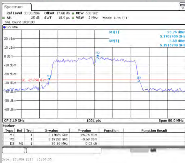
11AC40MIMO-Ant1-5190
