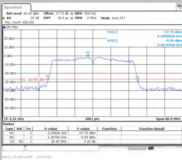
11AC40MIMO-Ant1-5310
