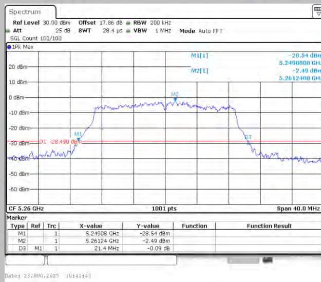
11N20MIMO-Ant2-5260
