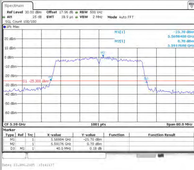
11AC40MIMO-Ant1-5590
