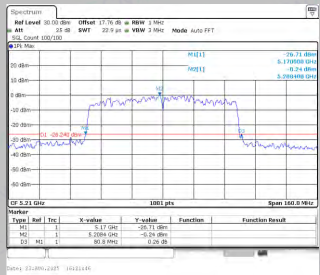
11AC80MIMO-Ant2-5210
