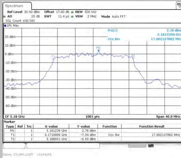
11N20MIMO-Ant2-5180
