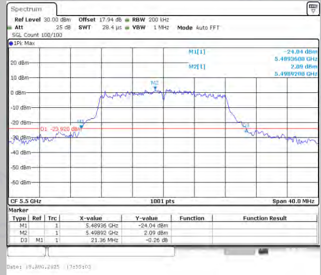
11A-Ant2-5500
