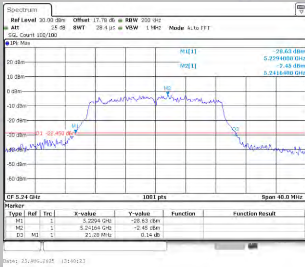
11AC20MIMO-Ant1-5240
