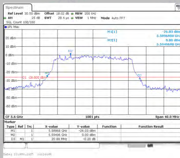
11AC20MIMO-Ant2-5600
