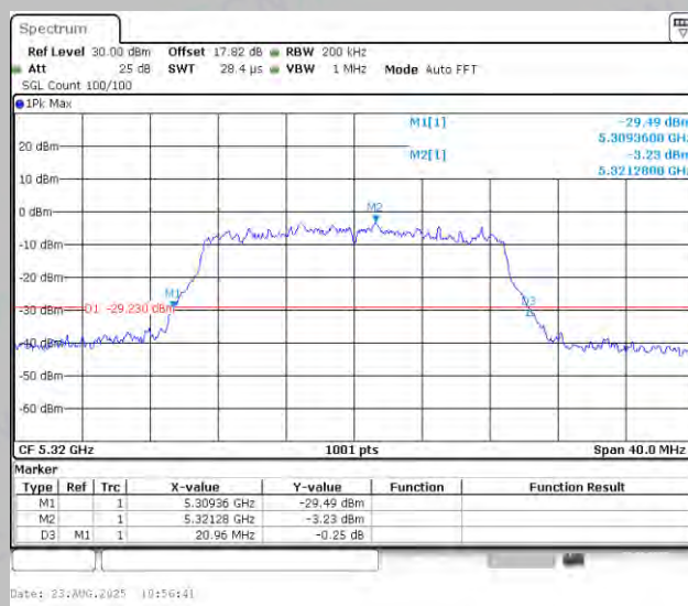
11N20MIMO-Ant2-5320
