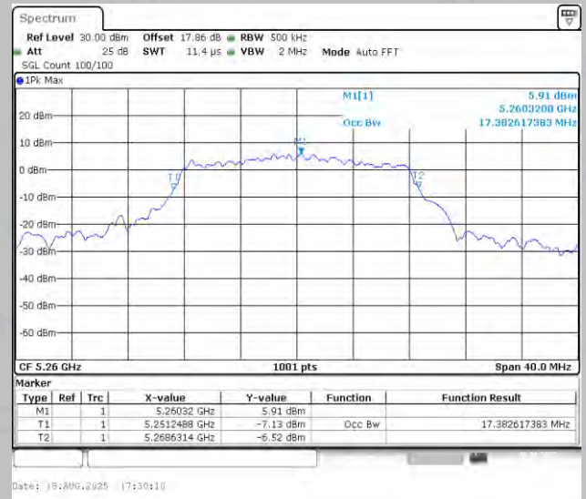
11A-Ant2-5260
