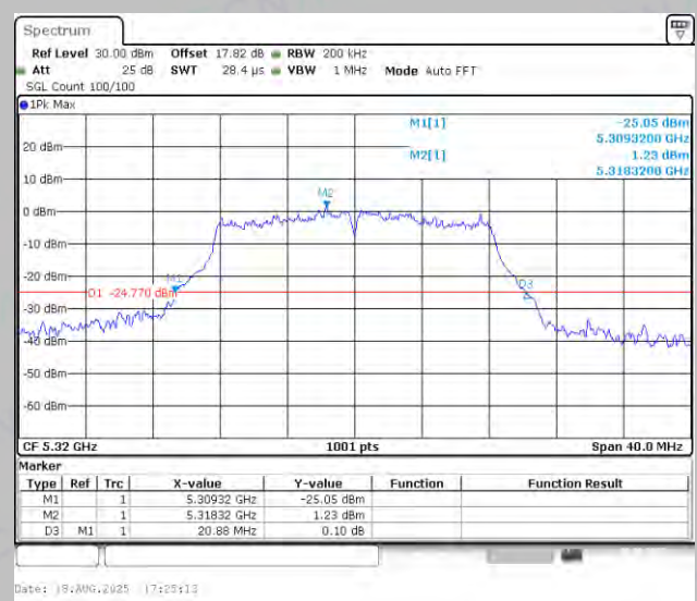
11A-Ant2-5320
