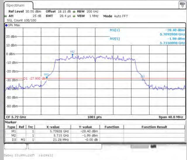
11AC20MIMO-Ant2-5720
