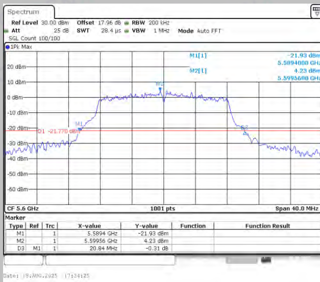
11A-Ant1-5600
