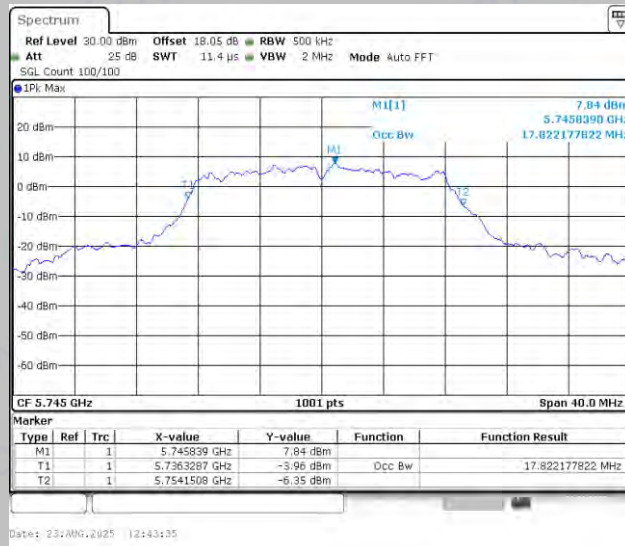
11A-Ant2-5745
