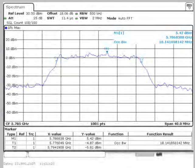
11N20MIMO-Ant2-5785
