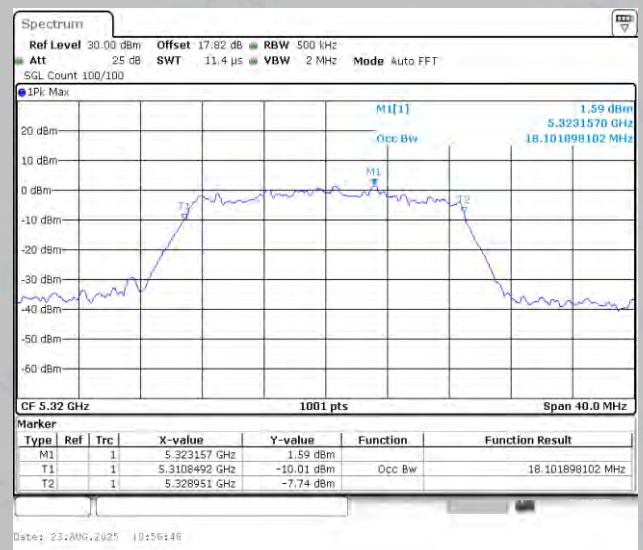
11N20MIMO-Ant2-5320
