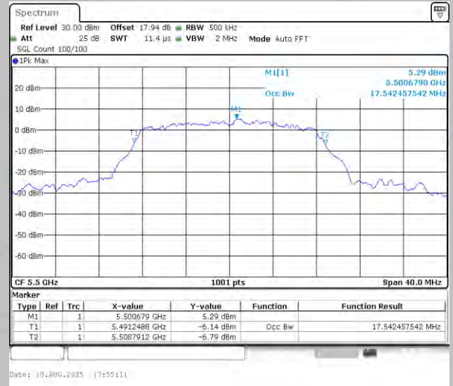
11A-Ant2-5500
