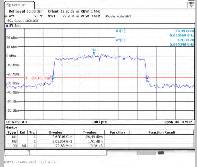
11AC80MIMO-Ant1-5690
