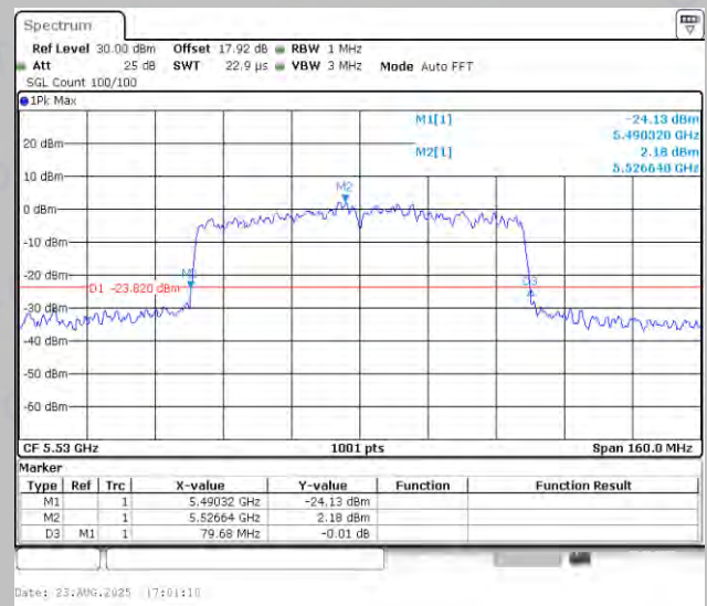
11AC80MIMO-Ant2-5530
