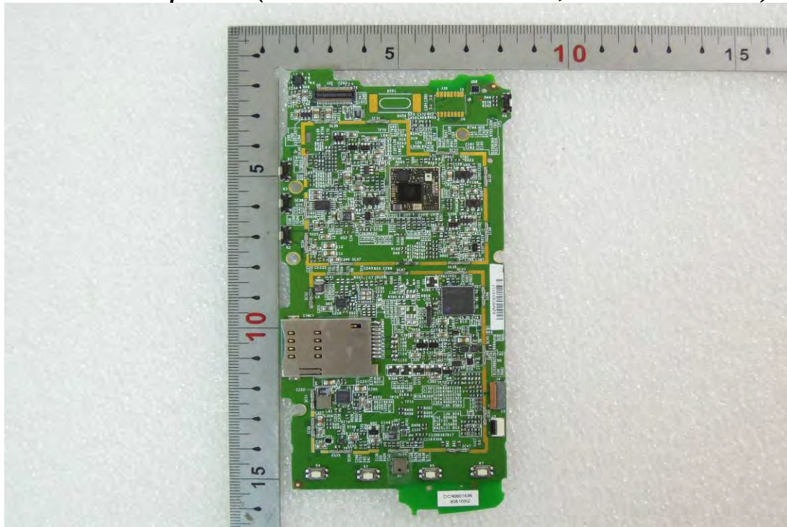
Internal View of EUT-40(Model no.: JUNO/T41/5-BWCSG; JUNO/T41/5-BWCRG)
