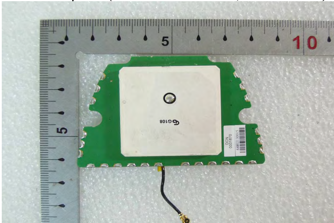
Internal View of EUT-44(Model no.: JUNO/T41/5-BWCSG; JUNO/T41/5-BWCRG)
