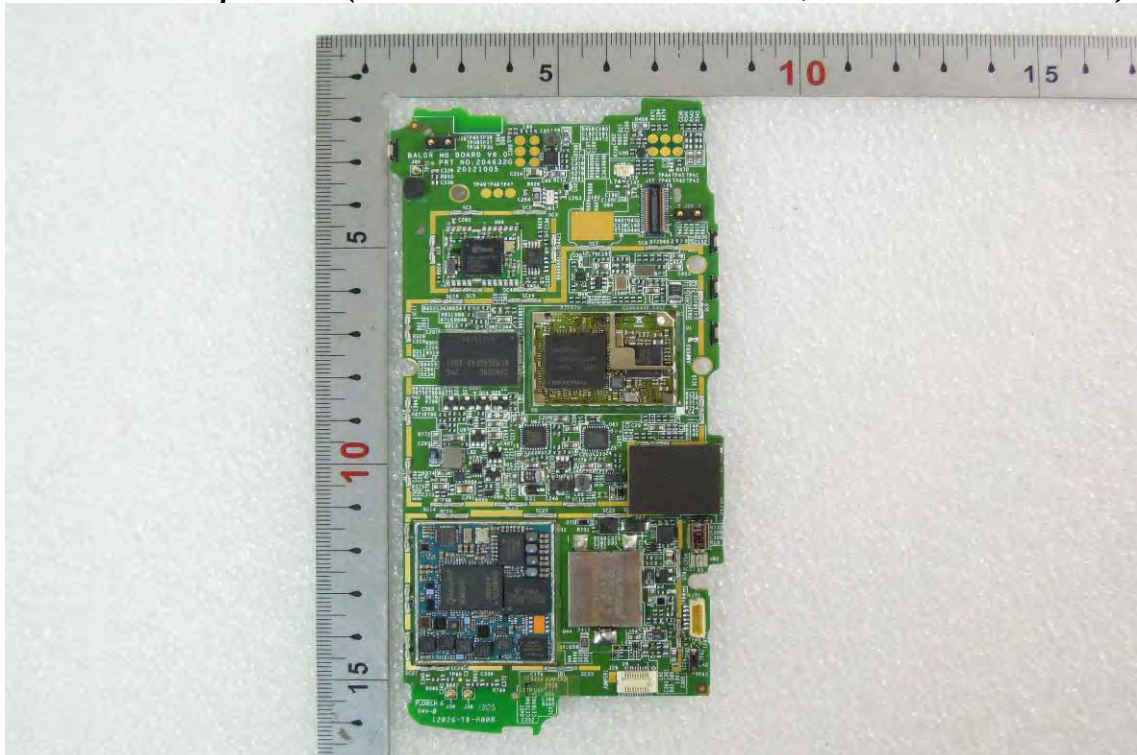
Internal View of EUT-42(Model no.: JUNO/T41/5-BWCSG; JUNO/T41/5-BWCRG)
