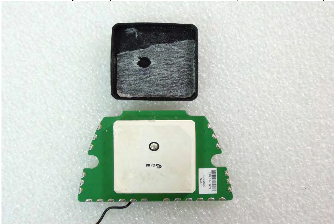
Internal View of EUT-18(Model no.: JUNO/T41/5-BWCSG; JUNO/T41/5-BWCRG)
