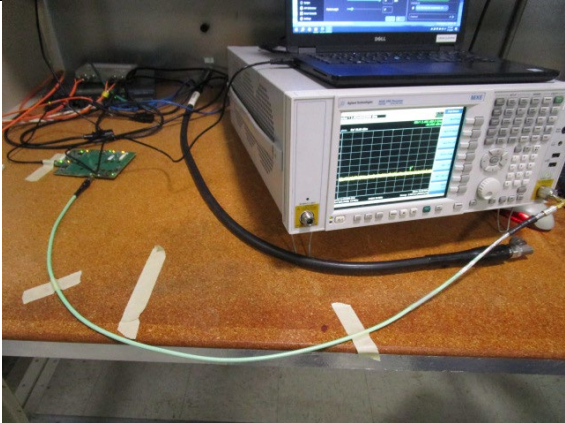
Conducted Setup
