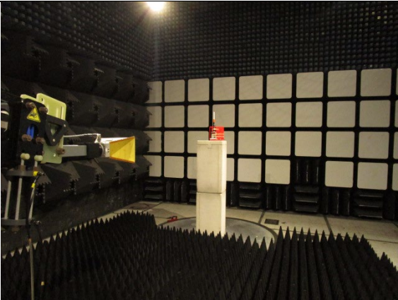
Radiated Setup
