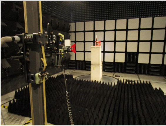
Radiated Setup
