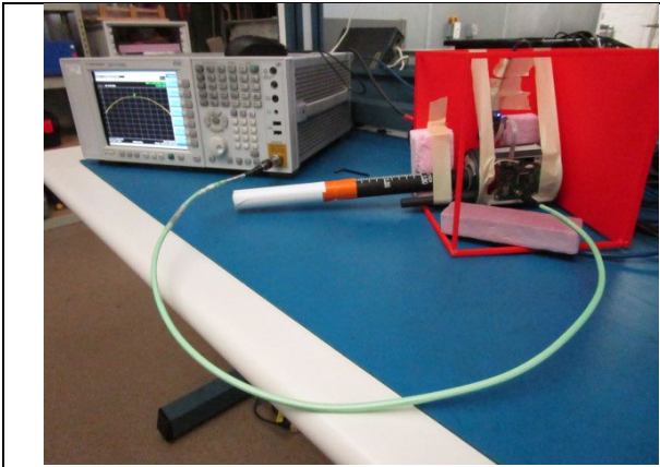
Conducted Setup
