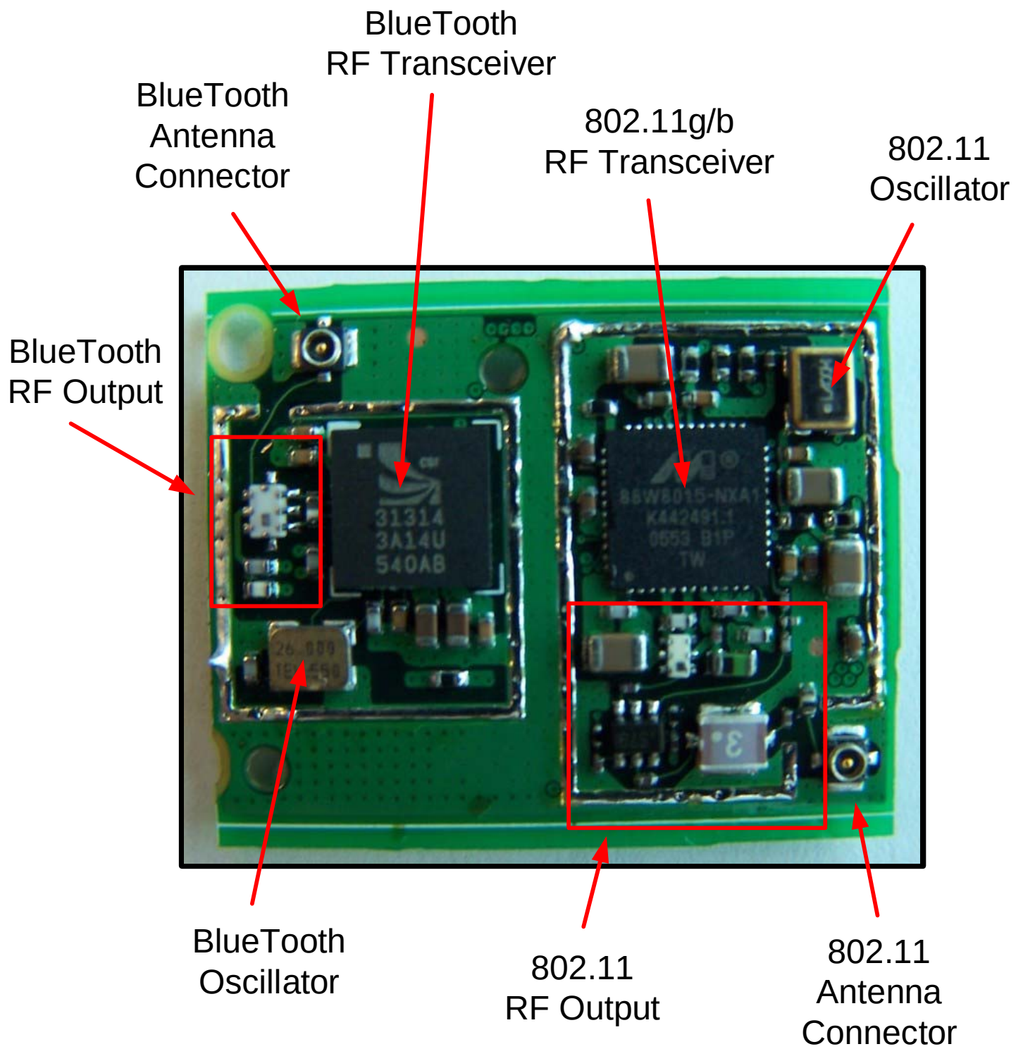
USI WM-BG-MR-01 Bluetooth / 802.11g Combo Module Top View Under Shielding
