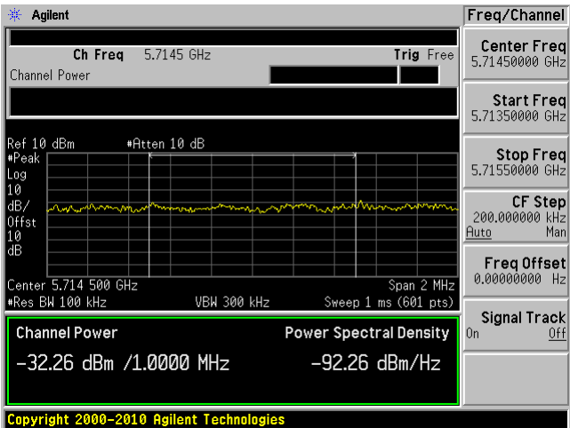
802.11ac 80, Chain 2 Low Band Edge
