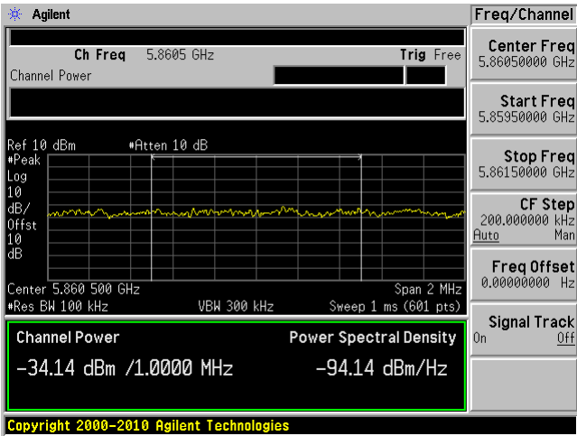
802.11ac 80, Chain 1 High Band Edge
