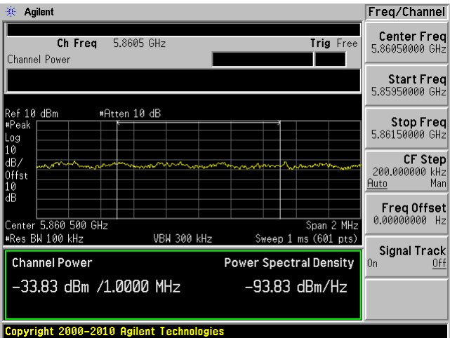
802.11ac 80, Chain 2 High Band Edge
