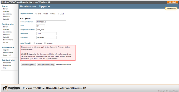
Figure 2: Sample Maintenance > Upgrade Page
