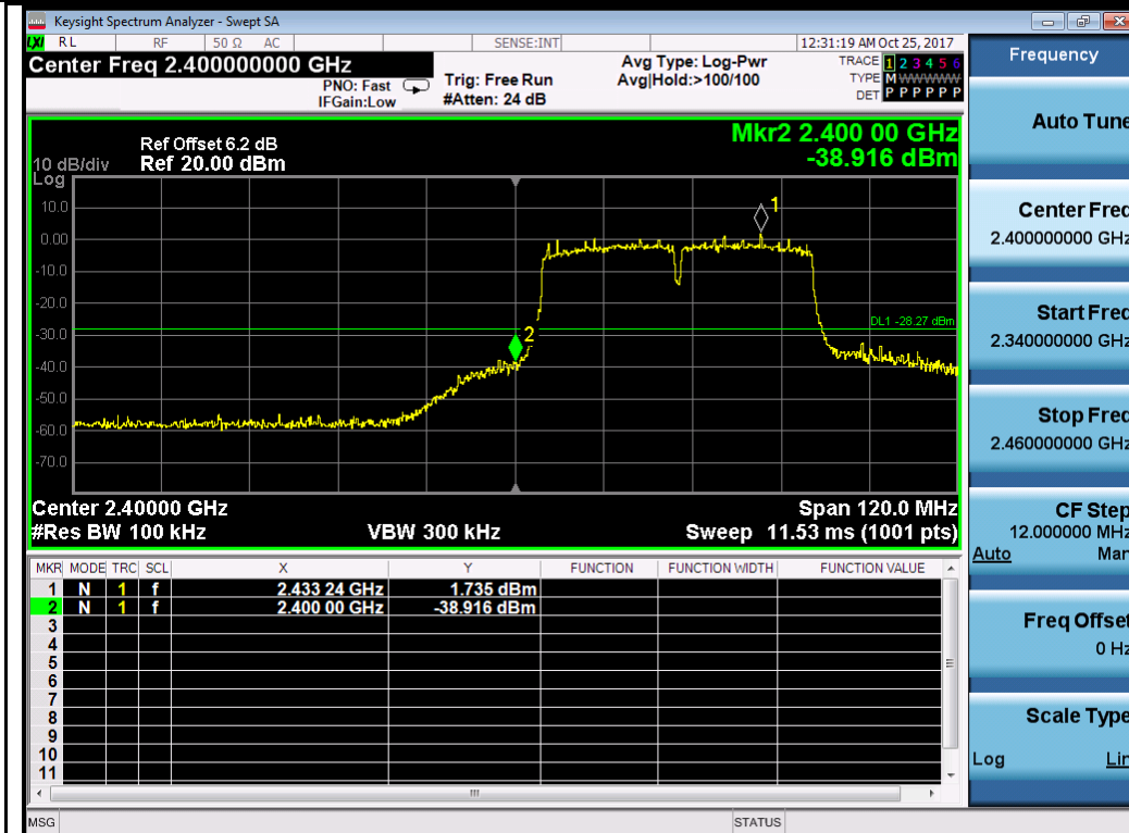
802.11n-HT40-2422MHz Chain 0
