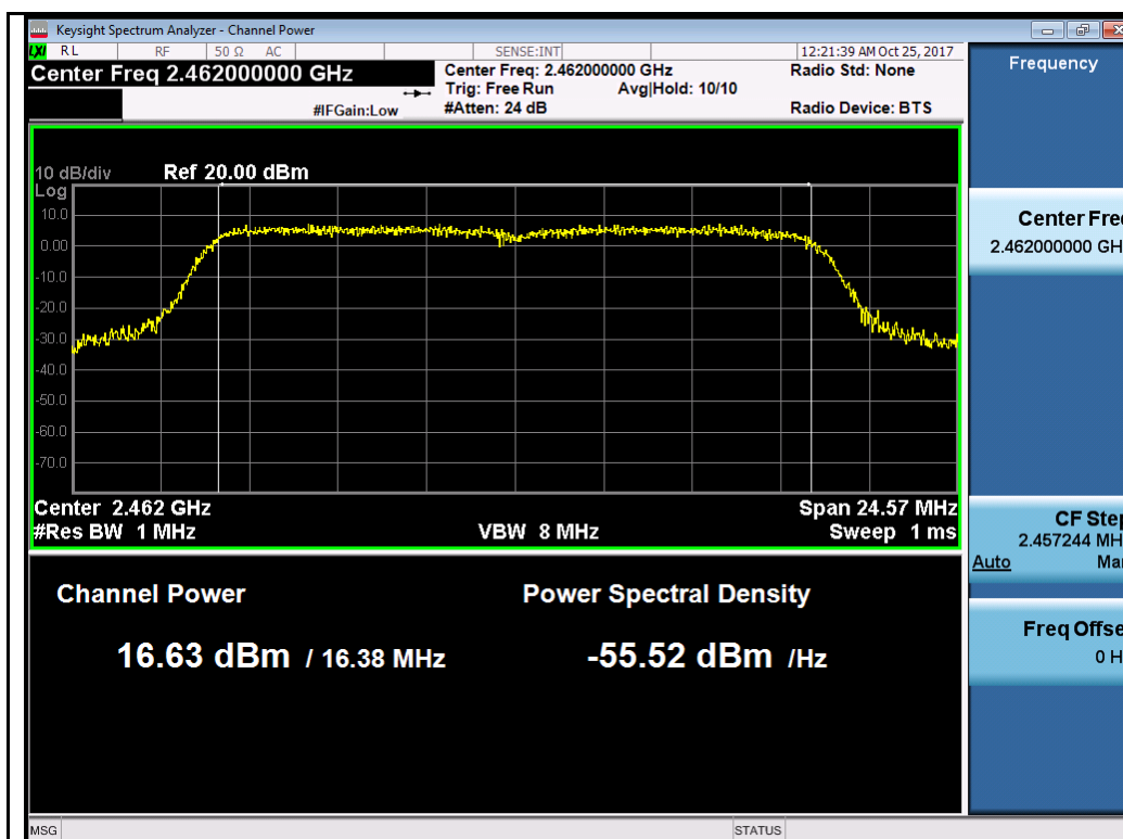
802.11g-2462MHz Chain 0
