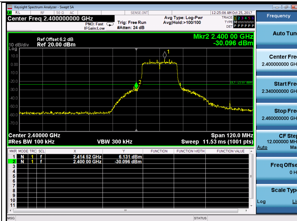
802.11n-HT20-2412MHz Chain 0
