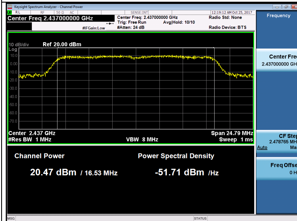
802.11g-2437MHz Chain 1
