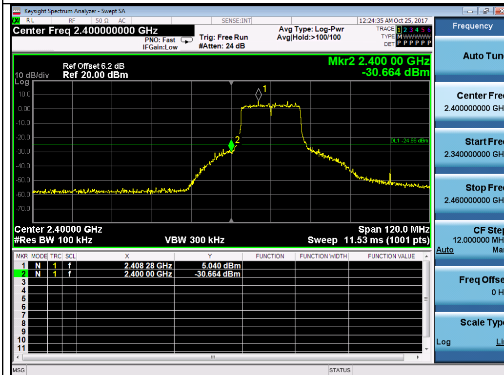
802.11n-HT20-2412MHz Chain 1
