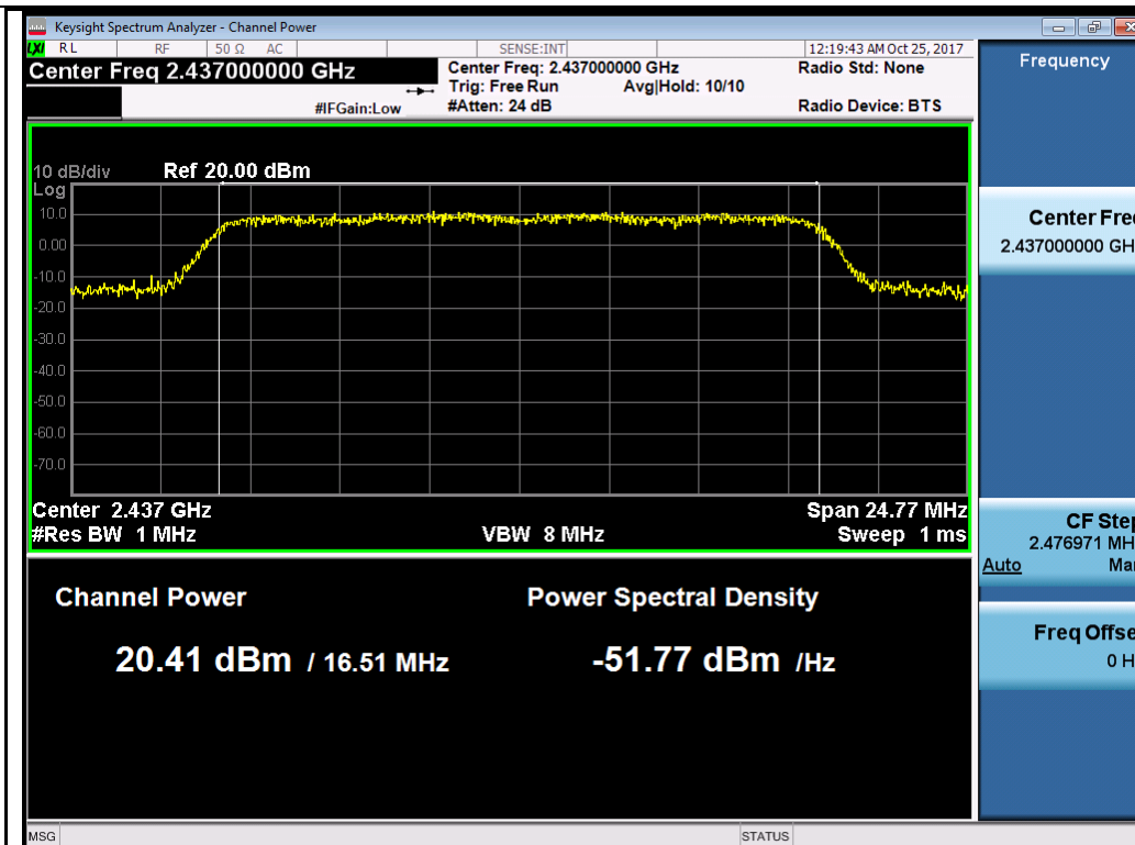
802.11g-2437MHz Chain 0
