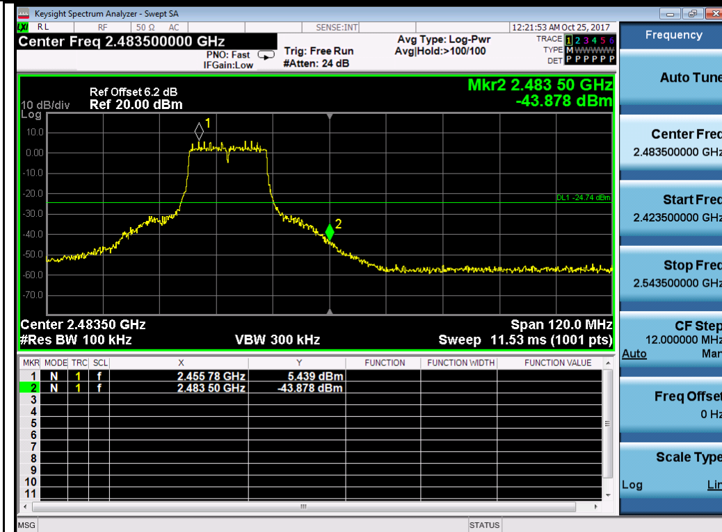
802.11g-2462MHz Chain 0
