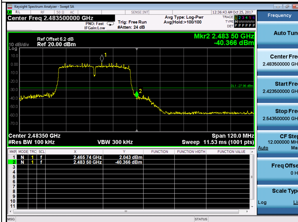
802.11n-HT40-2452MHz Chain 1
