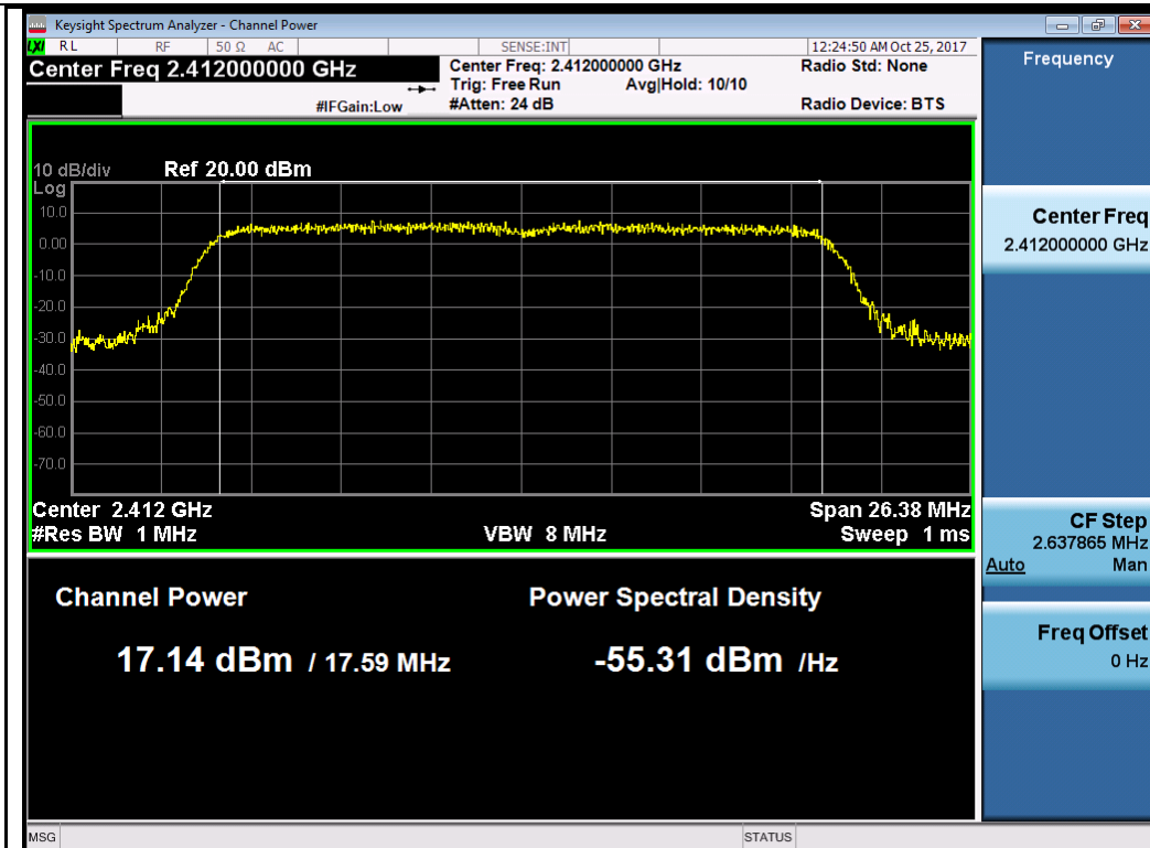
802.11n-HT20 2412MHz Chain 0
