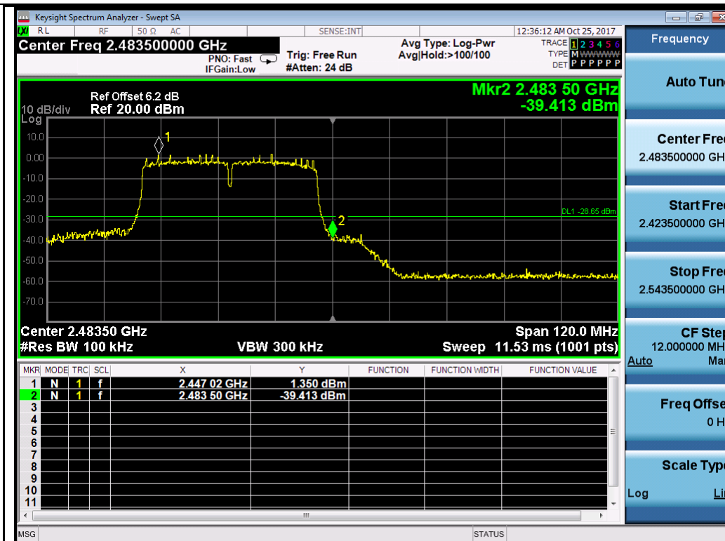
802.11n-HT40-2452MHz Chain 0
