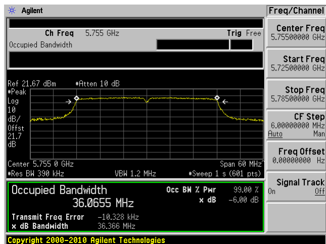
Low Channel 99% dB OBW ANT J15
