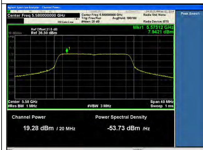
PSD-802.11n-20-5580M-chain0
