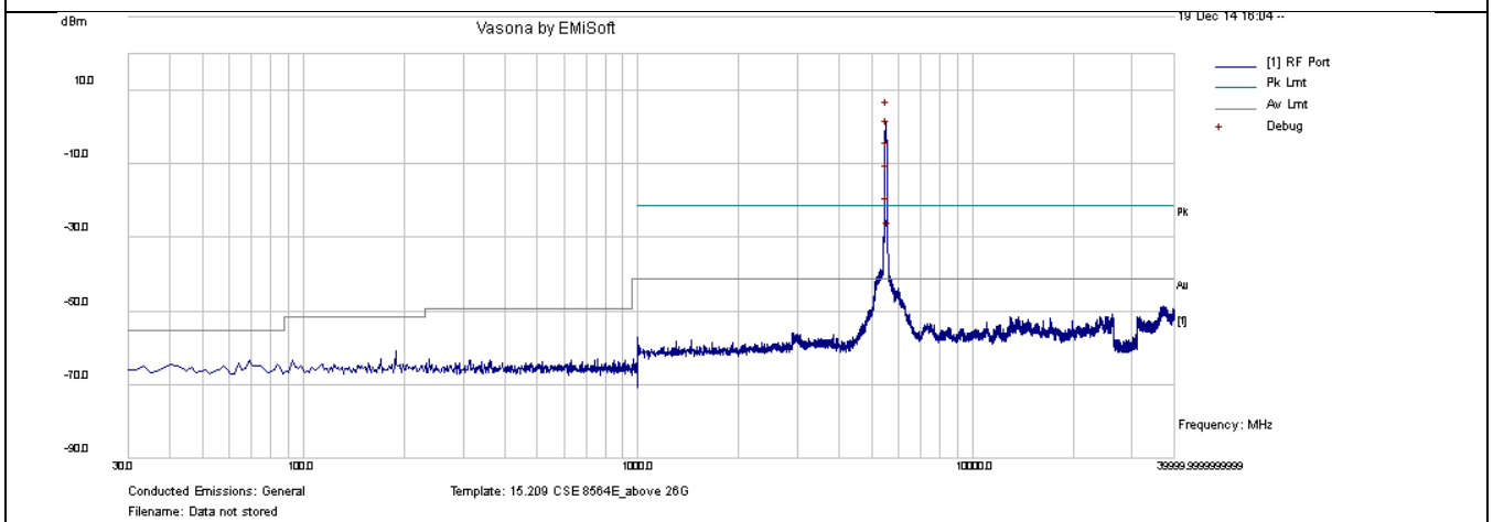
CSE-802.11n-40M-5510MHz-chain1
