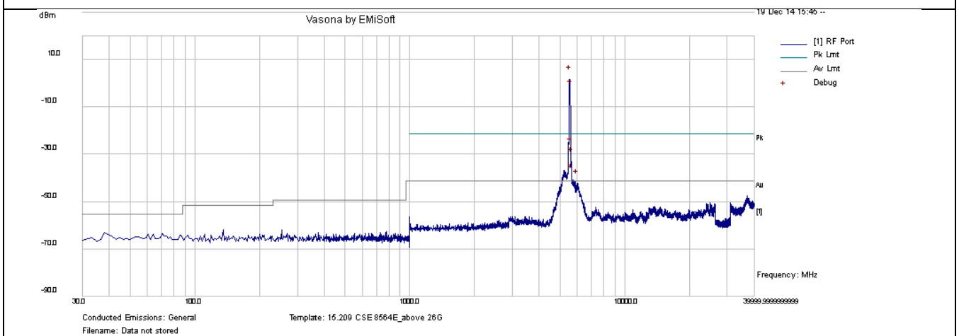
CSE-802.11n-40M-5550MHz-chain0
