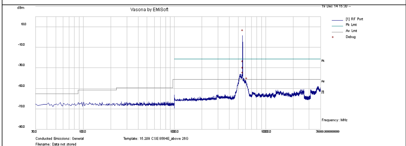
CSE-802.11n-20M 5580MHz-chain0
