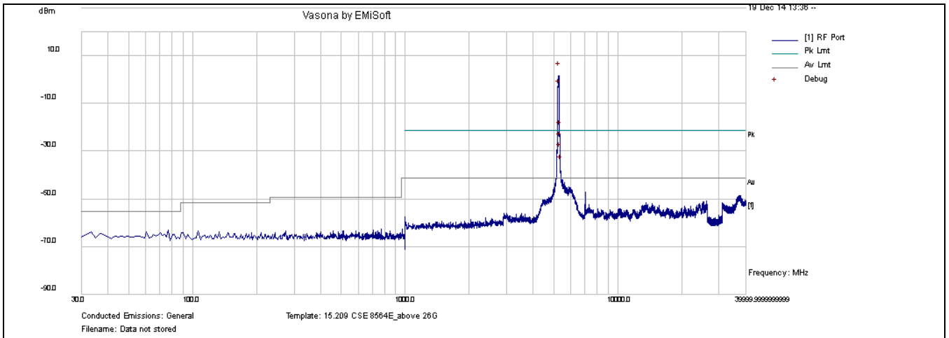
CSE-802.11n-40M 5270MHz-chain0
