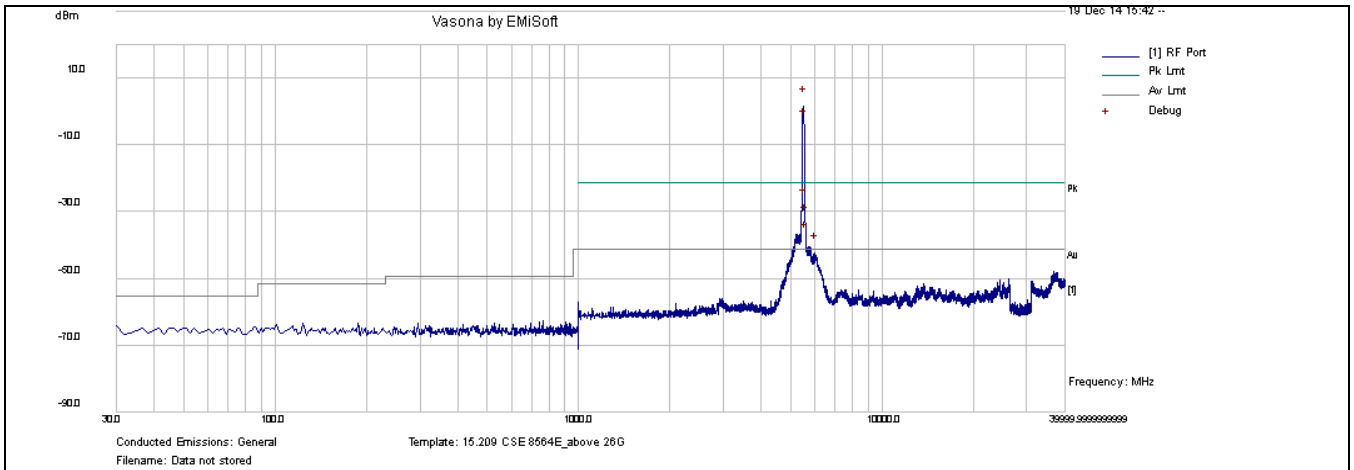
CSE-802.11n-40M-5510MHz-chain0
