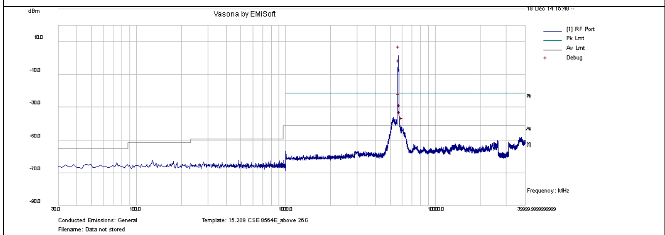
CSE-802.11n-40M-5670MHz-chain0
