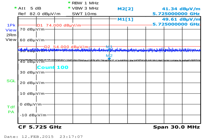
Restricted Band-802.11ac-80M 5530M– Edge Freq 5725MHz
