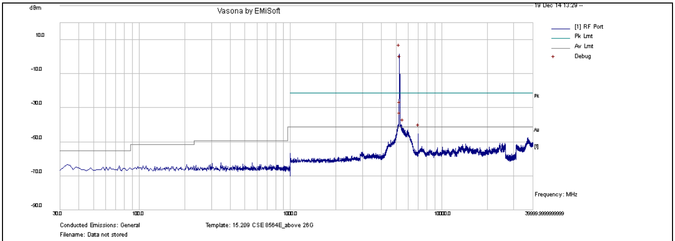
CSE-802.11n-20M 5260MHz-chain0
