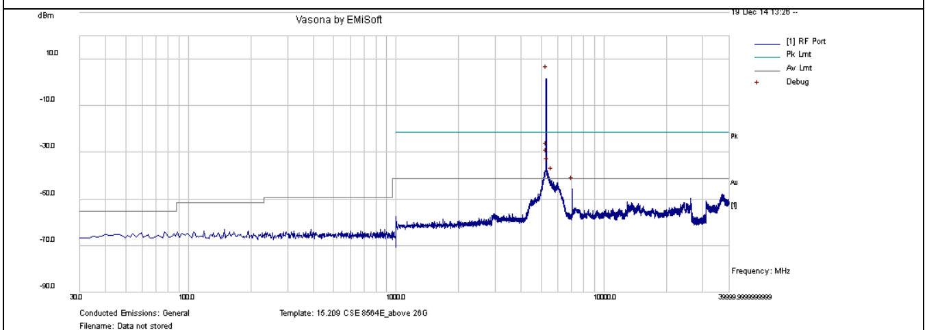
CSE-802.11n-20M 5280MHz-chain0
