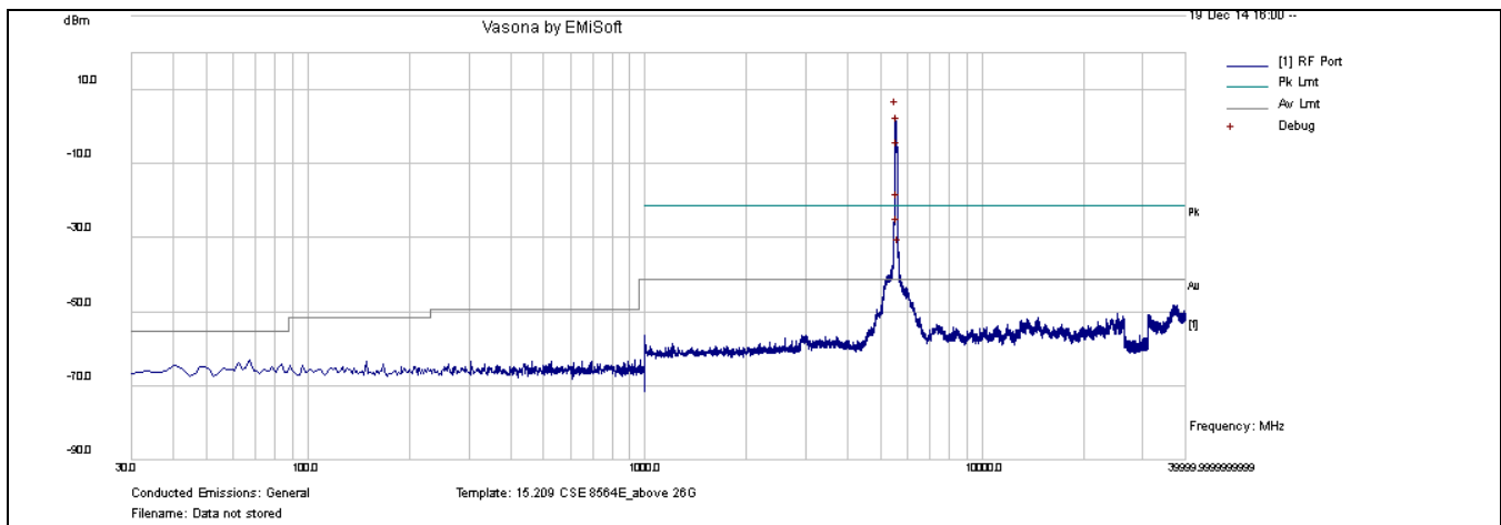
CSE-802.11n-40M-5550MHz-chain1
