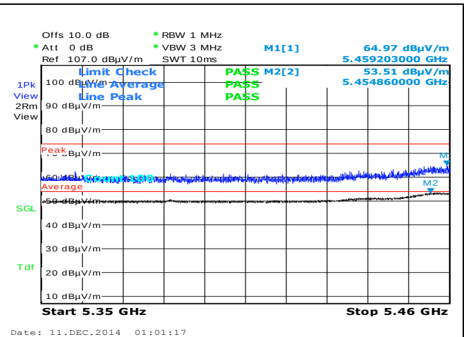
Restrictd Band-802.11ac-80M 5530M– Edge Freq 5460MHz
