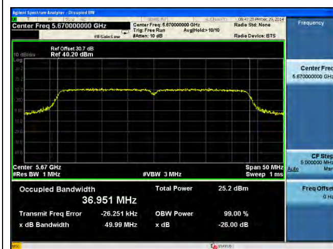
26dB BW - 802.11n-40M 5570MHz
