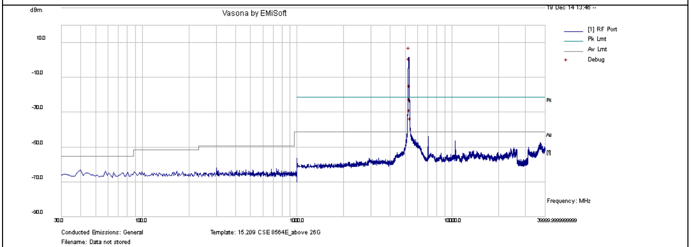
CSE-802.11n-40M 5270MHz-chain1
