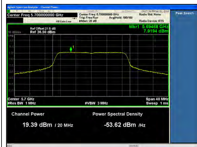
PSD-802.11n-20-5700M-chain0
