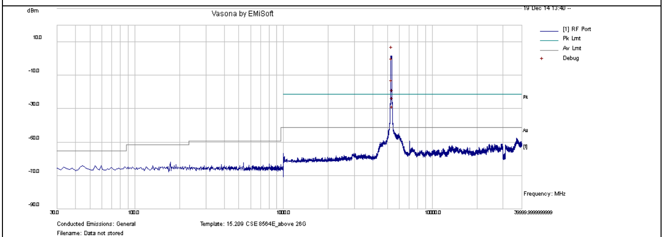
CSE-802.11n-40M 5310MHz-chain0
