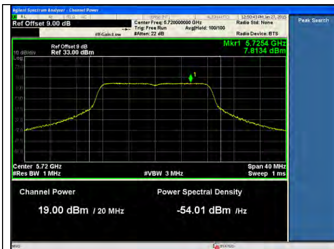
PSD-802.11a-5720M-chain0
