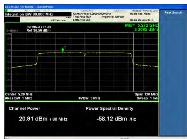
PSD-802.11ac-80M-5290M-chain1
