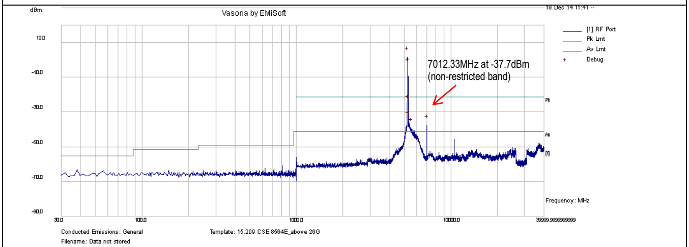
CSE-802.11n-20M 5260MHz-chain1
