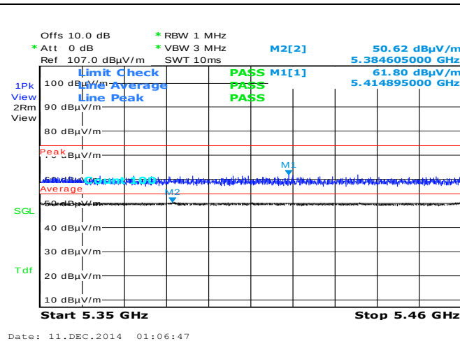
Restrictd Band-802.11n-40M 5510M– Edge Freq 5460MHz
