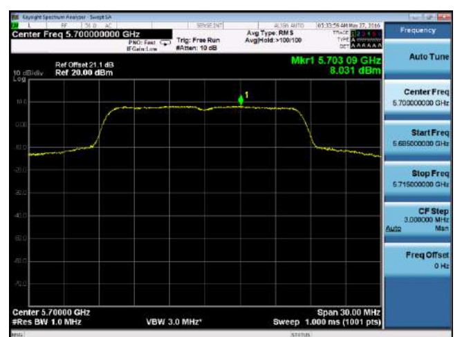
PSD-802.11a-5700M-chain1
