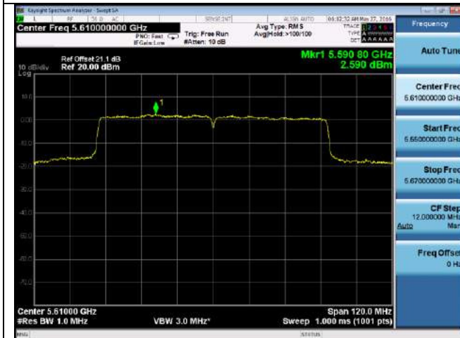
PSD-802.11ac-80M-5610M-chain0
