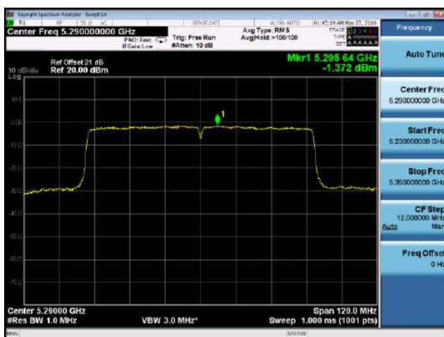
PSD-802.11ac-80M-5290M-chain0
