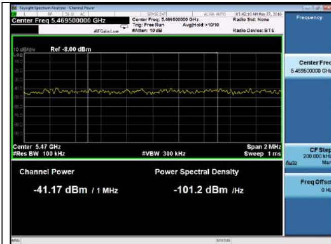
Band Edge -802.11n-20M -5500M-chain0
