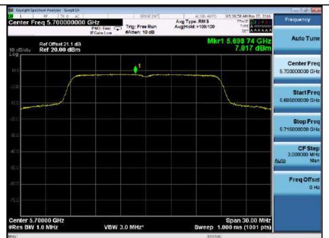
PSD-802.11n-20M-5700M-chain1
