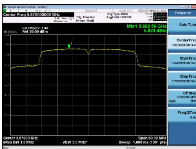
PSD-802.11n-40M-5670M-chain0
