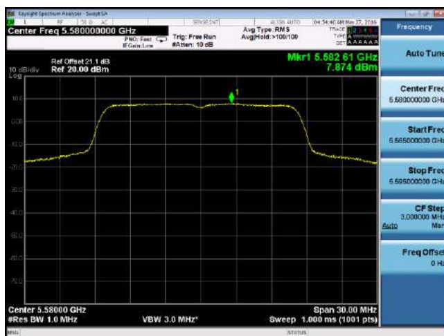
PSD-802.11a-5580M-chain0
