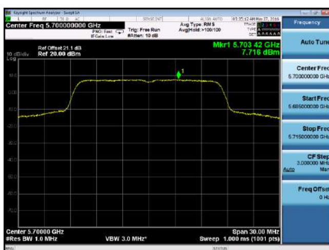
PSD-802.11a-5700M-chain0
