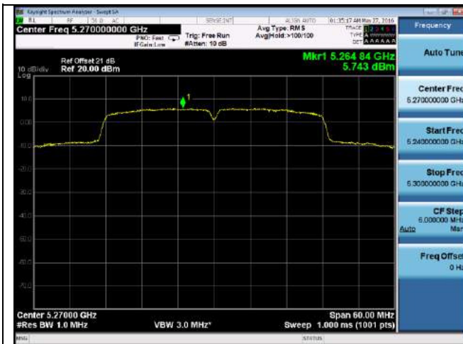
PSD-802.11n-40M-5270M-chain0
