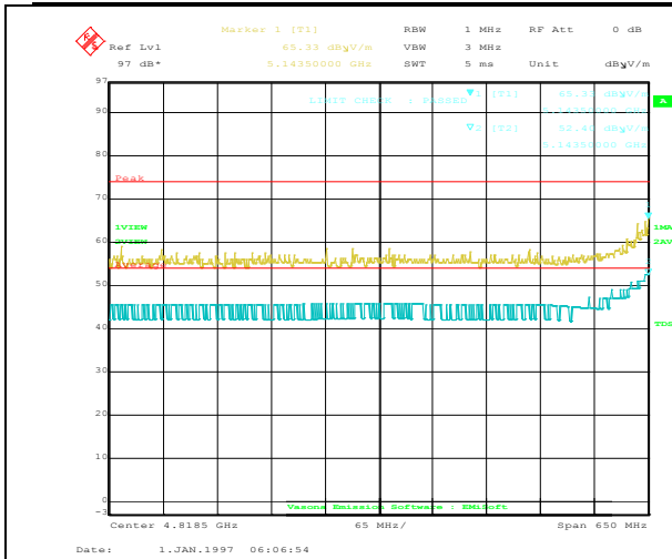
802.11ac-VHT80 5290M(4500-5150MHz)
