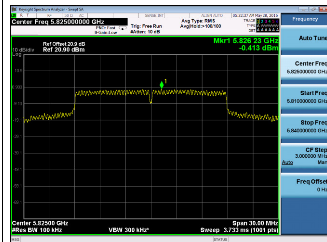
PSD-802.11n-20M -5825M-chain0
