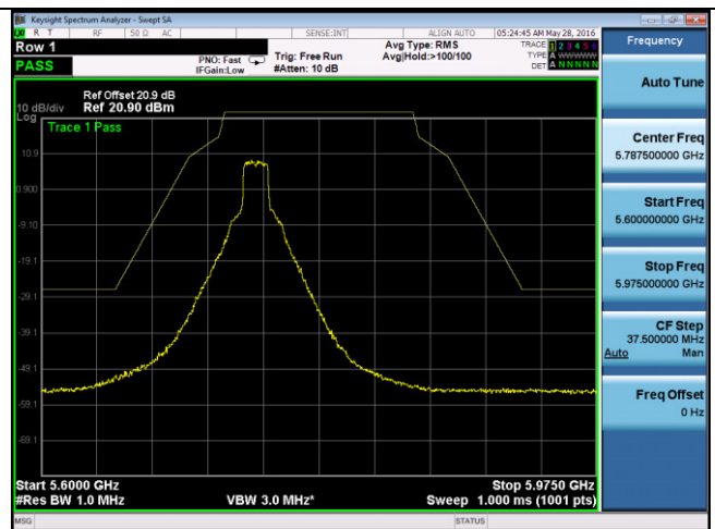
Emission Mask -802.11a-5745M-chain1
