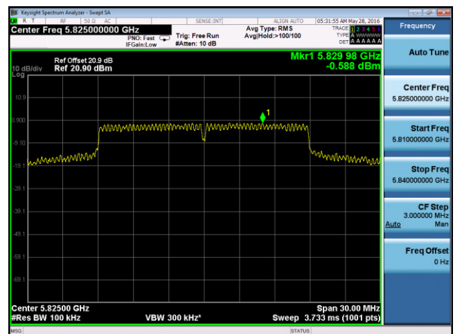
PSD-802.11n-20M -5825M-chain1
