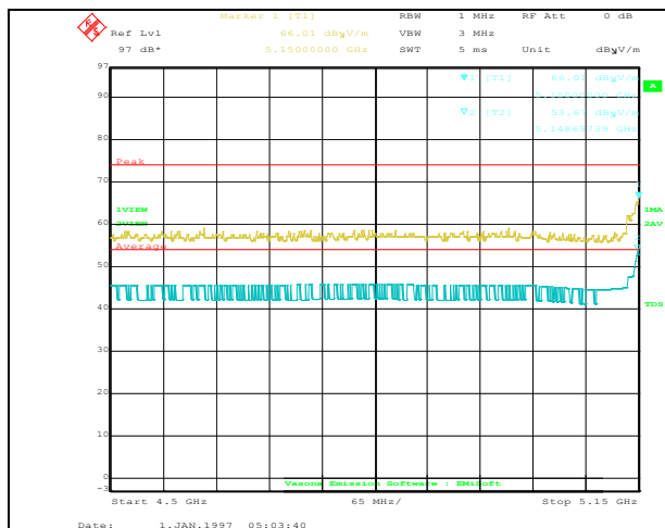
Restricted Band-802.11a 5180M- Edge Freq 5150MHz
