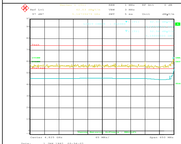
Restricted Band-802.11n-40M 5190M- Edge Freq 5150MHz
