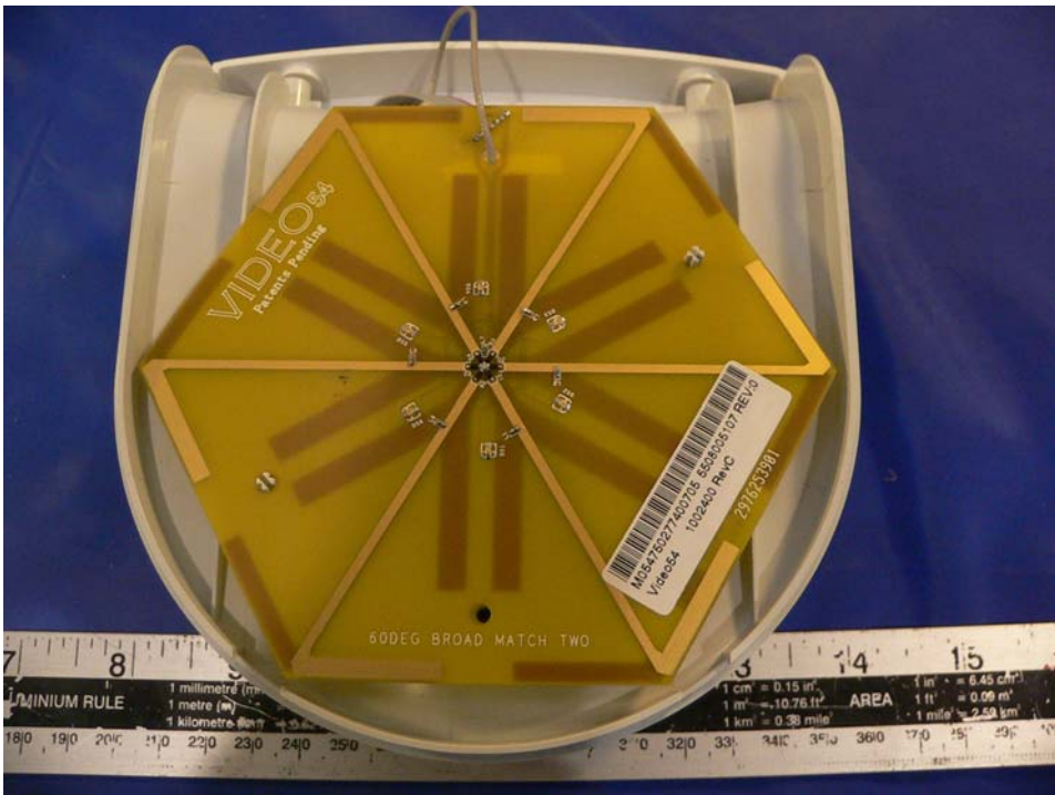
MM2225: EUT – Cover Off View 2
