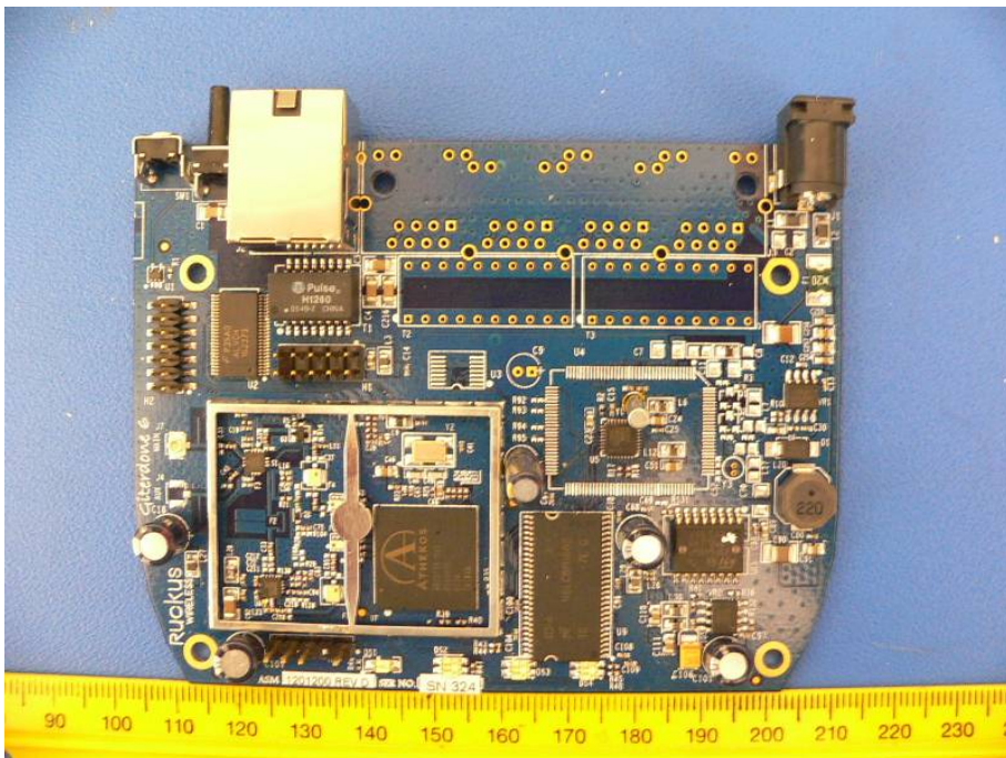
MM22X1: EUT – Main Board Component View
