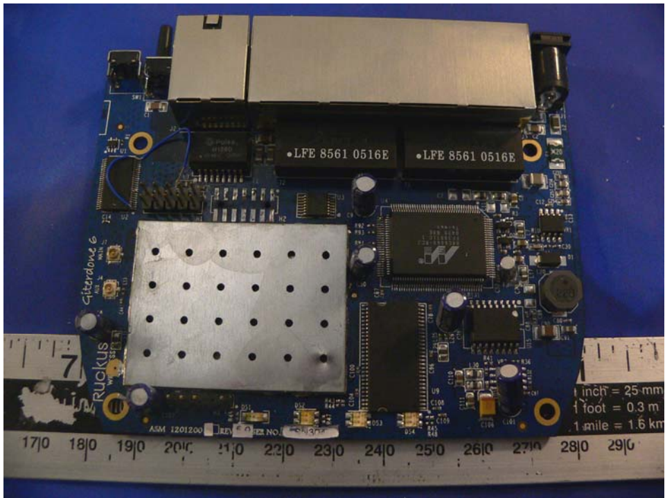
MM2225: EUT – Component View with shielding
