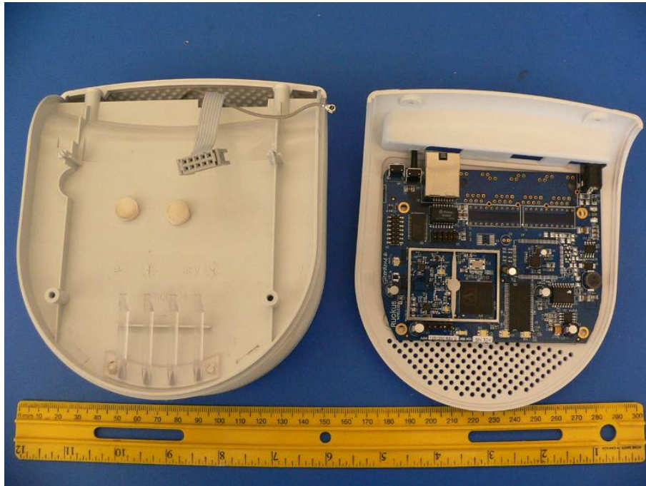
MM22X1: EUT – Cover Off View
