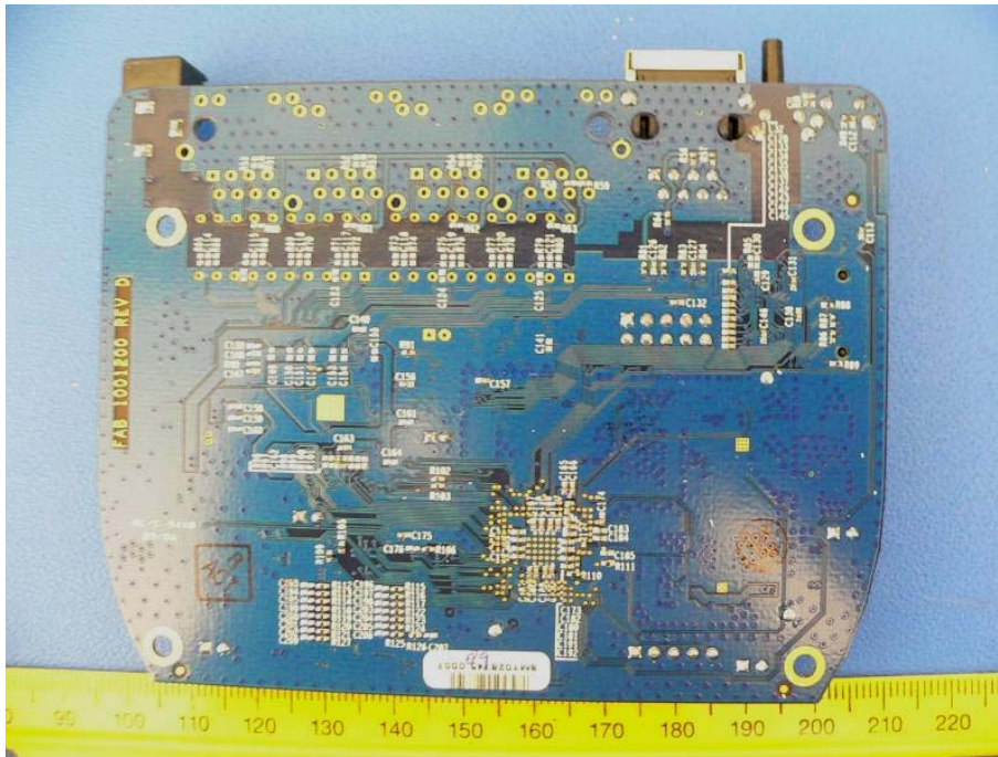
MM22X1: EUT – Main Board Solder View
