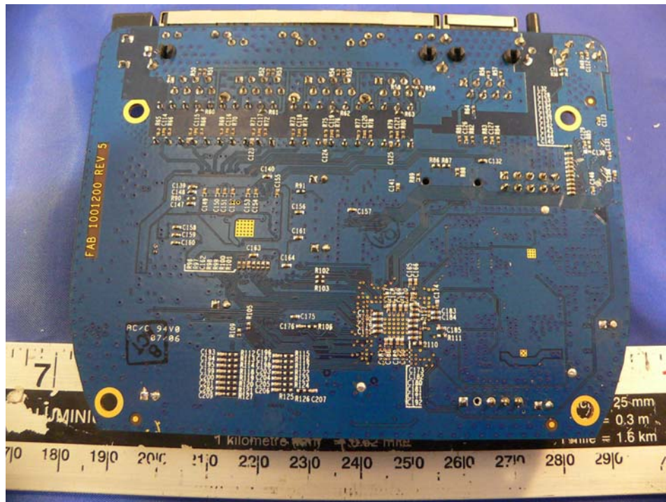
MM2225: EUT – Port View
