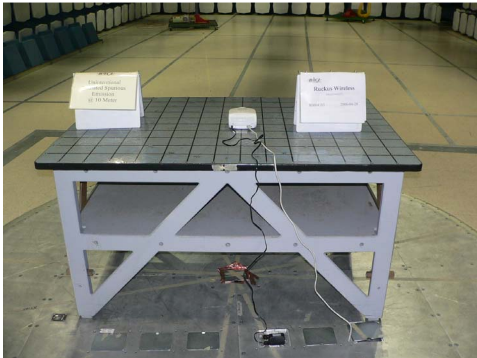
MM22X1: Radiated Emissions - Rear View
