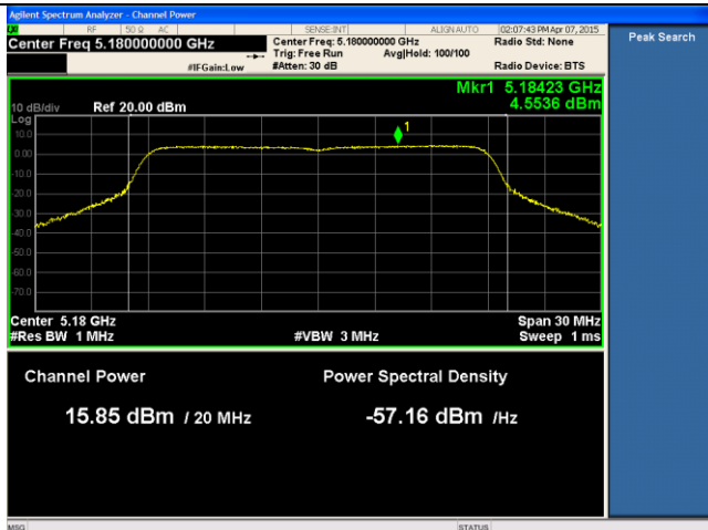
14dBi ANT-PSD-802.11n-HT20-5180M-chain1
