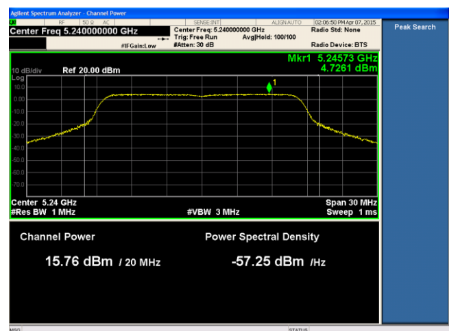
21dBi ANT-PSD-802.11a-5240M-chain2
