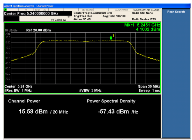
14dBi ANT-PSD-802.11n-HT20-5240M-chain2
