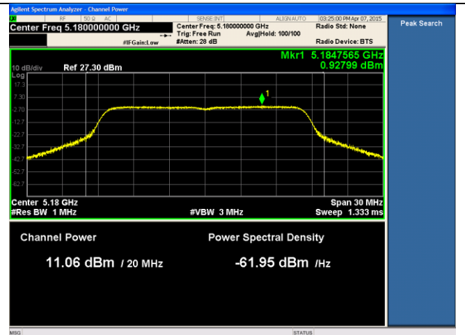
24dBi ANT-PSD-802.11a-5180M-chain2
