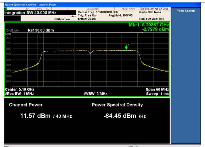
24dBi ANT-PSD-802.11n-HT40-5190M-chain2
