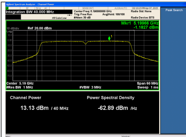
14dBi ANT-PSD-802.11n-HT40-5190M-chain1
