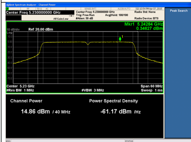
14dBi ANT-PSD-802.11n-HT40-5230M-chain1
