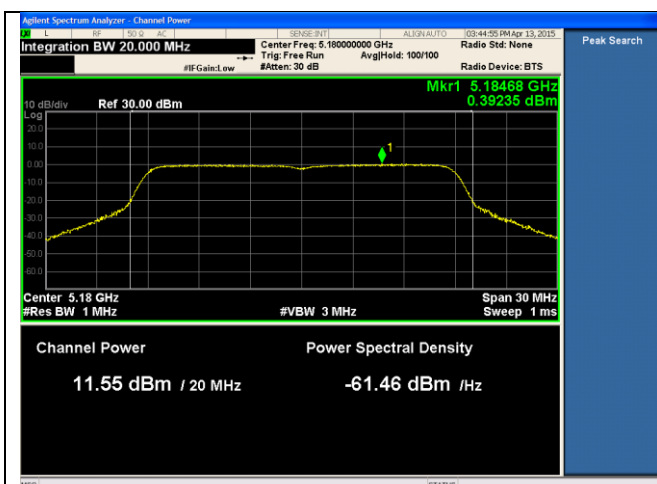
21dBi ANT-PSD-802.11n-HT20-5180M-chain1
