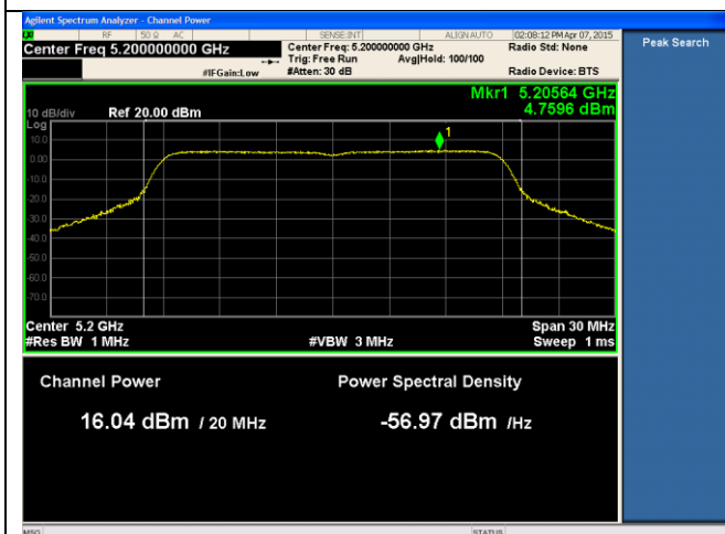
21dBi ANT-PSD-802.11n-HT20-5200M-chain1
