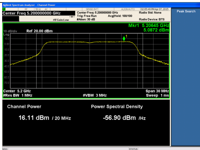
24dBi ANT-PSD-802.11a-5200M-chain1
