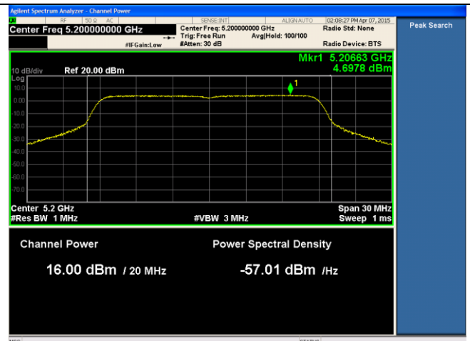
14dBi ANT-PSD-802.11n-HT20-5200M-chain2
