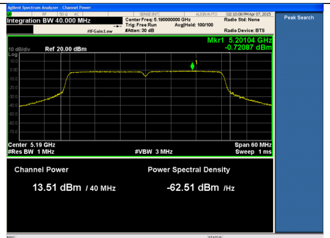
14dBi ANT-PSD-802.11n-HT40-5190M-chain2
