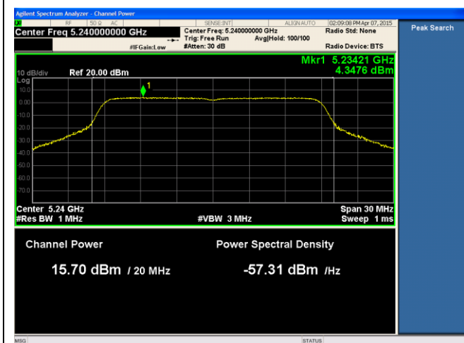
21dBi ANT-PSD-802.11n-HT20-5240M-chain1
