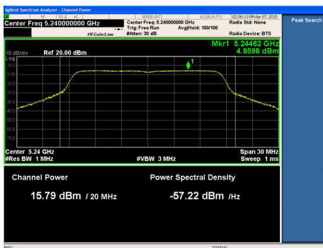
21dBi ANT-PSD-802.11a-5240M-chain1
