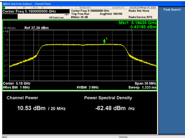
24dBi ANT-PSD-802.11a-5180M-chain1
