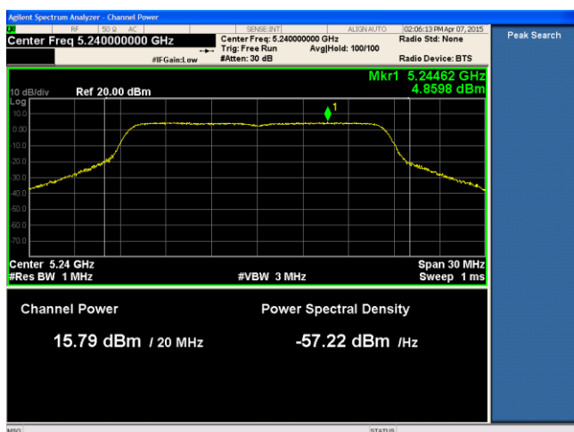
24dBi ANT-PSD-802.11a-5240M-chain1
