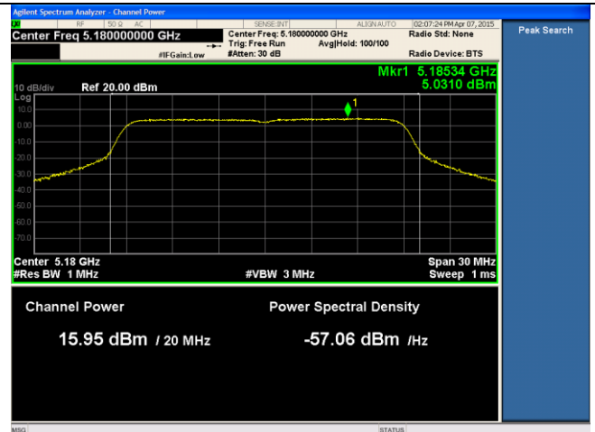
14dBi ANT-PSD-802.11n-HT20-5180M-chain2
