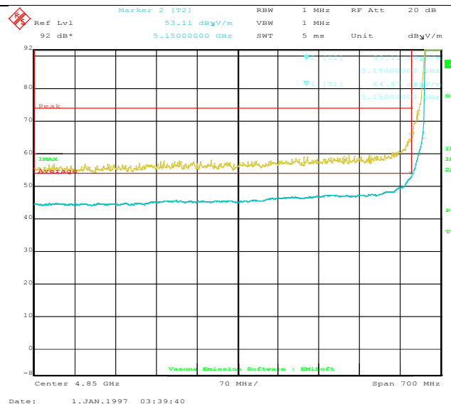
Restricted Band-802.11ac 5210M- Edge Freq 5150MHz
