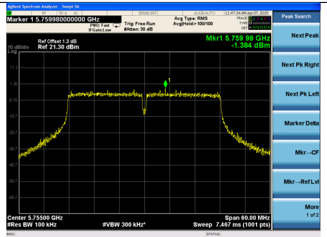
14dB ANT-PSD-802.11n-HT40-5755M-chain2
