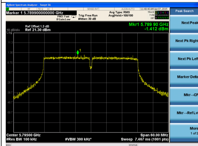
24dB ANT-PSD-802.11n-HT40-5795M-chain1
