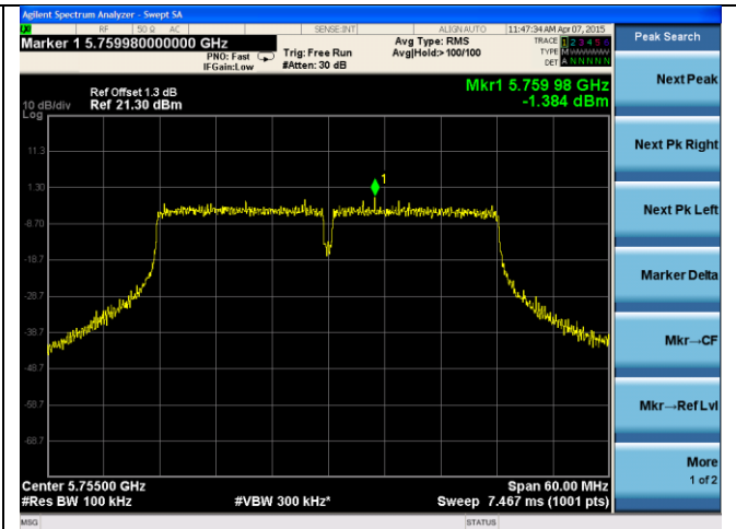
21dB ANT-PSD-802.11n-HT40-5755M-chain2
