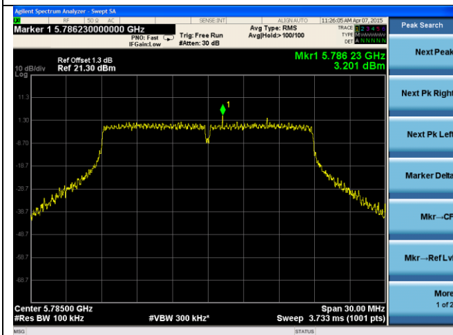
24dB ANT-PSD-802.11n-HT20-5785M-chain1
