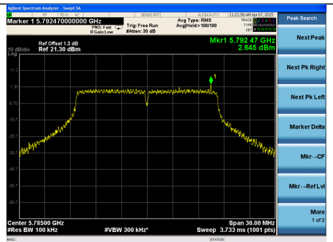
21dB ANT-PSD-802.11a-5785M-chain2
