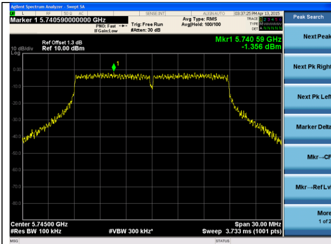
24dB ANT-PSD-802.11n-HT20-5745M-chain1
