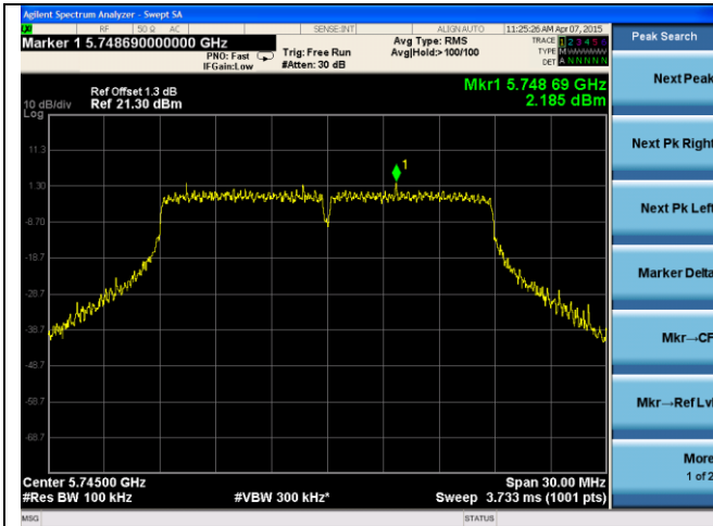
14dB ANT-PSD-802.11n-HT20-5745M-chain1
