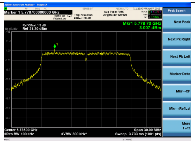
24dB ANT-PSD-802.11n-HT20-5785M-chain2
