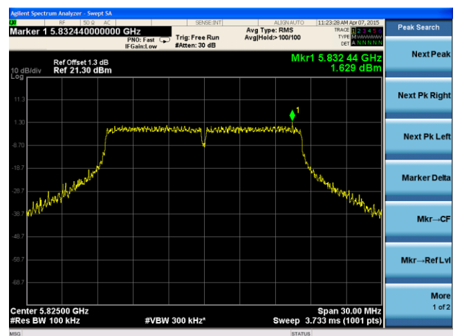
24dB ANT-PSD-802.11a-5825M-chain2
