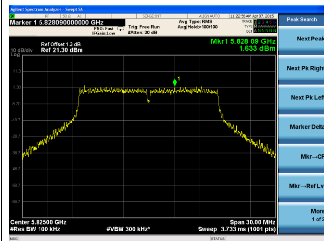
21dB ANT-PSD-802.11a-5825M-chain1
