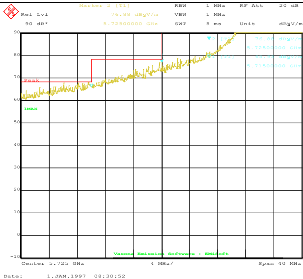
Restricted Band-802.11ac 5775M- Edge Freq 5725MHz
