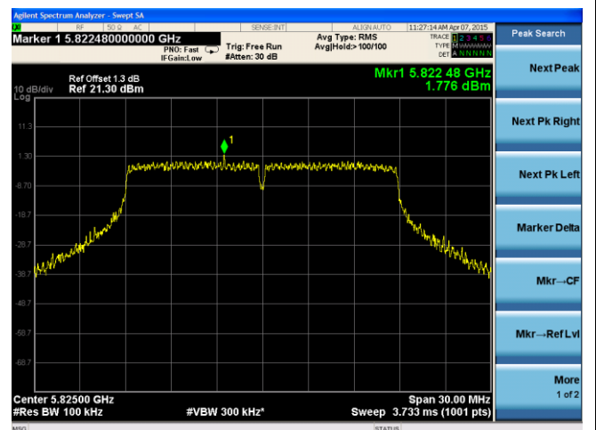
14dB ANT-PSD-802.11n-HT20-5825M-chain2
