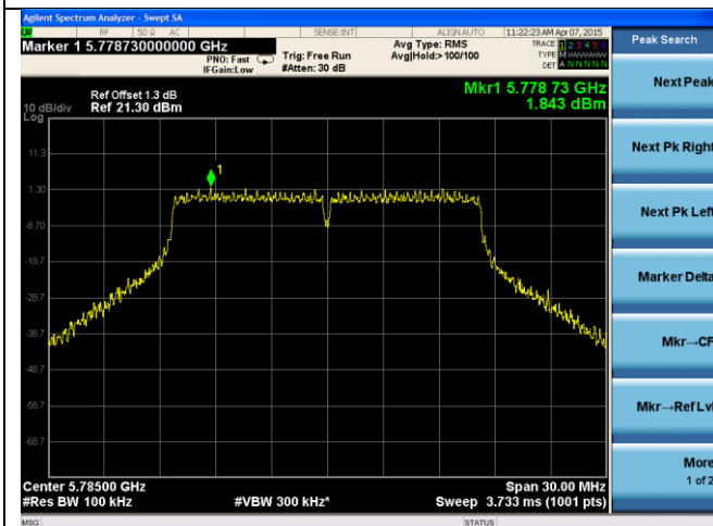
24dB ANT-PSD-802.11a-5785M-chain1
