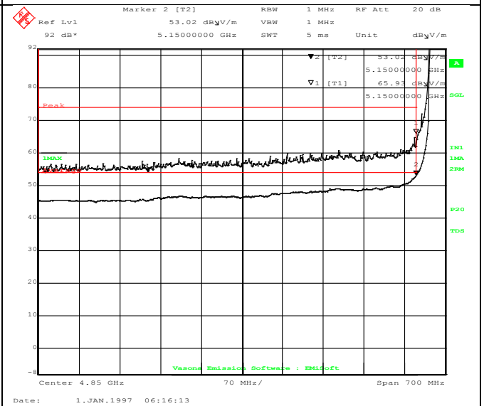
Restricted Band-802.11ac 5210M– Edge Freq 5150MHz
