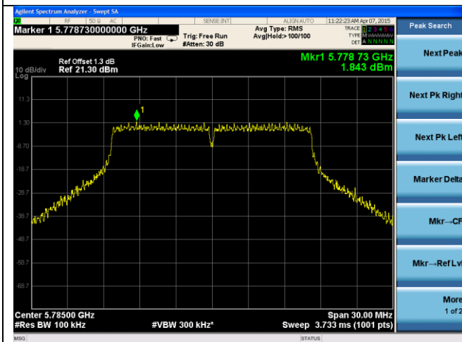
14dB ANT-PSD-802.11a-5785M-chain1
