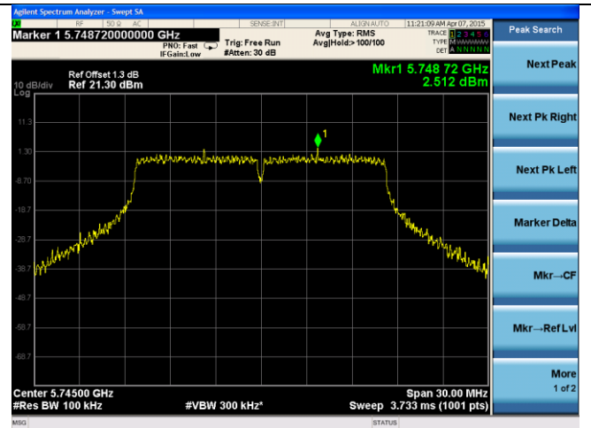
21dB ANT-PSD-802.11a-5745M-chain2
