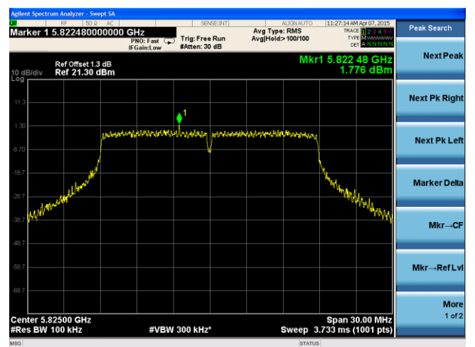
24dB ANT-PSD-802.11n-HT20-5825M-chain2
