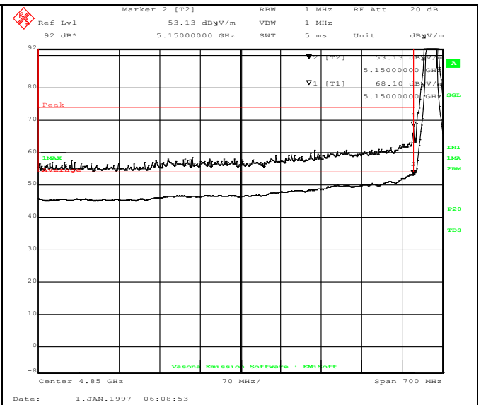
Restricted Band-802.11n-HT20 5180M– Edge Freq 5150MHz
