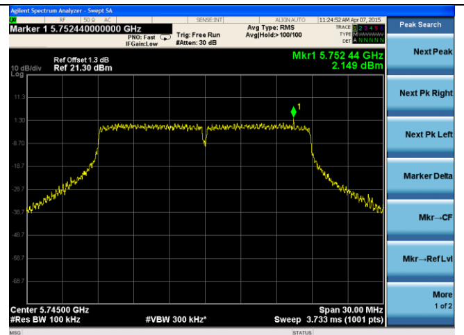
21dB ANT-PSD-802.11n-HT20-5745M-chain2
