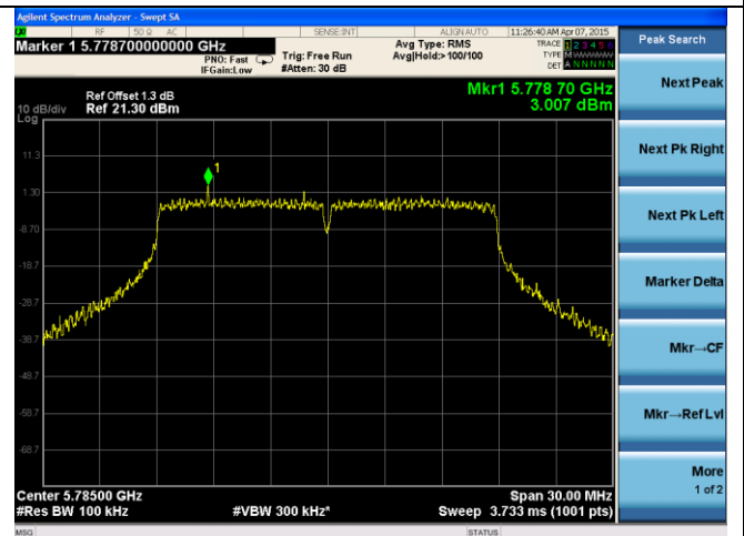
14dB ANT-PSD-802.11n-HT20-5785M-chain2
