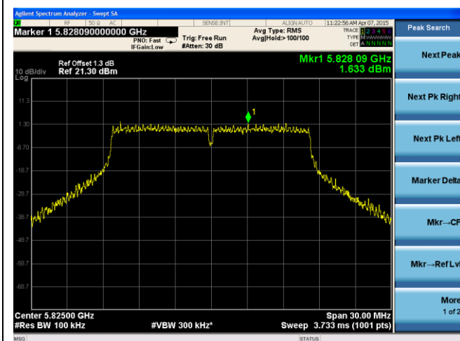
24dB ANT-PSD-802.11a-5825M-chain1
