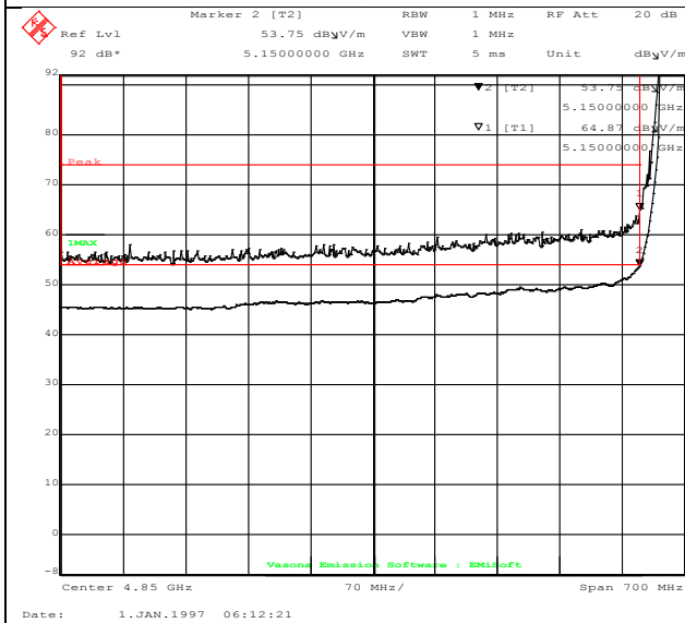
Restricted Band-802.11n-HT40 5190M– Edge Freq 5150MHz
