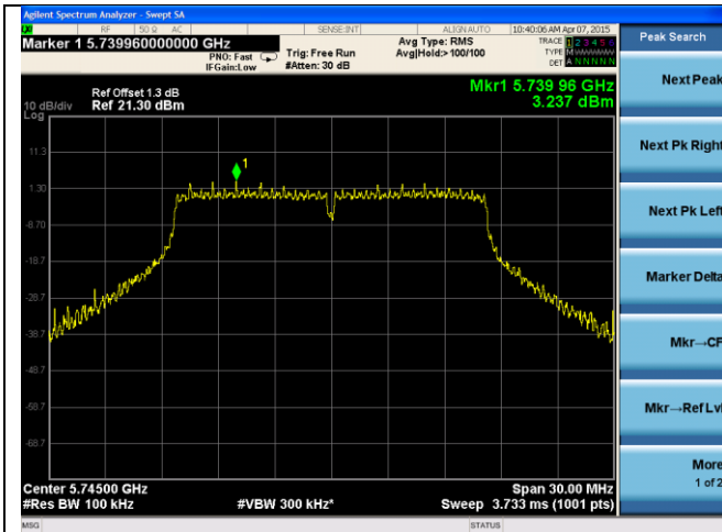
21dB ANT-PSD-802.11a-5745M-chain1
