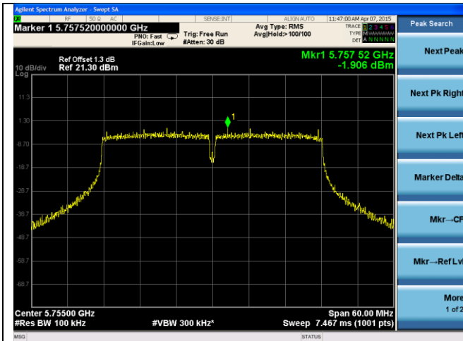
14dB ANT-PSD-802.11n-HT40-5755M-chain1
