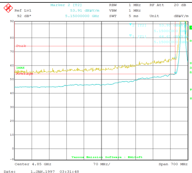
Restricted Band-802.11n-HT20 5180M- Edge Freq 5150MHz
