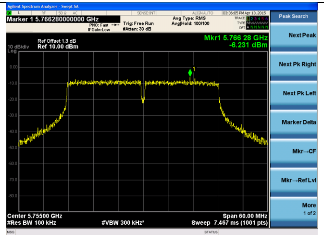
24dB ANT-PSD-802.11n-HT40-5755M-chain2
