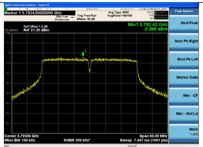
24dB ANT-PSD-802.11n-HT40-5795M-chain2
