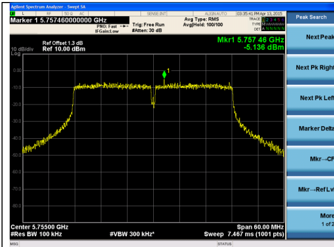
24dB ANT-PSD-802.11n-HT40-5755M-chain1
