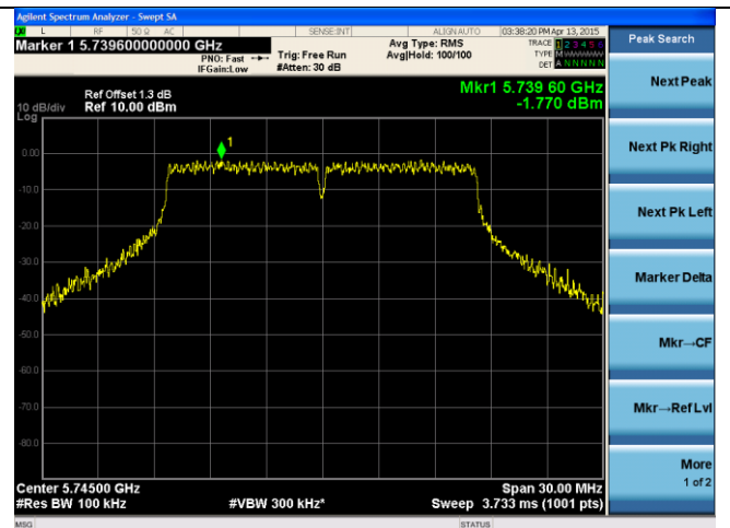
24dB ANT-PSD-802.11a-5745M-chain2
