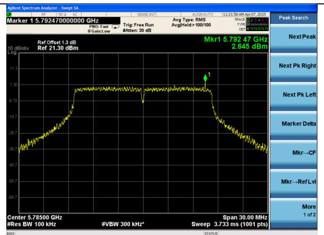
24dB ANT-PSD-802.11a-5785M-chain2
