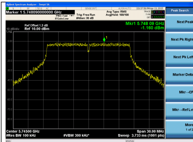
24dB ANT-PSD-802.11a-5745M-chain1
