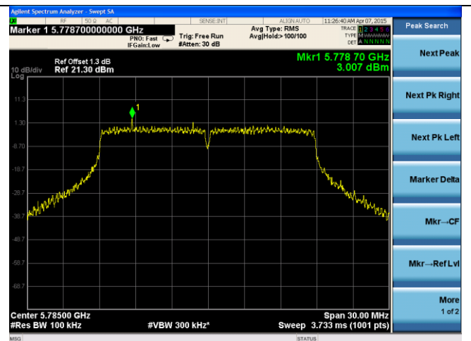
21dB ANT-PSD-802.11n-HT20-5785M-chain2
