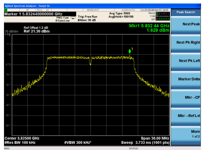
14dB ANT-PSD-802.11a-5825M-chain2
