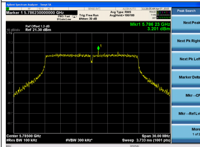
14dB ANT-PSD-802.11n-HT20-5785M-chain1
