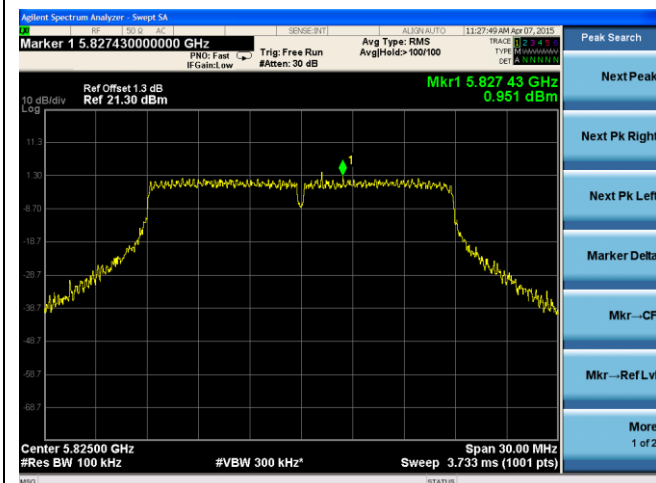
14dB ANT-PSD-802.11n-HT20-5825M-chain1
