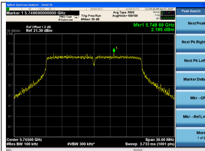
21dB ANT-PSD-802.11n-HT20-5745M-chain1
