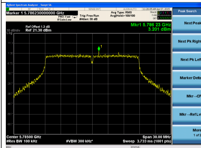
21dB ANT-PSD-802.11n-HT20-5785M-chain1
