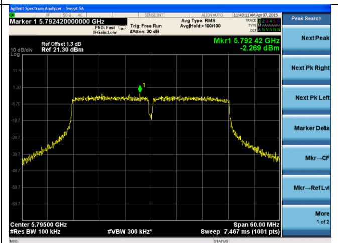
21dB ANT-PSD-802.11n-HT40-5795M-chain2
