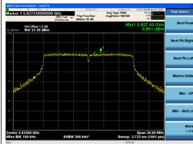
24dB ANT-PSD-802.11n-HT20-5825M-chain1
