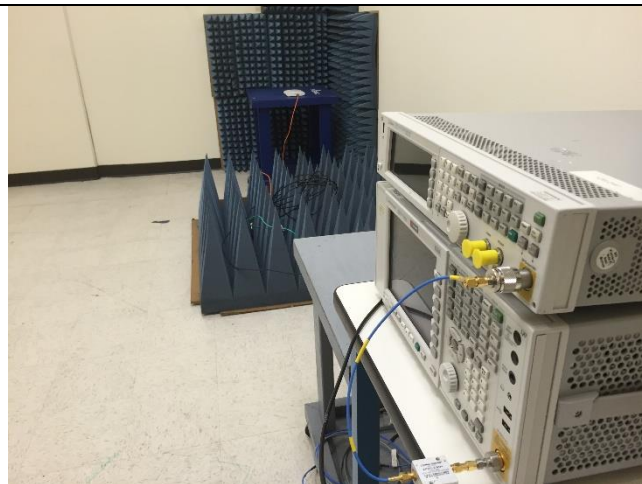
DFS set up – Back View
