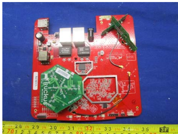
Main Board Top View without shielding
