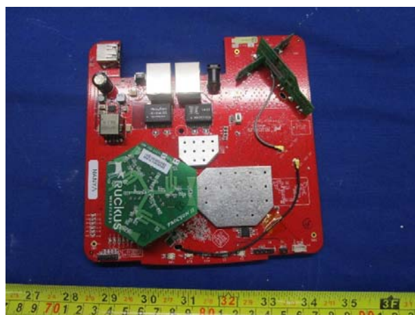
Modem Board Top View
