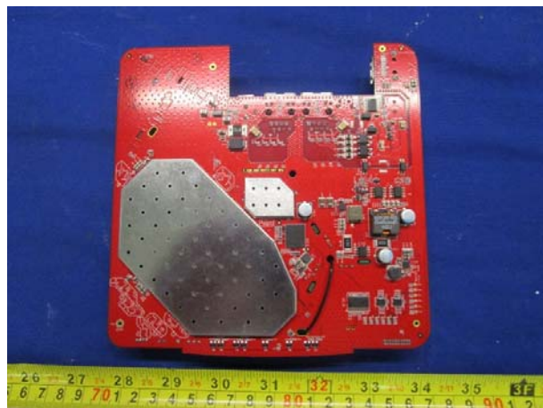
Modem Board Bottom View
