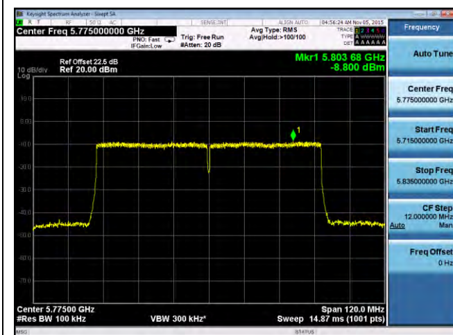
PSD-802.11ac-80M-5775M-chain0
