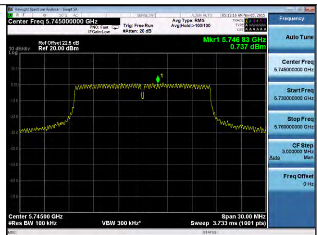
PSD-802.11a-5745M-chain1
