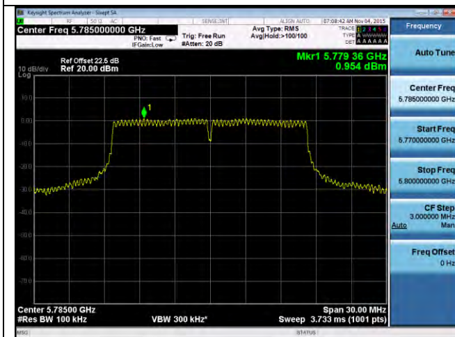
PSD-802.11a-5785M-chain0
