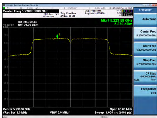
PSD-802.11n-40M-5230M-chain0
