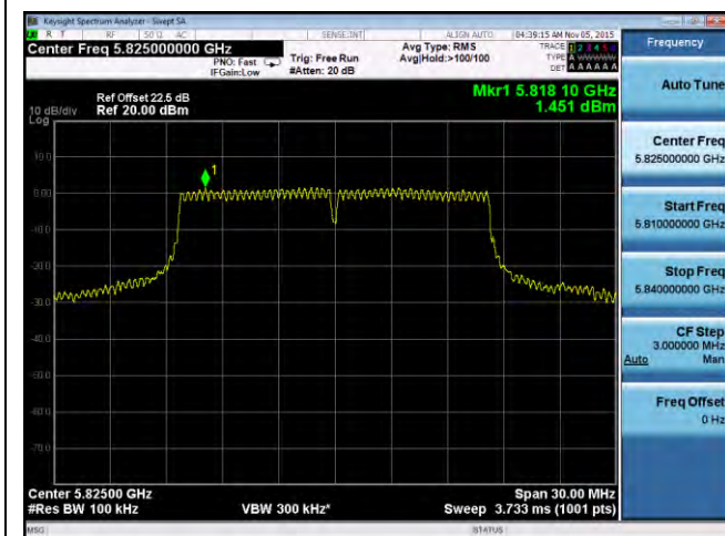
PSD-802.11a-5825M-chain0
