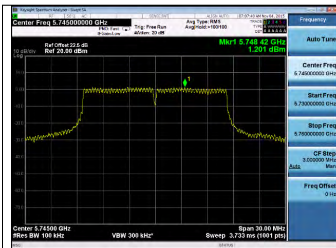
PSD-802.11a-5745M-chain0
