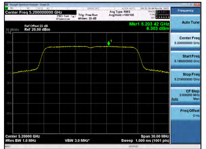
PSD-802.11n-20M -5200M-chain1
