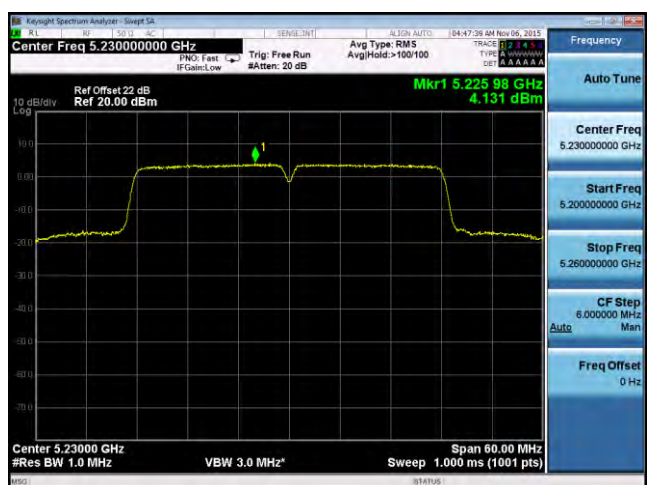
PSD-802.11n-40M-5230M-chain1
