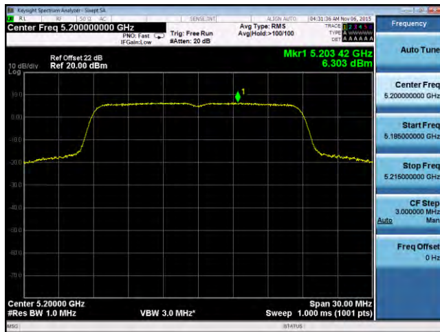
PSD-802.11n-20M -5200M-chain0
