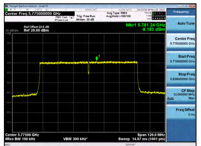
PSD-802.11ac-80M-5775M-chain1
