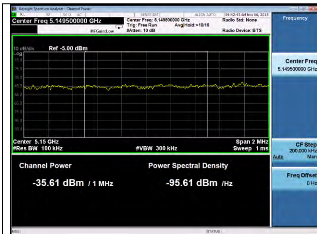
Band Edge -802.11n-20M -5180M-chain0
