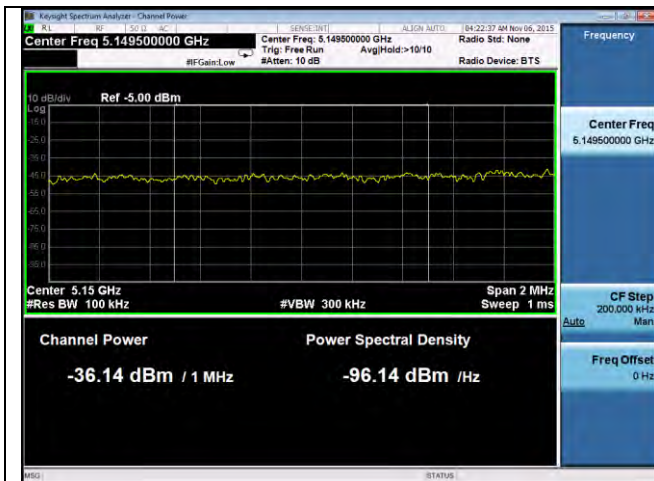
Band Edge-802.11a-5180M-chain0
