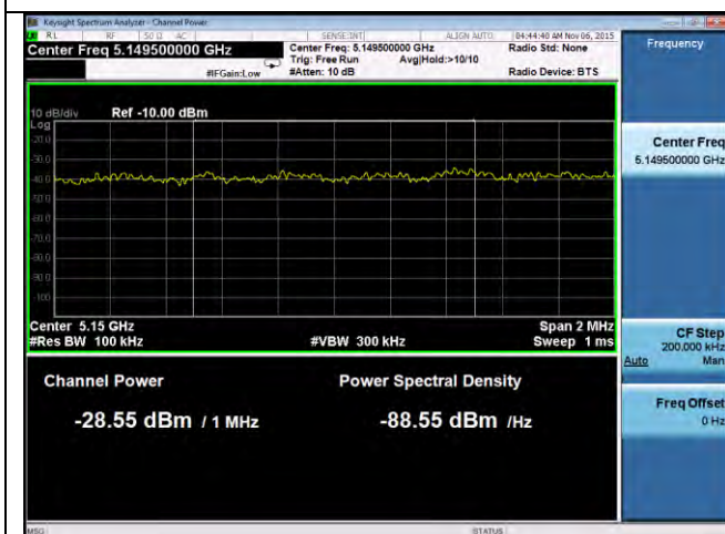
Band Edge -802.11n-40M -5190M-chain0
